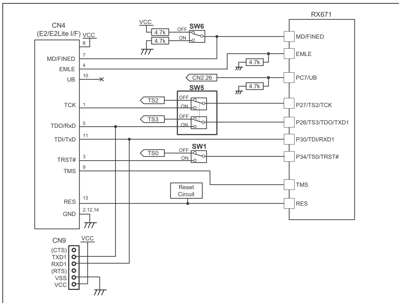
Figure 2-5. RX671 Operating Mode Setting CircuitPower Supply
