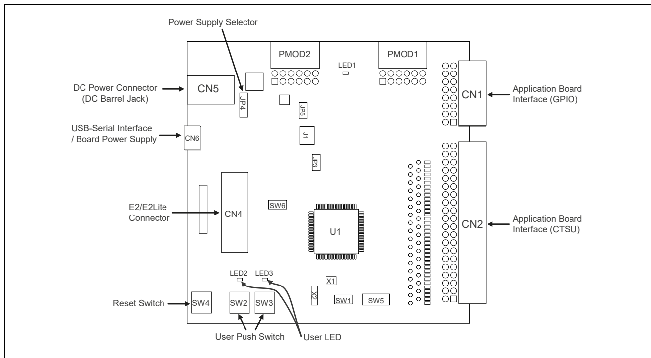
Figure 2-2. Parts Location
