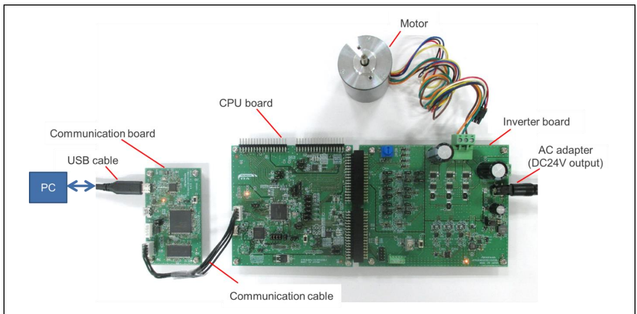
Figure 4-5 Connection Example
