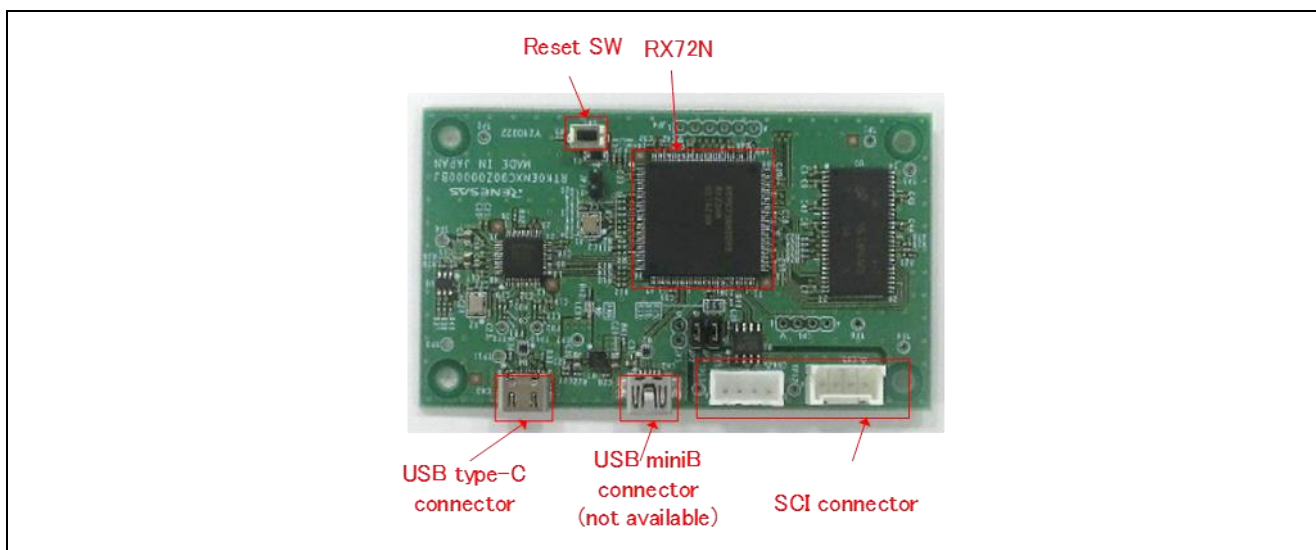
Figure 4-2 Communication board
