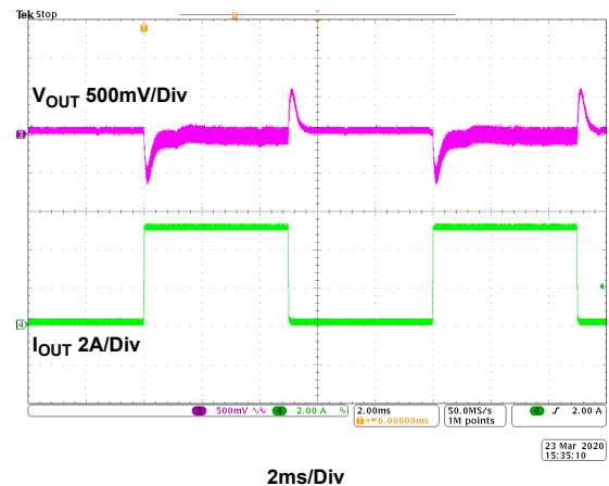
Figure 21. Load Transient, V_{IN} = 36V , I_{OUT} = 0A to 5A , 2.5A/\mu s , CCM
