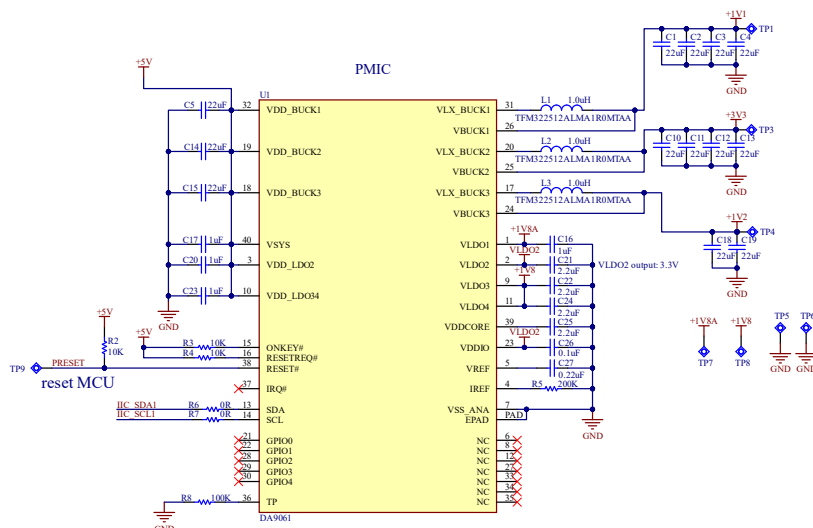
Figure 3-1 PMIC
