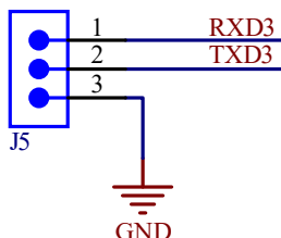
Figure 3-13 UART Interface
