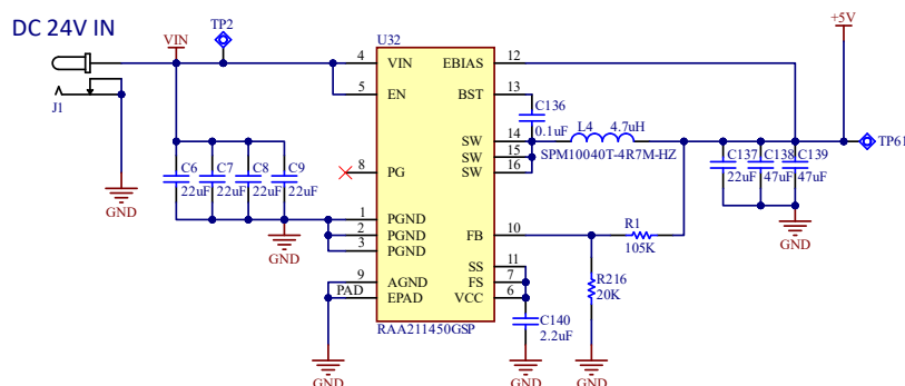
Figure 3-3 12-24V DC power supply of controller board
