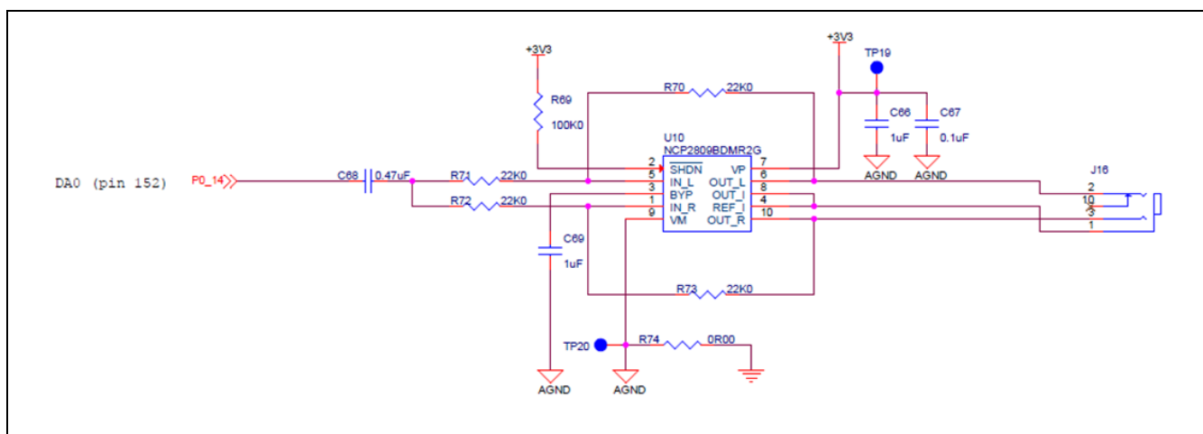
Figure 4.10 Audio output
