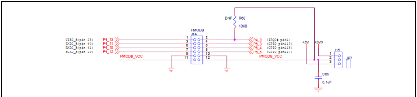
Figure 4.5 PMODB interface
