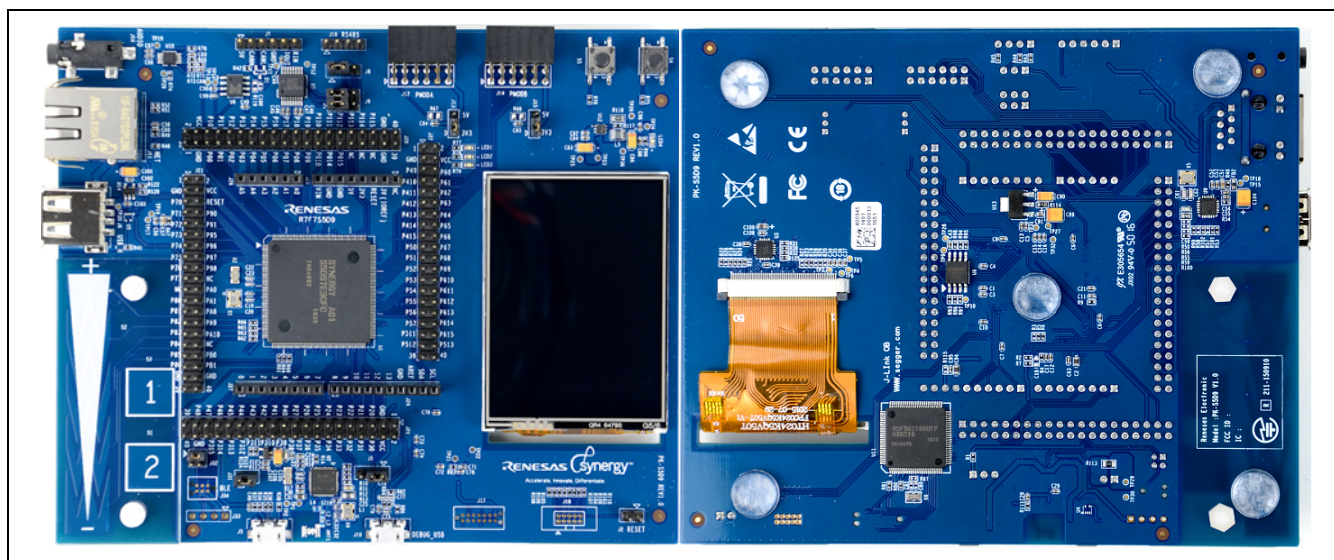
Figure 1.1 PK-S5D9 board
