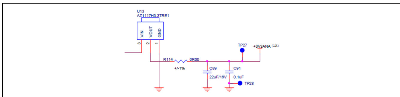
Figure 3.4 Measuring analog current consumption on the MCU
