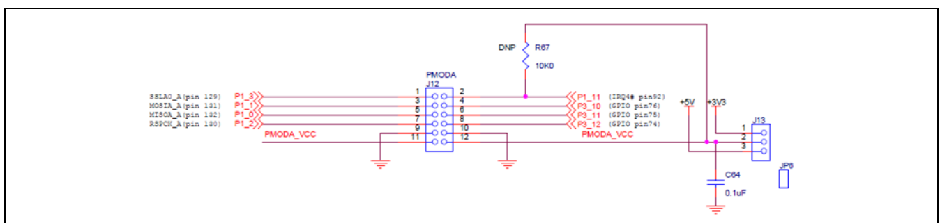
Figure 4.4 PMODA interface
