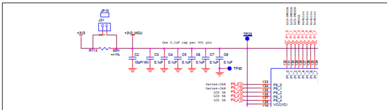
Figure 3.3 Measuring digital current consumption on the MCU
