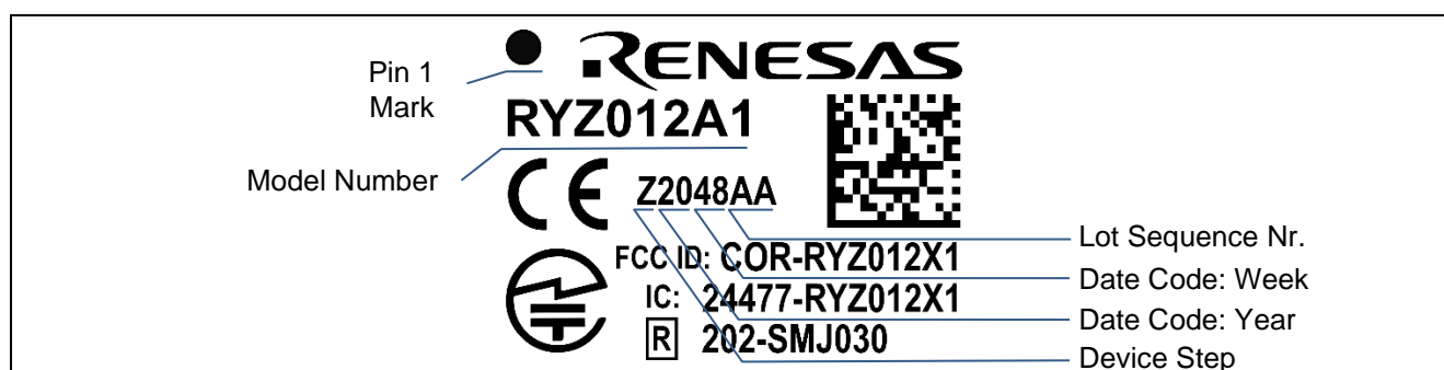
Figure 5. Marking diagram
