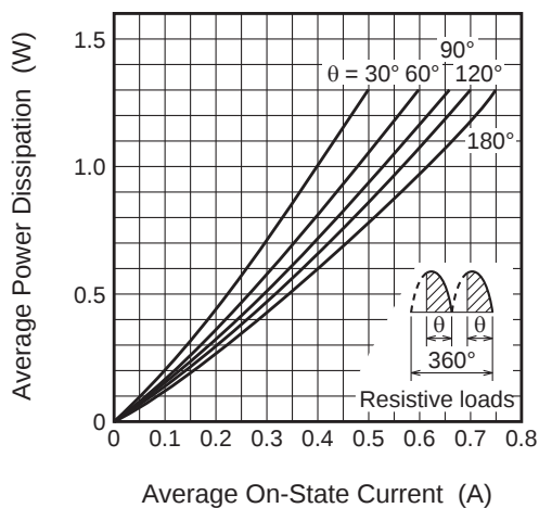
Maximum Average Power Dissipation (Single-Phase Full Wave)
