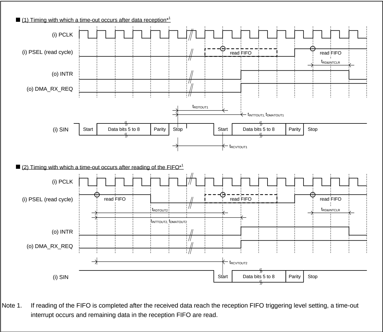
Figure 31.4-8 Time-out Timing
