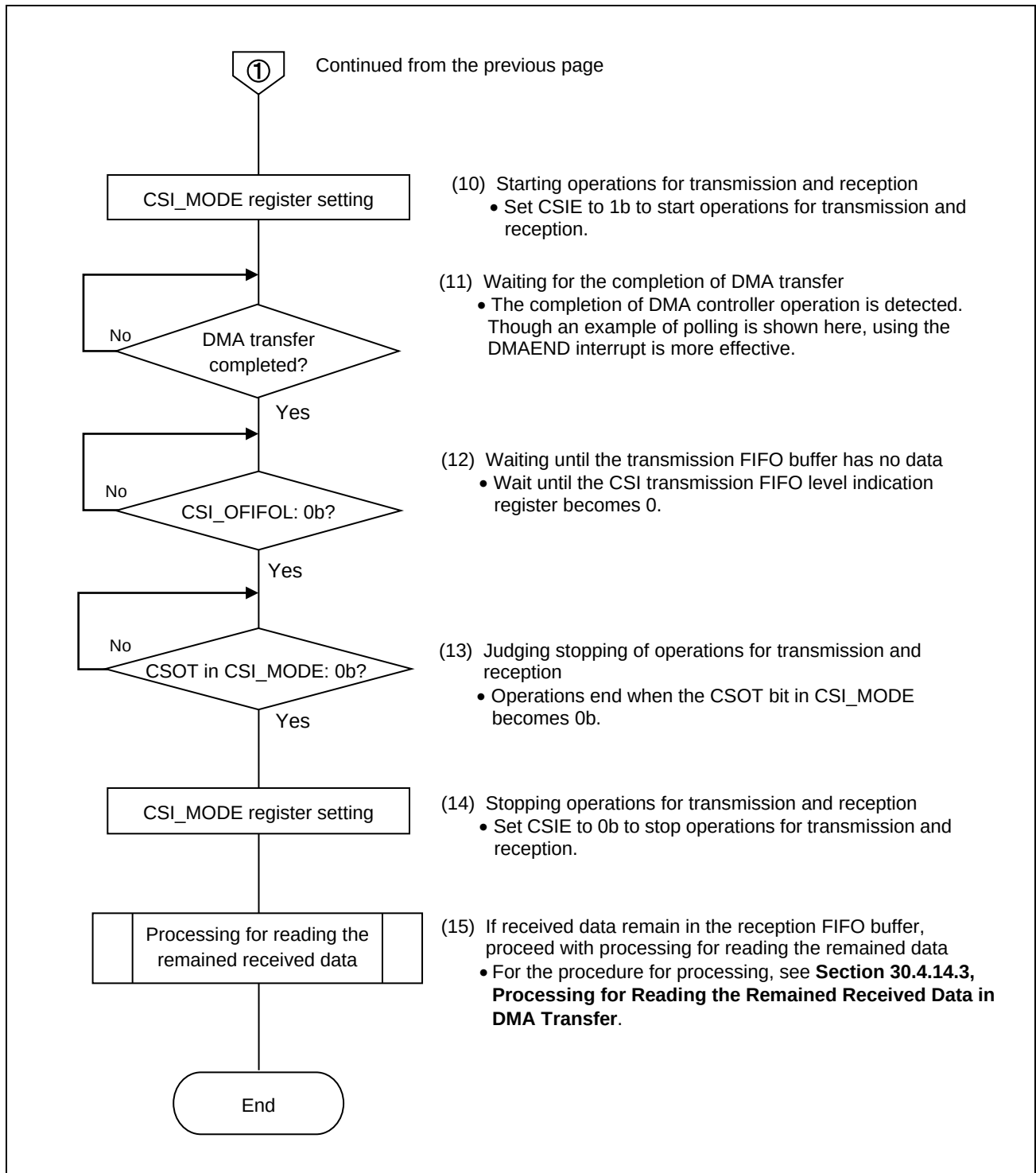
Figure 30.4-23 Flow of Operations of DMA Transfer in Master Transmission/Reception Mode (Continuous Data Transmission) (2/3)
