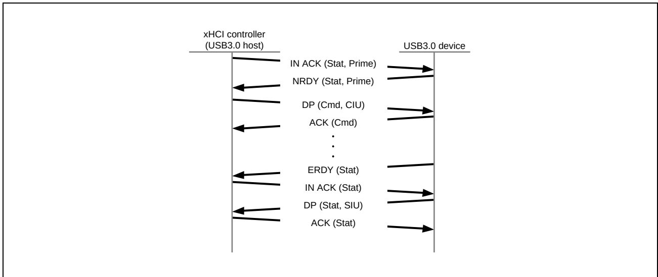
Figure 26.6-34 Example SuperSpeed UASP Non-Data Transfer
