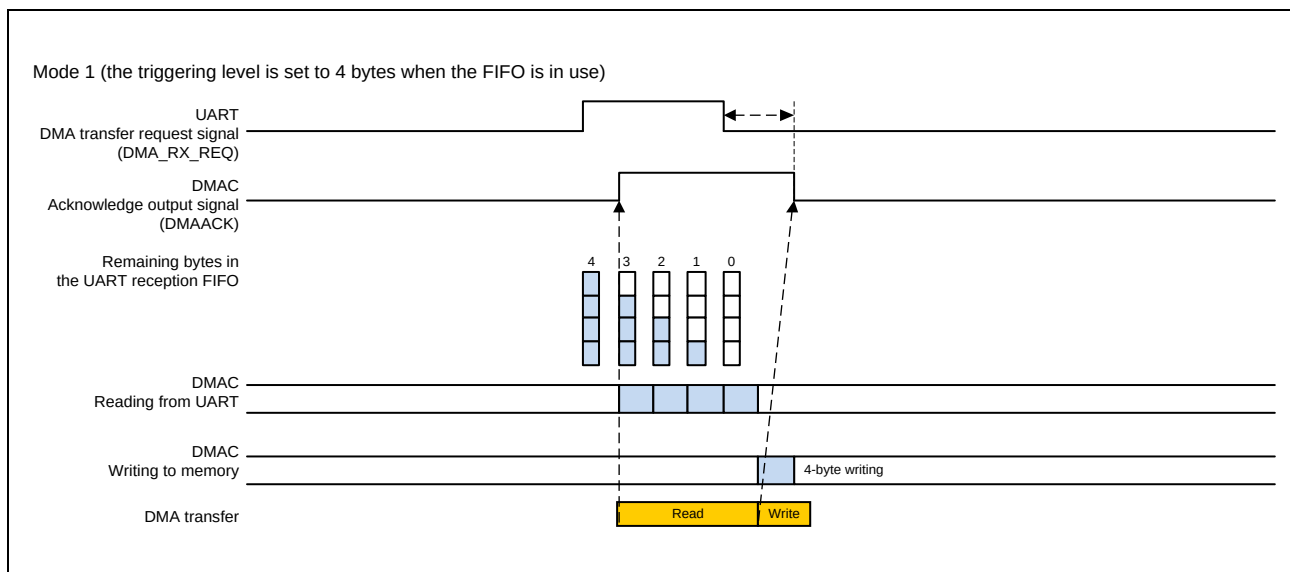
Figure 31.4-5 Example Timing of DMA Transfer for Reception
