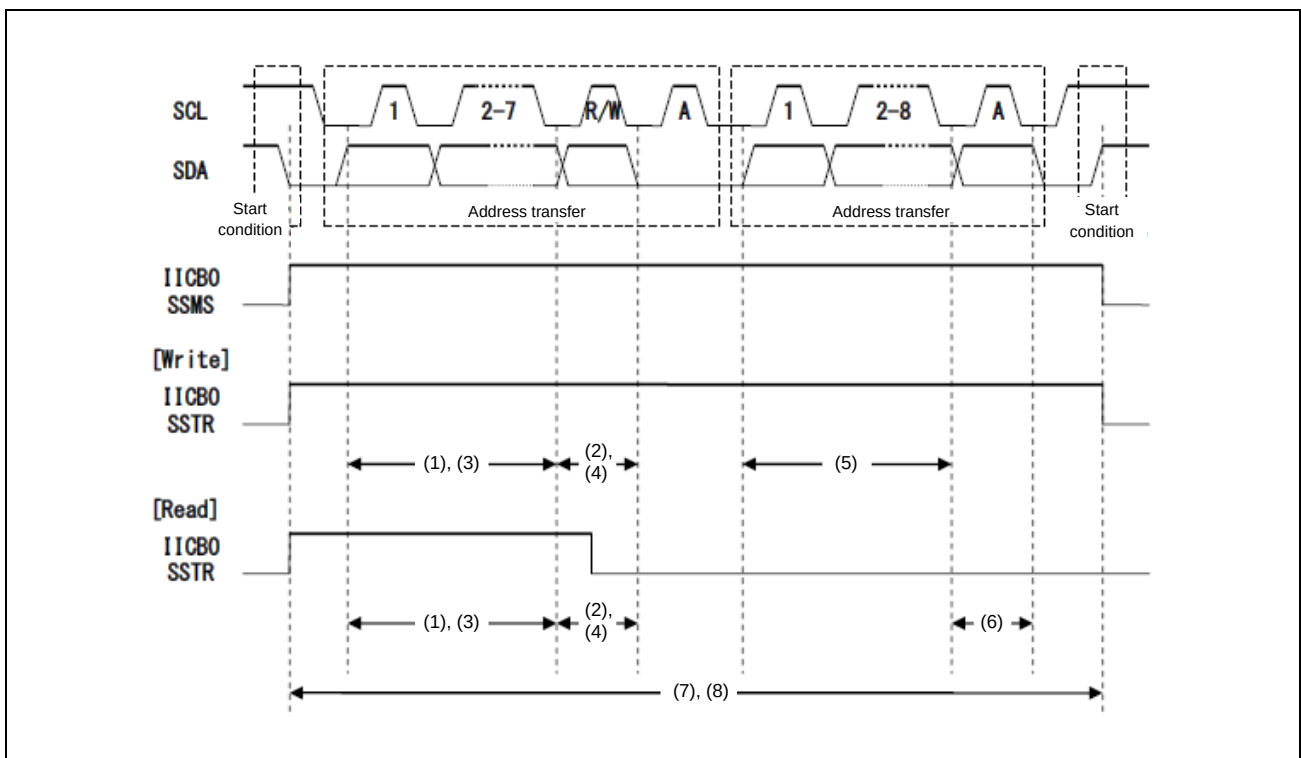
Figure 29.6-12 Arbitration Checking Range (from (1) to (8))
