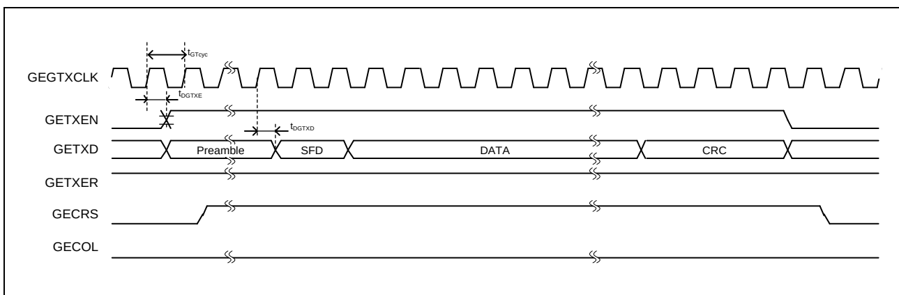
Figure 40.5-7 Transmission Timing
