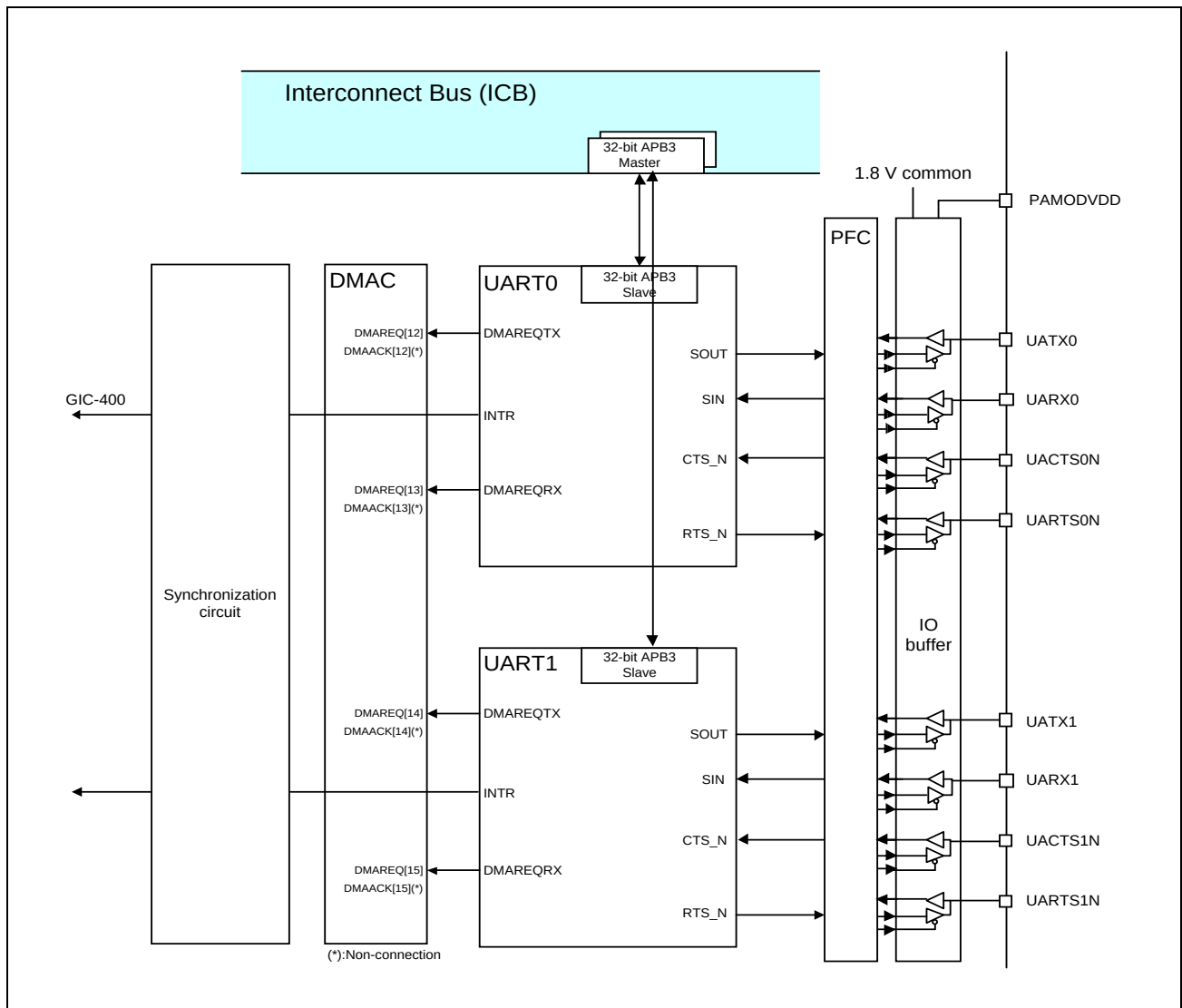
Figure 31.1-1 Connection Configuration
