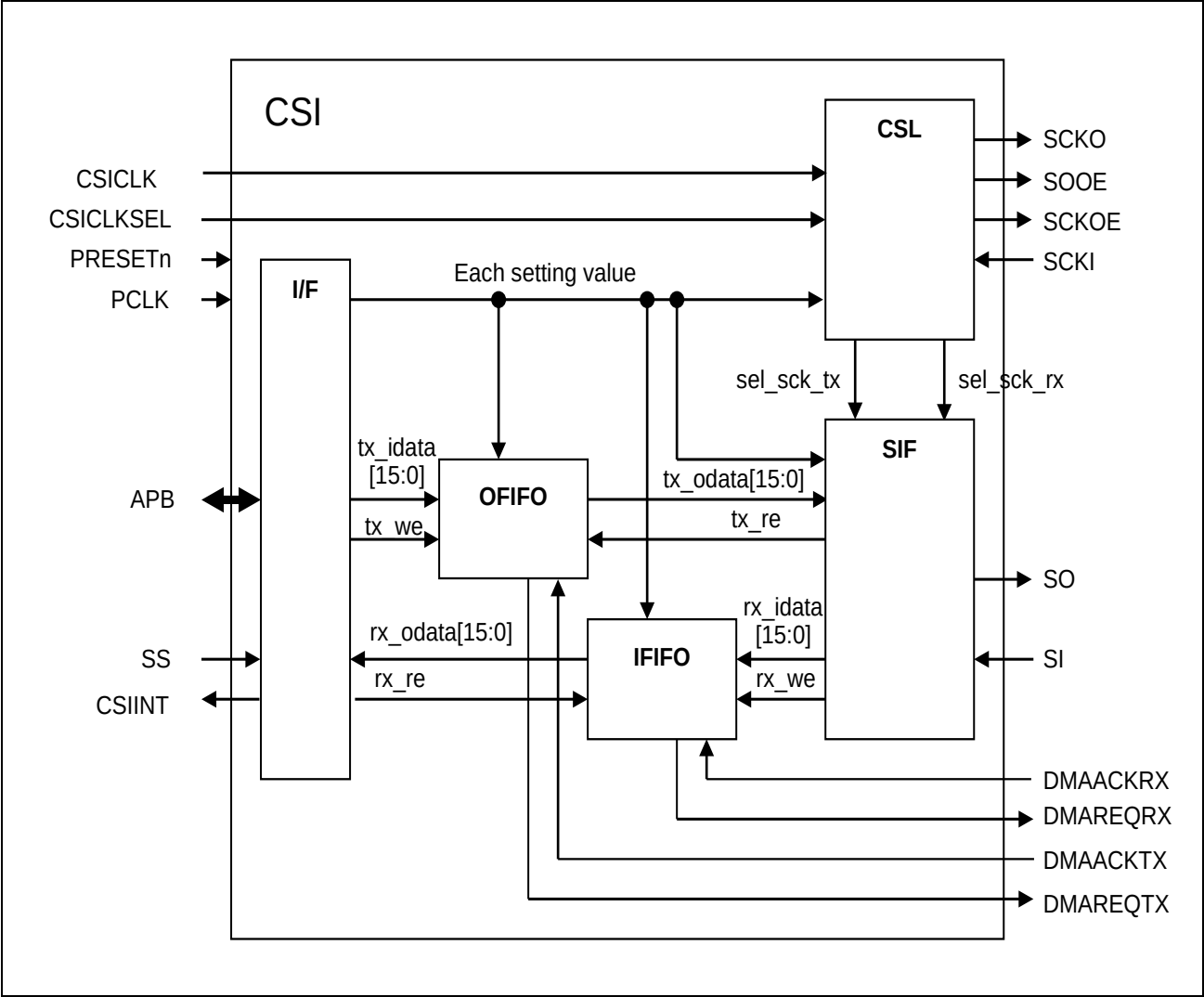
Figure 30.1-1 Block Diagram
