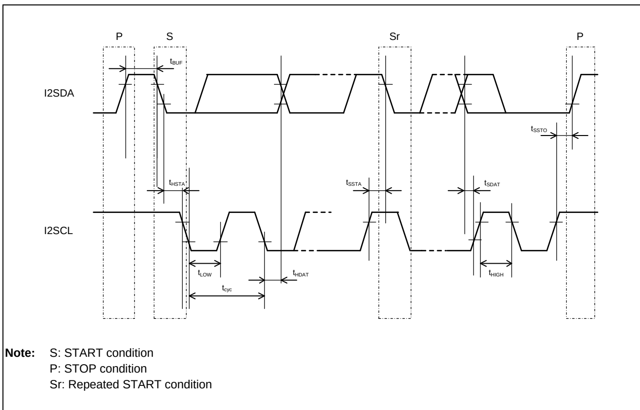
Figure 40.5-1 IIC Timing
