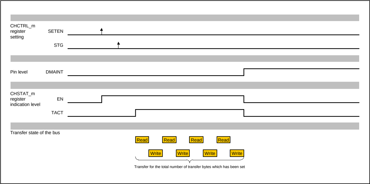
Figure 18.6-27 DMAC State Example 2 (Software Request)
