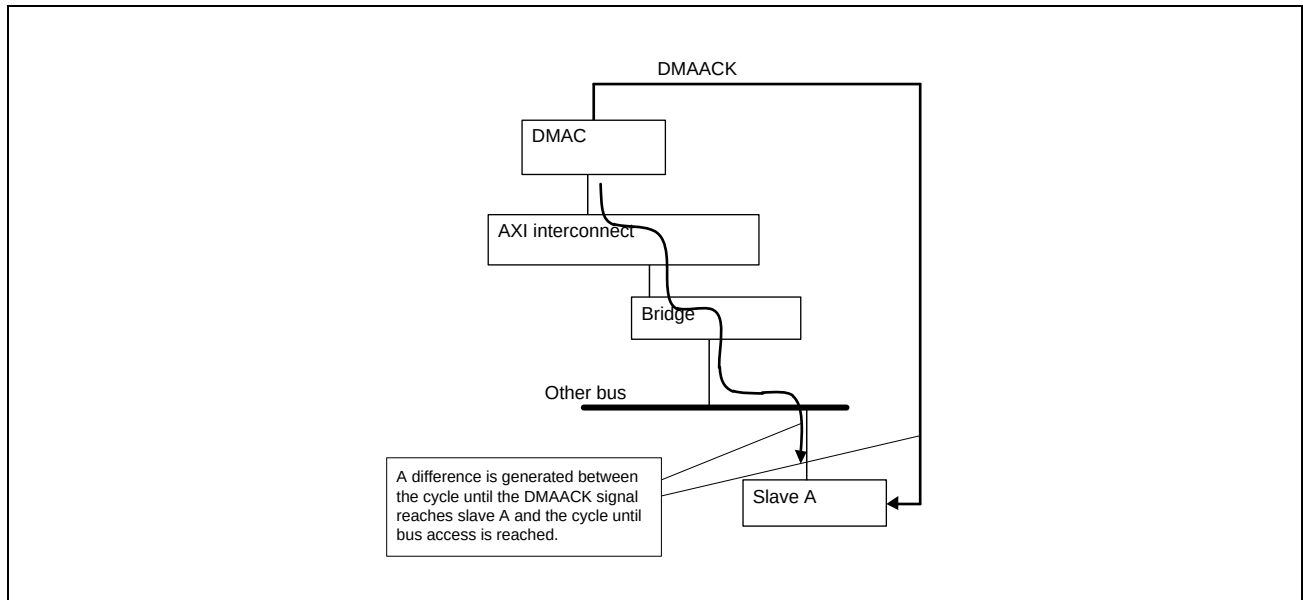
Figure 18.8-2 Example: Circuit where a Delay from Activation of the DMAACK Signal to Actual Access is Caused via a Bus Bridge
