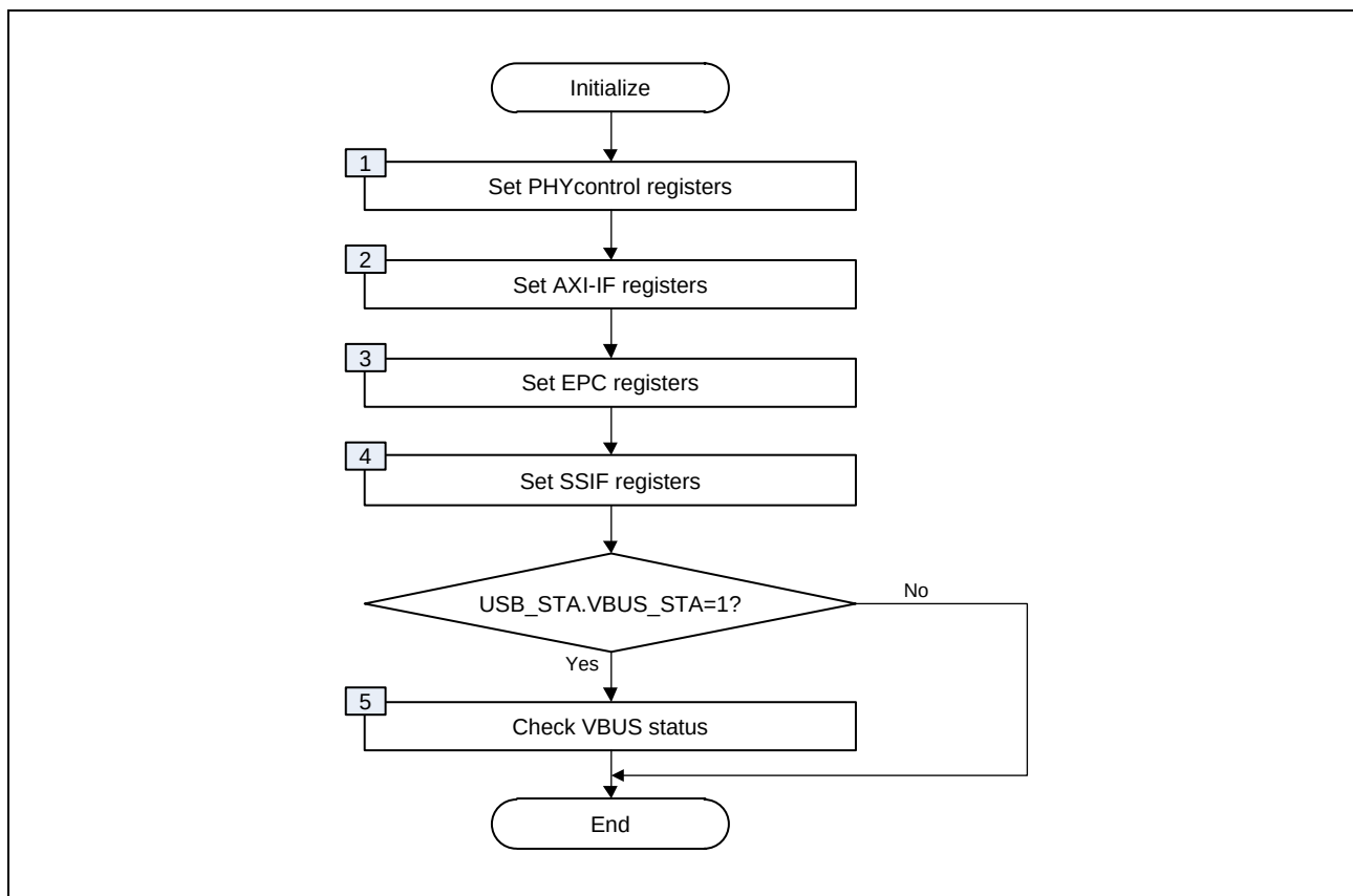
Figure 26.6-19 Initialization Flow
