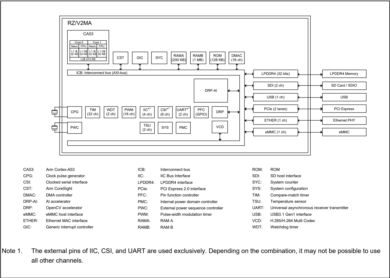
Figure 1.4-1 Block Diagram
