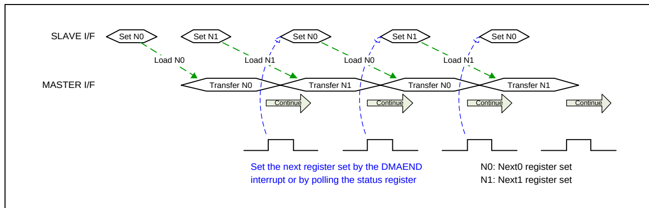
Figure 18.7-5 Schematic View of Next Register Continuous Execution
