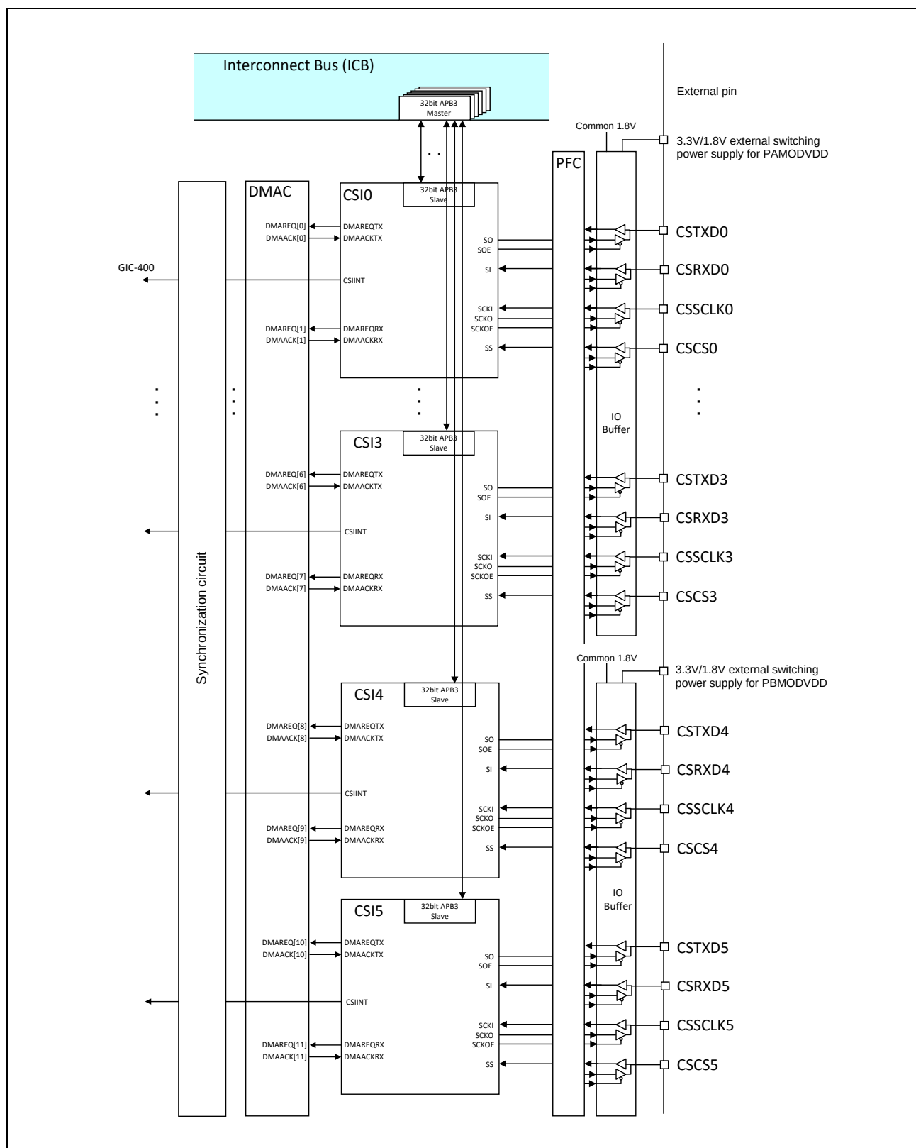
Figure 30.1-2 Connection Configuration
