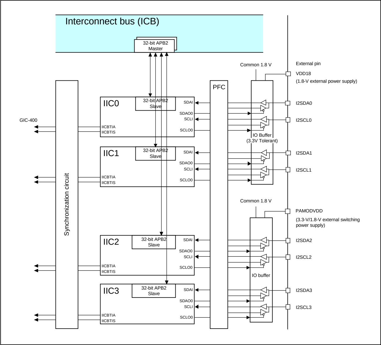
Figure 29.1-1 Connection Configuration
