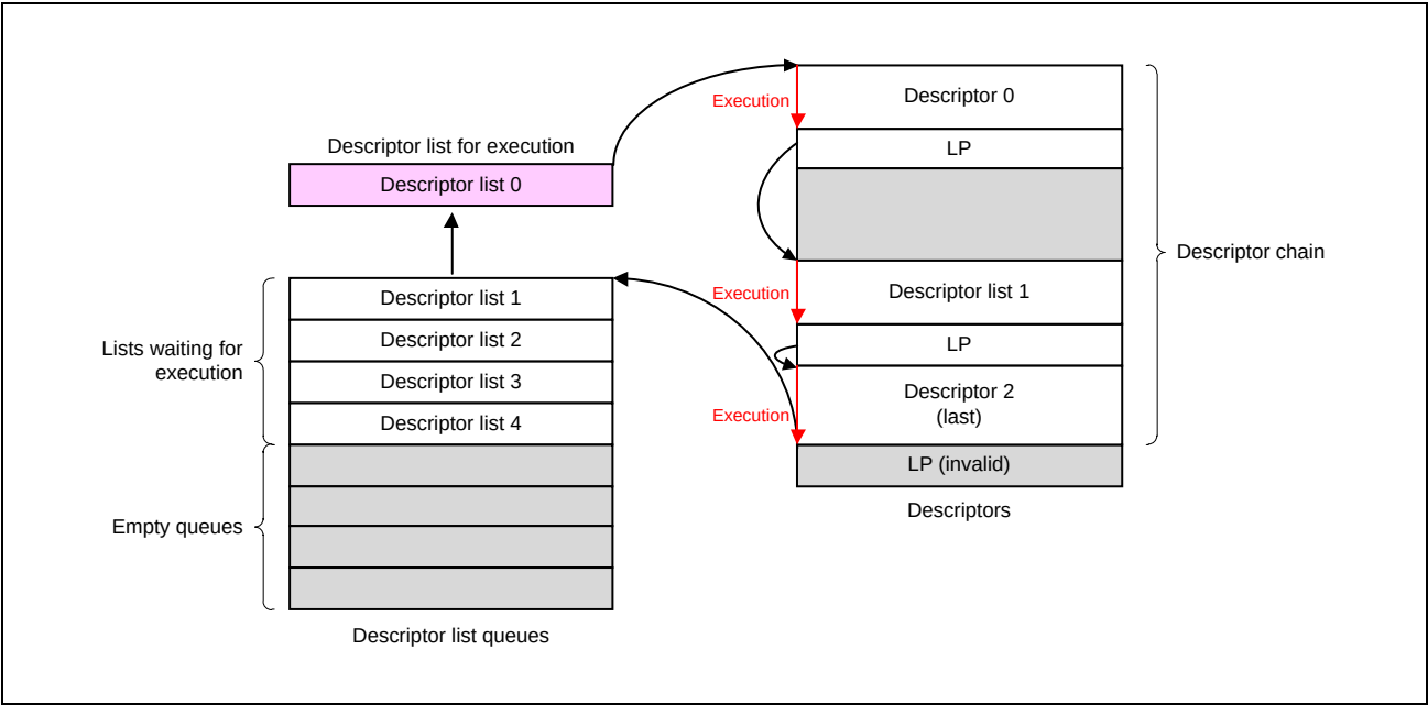
Figure 27.7-1 Descriptor Chain
