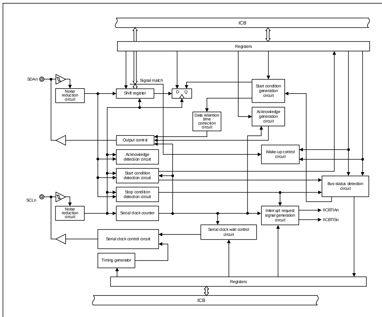
Figure 29.2-1 Block Diagram
