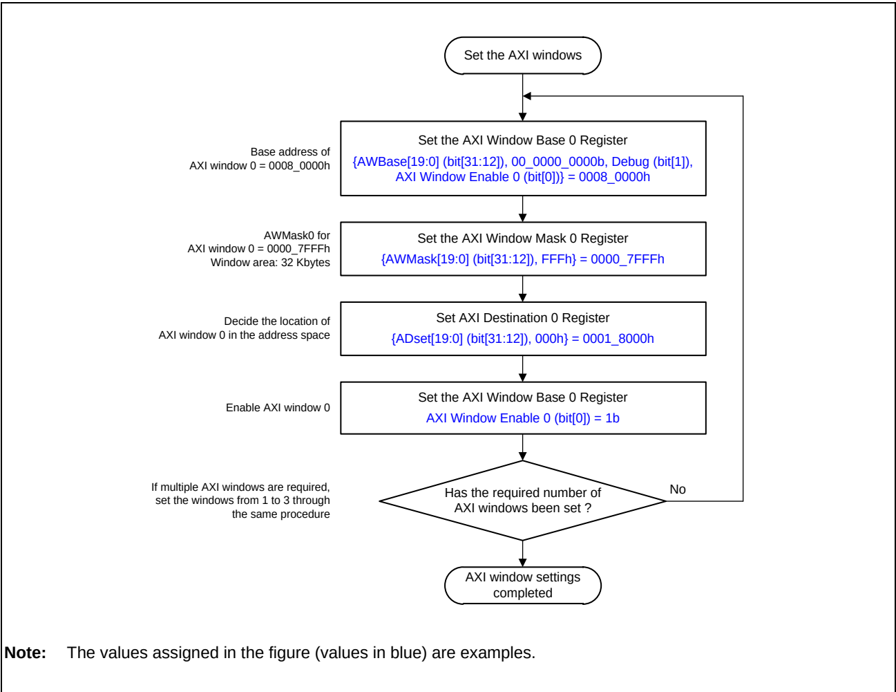
Figure 27.8-2 Example Settings of the AXI Windows
