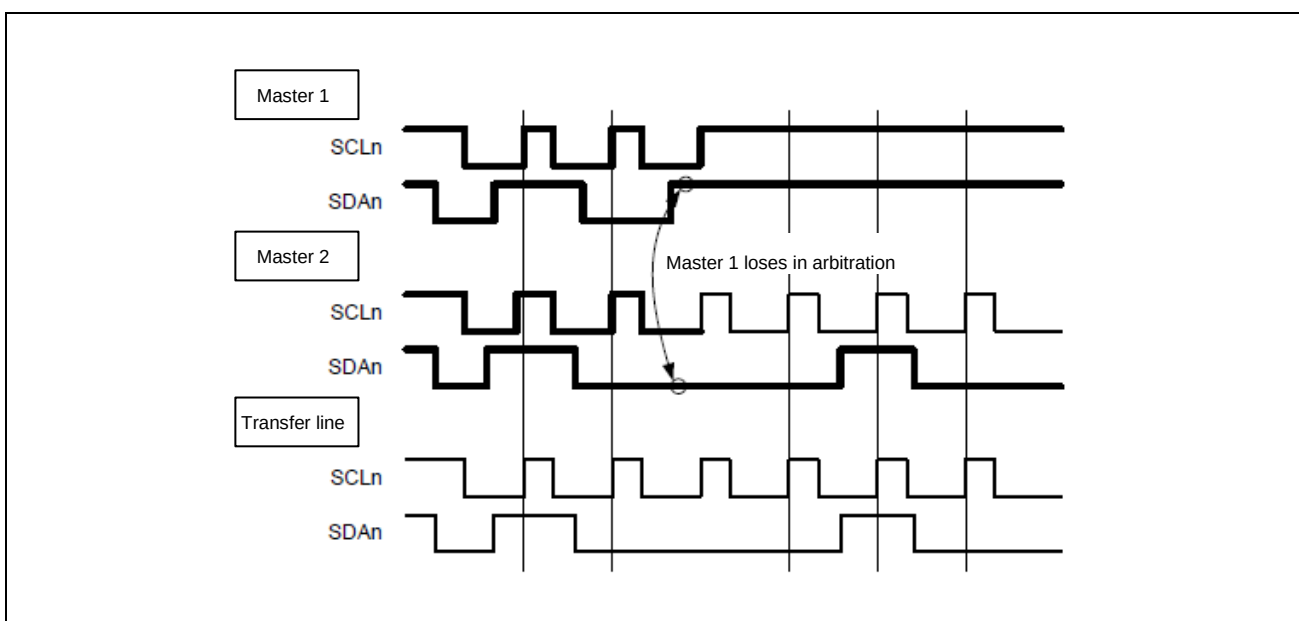
Figure 29.6-8 Example Timing of Arbitration
