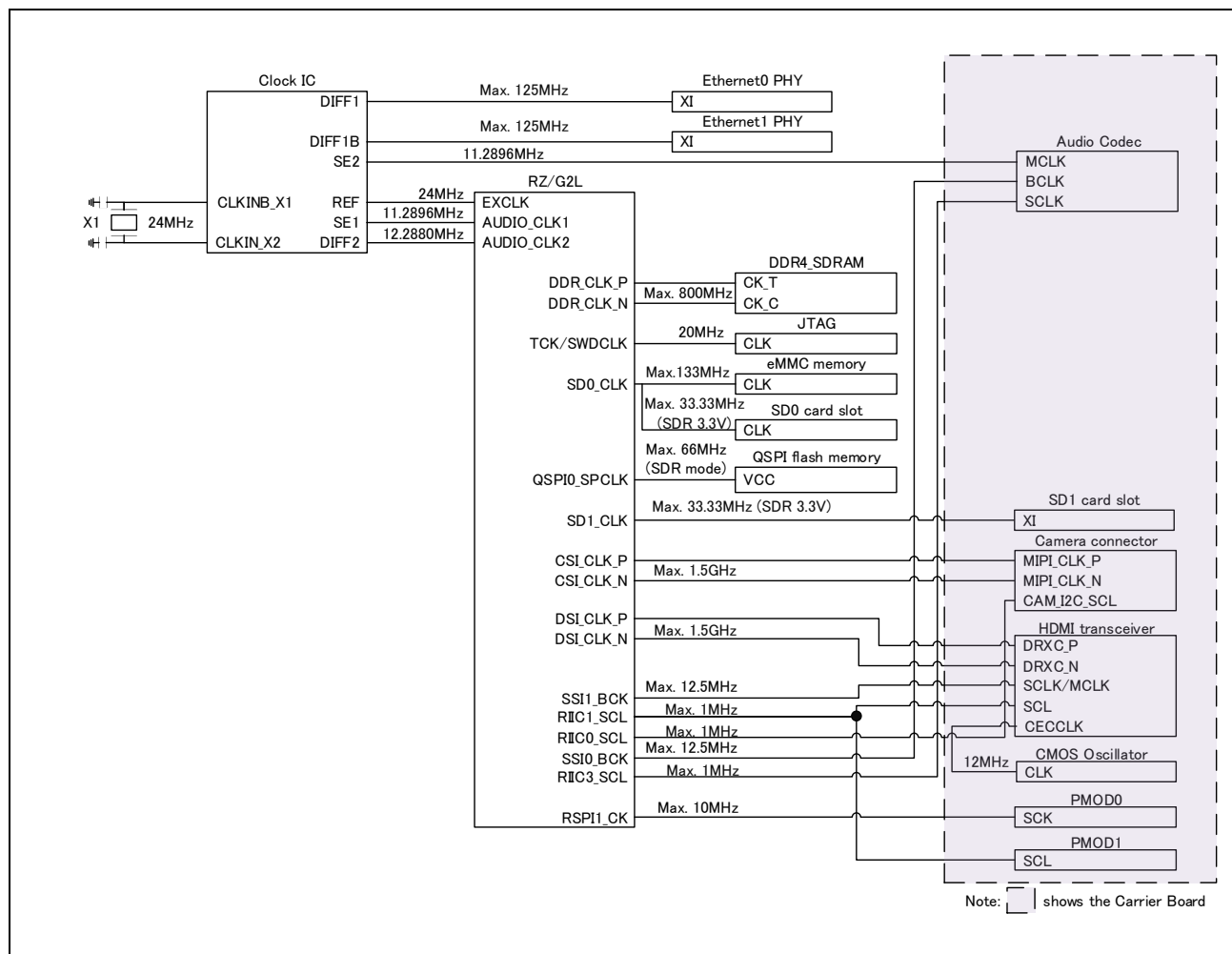
Figure 2.6 Block Diagram of Clock Configuration
