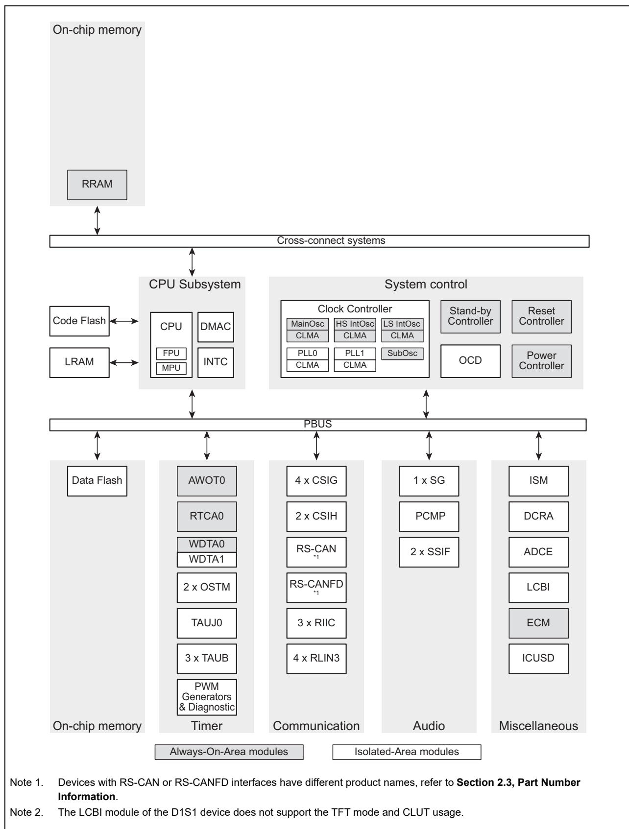
Figure 2.1 D1S1 block diagram
