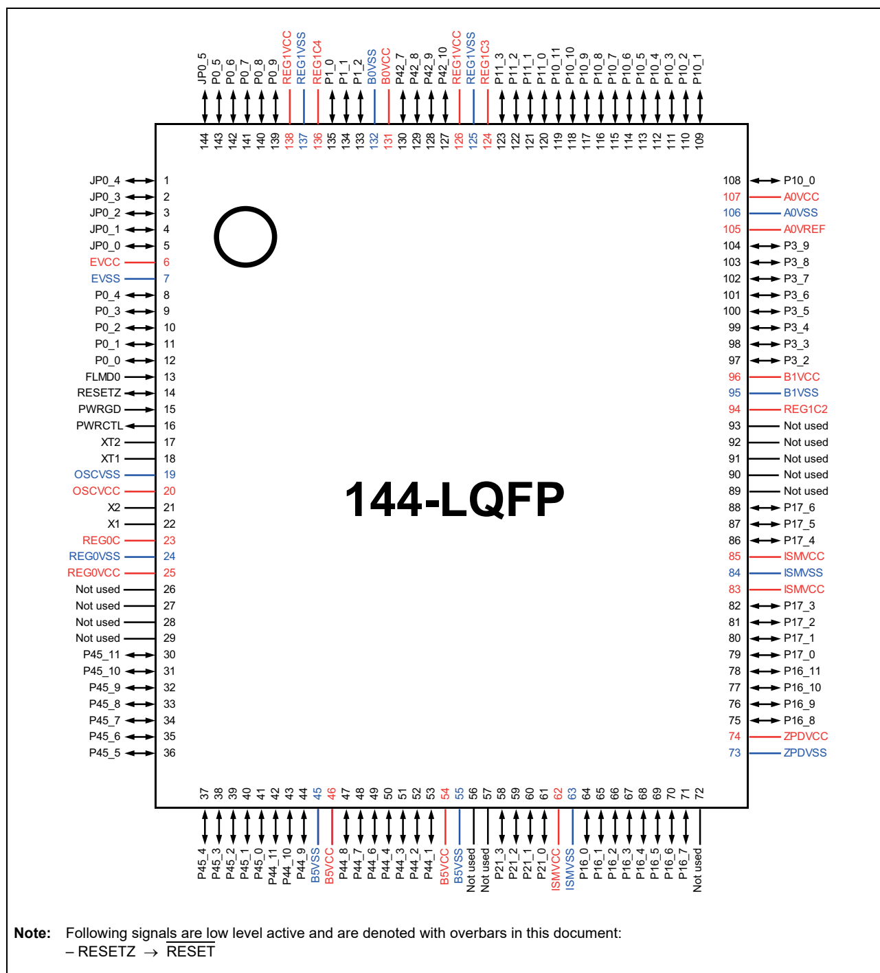
Figure 3.1 D1S1 Pin Connection Diagram (144pin LQFP package)
