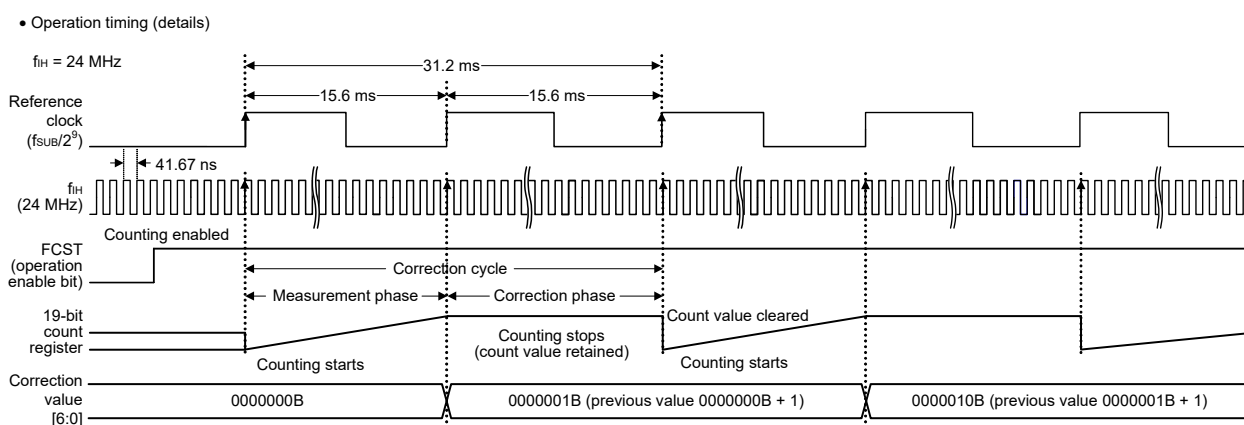
Figure 6-3. Operation Timing (Details) of High-speed On-chip Oscillator Clock Frequency Correction
