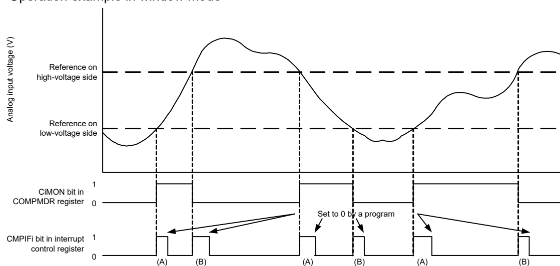
Figure 17-7. Comparator i (i = 0 or 1) Operation Example in Window Mode
