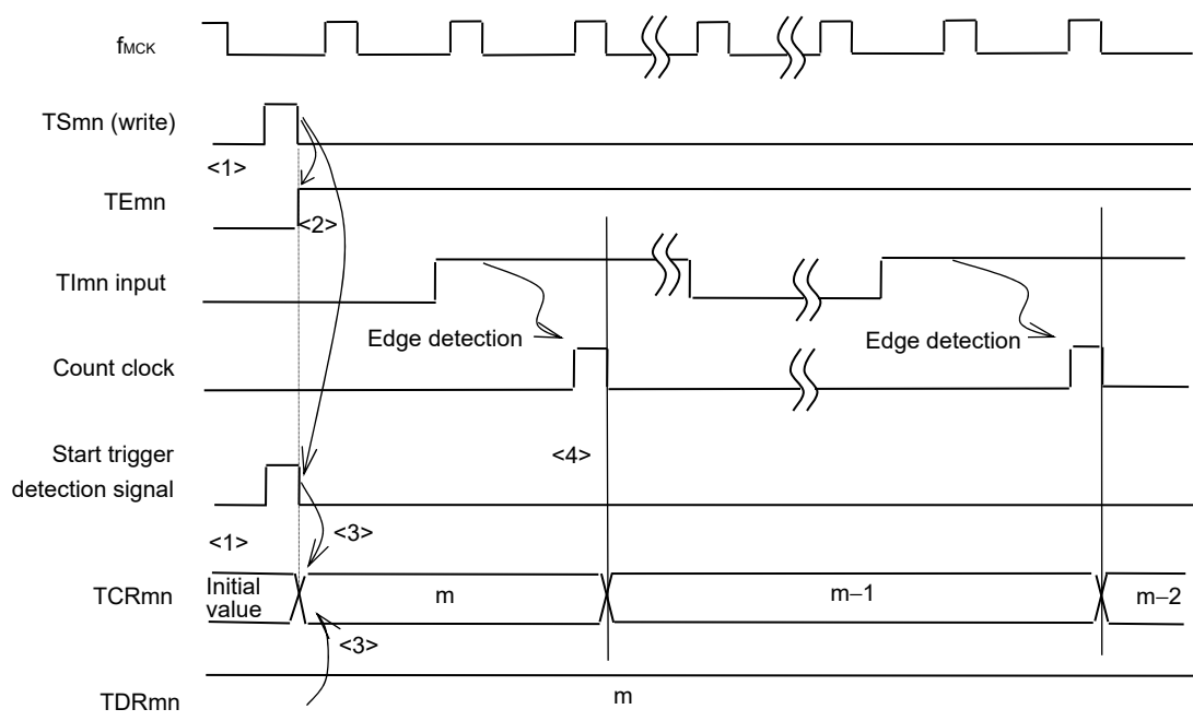
Figure 7-27. Operation Timing (In Event Counter Mode)
