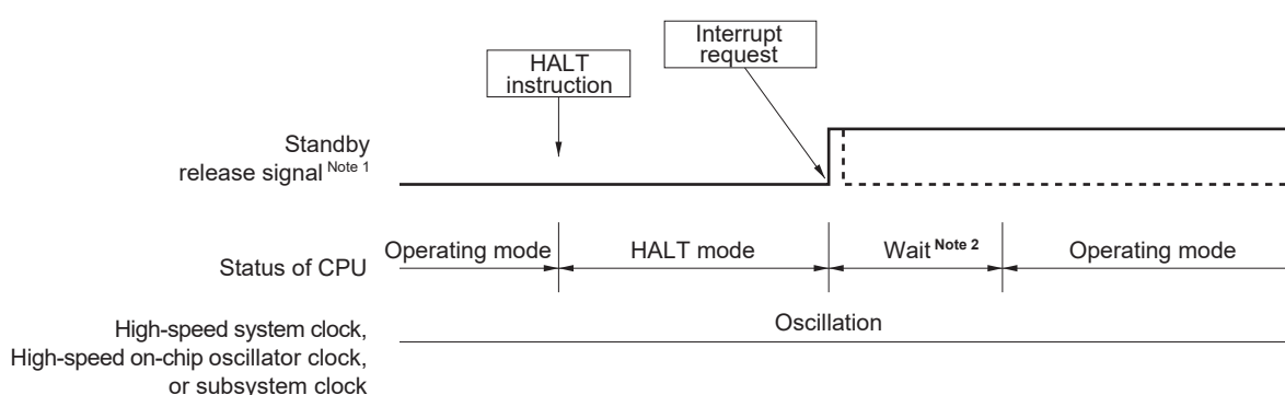
Figure 24-1. HALT Mode Release by Interrupt Request Generation
