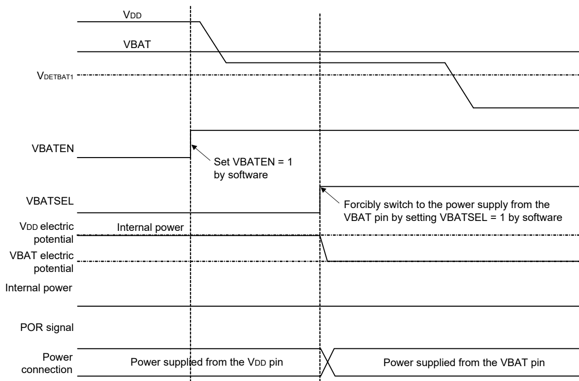
Figure 28-6. Battery Backup Operation (2) with VBATEN = 1 and VBATSEL = 1
