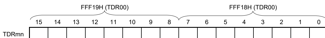
Figure 7-9. Format of Timer Data Register mn (TDRmn) (n = 1, 3)
