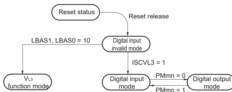
Figure 4-13. V L3 /P125 Pin Function Status Transition Diagram
