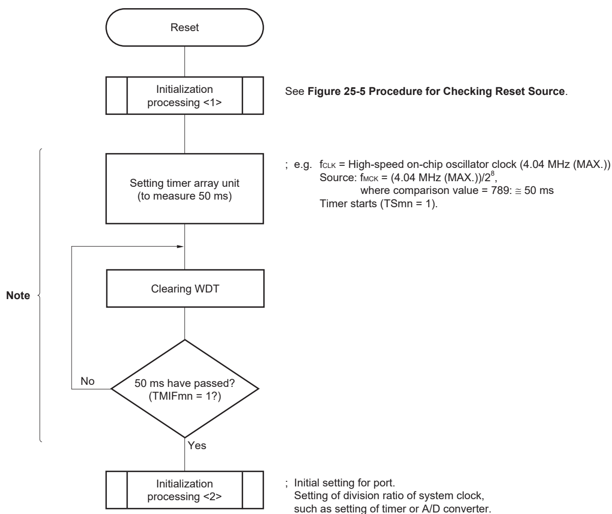
Figure 27-10. Example of Software Processing If Internal Power Supply Voltage Fluctuation is 50 ms or Less in Vicinity of LVD Detection Voltage
