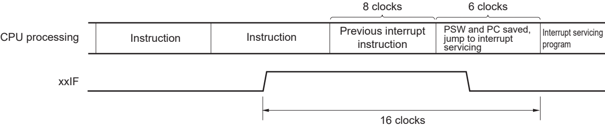
Figure 23-9. Interrupt Request Acknowledgment Timing (Maximum Time)
