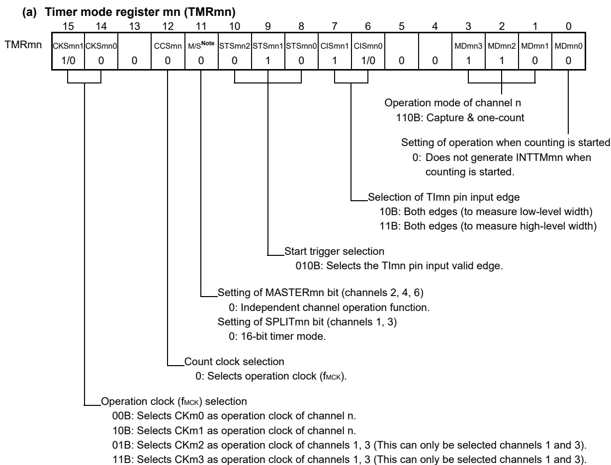
Figure 7-56. Example of Set Contents of Registers to Measure Input Signal High-/Low-Level Width
