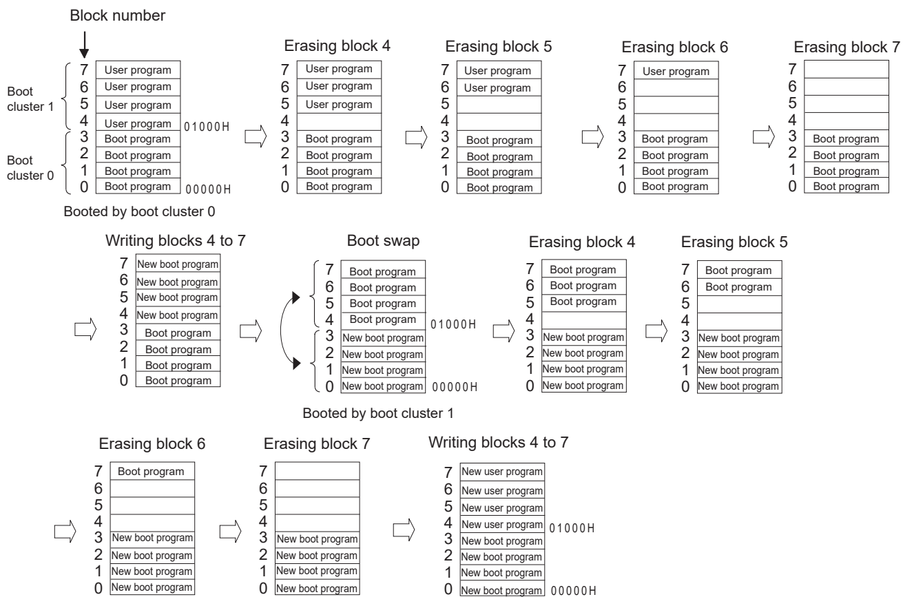
Figure 33-10. Example of Executing Boot Swapping
