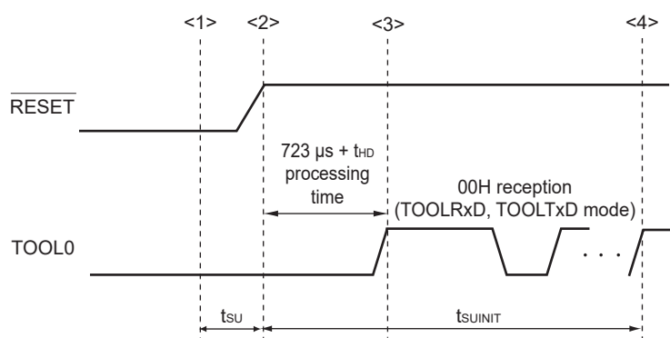
Figure 33-7. Setting of Flash Memory Programming Mode
