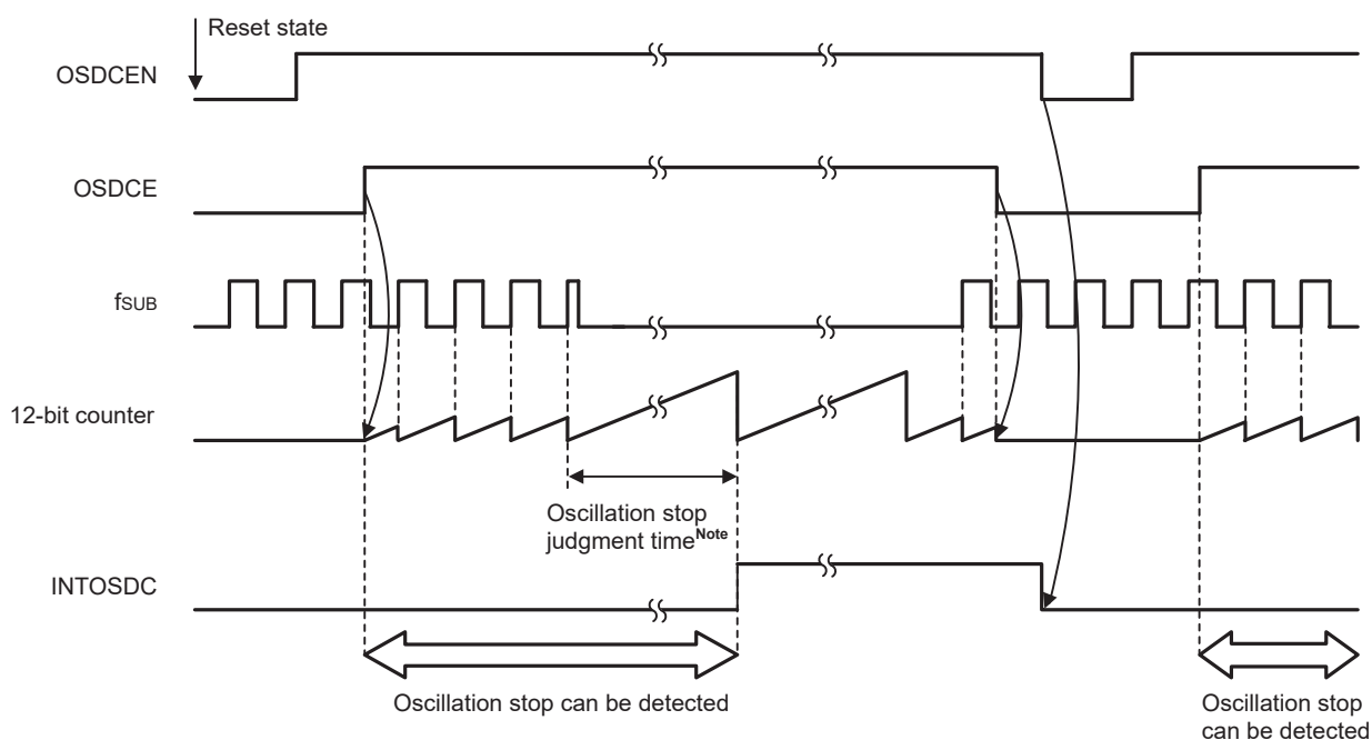
Figure 29-5. Timing of Oscillation Stop Detection by Oscillation Stop Detector
