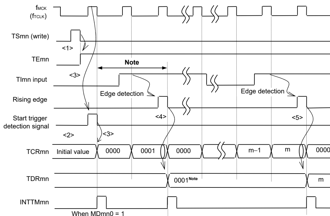
Figure 7-28. Operation Timing (In Capture Mode: Input Pulse Interval Measurement)
