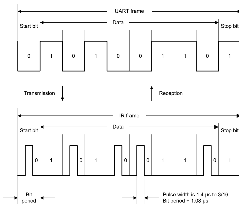
Figure 20-4. IrDA Transmission/Reception
