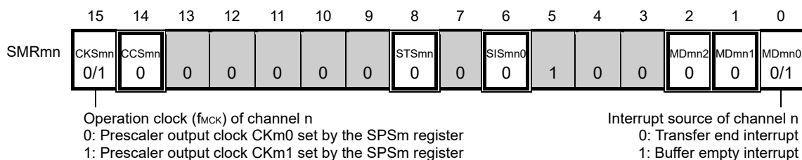
Figure 18-25. Example of Contents of Registers for Master Transmission of simplified SPI (CS100) (1/2)
