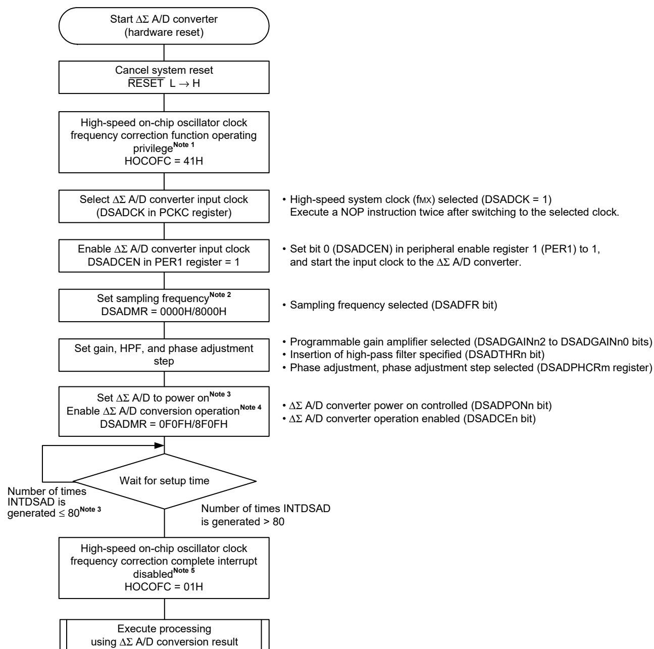
Figure 16-13. Initialization Flowchart
