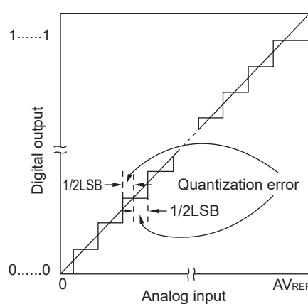
Figure 14-39. Quantization Error
