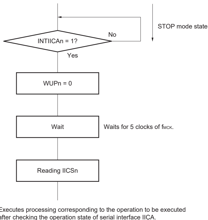
Figure 19-23. Flow When Setting WUPn = 0 upon Address Match (Including Extension Code Reception)
