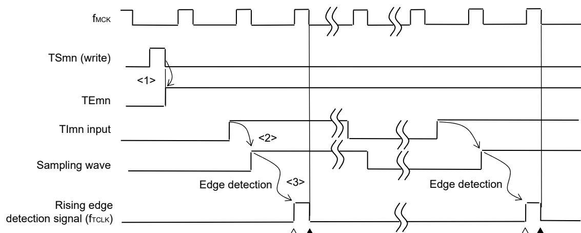
Figure 7-25. Timing of f_{CLK} and count clock ( f_{CLK} ) (When CCSmn = 1, noise filter unused)
