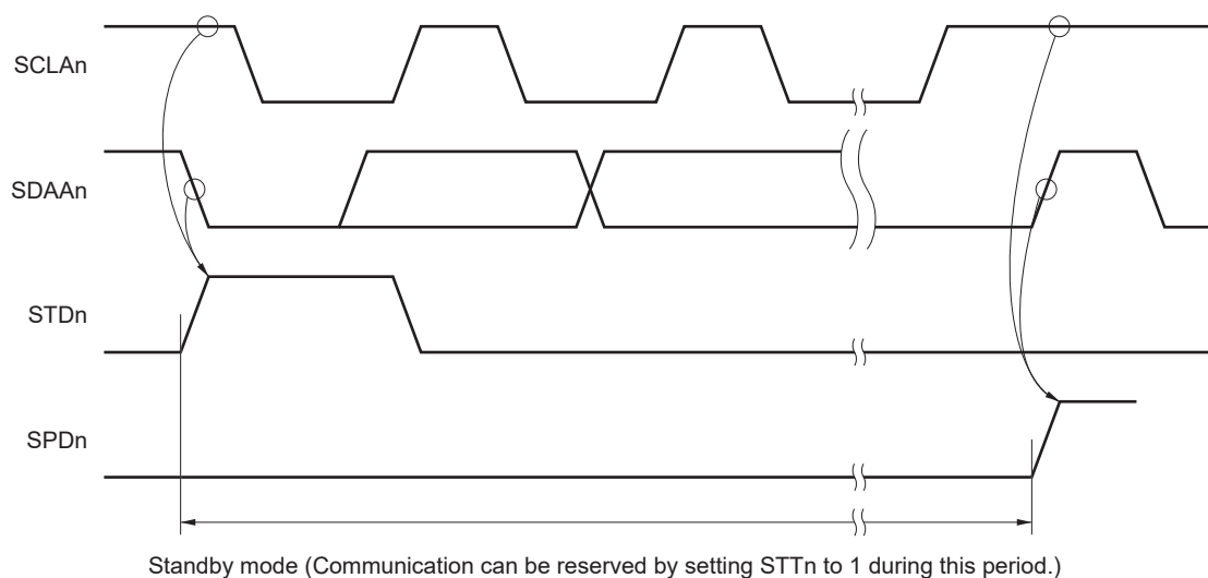
Figure 19-26. Timing for Accepting Communication Reservations
