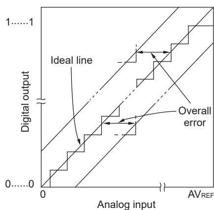
Figure 14-38. Overall Error
