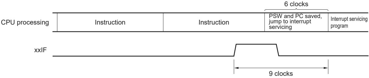
Figure 23-8. Interrupt Request Acknowledgment Timing (Minimum Time)
