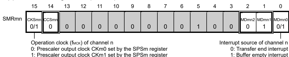
Figure 18-76. Example of Contents of Registers for UART Transmission of UART (UART0 to UART2) (1/2)
