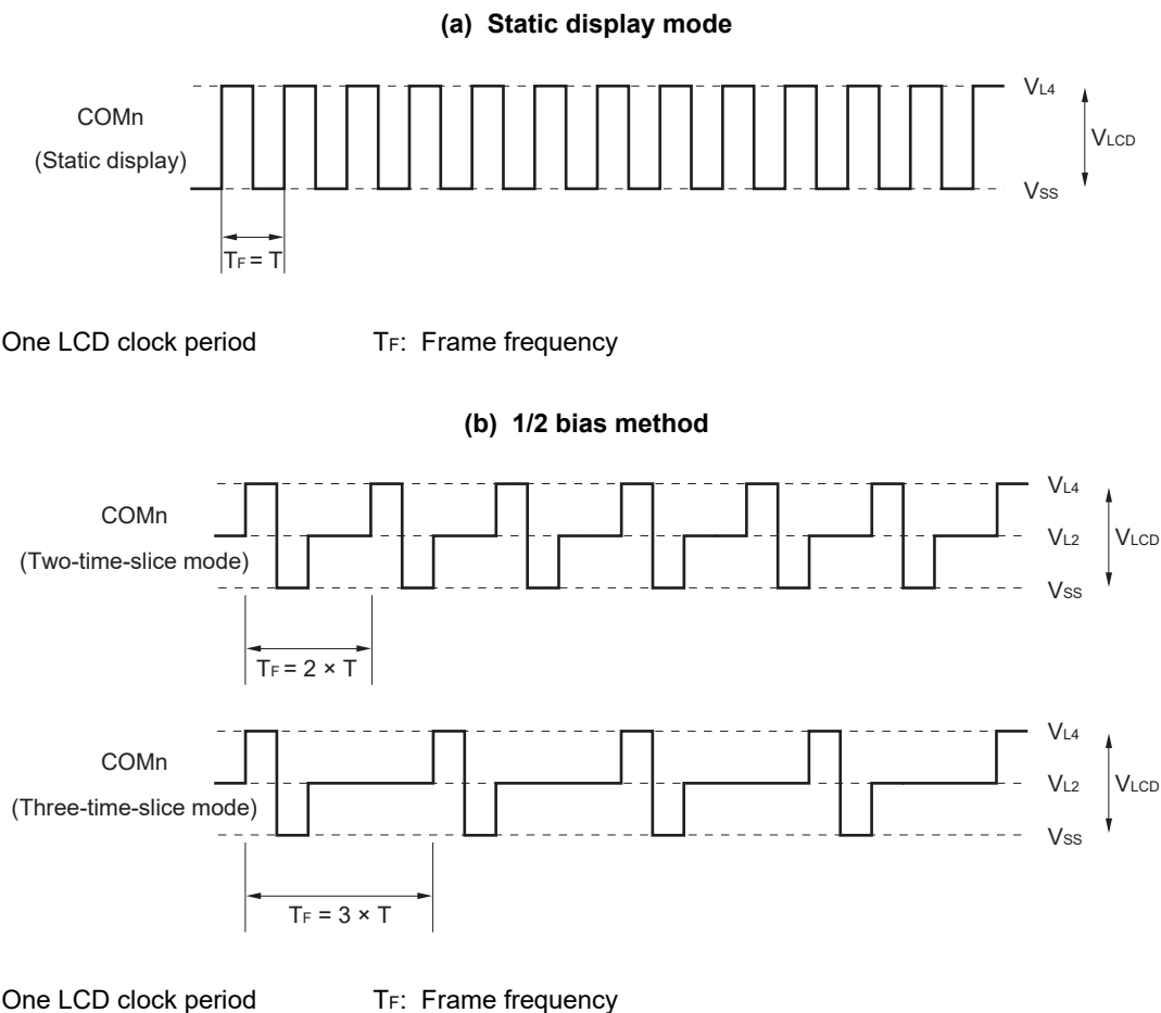
Figure 21-23. Common Signal Waveforms (1/2)
