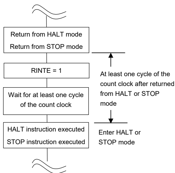
Figure 10-6. Procedure of Entering to HALT or STOP Mode After Setting RINTE to 1
