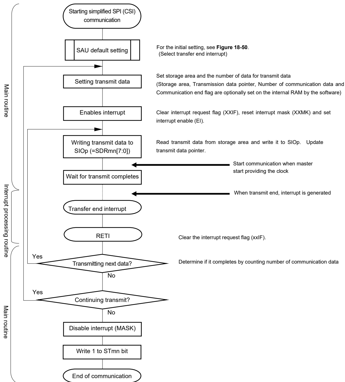
Figure 18-54. Flowchart of Slave Transmission (in Single-Transmission Mode)
