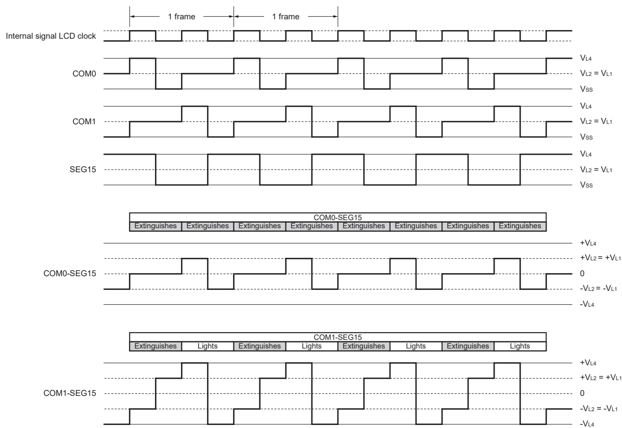
Figure 21-30. Two-Time-Slice LCD Drive Waveform Examples Between SEG15 and Each Common Signals (1/2 Bias Method)
