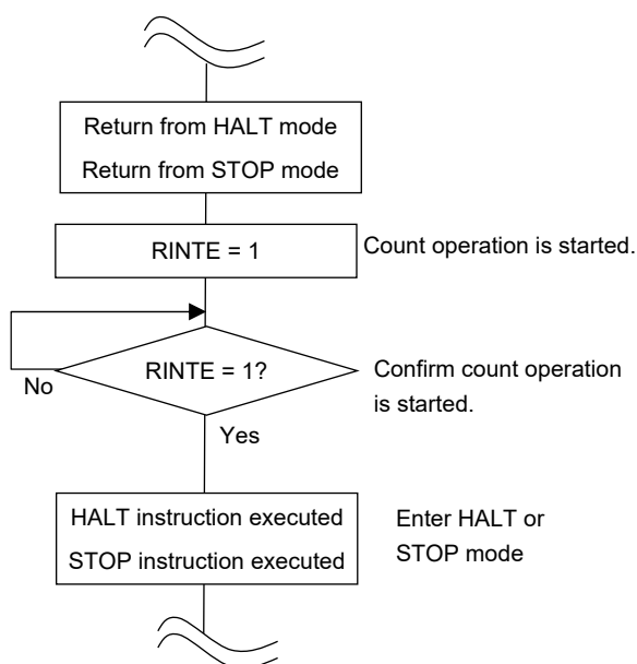
Figure 10-6. Procedure of Entering to HALT or STOP Mode After Setting RINTE to 1
