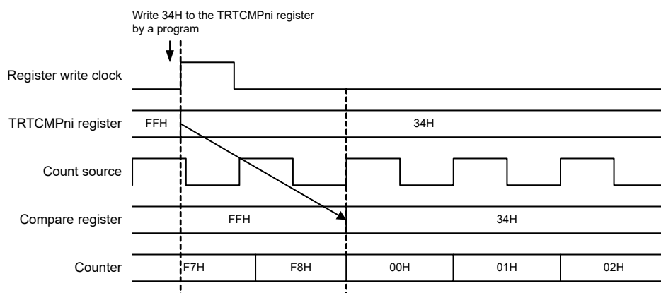
Figure 11-13. Timing of Rewriting the Compare Value
