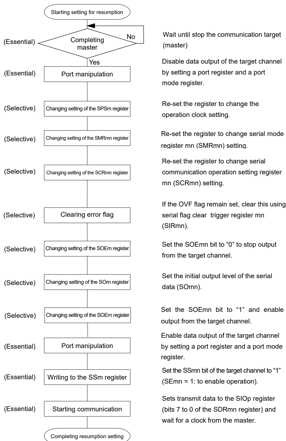
Figure 18-66. Procedure for Resuming Slave Transmission/Reception
