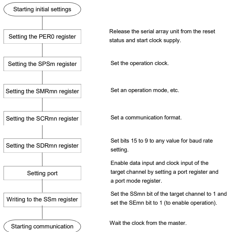
Figure 15-58. Initial Setting Procedure for Slave Reception
