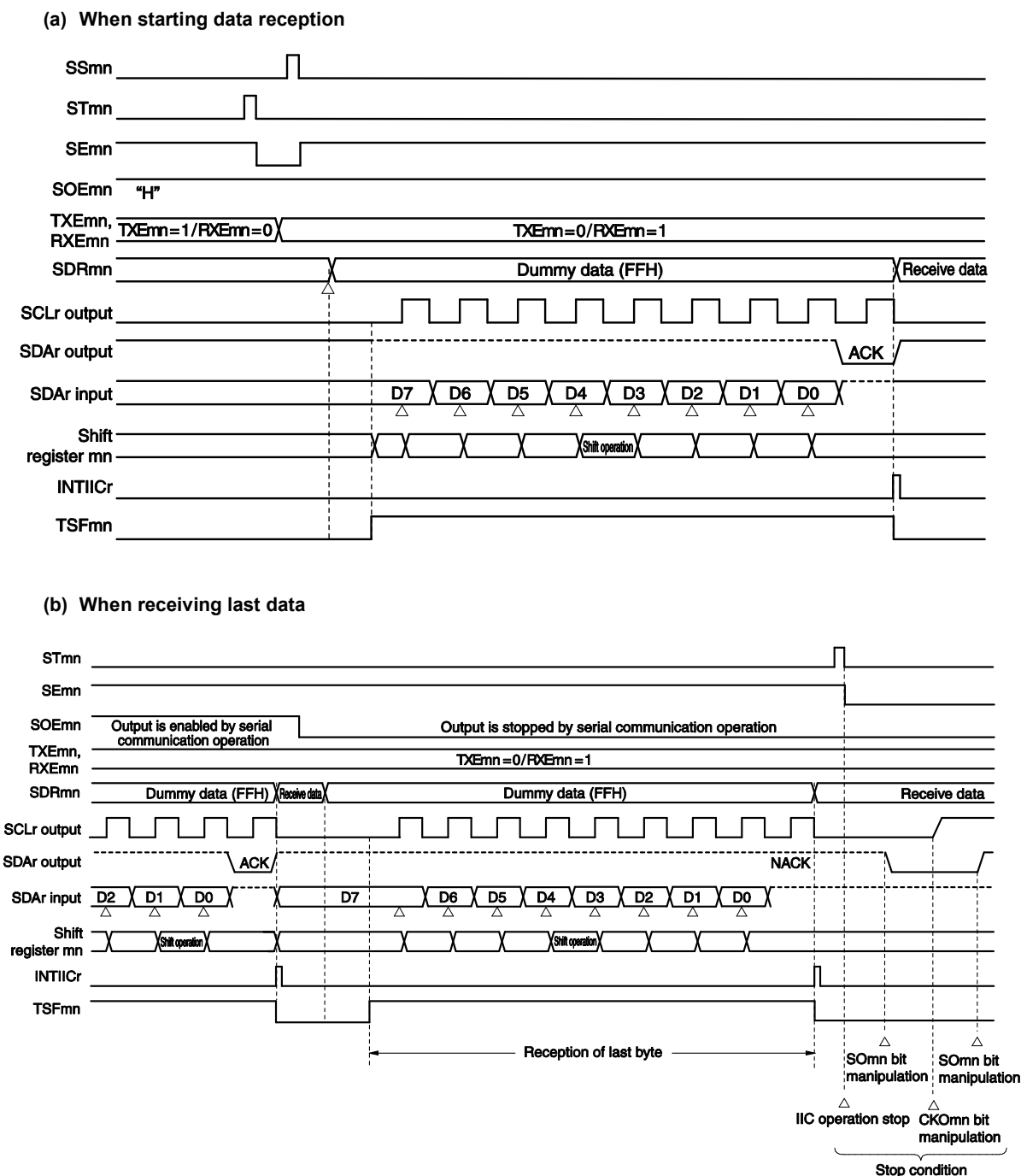
Figure 15-151. Timing Chart of Data Reception
