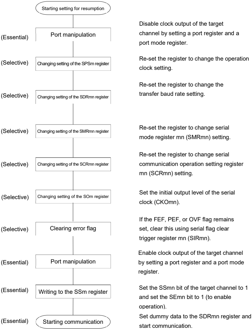
Figure 15-36. Procedure for Resuming Master Reception
