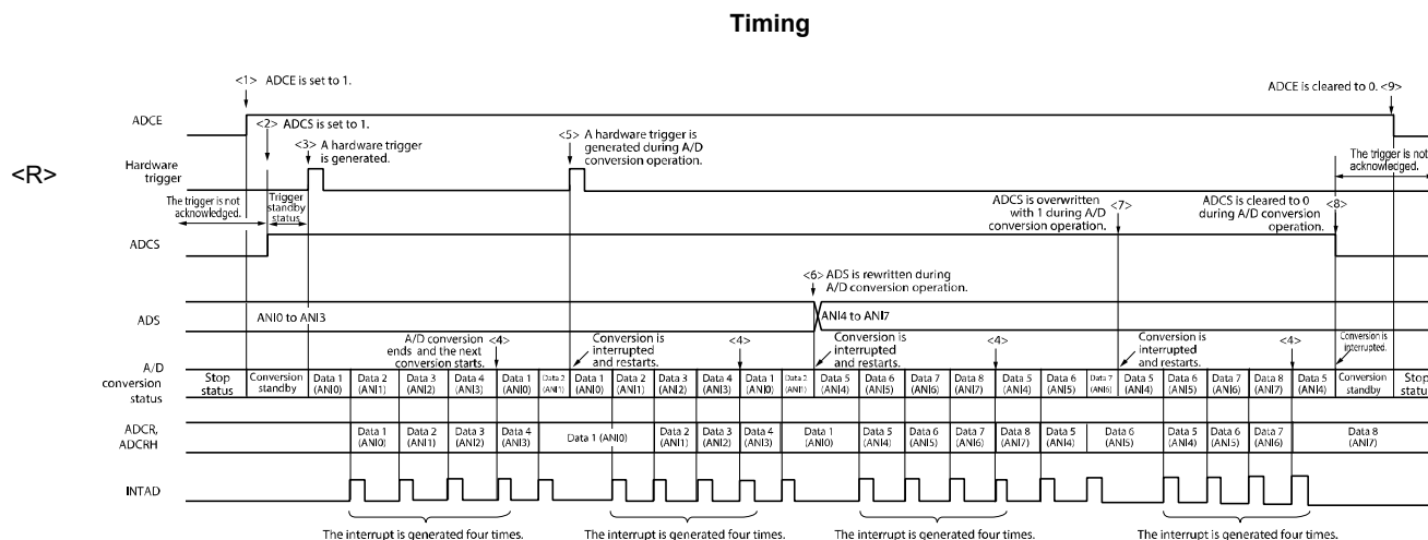
Figure 12-28. Example of Hardware Trigger No-Wait Mode (Scan Mode, Sequential Conversion Mode) Operation
