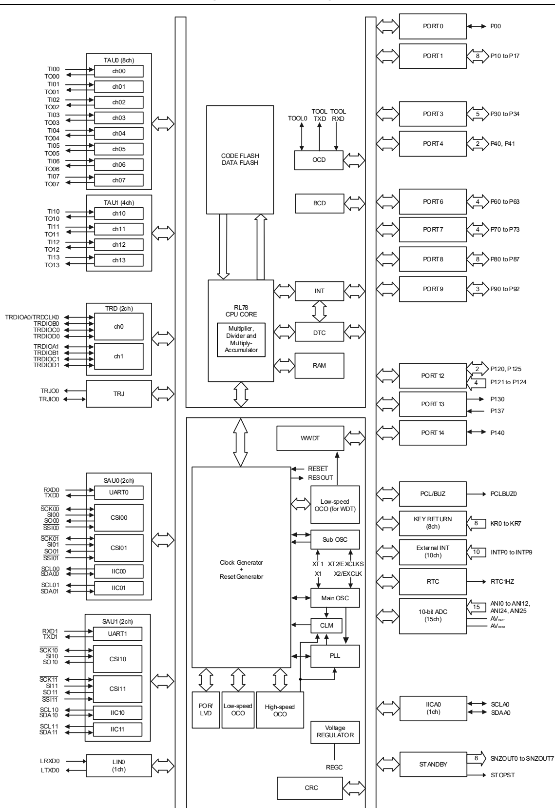
Figure 1-17. Block Diagram
