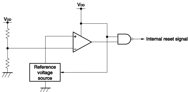
Figure 25-1. Block Diagram of Power-on-reset Circuit
