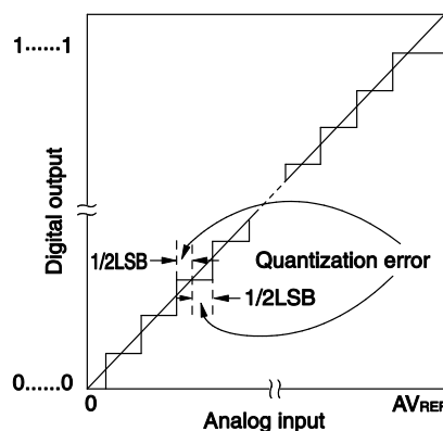
Figure 12-43. Quantization Error
