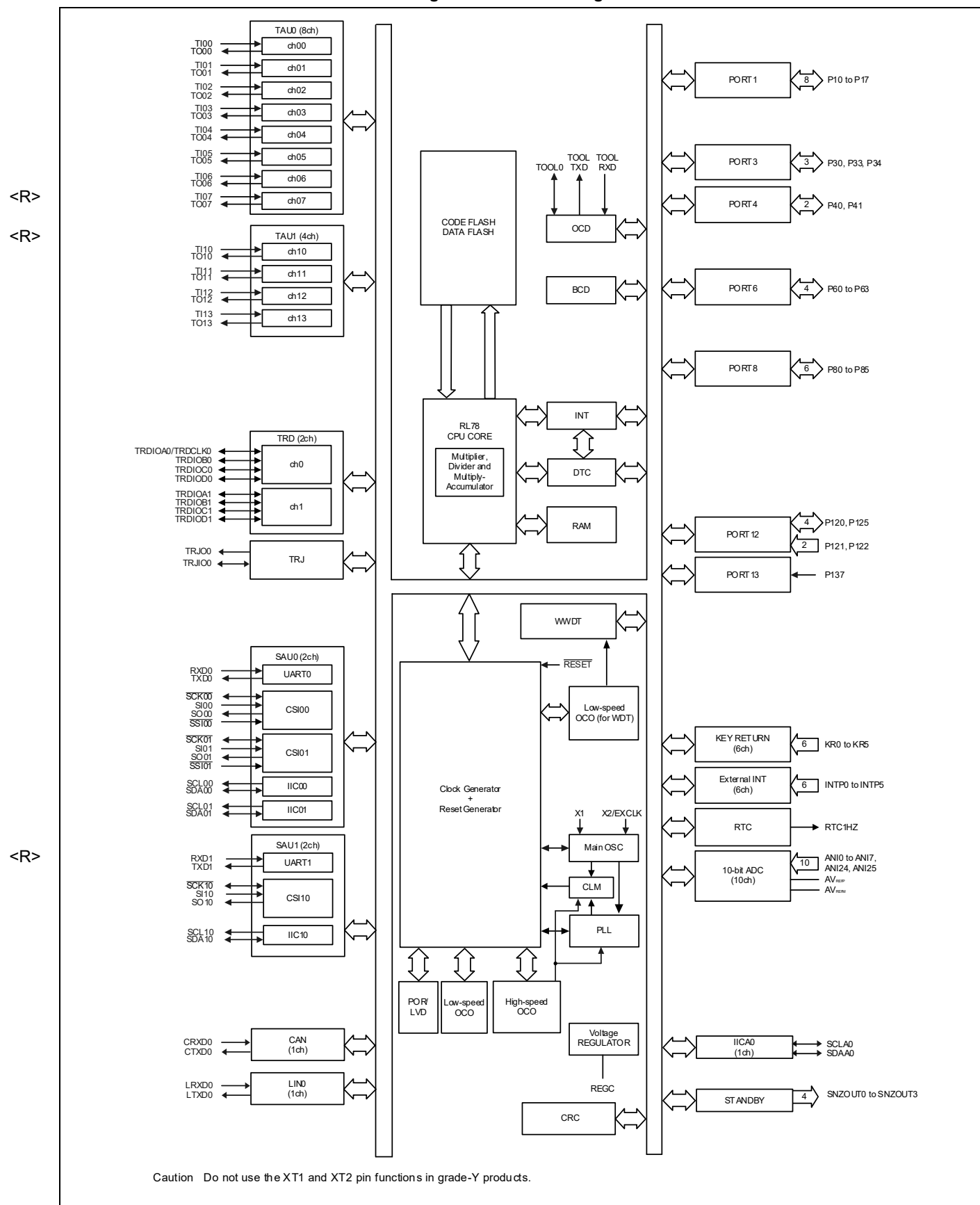
Figure 1-13. Block Diagram
