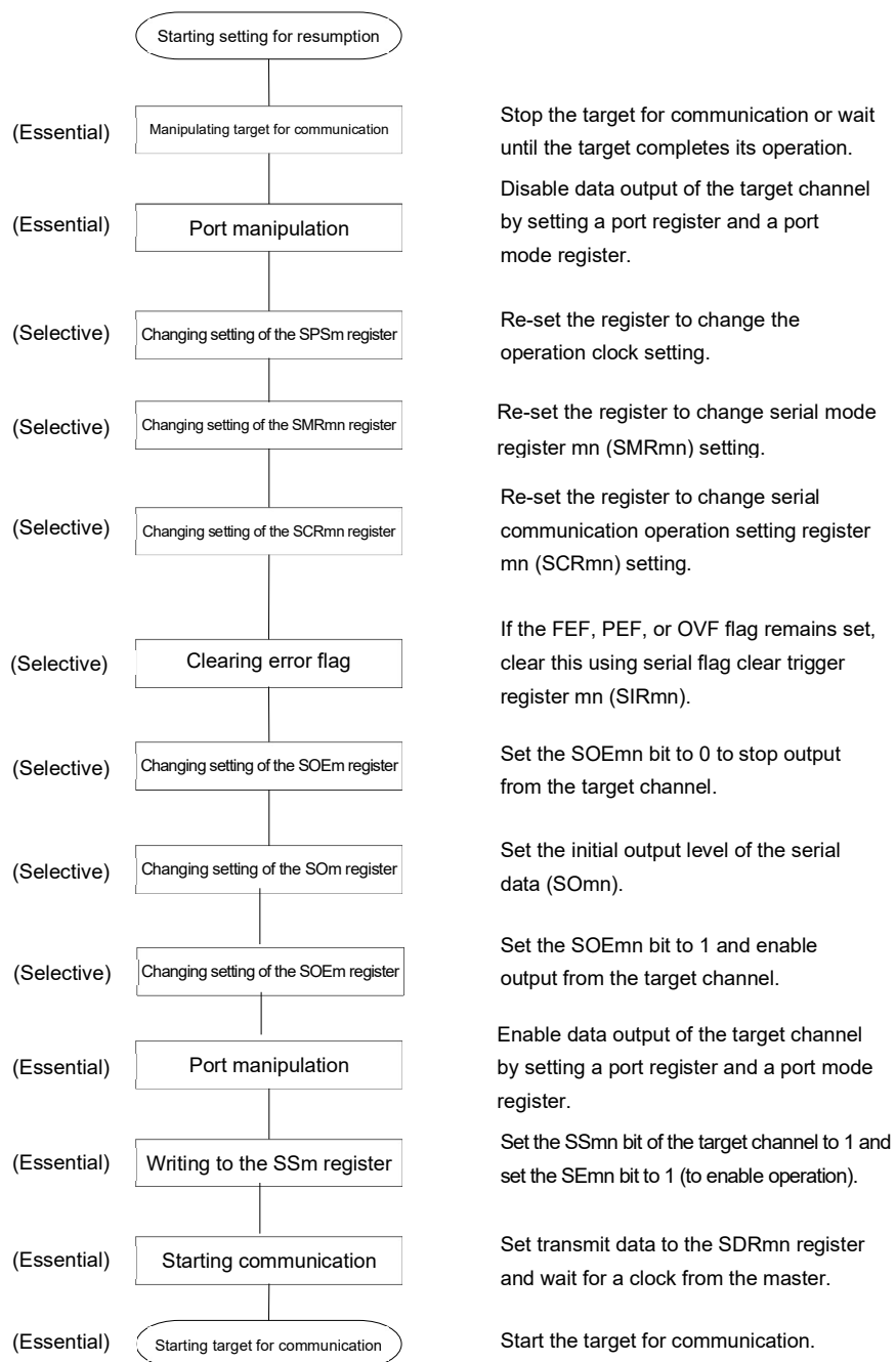
Figure 15-115. Procedure for Resuming Slave Transmission/Reception
