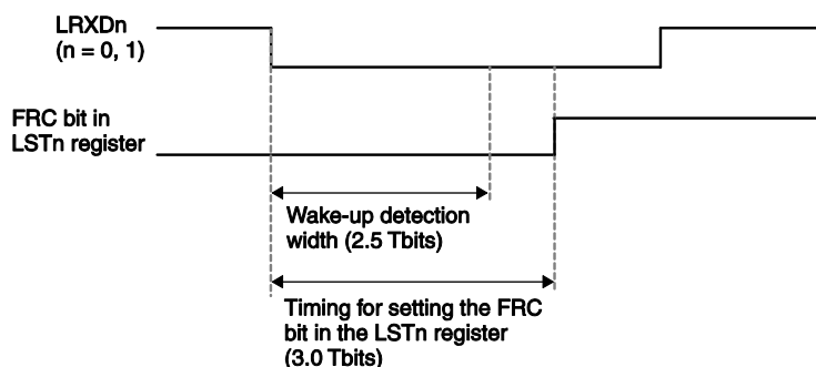
Figure 17-19. Input Signal Low Count Function
