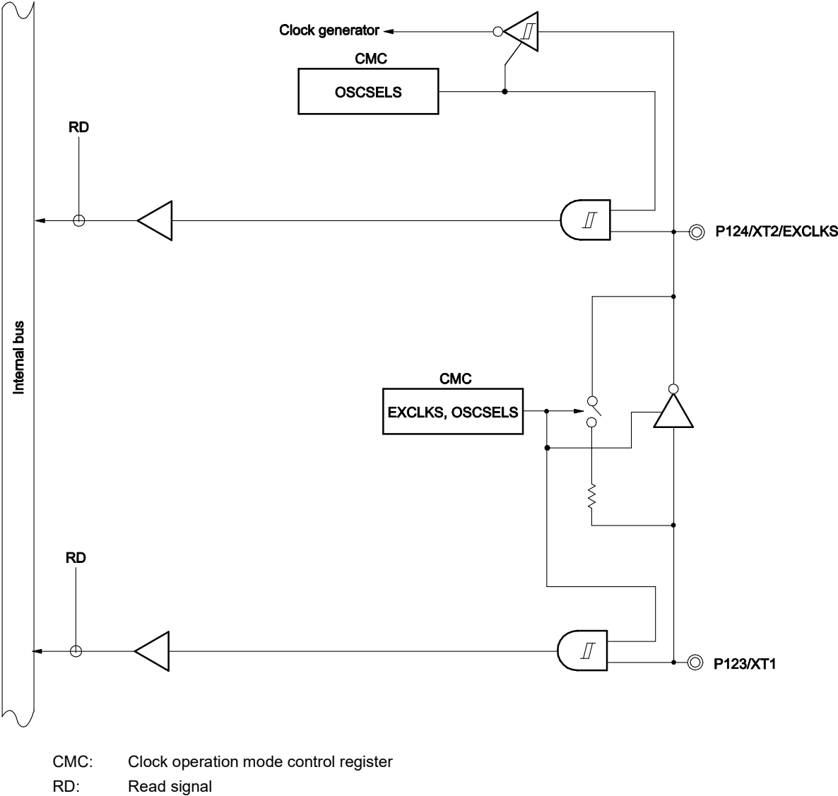
Figure 4-63. Block Diagram of P123 and P124
