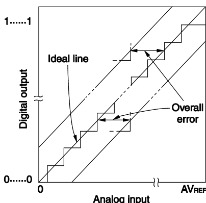
Figure 12-42. Overall Error
