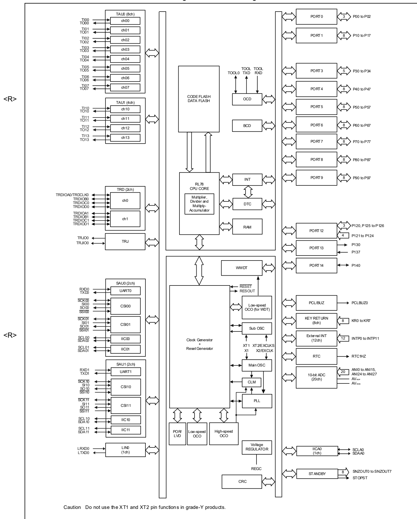
Figure 1-15. Block Diagram
