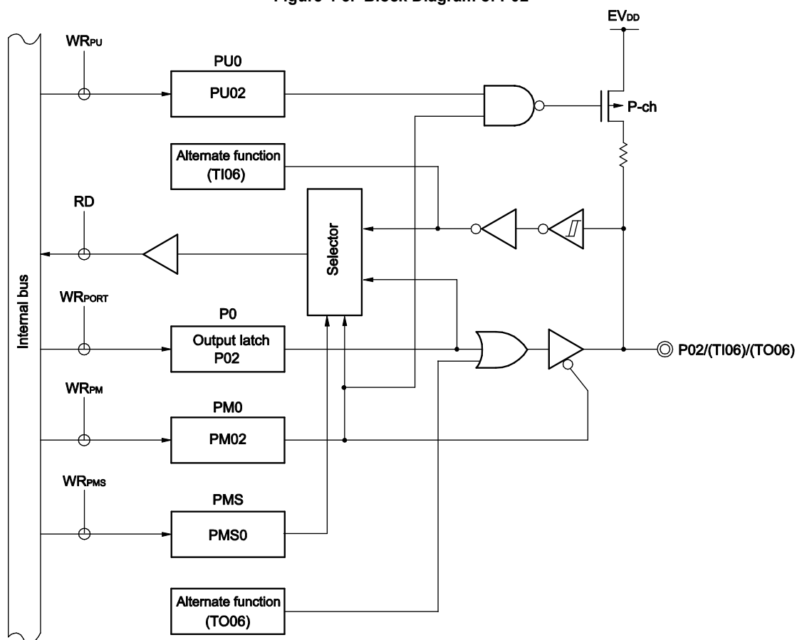
Figure 4-3. Block Diagram of P02
