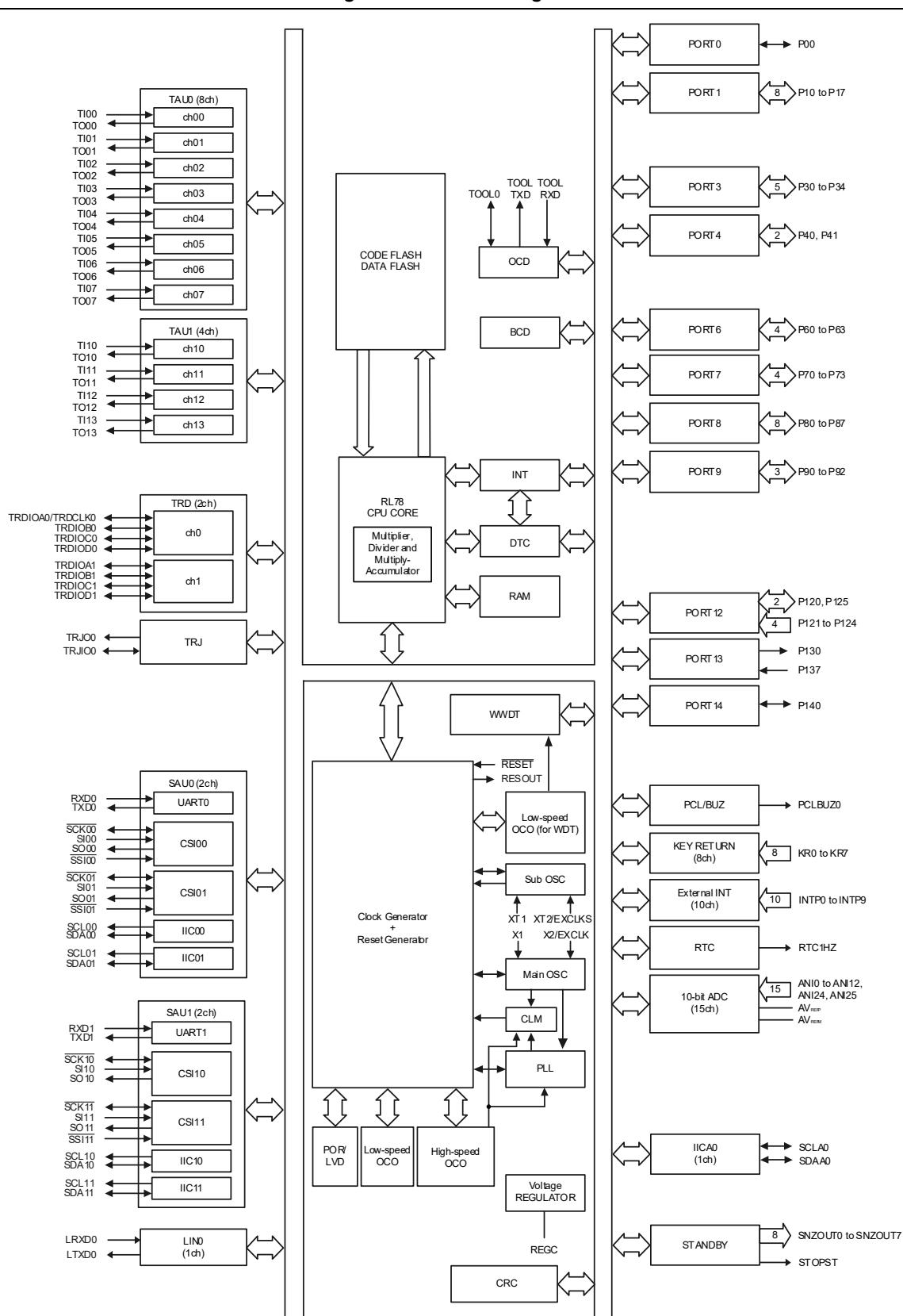
Figure 1-17. Block Diagram
