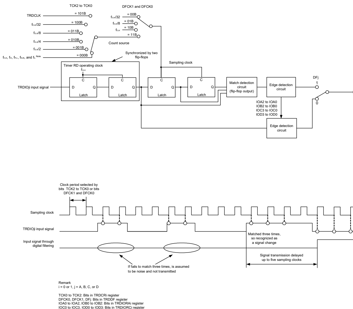
Figure 8-47. Block Diagram of Digital Filter
