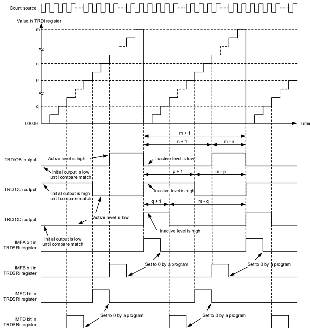
Figure 8-53. Operation Example in PWM Function
