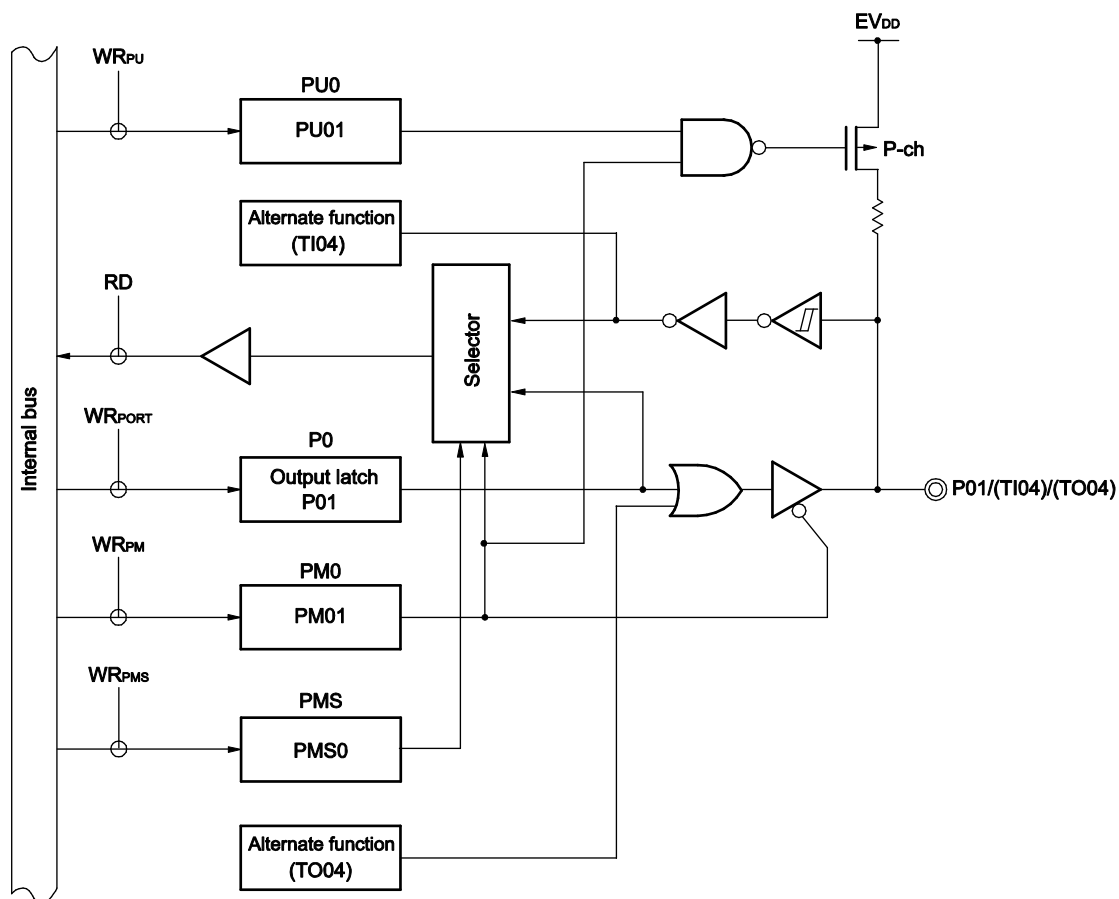
Figure 4-2. Block Diagram of P01
