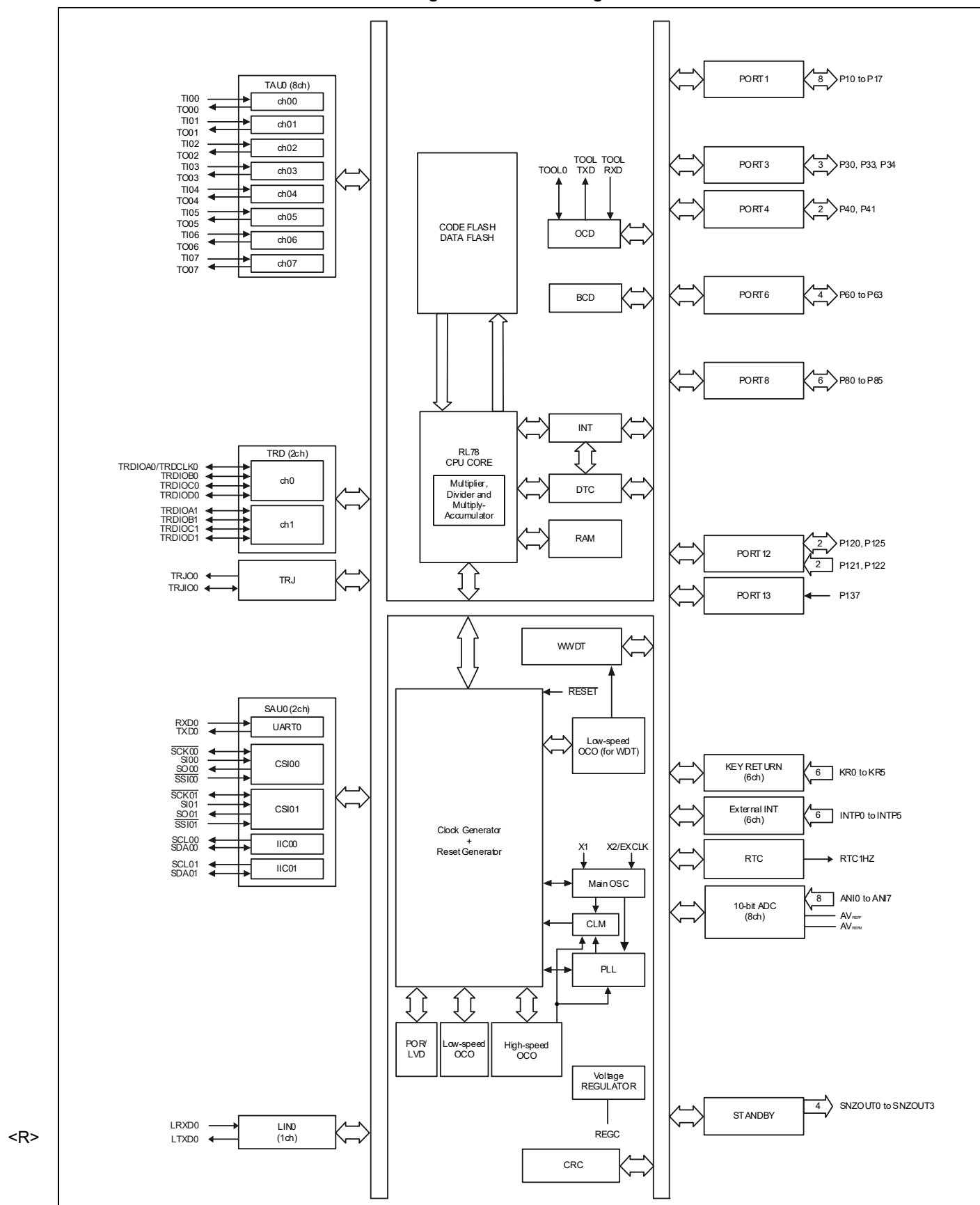
Figure 1-20. Block Diagram
