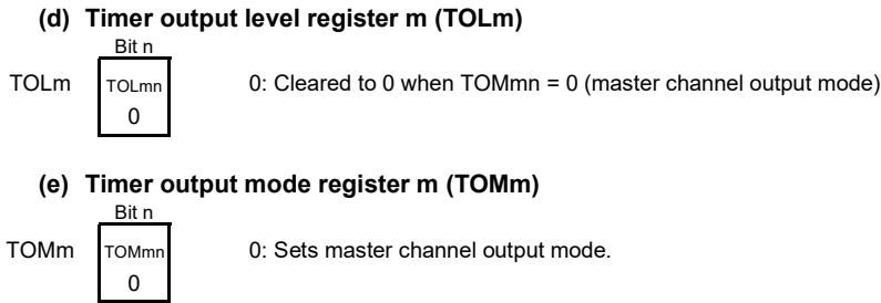
Figure 6-45. Example of Set Contents of Registers During Operation as Interval Timer/Square Wave Output (2/2)
