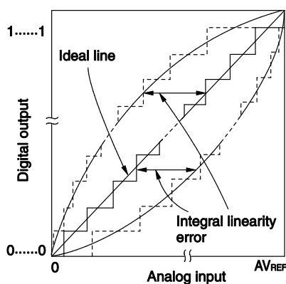
Figure 12-46. Integral Linearity Error
