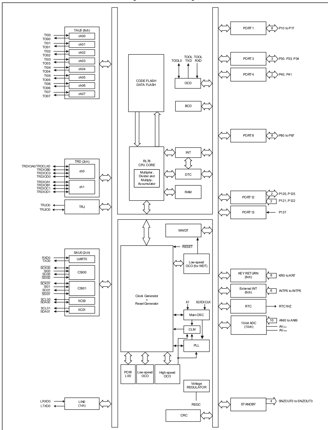
Figure 1-21. Block Diagram
