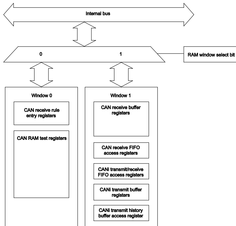
Figure 18-15. RAM Window
