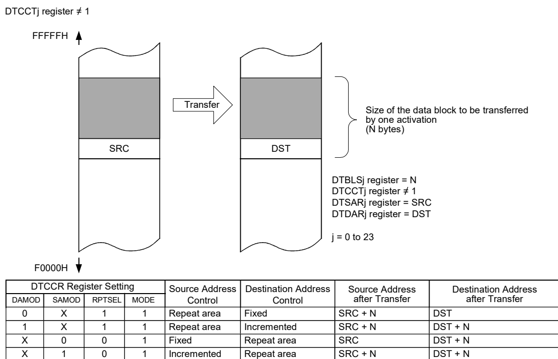
Figure 19-23. Data Transfers in Repeat Mode
