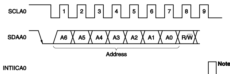
Figure 16-17. Address
