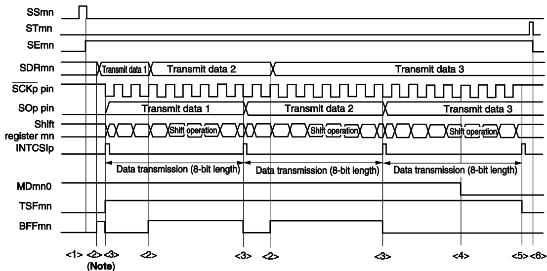
Figure 15-80. Timing Chart of Master Transmission (in Continuous Transmission Mode)
