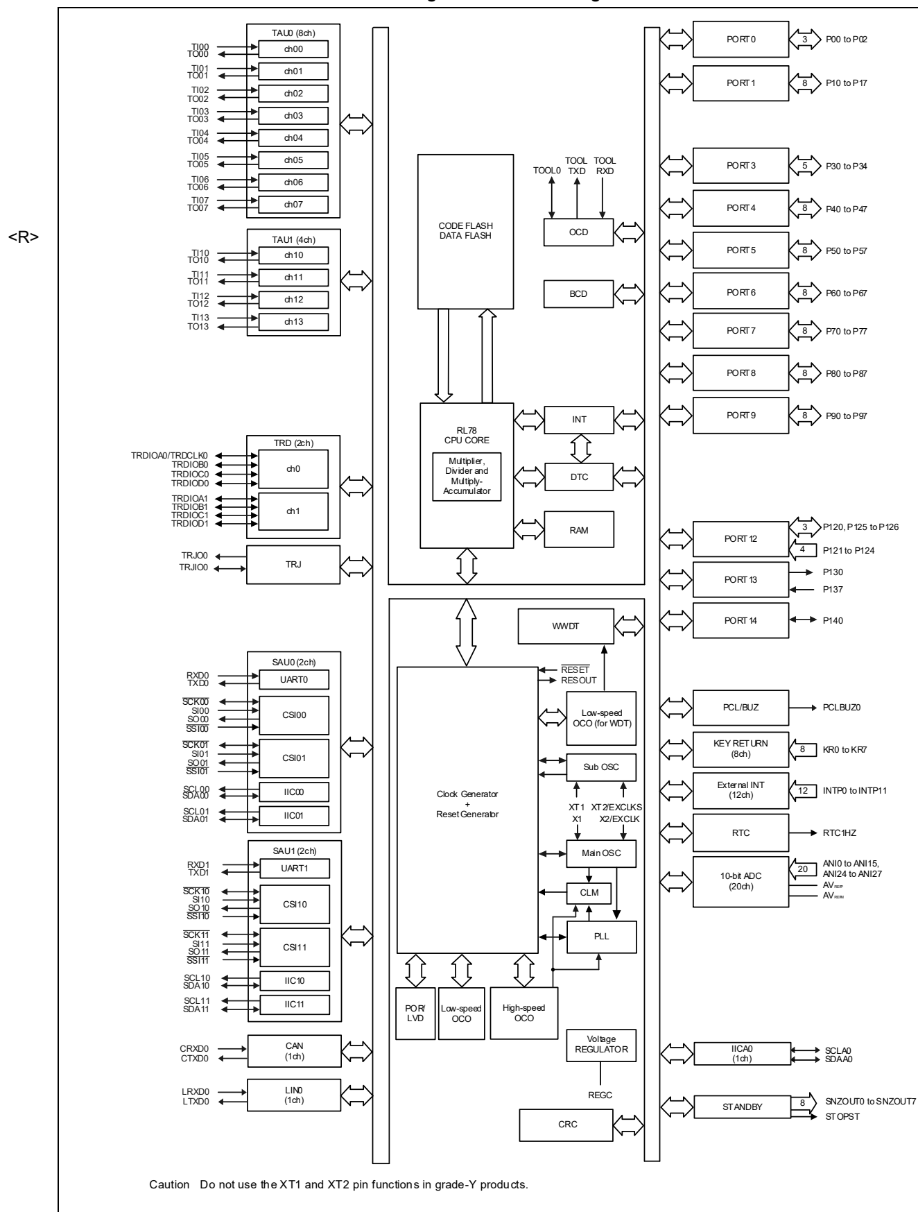
Figure 1-10. Block Diagram
