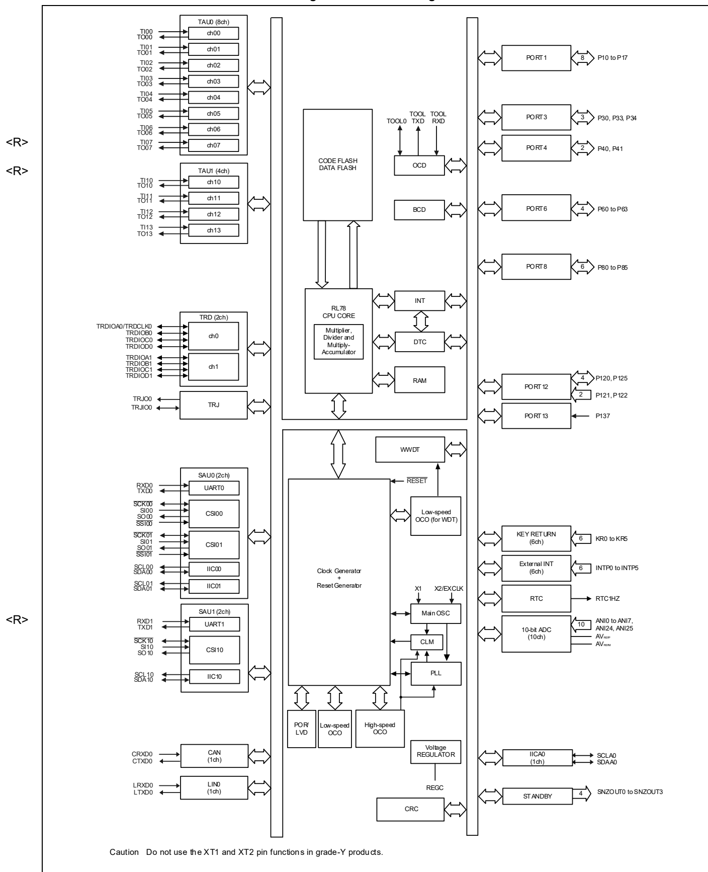
Figure 1-13. Block Diagram
