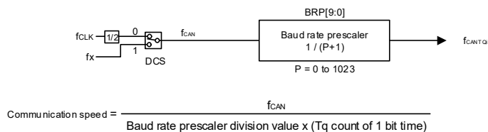
Figure 18-18. CAN Clock Control Block Diagram
