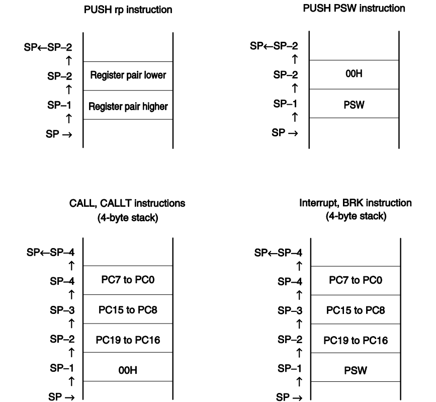
Figure 3-39. Data to Be Saved to Stack Memory
