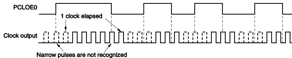
Figure 10-5. Remote Control Output Application Example
