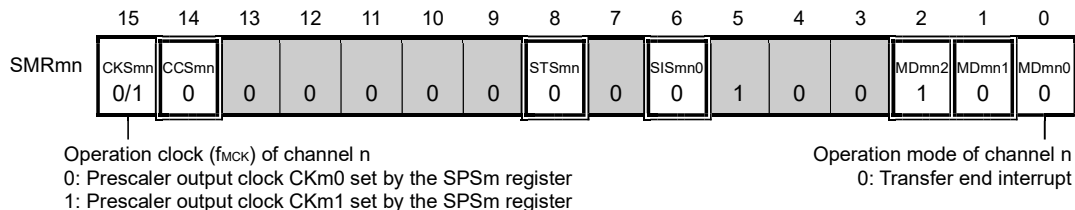
Figure 15-143. Example of Contents of Registers for Address Field Transmission of Simplified I 2 C (IIC00, IIC01, IIC10, IIC11) (1/2)
