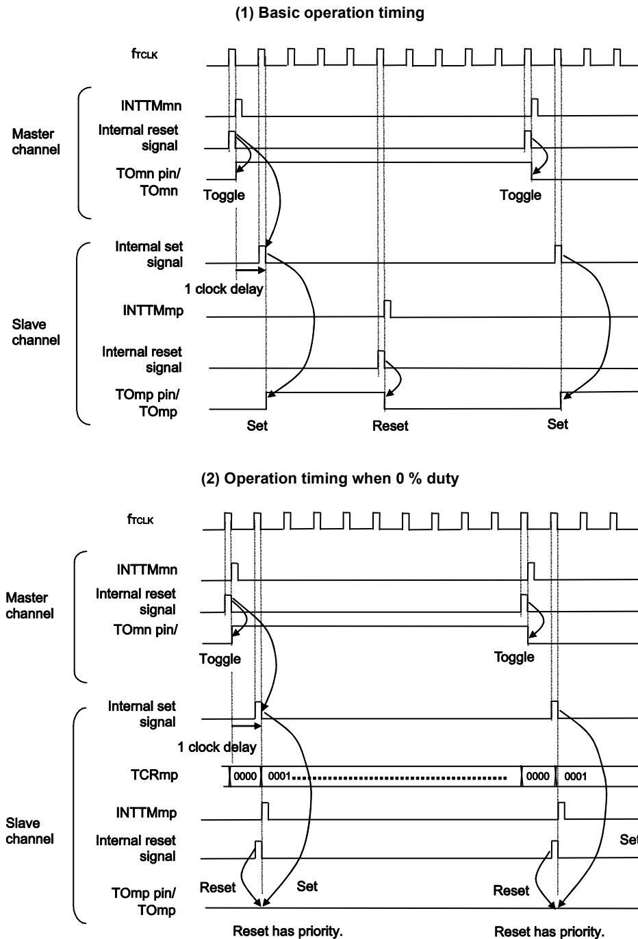
Figure 6-39. Set/Reset Timing Operating Statuses
