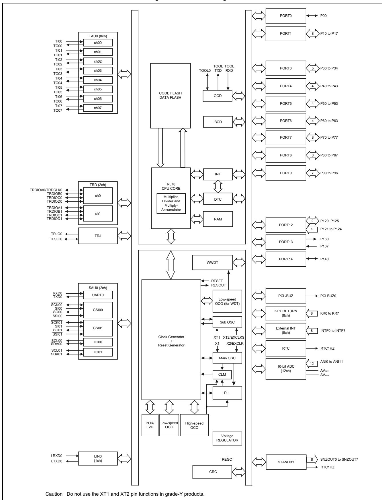
Figure 1-18. Block Diagram
