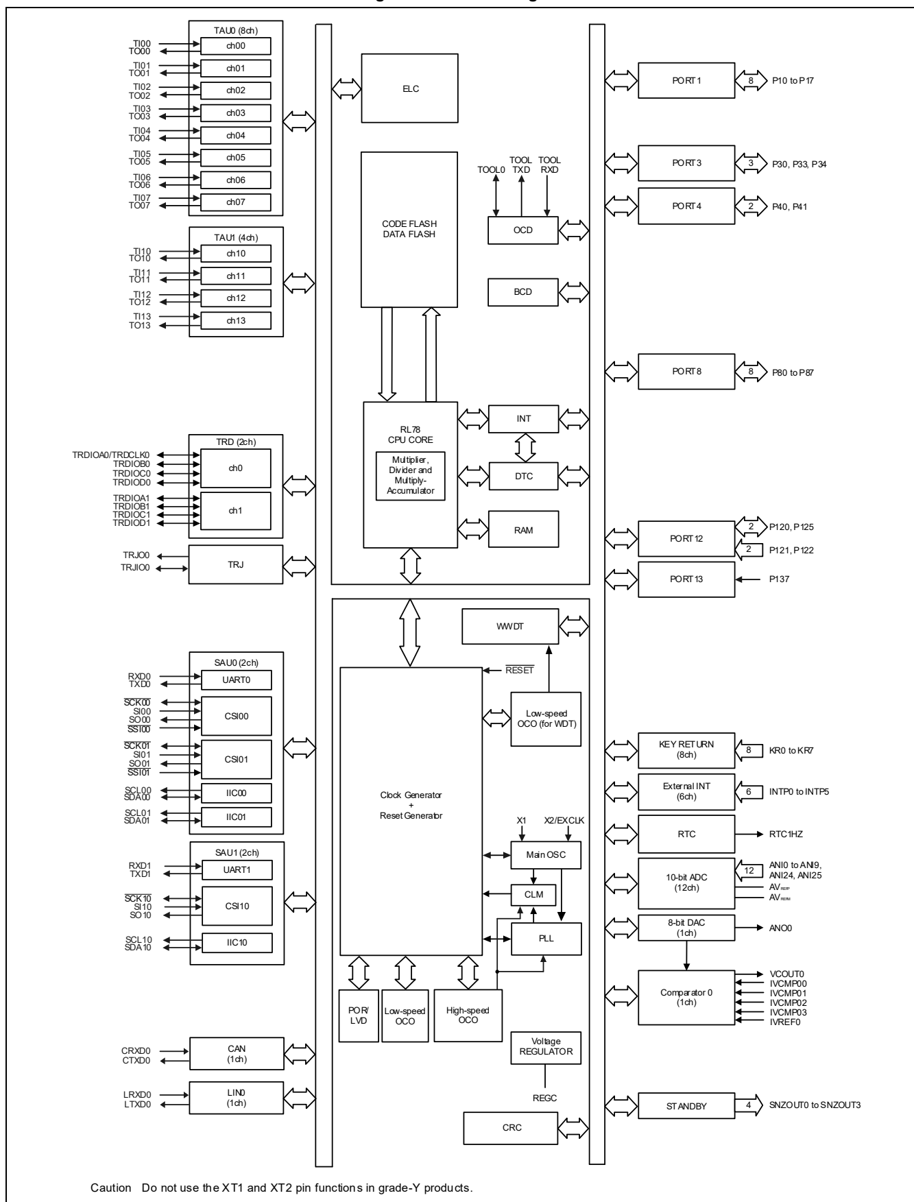
Figure 1-9. Block Diagram
