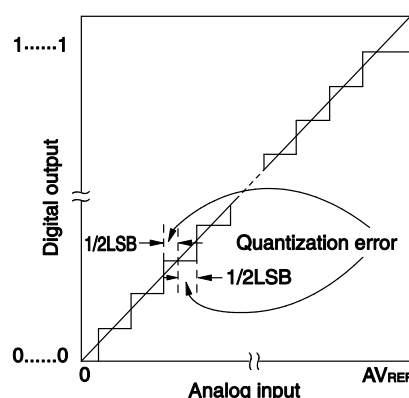
Figure 12-43. Quantization Error
