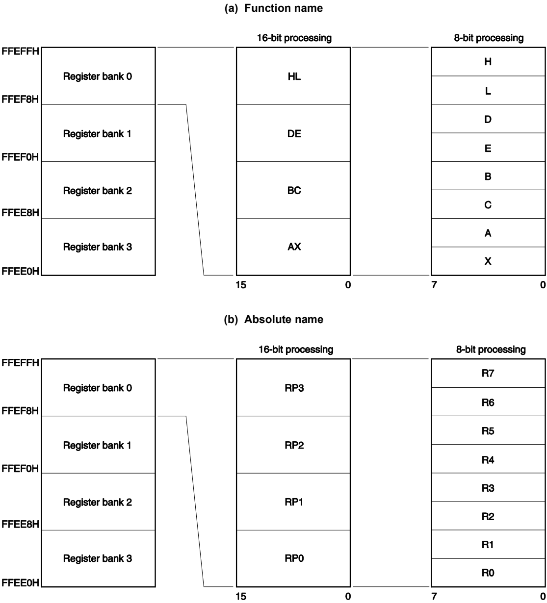
Figure 3-40. Configuration of General-Purpose Registers
