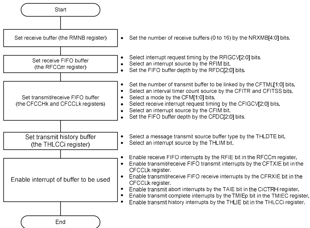
Figure 18-21. Buffer Setting Procedure
