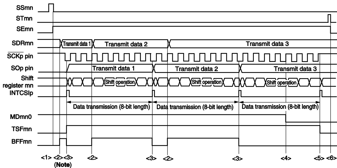
Figure 15-104. Timing Chart of Slave Transmission (in Continuous Transmission Mode)
