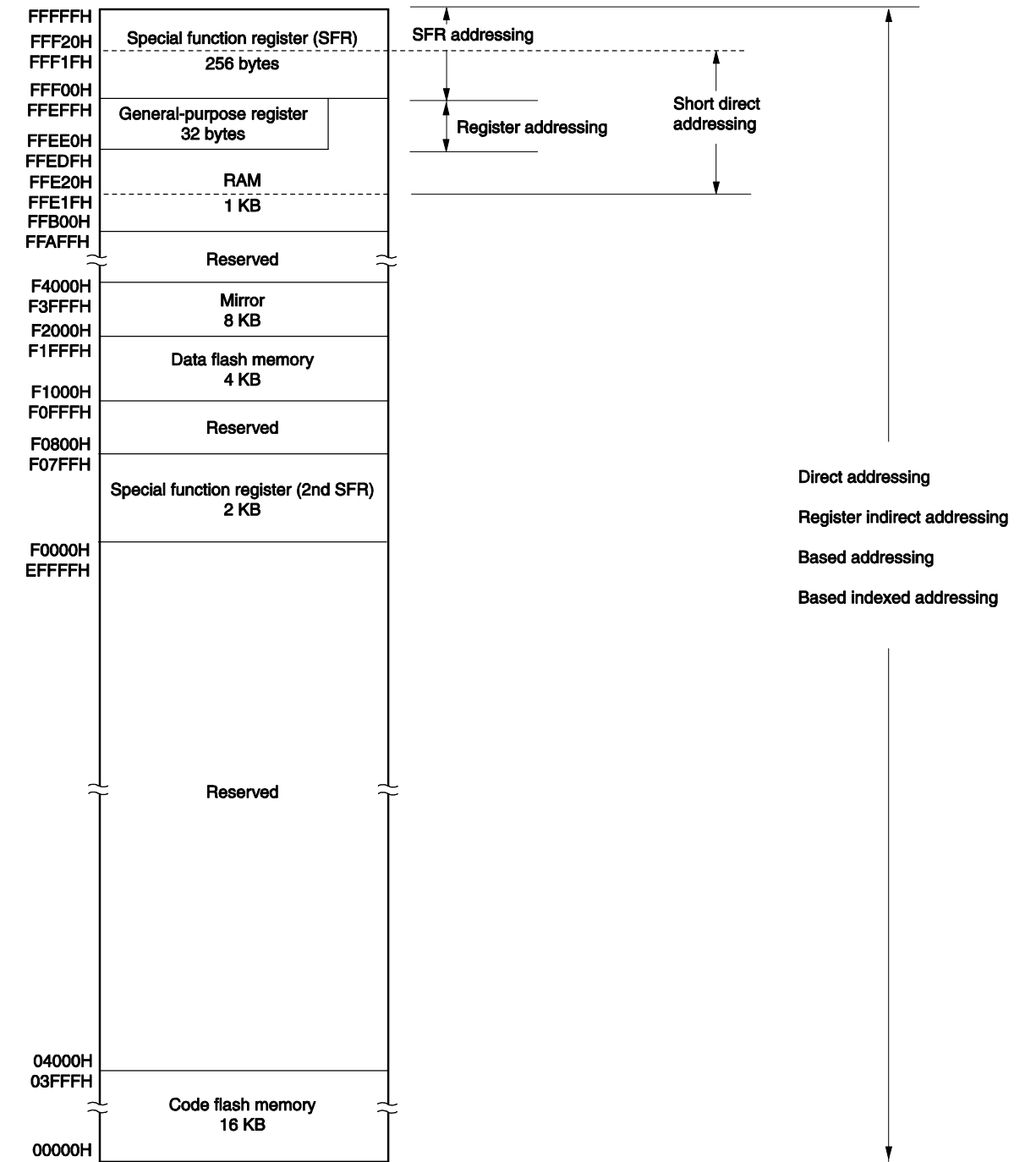
Figure 3-19. Correspondence between Data Memory and Addressing (R5F10AmA (m = 6, A, B, G))
