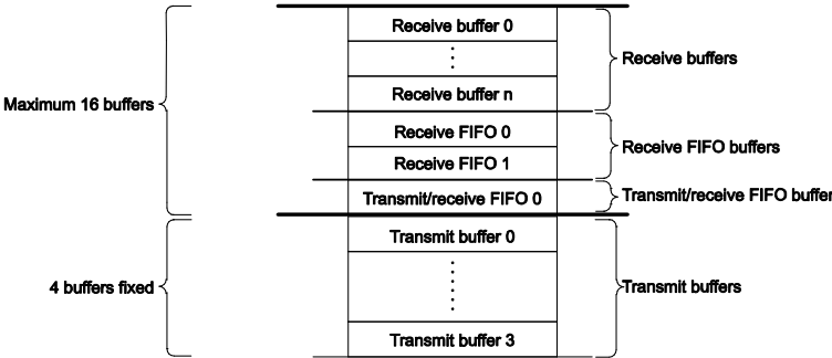
Figure 18-20. Buffer Configuration
