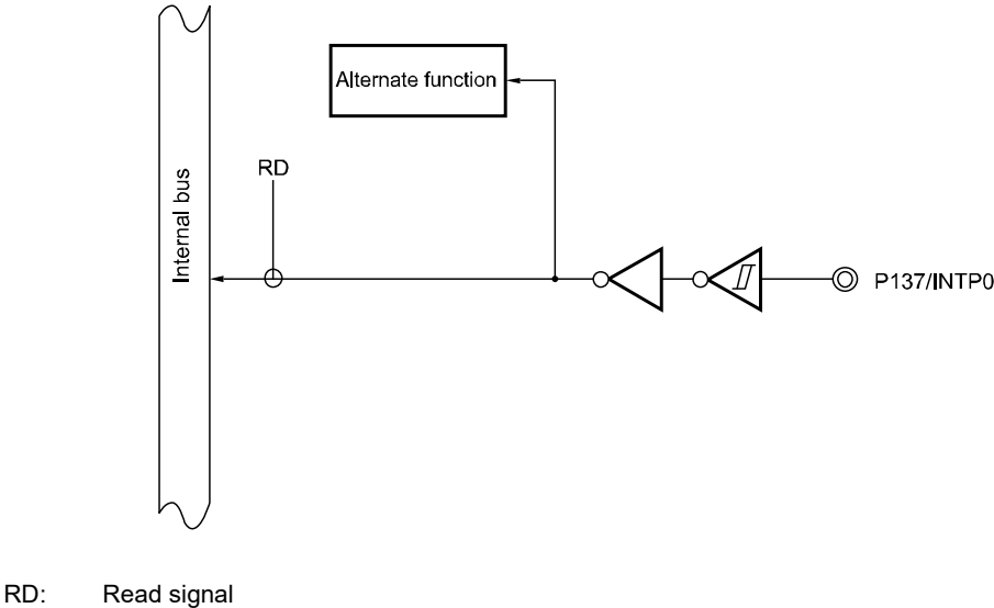
Figure 4-67. Block Diagram of P137
