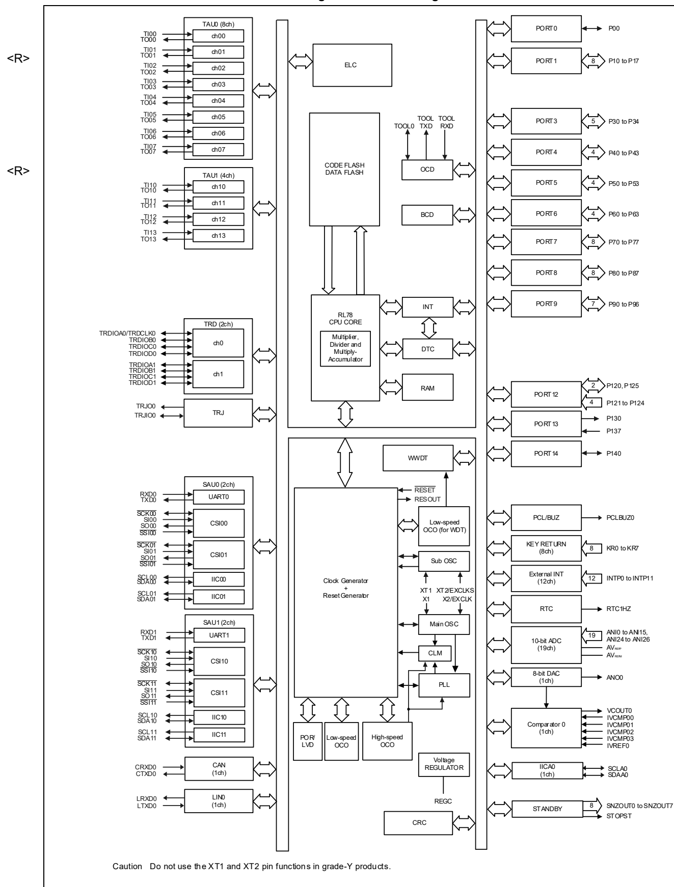
Figure 1-6. Block Diagram
