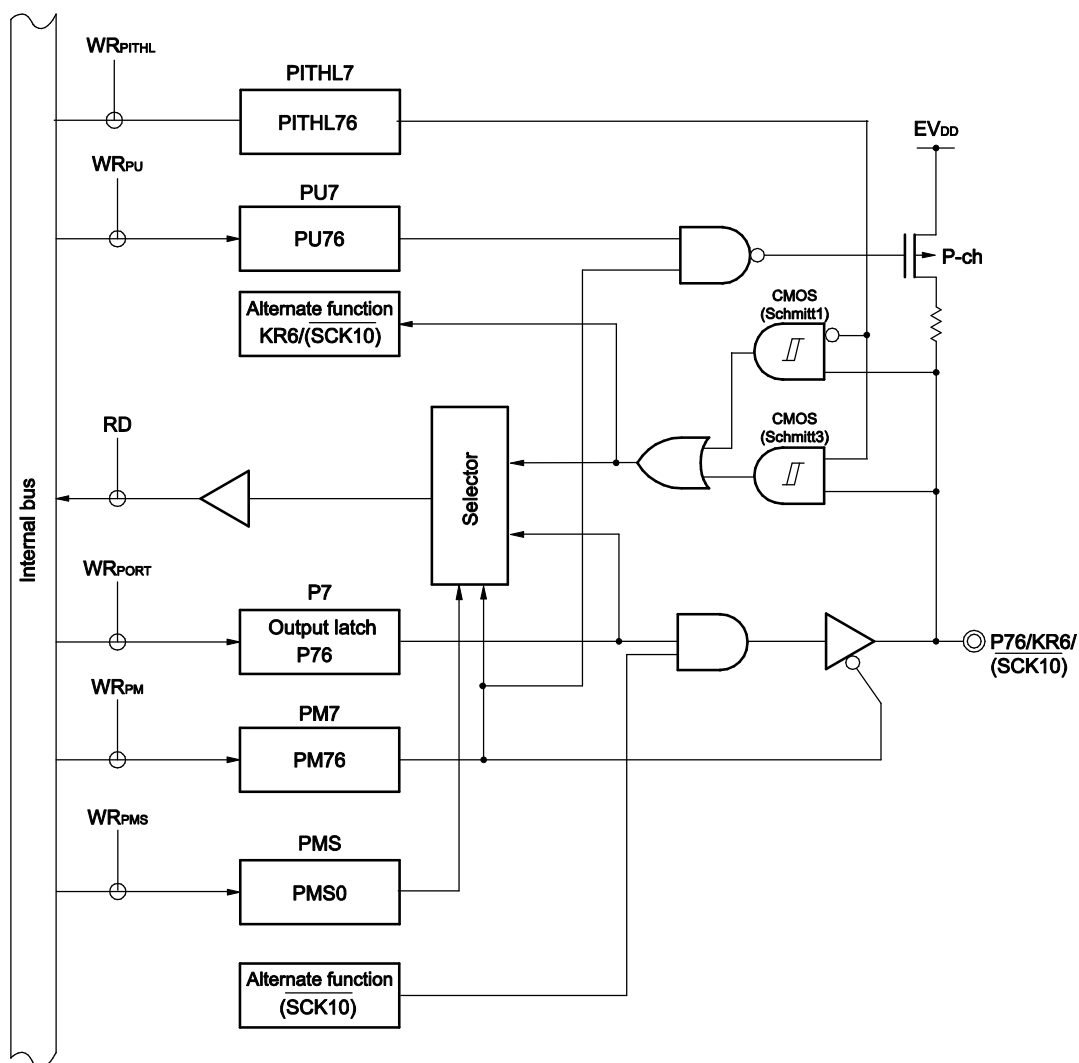
Figure 4-47. Block Diagram of P76
