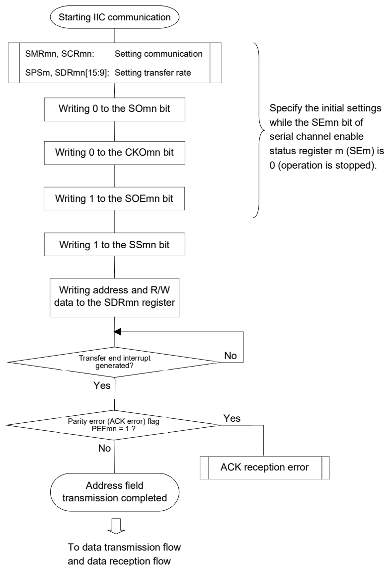
Figure 15-146. Flowchart of Address Field Transmission
