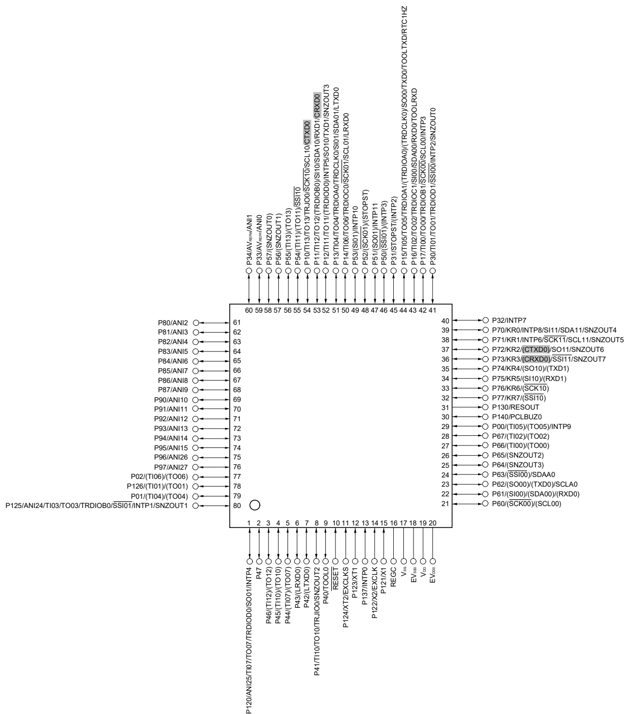
Figure 1-25. RL78/F13 Pin Configuration for 80-pin Products
