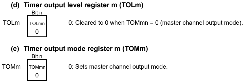
Figure 6-49. Example of Set Contents of Registers in External Event Counter Mode (2/2)
