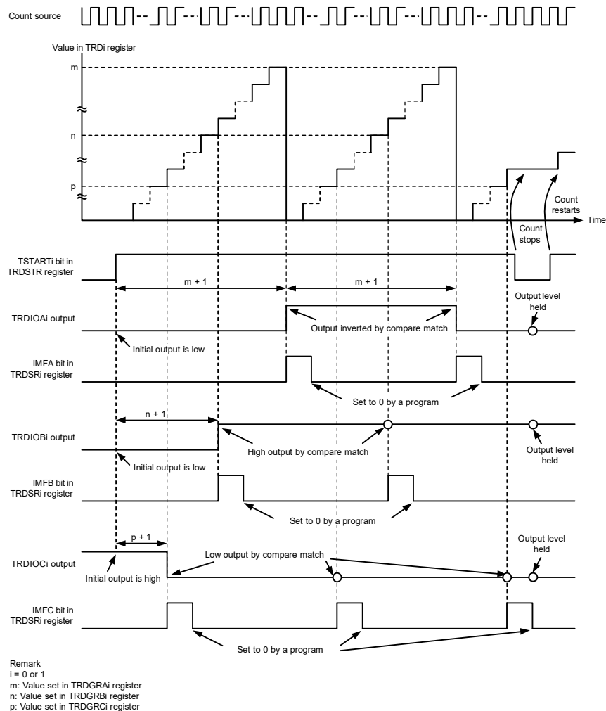
Figure 8-49. Operation Example of Output Compare Function
