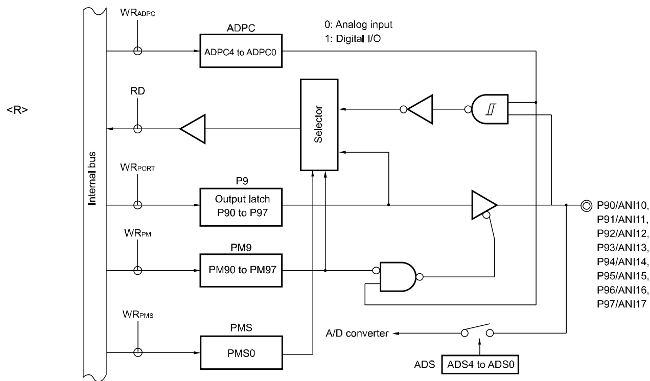
Figure 4-57. Block Diagram of P90 to P97
