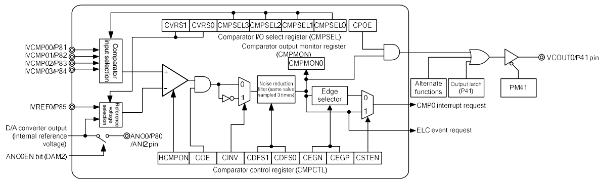
Figure 14-1. Comparator Block Diagram
