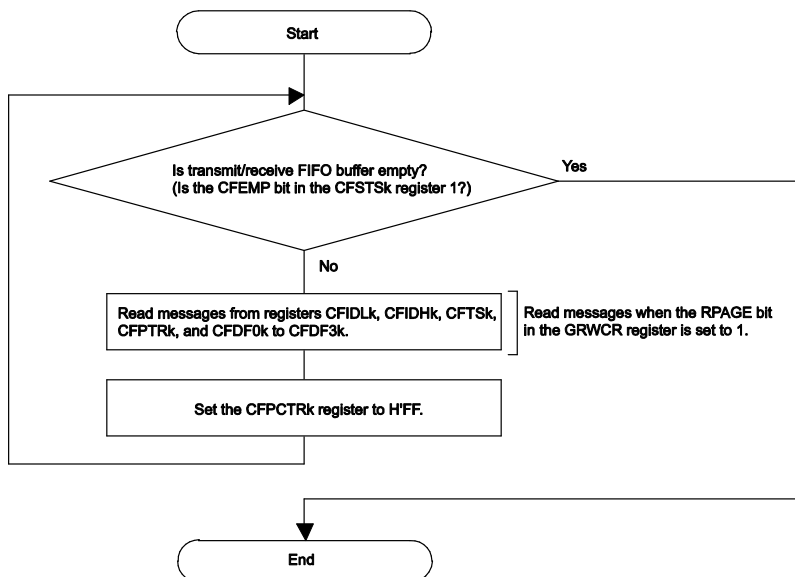
Figure 18-24. Transmit/Receive FIFO Buffer Reading Procedure
