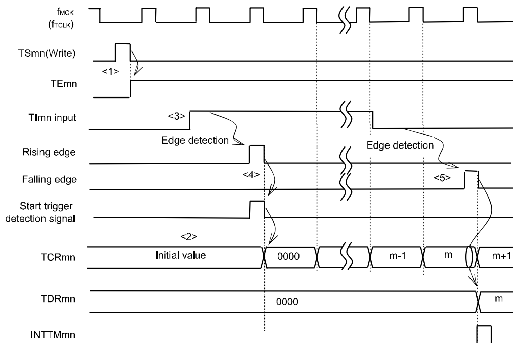
<R> Figure 6-33. Operation Timing (In Capture & One-count Mode: High-level Width Measurement)
