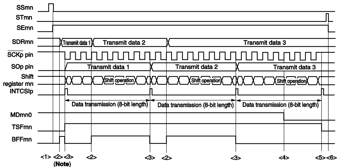
Figure 15-31. Timing Chart of Master Transmission (in Continuous Transmission Mode)
