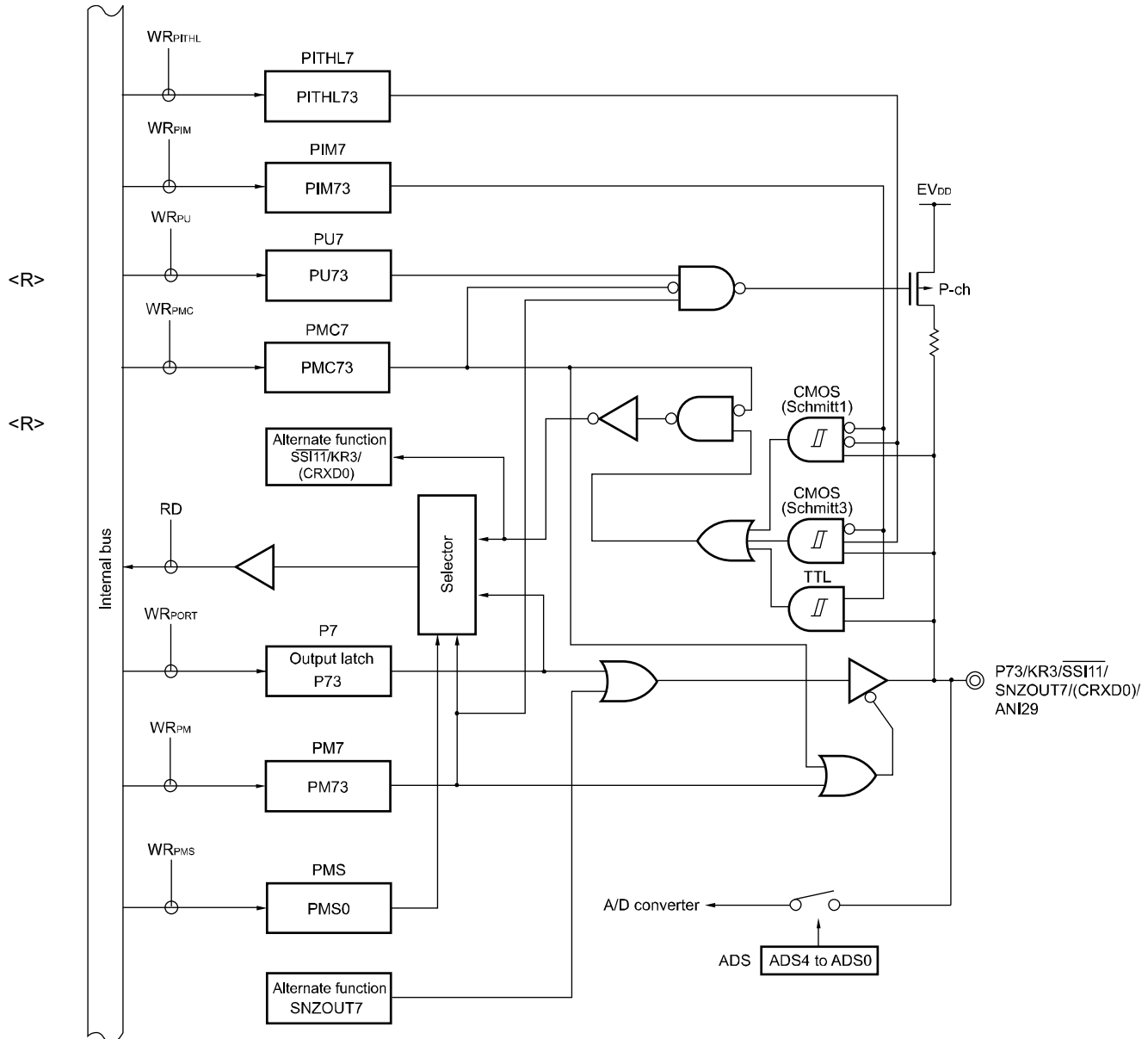
Figure 4-44. Block Diagram of P73
