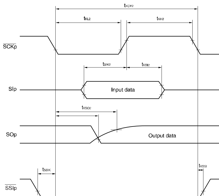
CSI mode serial transfer timing (during communication at same potential)
