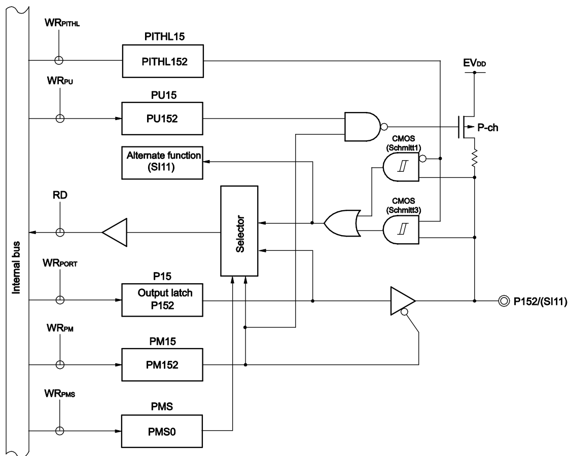
Figure 4-71. Block Diagram of P152
