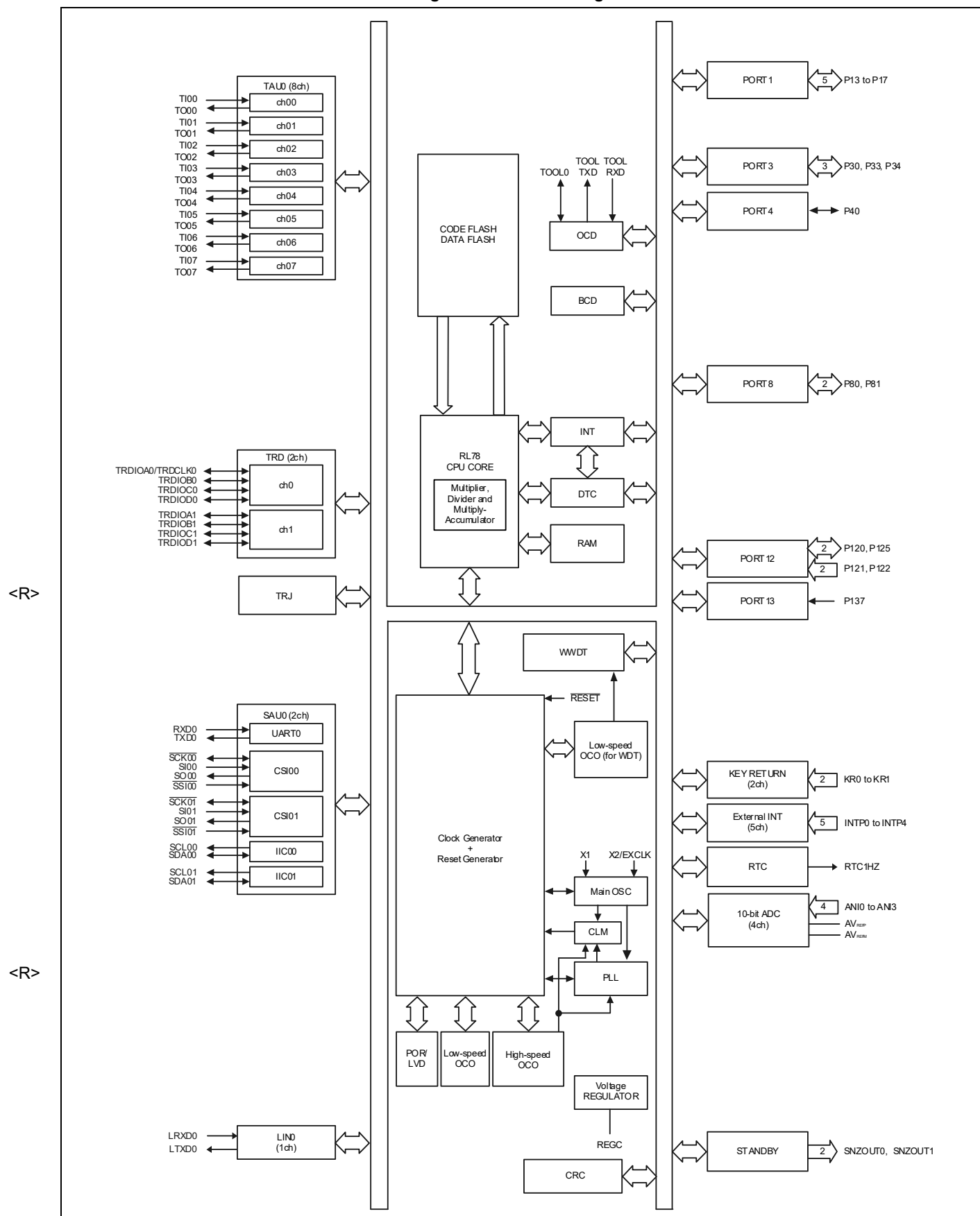
Figure 1-22. Block Diagram
