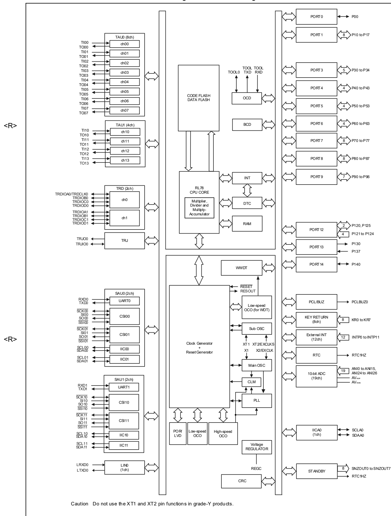
Figure 1-16. Block Diagram
