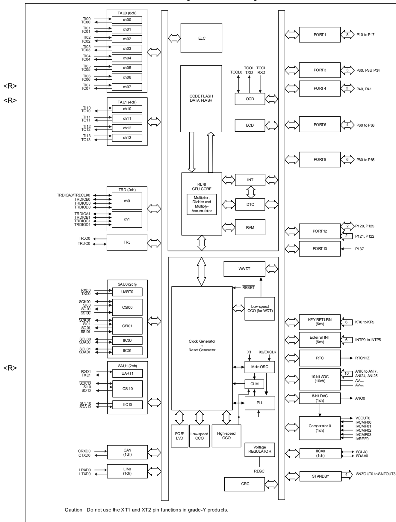
Figure 1-8. Block Diagram
