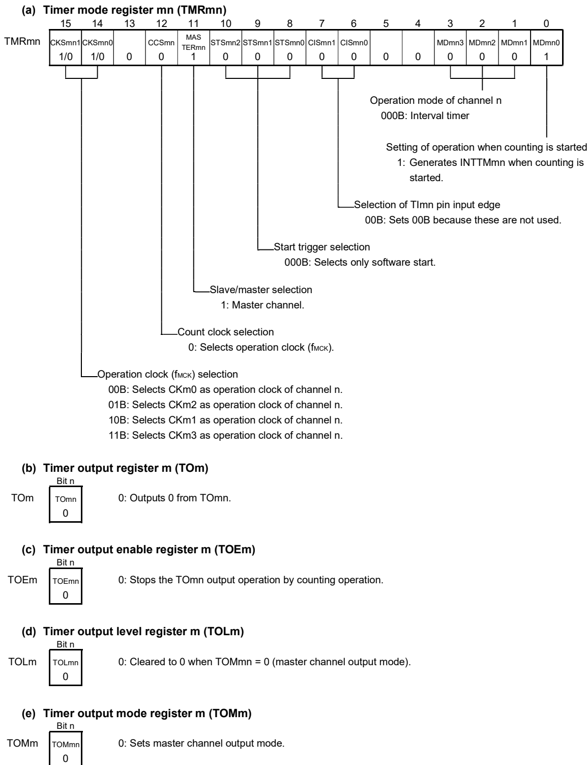
Figure 6-79. Example of Set Contents of Registers When Multiple PWM Output Function (Master Channel) Is Used
