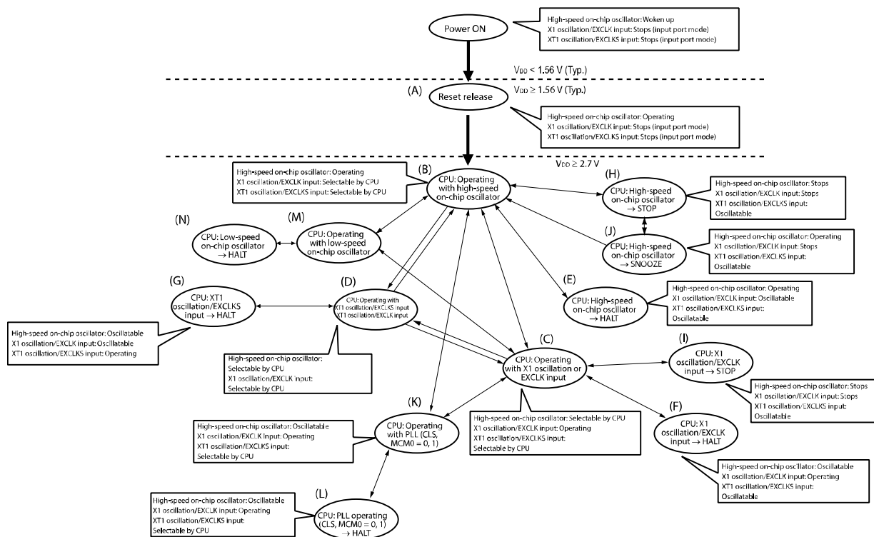
Figure 5-27. CPU Clock Status Transition Diagram
