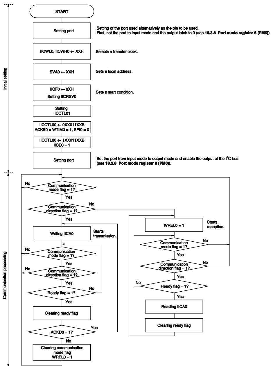
Figure 16-31. Slave Operation Flowchart (1)
