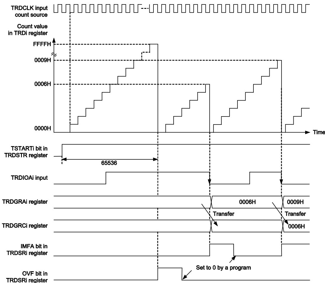
Figure 8-46. Operation Example of Input Capture Function
