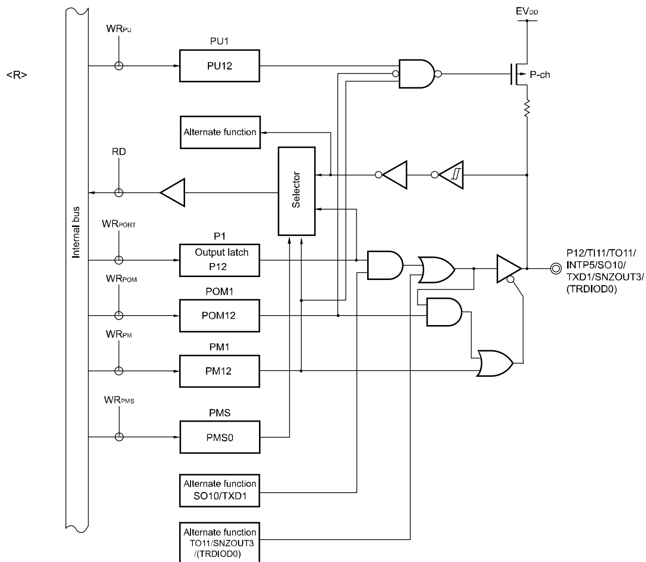
Figure 4-7. Block Diagram of P12
