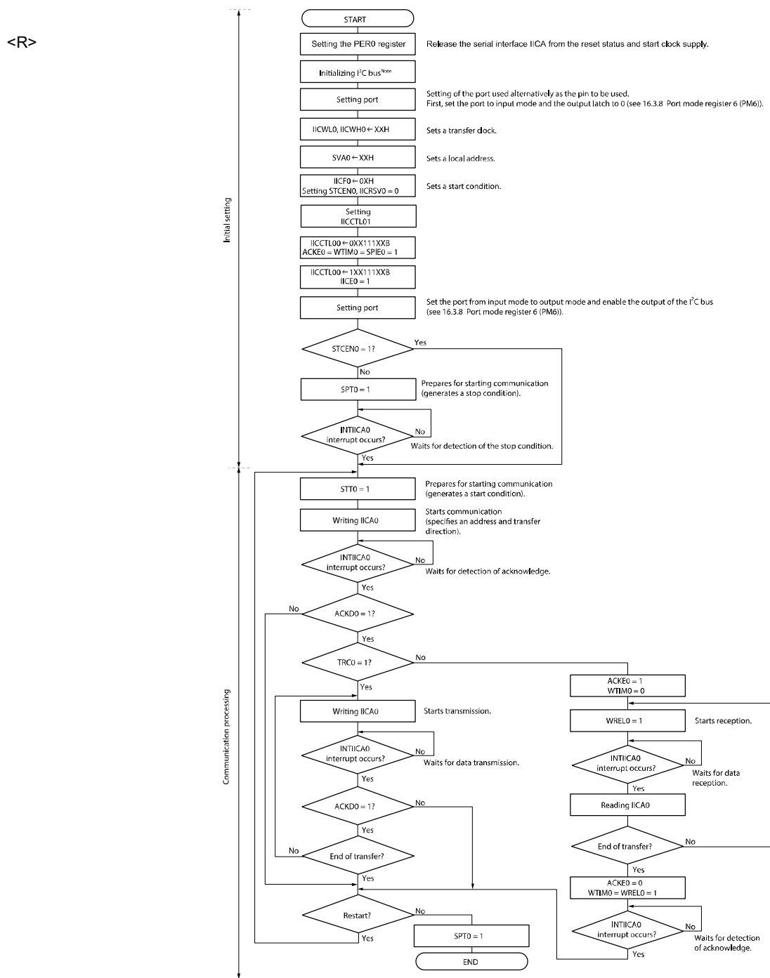
Figure 16-29. Master Operation in Single-Master System
