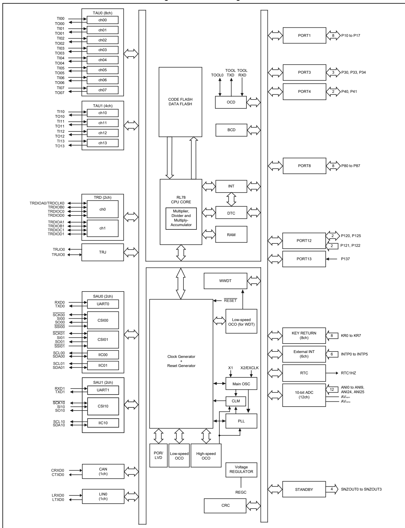
Figure 1-14. Block Diagram
