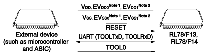
Figure 30-3. Environment for Writing Program to Flash Memory
