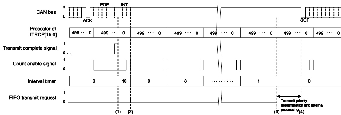
Figure 18-9. Interval Timer Timing Chart
