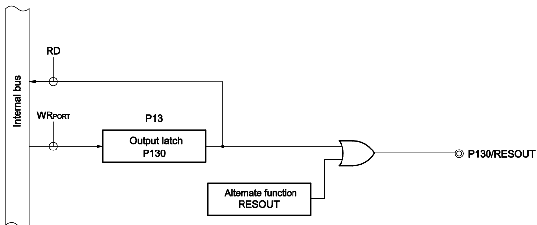
Figure 4-66. Block Diagram of P130
