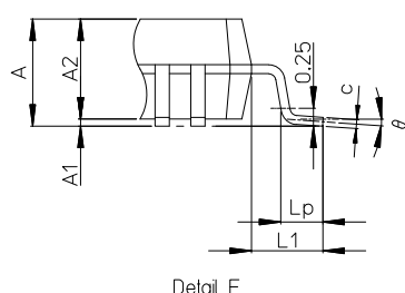
Detail F
