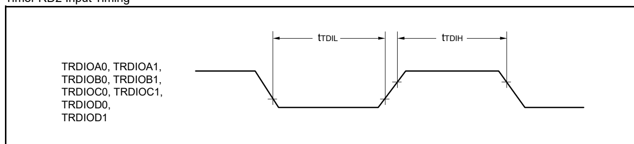
Timer RD2 Input Timing
