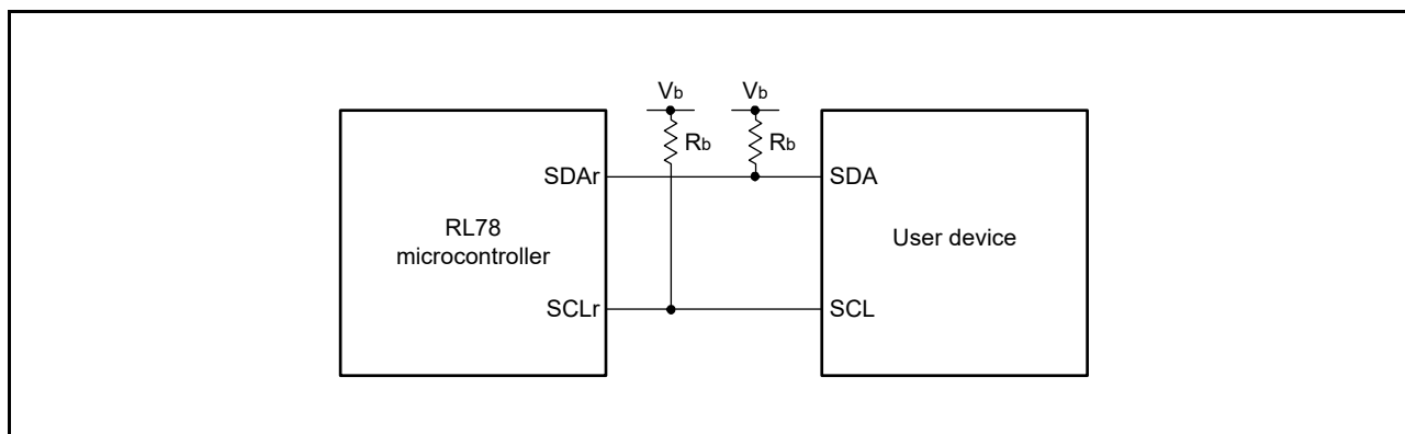
(a) Connection in the I 2 C communications with devices operating at different voltage levels
