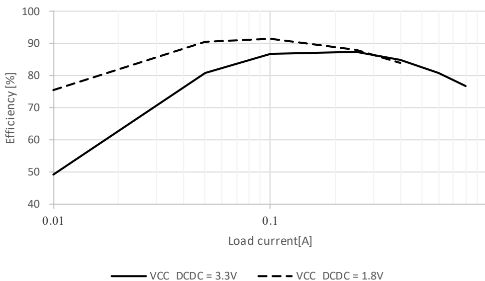
Figure 2.9 Typical DCDC efficiency (%) vs load current (A) in High-speed mode, T_j = 25^\circ\text{C}
