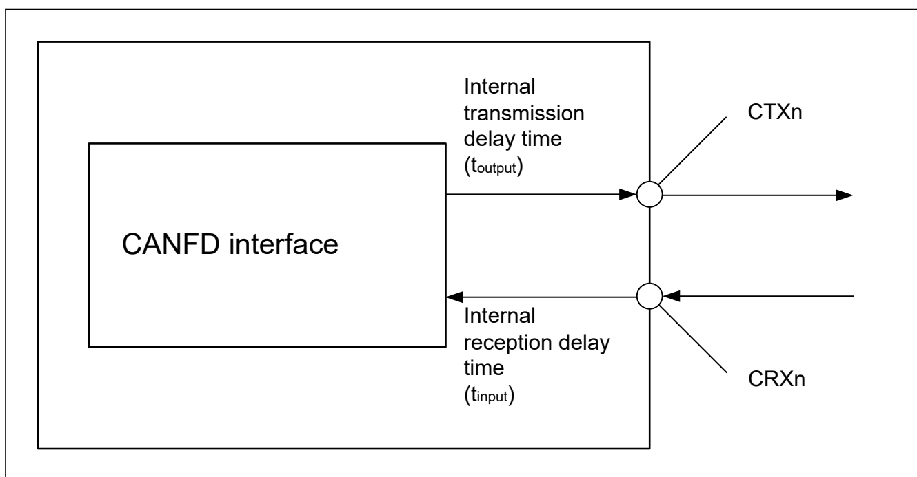
Figure 2.90 CANFD interface condition
