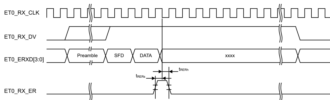
Figure 2.99 MII reception timing when an error occurs
