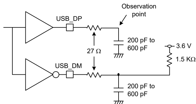
Figure 2.109 Test circuit in low-speed mode
