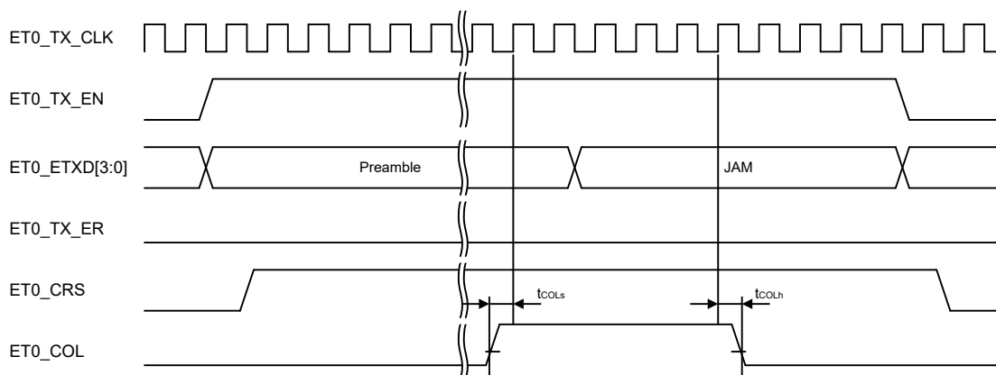
Figure 2.97 MII transmission timing when a conflict occurs
