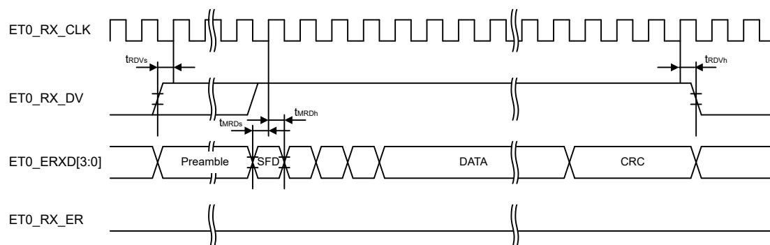
Figure 2.98 MII reception timing in normal operation
