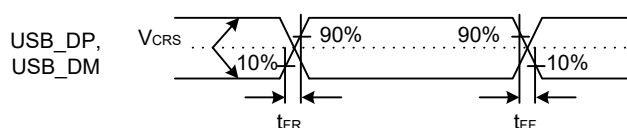
Figure 2.110 USB_DP and USB_DM output timing in full-speed mode
