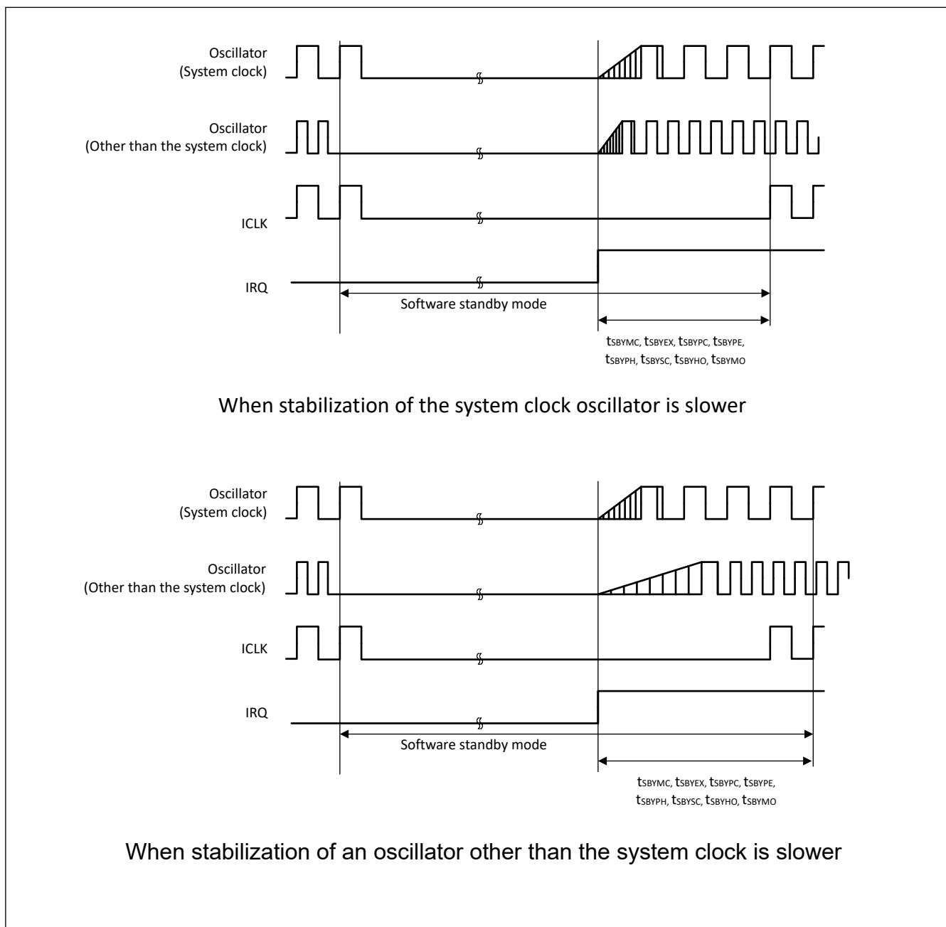
Figure 2.24 Software Standby mode cancellation timing
