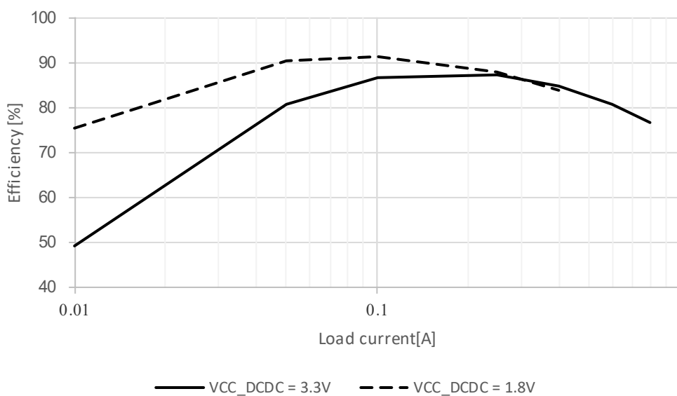
Figure 2.9 Typical DCDC efficiency (%) vs load current (A) in High-speed mode, T_j = 25^\circ C
