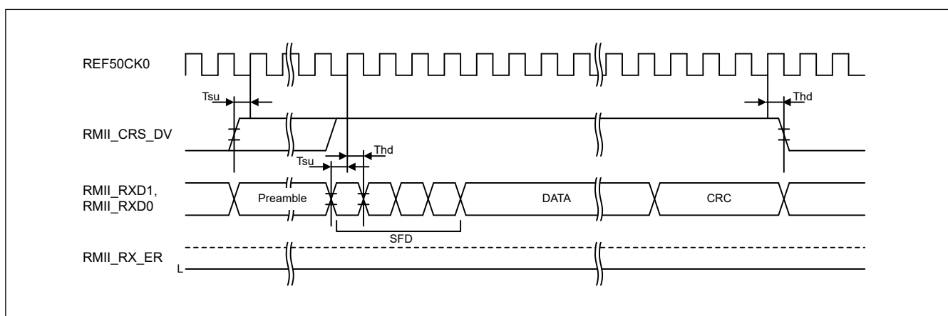
Figure 2.93 RMII reception timing in normal operation
