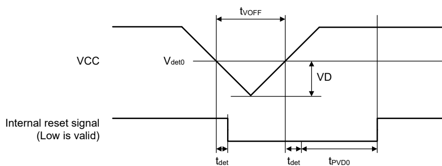
Figure 2.119 Voltage detection circuit timing ( V_{det0} )
