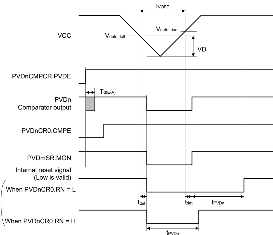
Figure 2.123 Voltage detection circuit timing ( V_{detn} ) ( n = 1, 2 )
