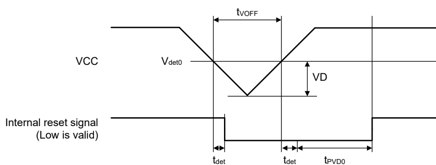
Figure 2.122 Voltage detection circuit timing ( V_{det0} )
