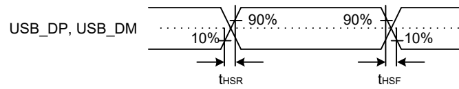
Figure 2.117 USB_DP and USB_DM output timing (high-speed)
