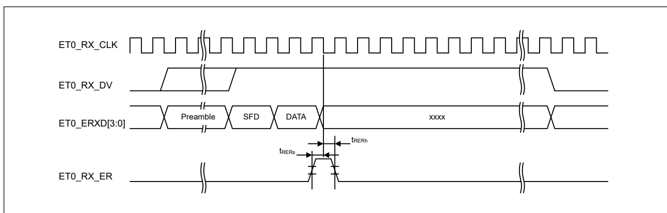
Figure 2.99 MII reception timing when an error occurs
