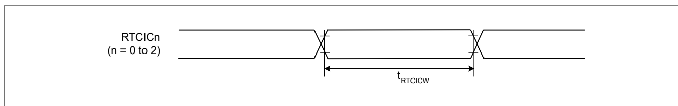
Figure 2.43 RTCICn input timing
