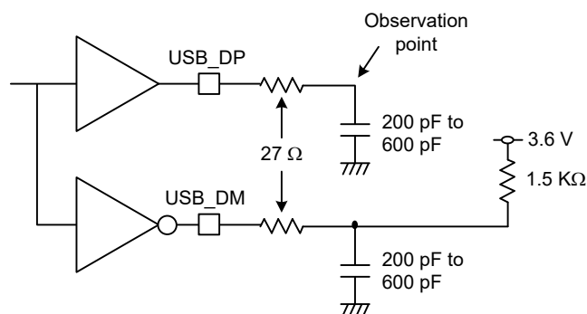
Figure 2.112 Test circuit in low-speed mode
