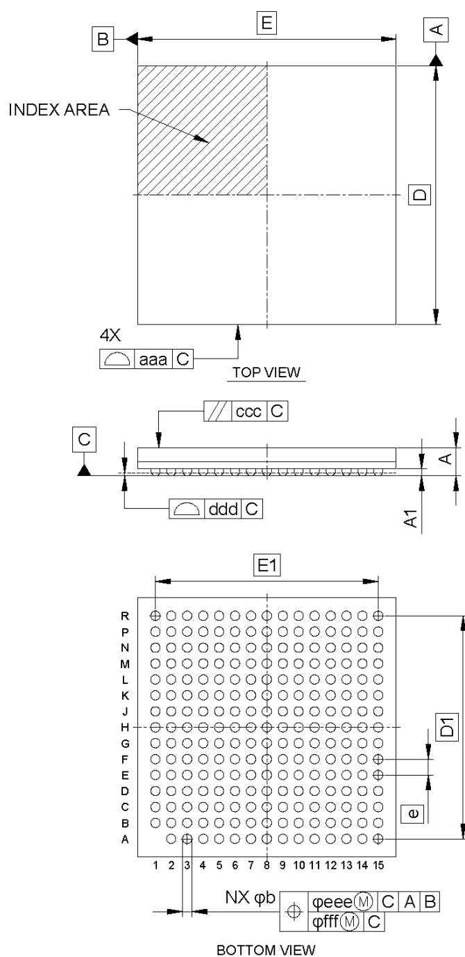
Figure 2.2 BGA 224-pin
