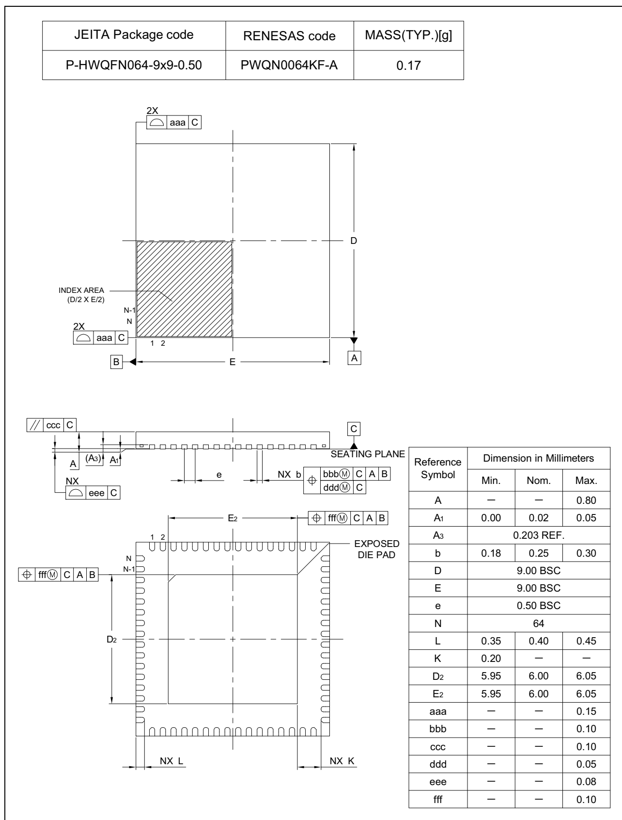
Figure D 64-Pin HWQFN (PWQN0064KF-A)
