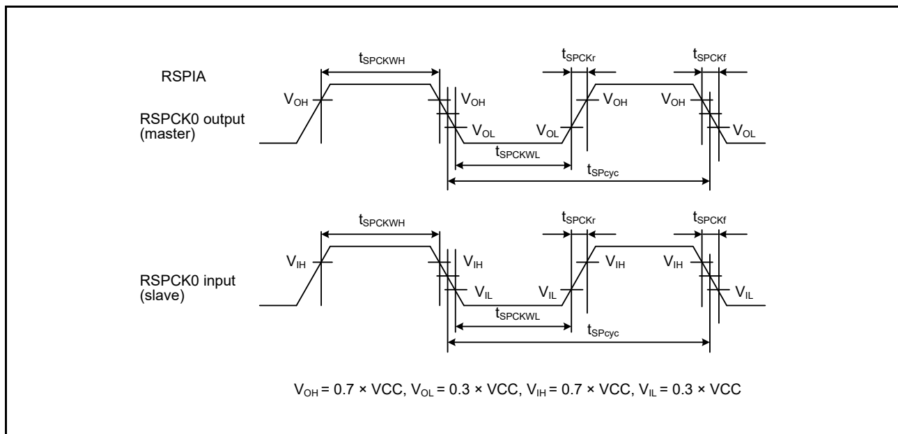
Figure 2.59 RSPIA Clock Timing
