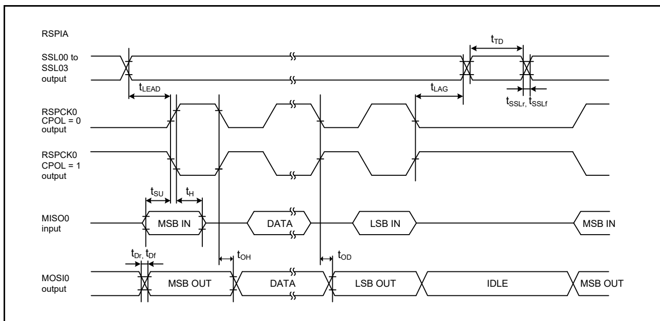
Figure 2.60 RSPIA Timing (Master, Motorola SPI, CPHA = 0)
