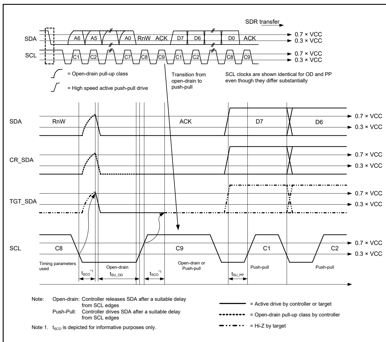
Figure 2.69 R13C Data Transfer — ACK by Target
