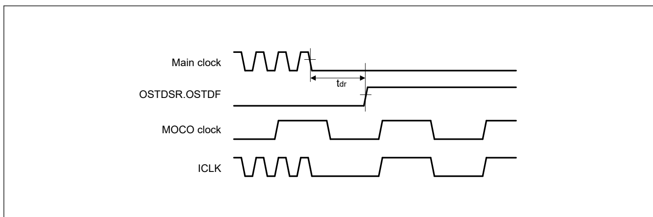
Figure 2.54 Oscillation stop detection timing
