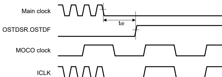
Figure 2.52 Oscillation stop detection timing
