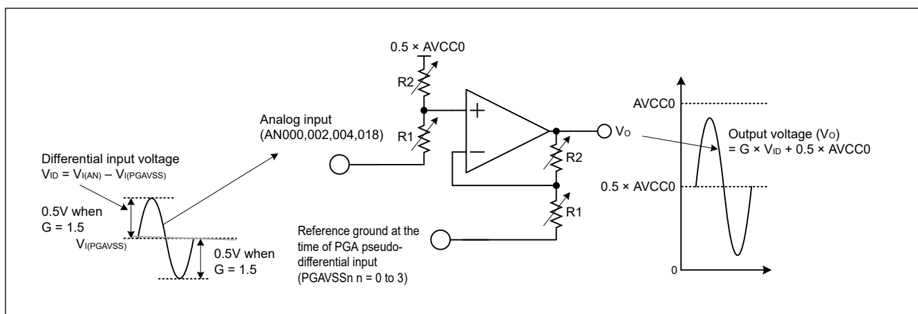
Figure 2.51 Input and Output Signal Levels with the PGA's Pseudo-Differential Setting
