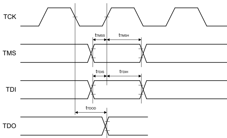
Figure 2.59 Boundary scan input/output timing
