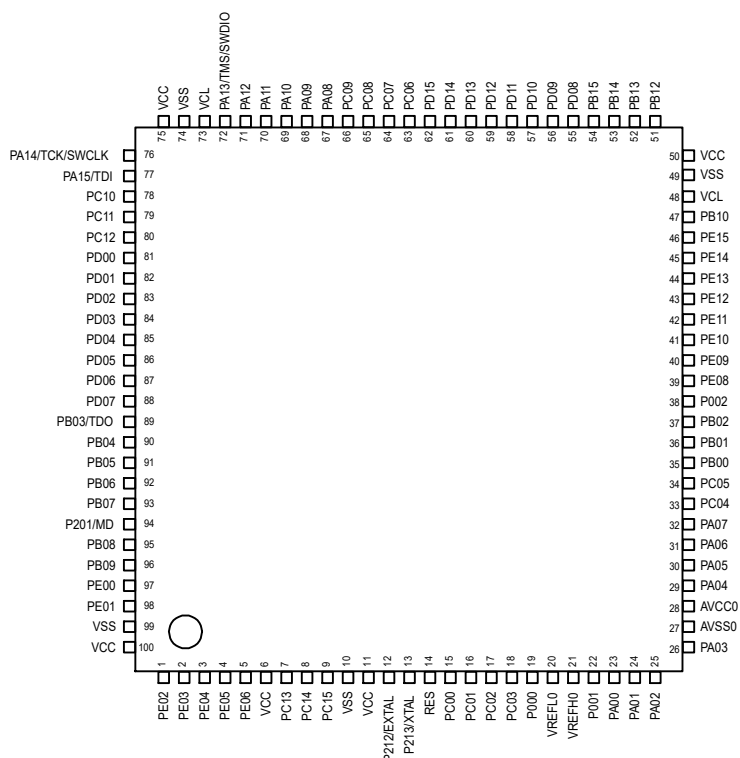
Figure 1.3 Pin assignment for LQFP 100-pin
