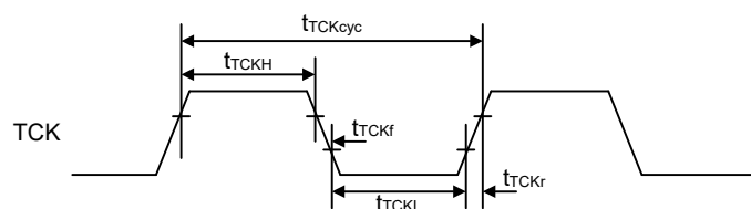
Figure 2.58 Boundary scan TCK timing
