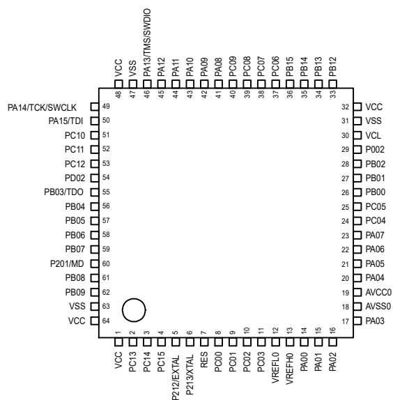
Figure 1.4 Pin assignment for LQFP 64-pin
