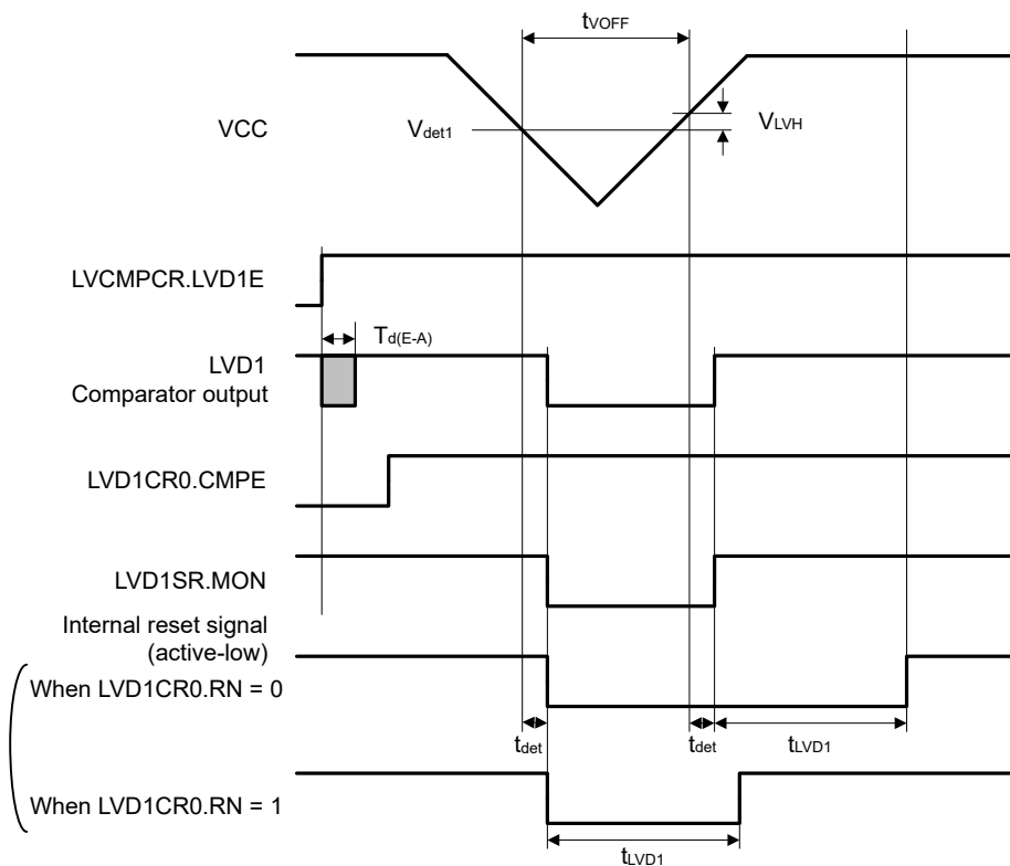
Figure 2.55 Voltage detection circuit timing ( V_{det1} )
