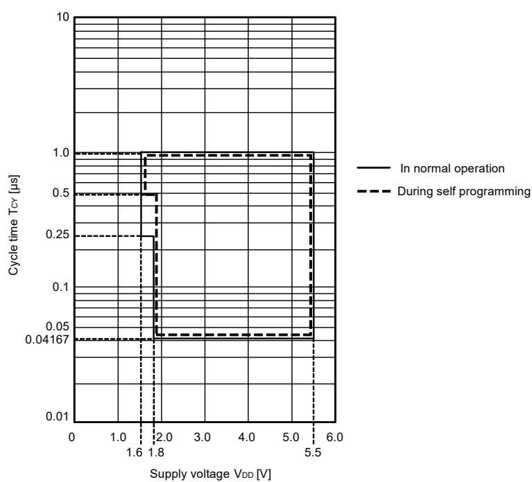
TCY vs VDD (LS (low-speed main) mode)
