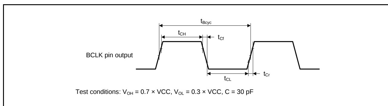
Figure 2.4 BCLK Pin Output Timing
