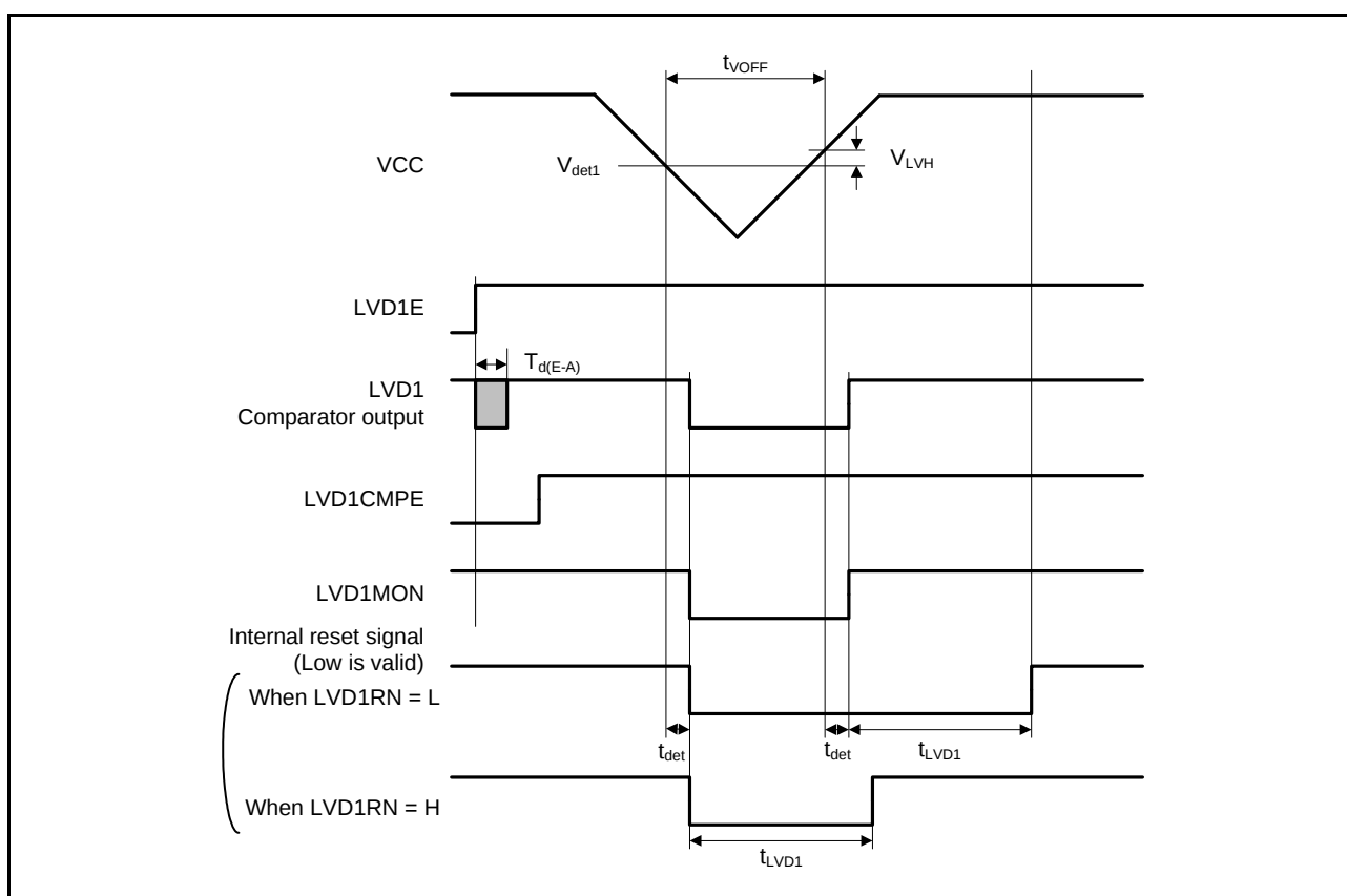
Figure 2.62 Voltage Detection Circuit Timing ( V_{\text{det1}} )
