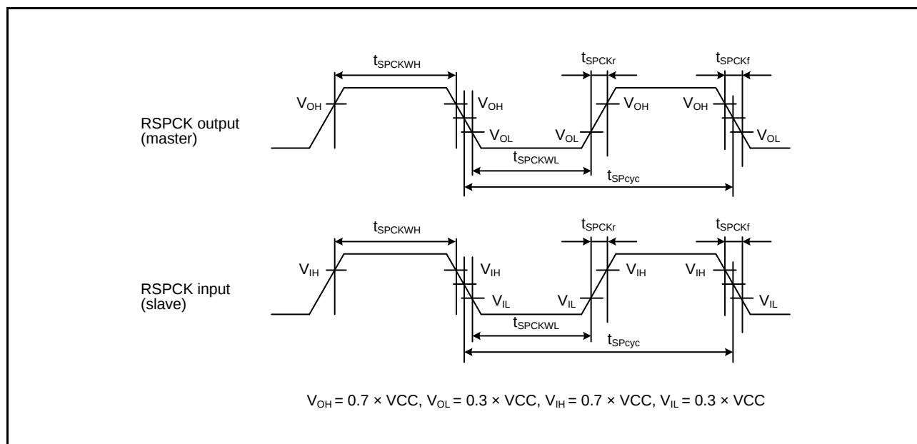
Figure 2.51 RSPI Clock Timing
