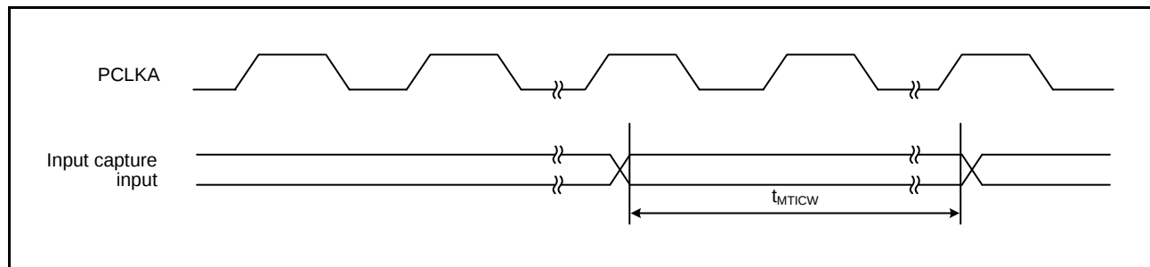
Figure 2.27 MTU Input Capture Input Timing
