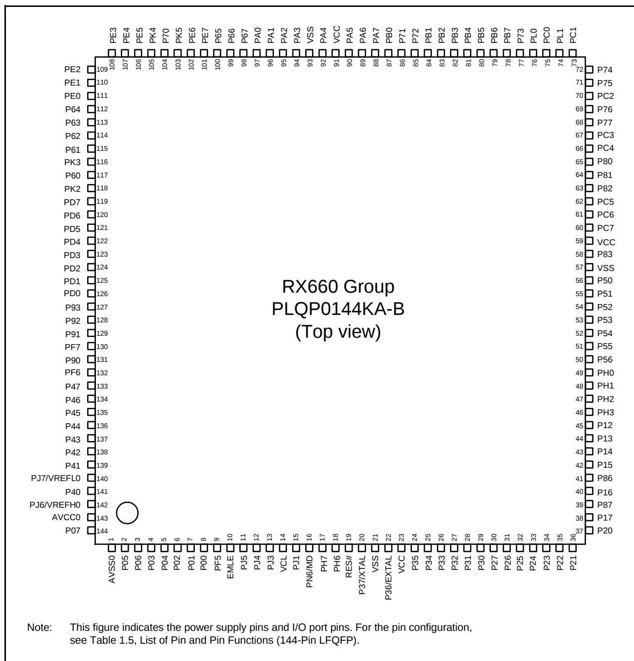
Figure 1.5 Pin Assignment (144-Pin LFQFP (with JTAG Interface, without Sub-clock Oscillator))
