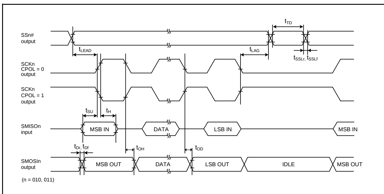
Figure 2.47 Simple SPI Timing (Master, CPHA = 0)
