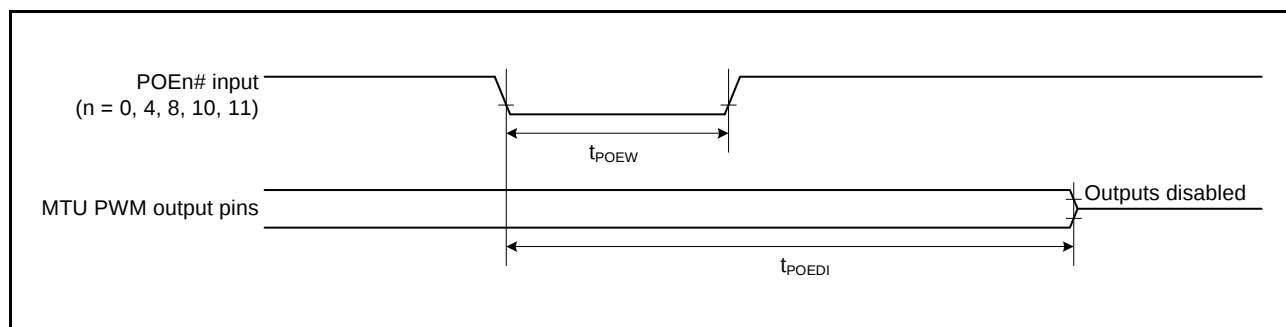
Figure 2.30 Output Disable Time for POE in Response to Transition of the POEn# Signal Level
