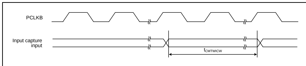
Figure 2.26 CMTW Input Capture Input Timing
