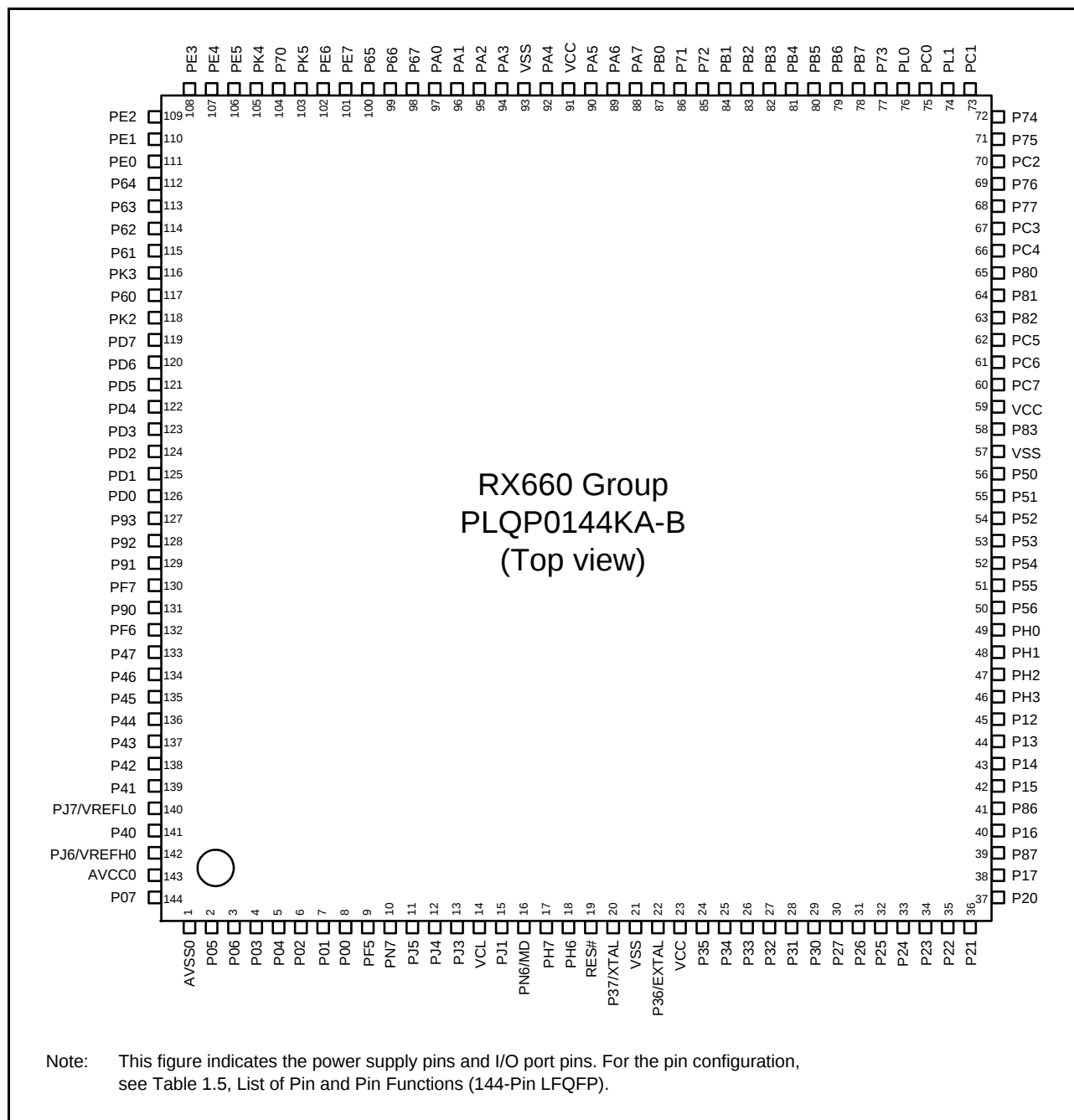
Figure 1.3 Pin Assignment (144-Pin LFQFP (without JTAG Interface, without Sub-clock Oscillator))
