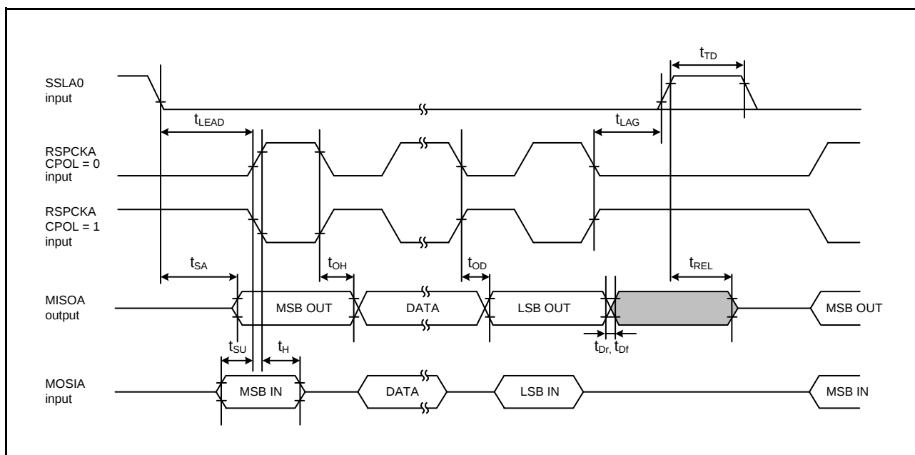
Figure 2.56 RSPI Timing (Slave, CPHA = 0)
