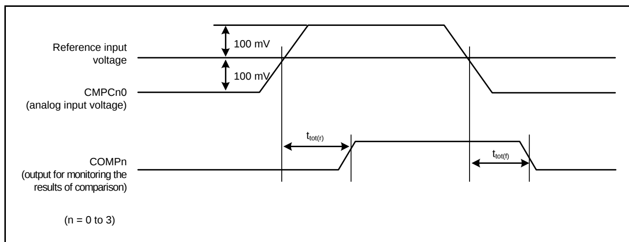
Figure 2.59 Comparator Response Time
