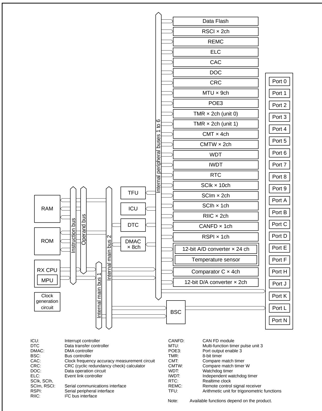
Figure 1.2 Block Diagram
