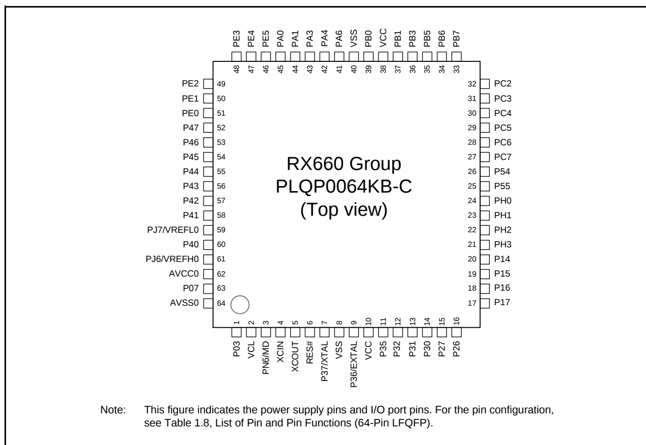
Figure 1.14 Pin Assignment (64-Pin LFQFP (with Sub-clock Oscillator))
