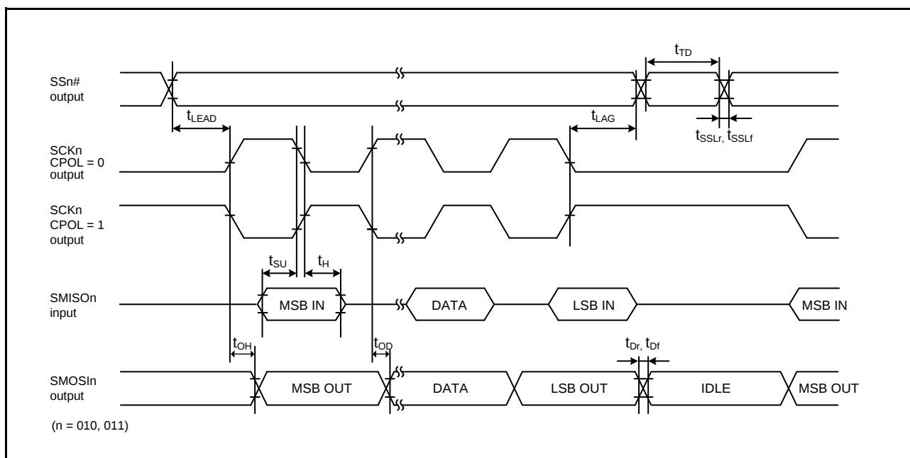
Figure 2.48 Simple SPI Timing (Master, CPHA = 1)
