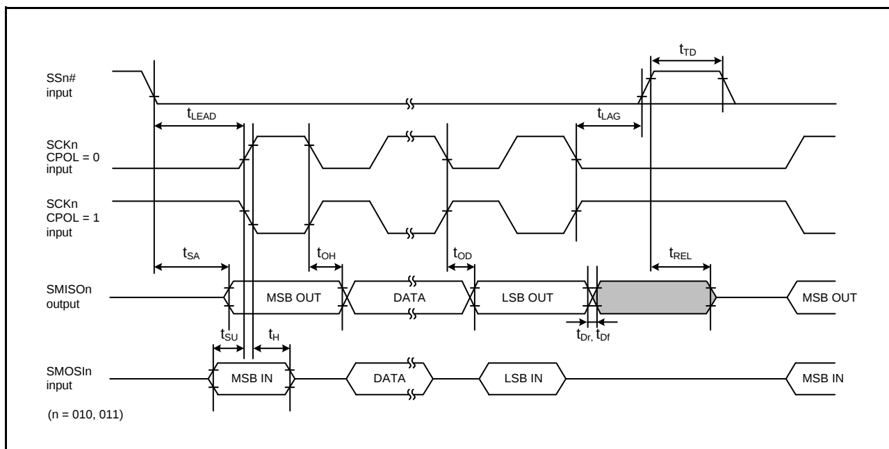
Figure 2.49 Simple SPI Timing (Slave, CPHA = 0)
