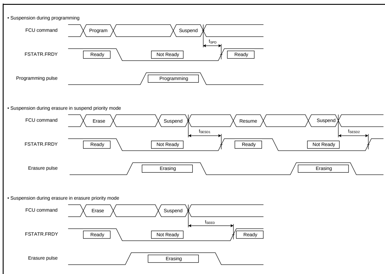
Figure 2.65 Flash Memory Programming/Erasure Suspension Timing
