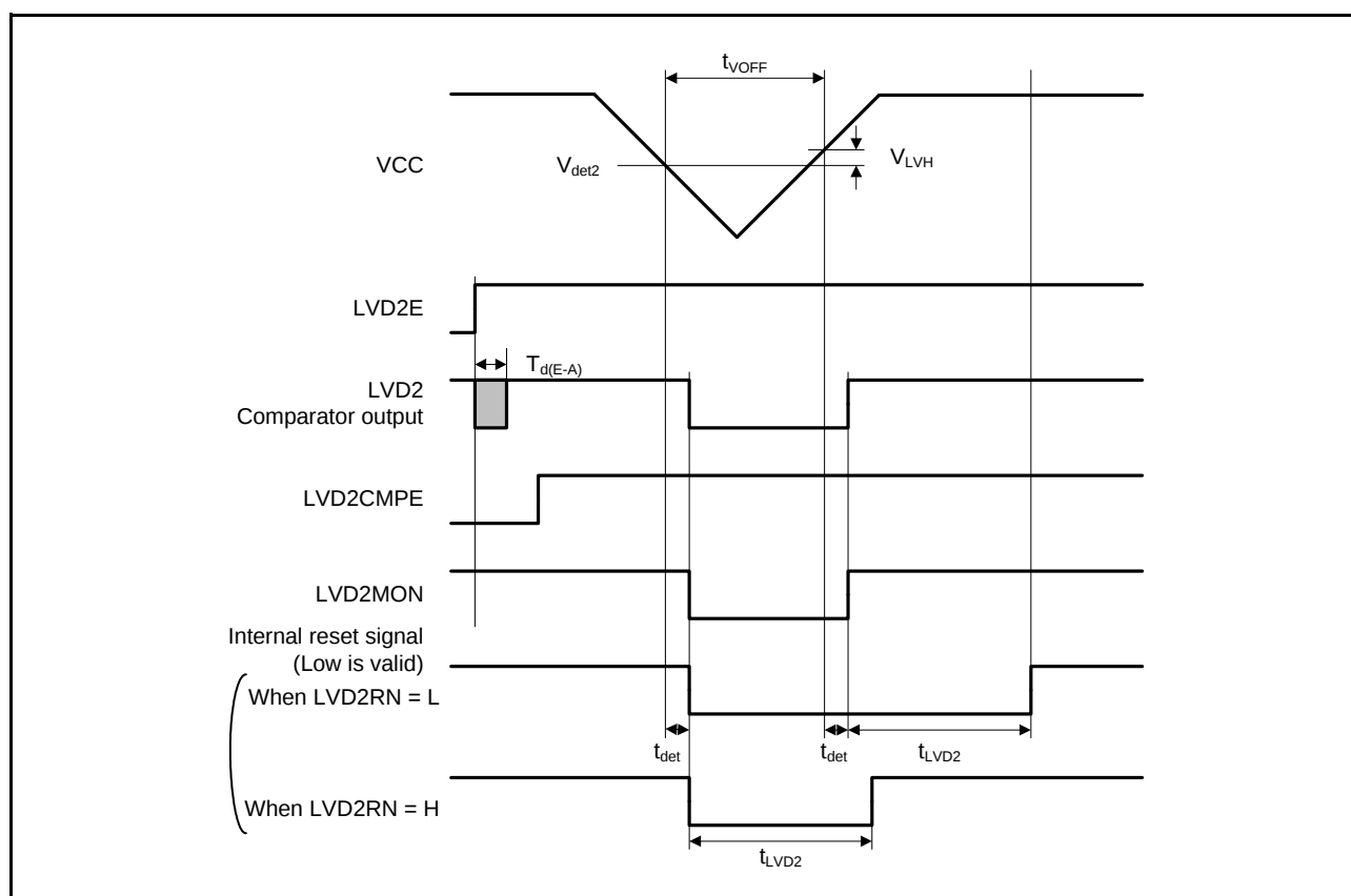
Figure 2.63 Voltage Detection Circuit Timing (V det2 )
