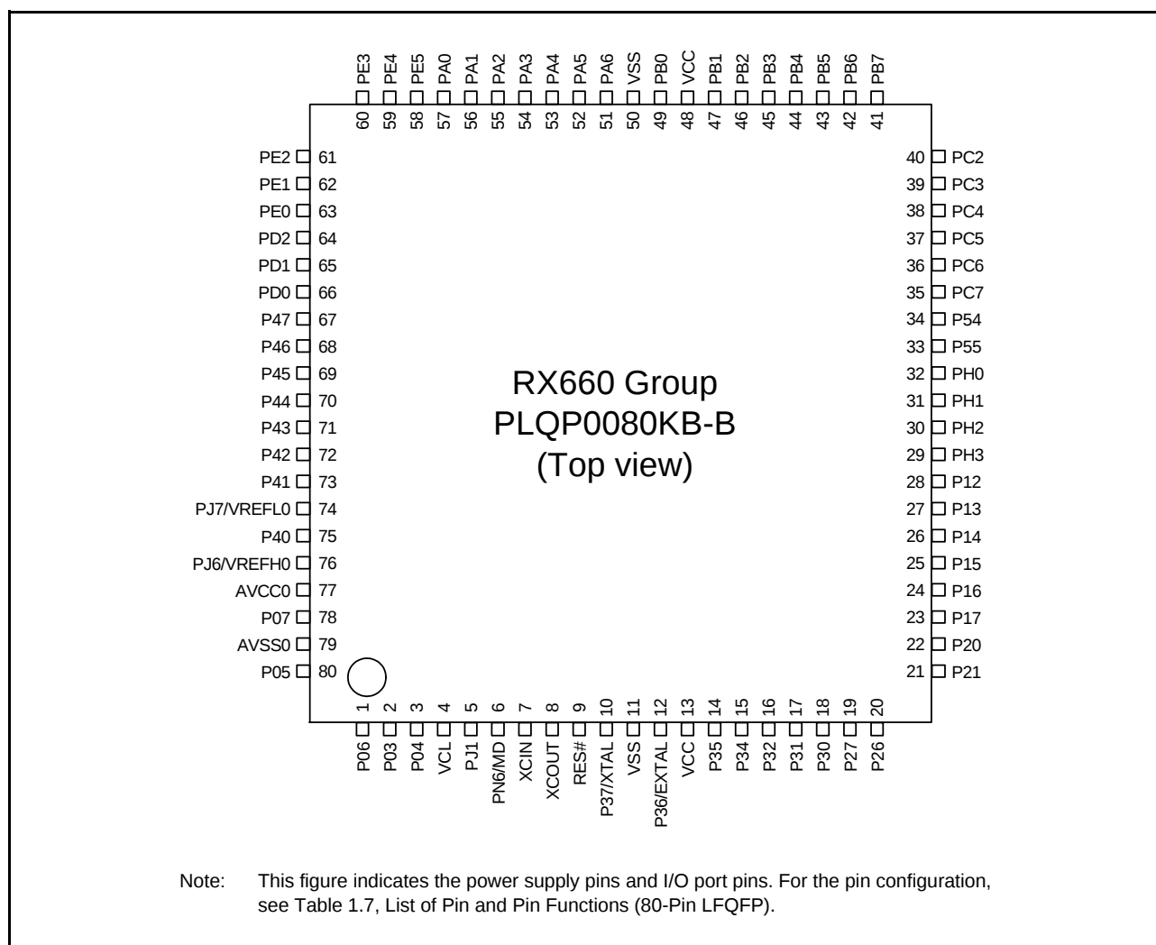
Figure 1.12 Pin Assignment (80-Pin LFQFP (with Sub-clock Oscillator))
