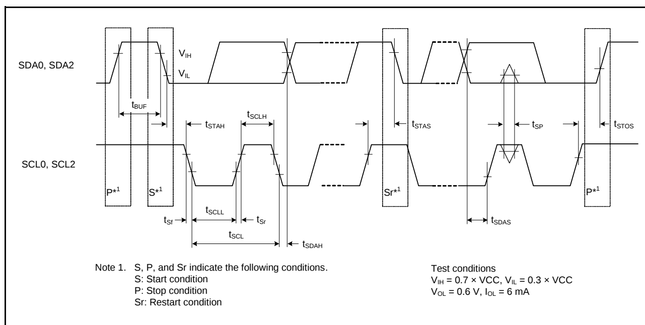
Figure 2.58 IIC Bus Interface Input/Output Timing
