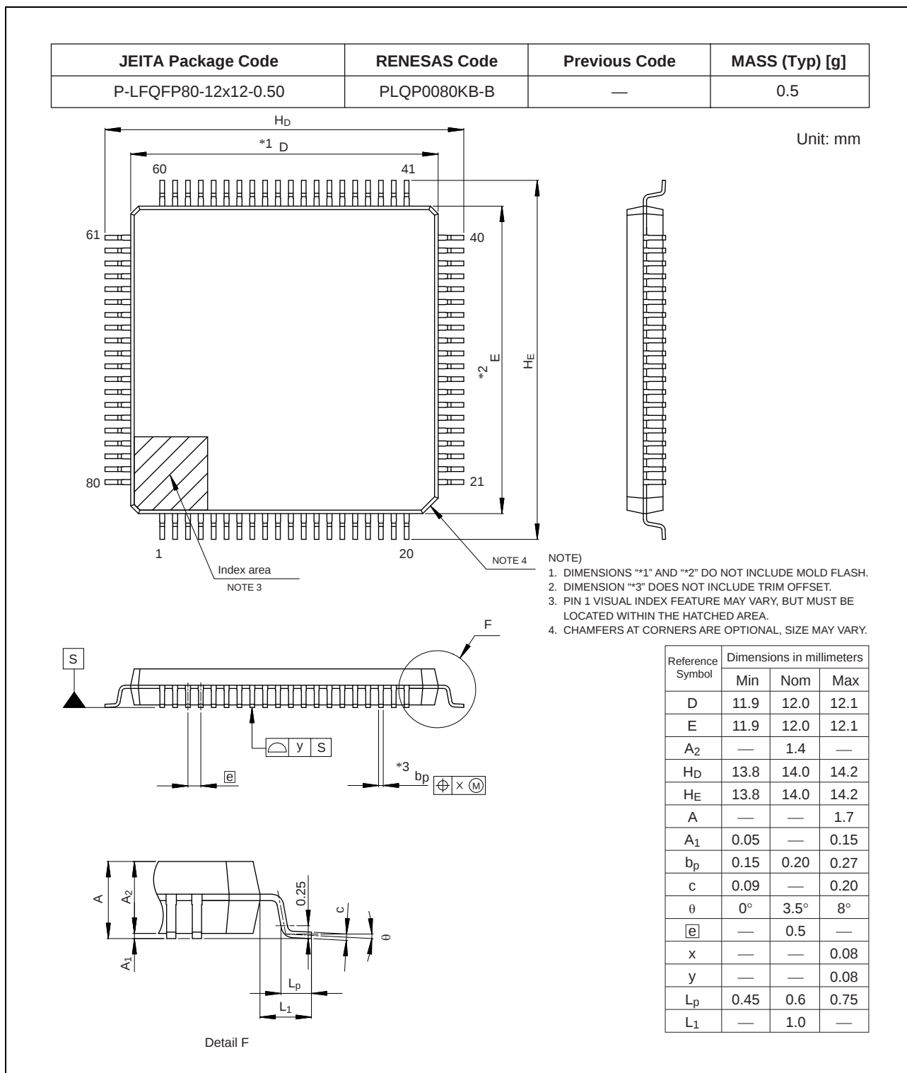
Figure C 80-Pin LFQFP (PLQP0080KB-B)
