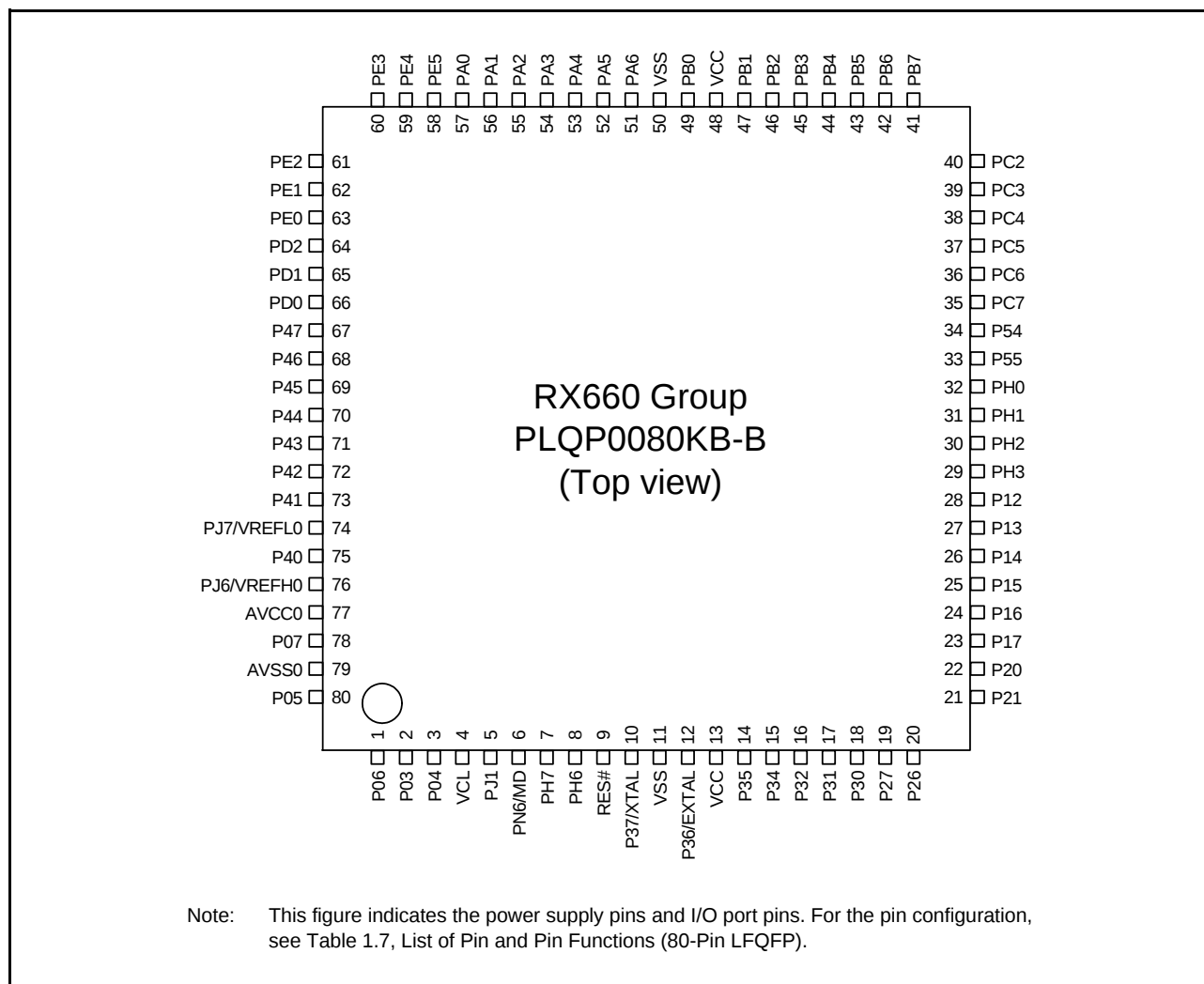
Figure 1.11 Pin Assignment (80-Pin LFQFP (without Sub-clock Oscillator))
