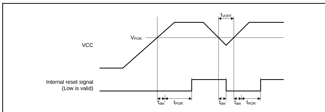
Figure 2.60 Power-on Reset Timing
