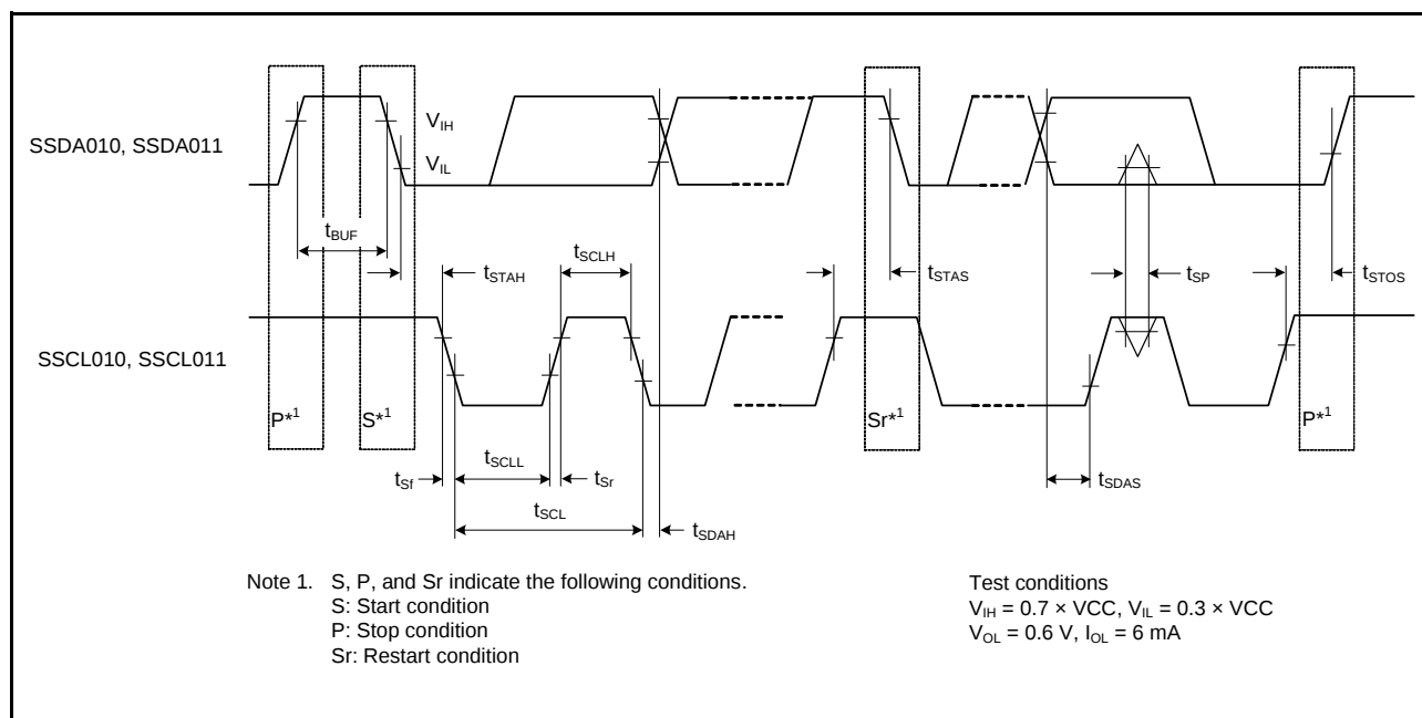
Figure 2.45 Simple IIC Bus Interface Input/Output Timing
