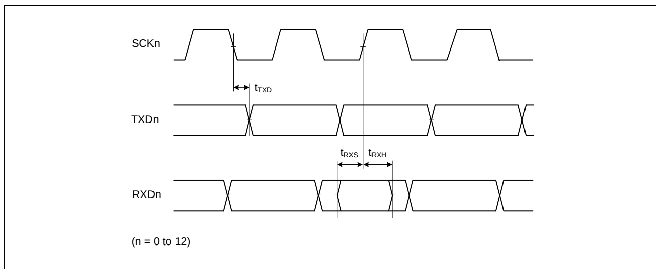
Figure 2.36 SCI Input/Output Timing: Clock Synchronous Mode
