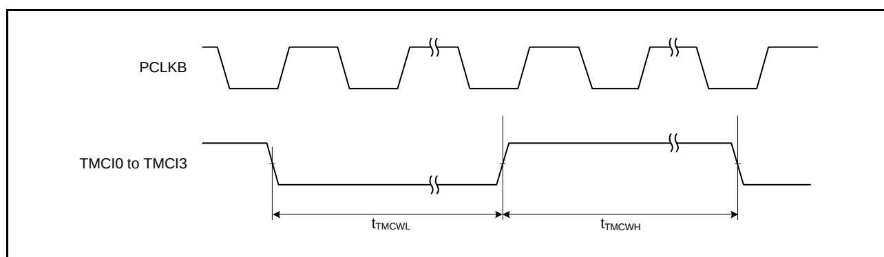
Figure 2.25 TMR Clock Input Timing
