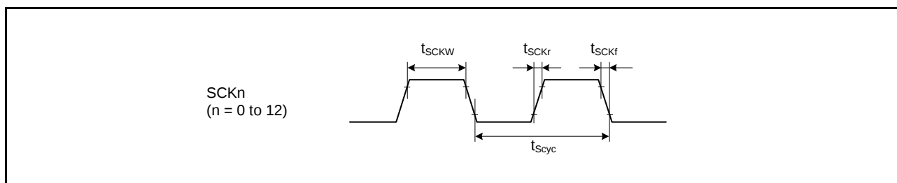
Figure 2.35 SCK Clock Input Timing
