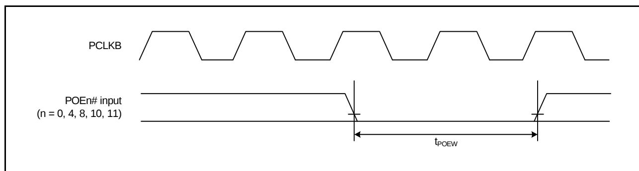
Figure 2.29 POE# Pin Input Timing
