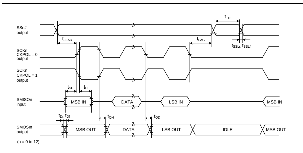
Figure 2.39 Simple SPI Timing (Master, CKPH = 1)
