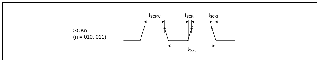
Figure 2.43 SCK Clock Input Timing
