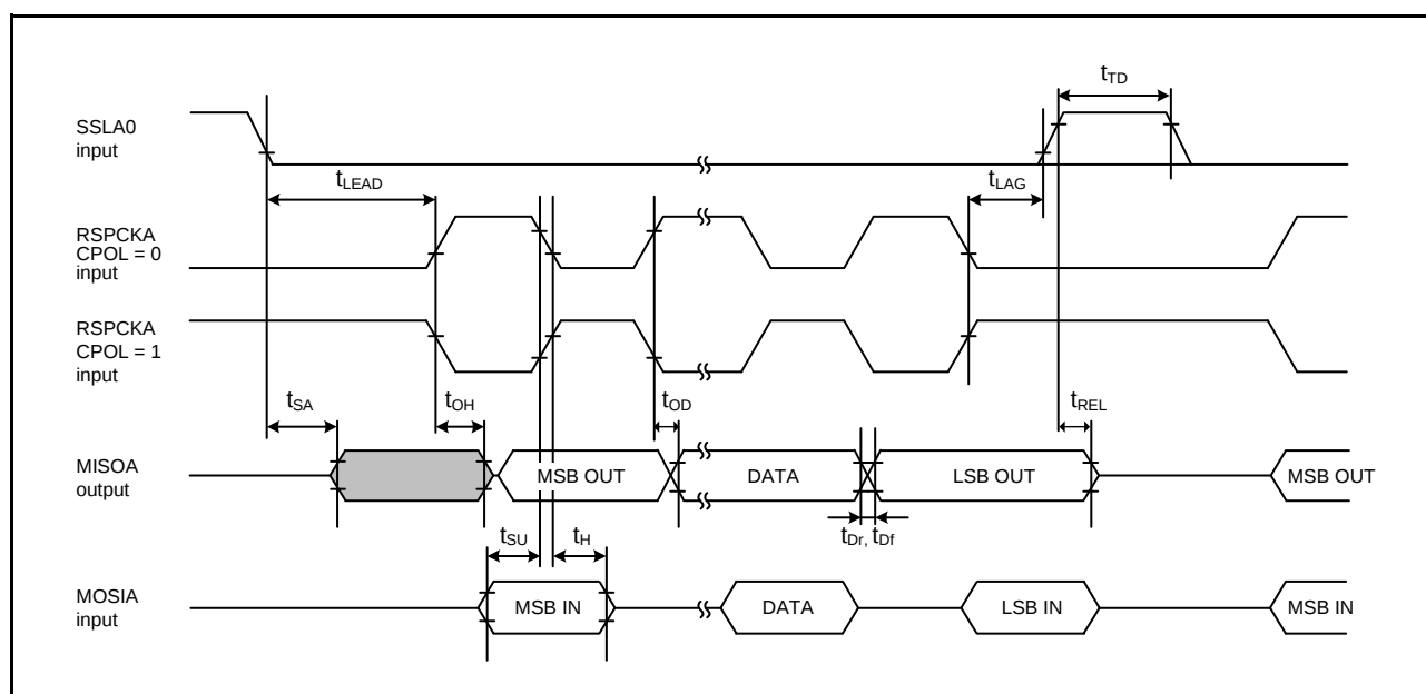
Figure 2.57 RSPi Timing (Slave, CPHA = 1)
