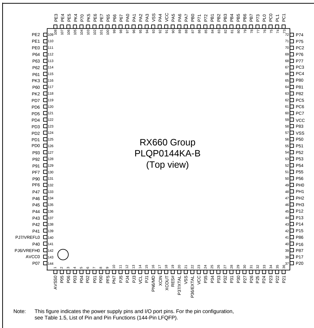
Figure 1.4 Pin Assignment (144-Pin LFQFP (without JTAG Interface, with Sub-clock Oscillator))
