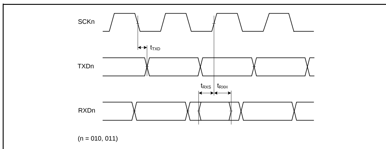
Figure 2.44 RSCI Input/Output Timing: Clock Synchronous Mode
