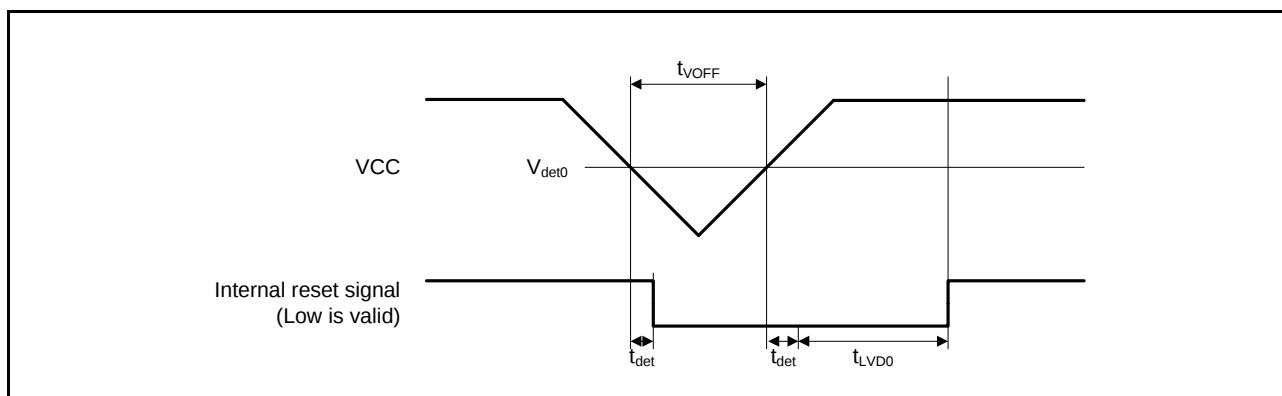
Figure 2.61 Voltage Detection Circuit Timing ( V_{det0} )
