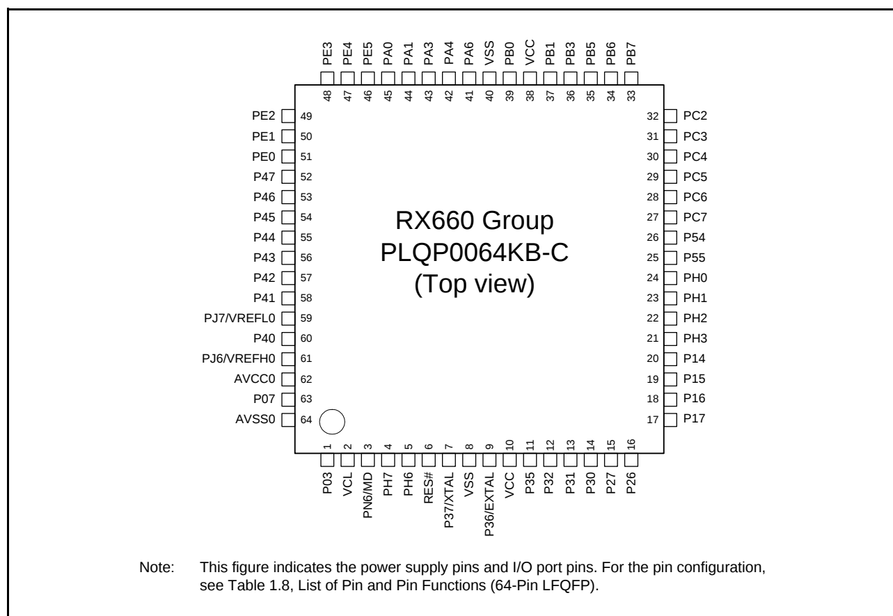
Figure 1.13 Pin Assignment (64-Pin LFQFP (without Sub-clock Oscillator))
