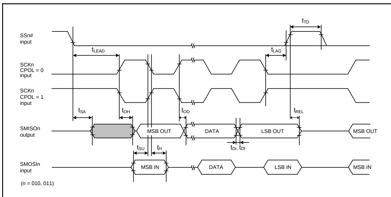
Figure 2.50 Simple SPI Timing (Slave, CPHA = 1)
