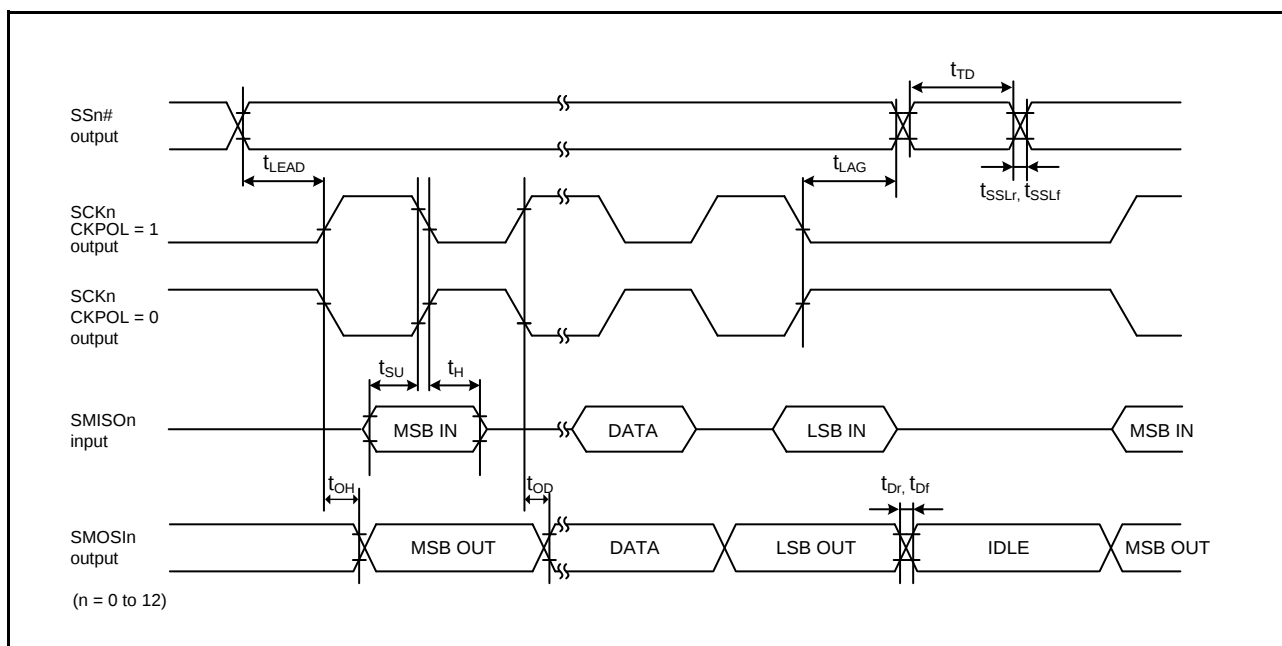
Figure 2.40 Simple SPI Timing (Master, CKPH = 0)
