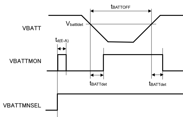
Figure 2.65 Battery backup function characteristics
