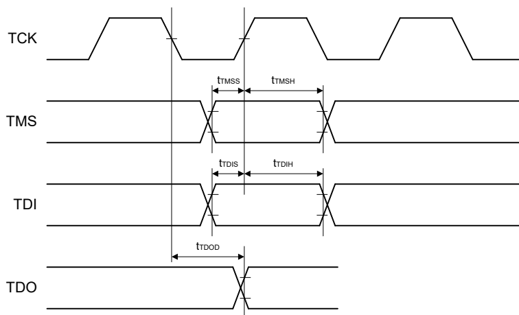
Figure 2.68 Boundary scan input/output timing
