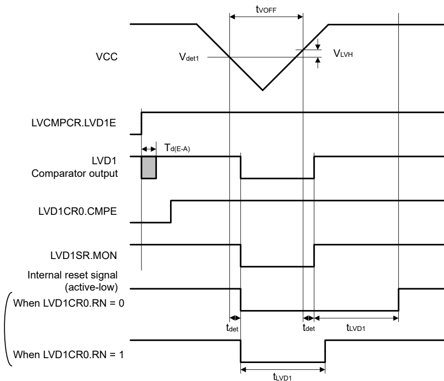
Figure 2.62 Voltage detection circuit timing ( V_{det1} )
