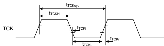
Figure 2.67 Boundary scan TCK timing
