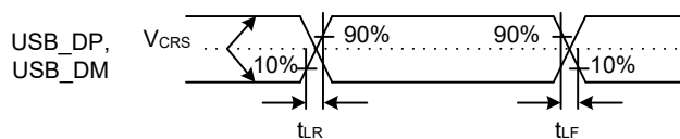
Figure 2.54 USB_DP and USB_DM output timing in low-speed mode
