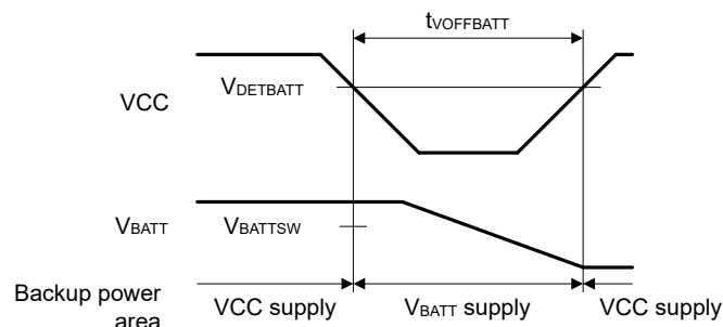
Figure 2.64 Battery backup function characteristics
