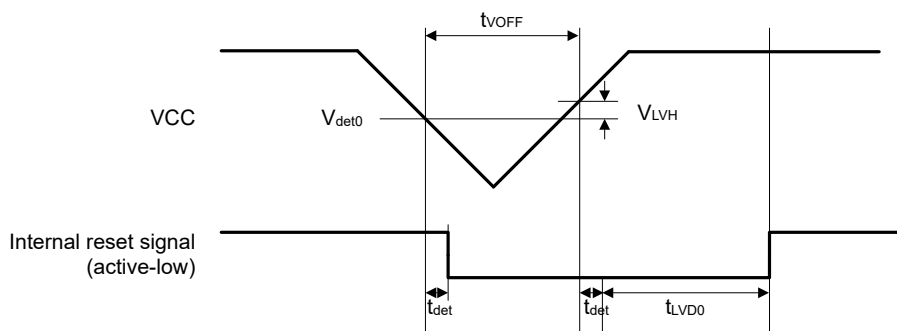
Figure 2.61 Voltage detection circuit timing ( V_{det0} )
