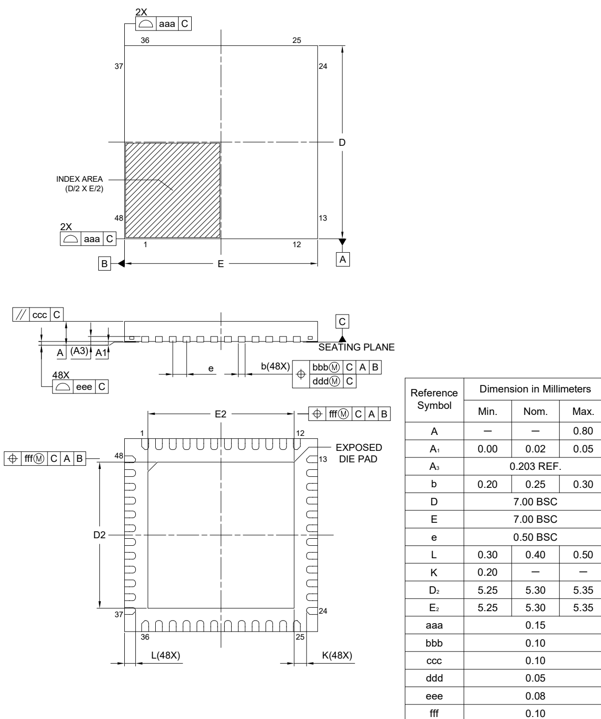
Figure 2.6 HWQFN 48-pin
