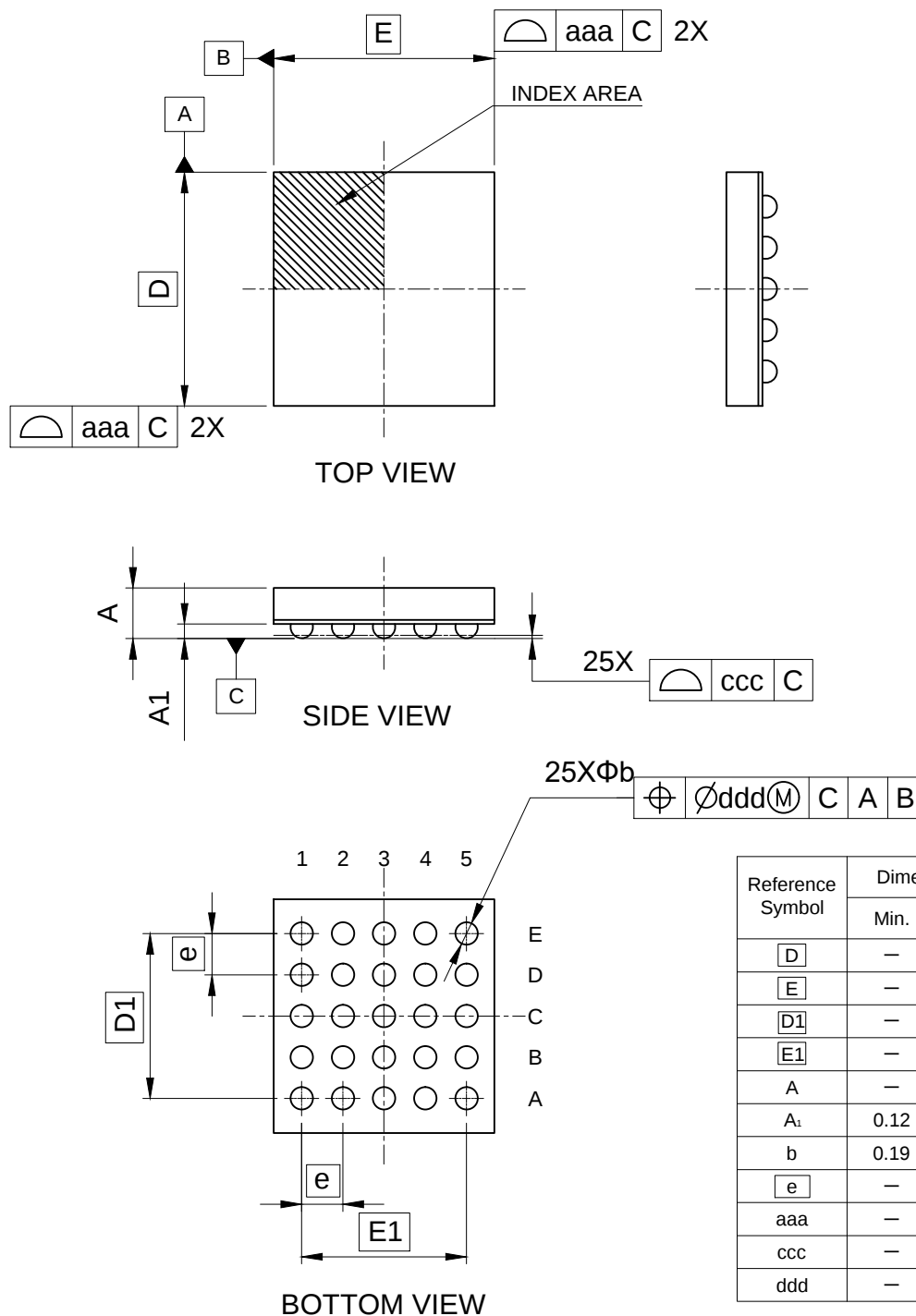
Figure 2.9 WLCSP 25-pin
