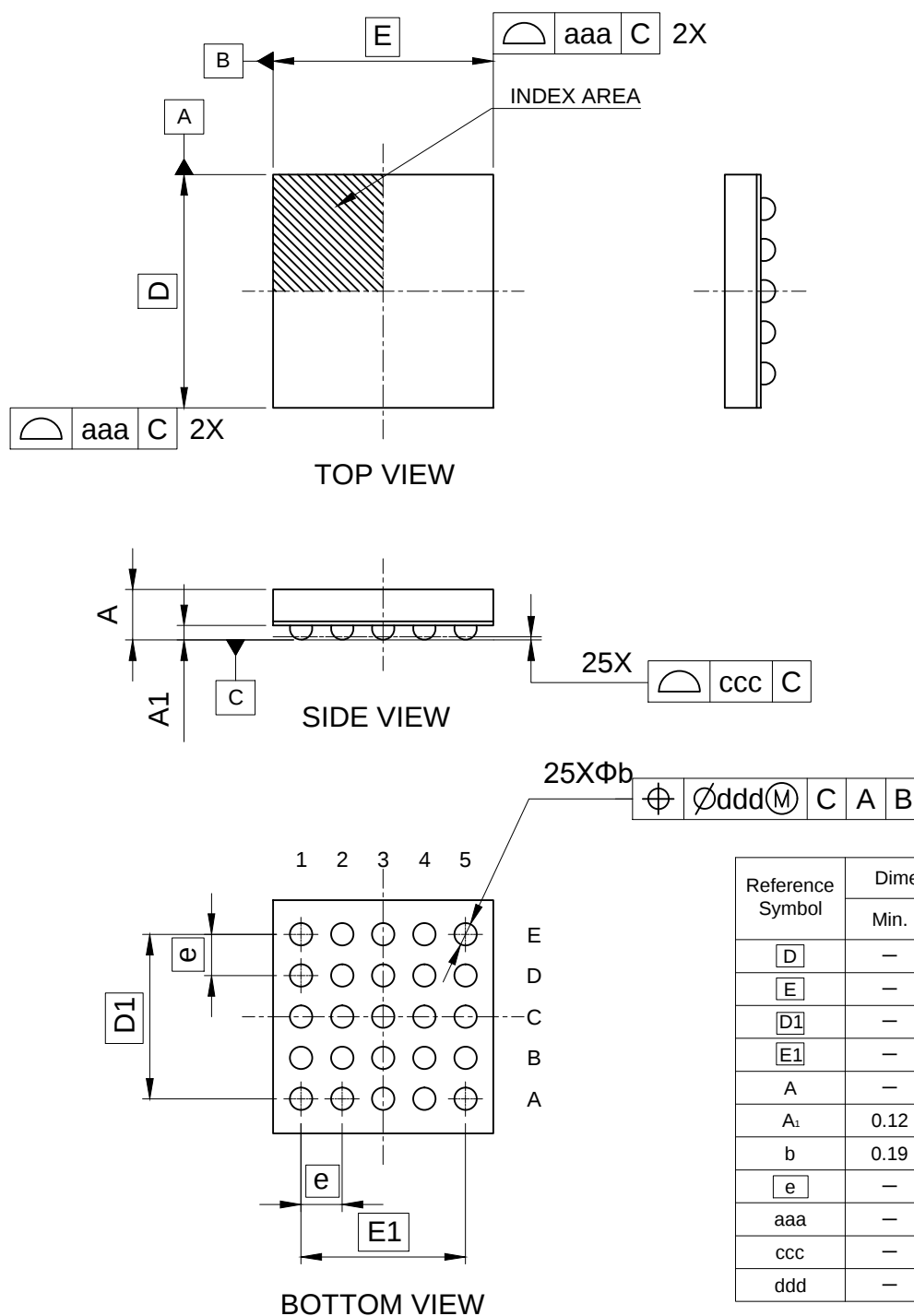
Figure 2.9 WLCSP 25-pin
