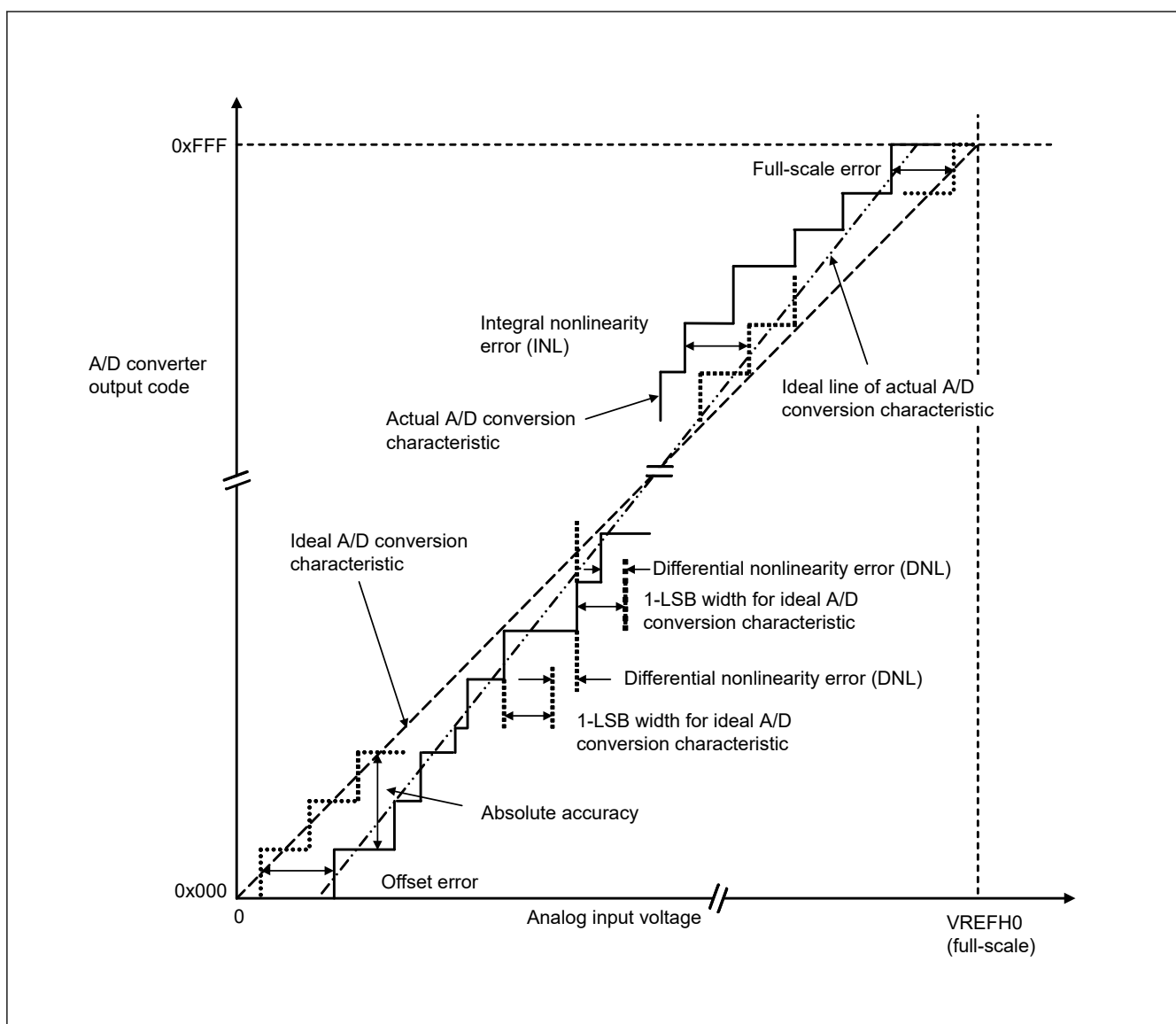
Figure 2.39 Illustration of 12-bit A/D converter characteristic terms
