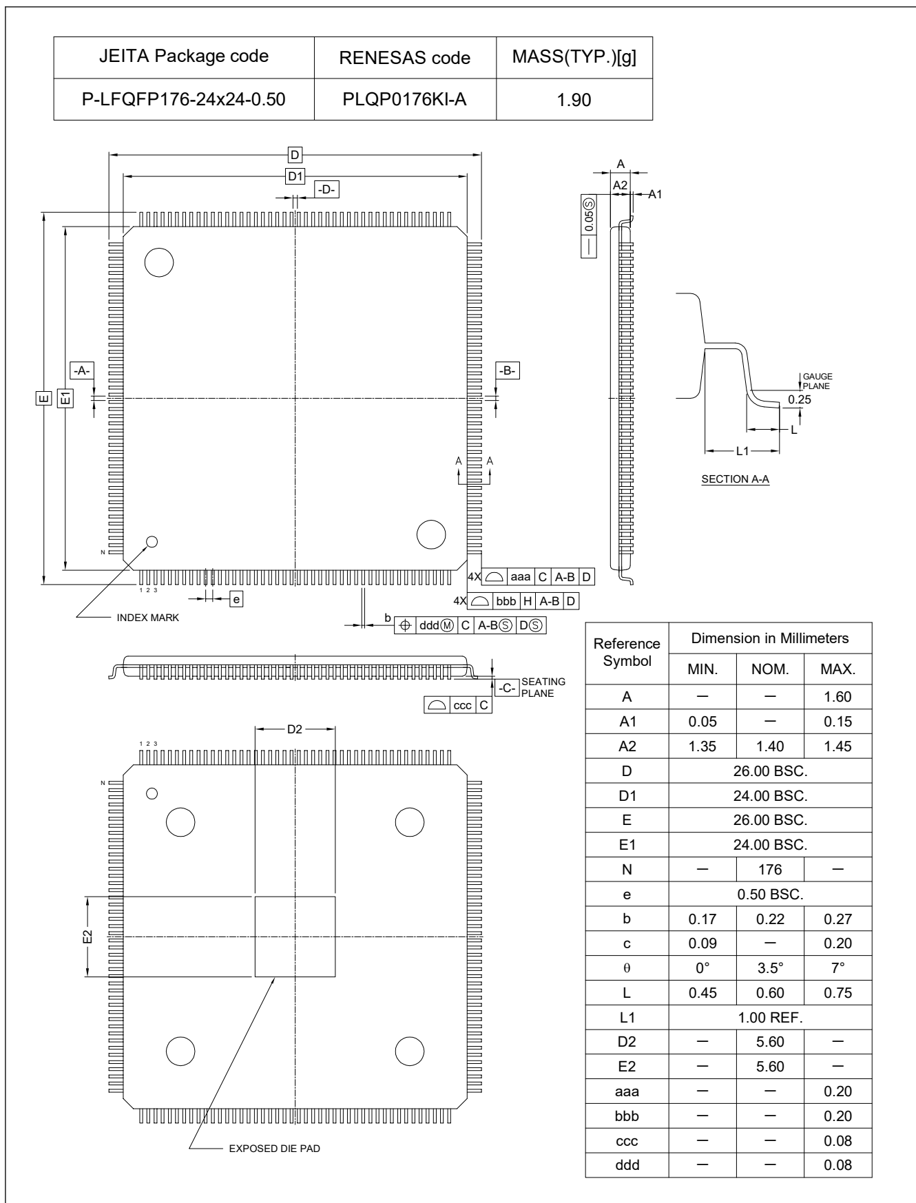
Figure 1.3 176-pin LQFP with exposed die pad
