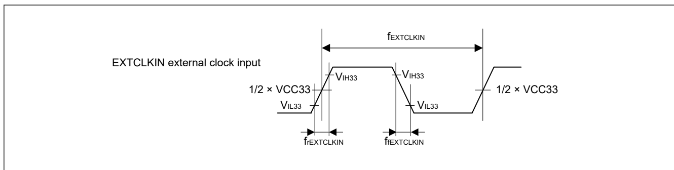
Figure 2.4 EXTCLKIN external clock input timing
