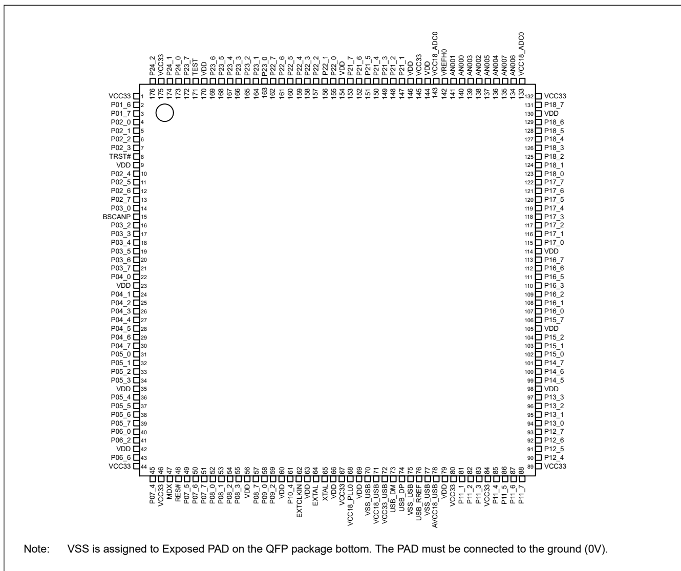
Figure 1.4 Pin arrangement (176-pin LQFP) (top view)
