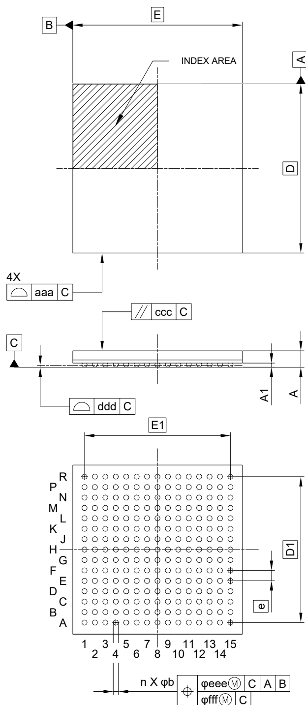
Figure 1.2 225-pin FBGA
