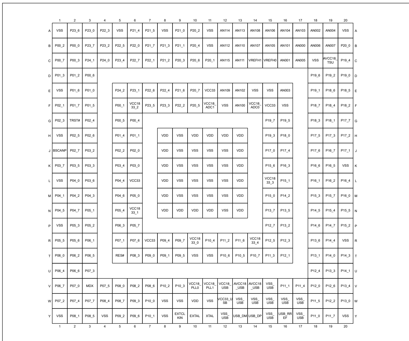
Figure 1.2 Pin arrangement (320-pin FBGA) (top view)
