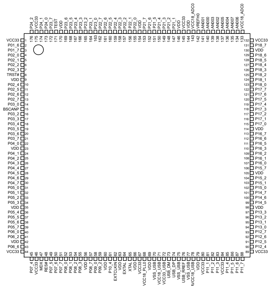
Figure 1.4 Pin arrangement (176-pin LQFP) (top view)
