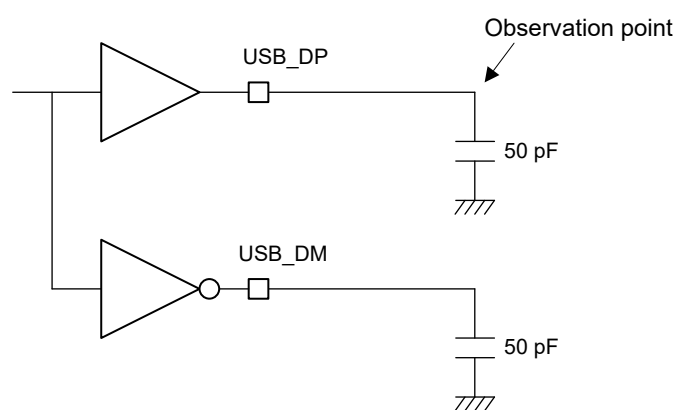
Figure 2.90 Measurement circuit (full speed)
