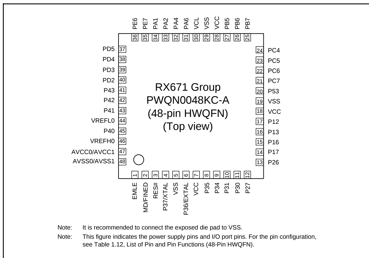
Figure 1.10 Pin Assignment (48-Pin HWQFN)
