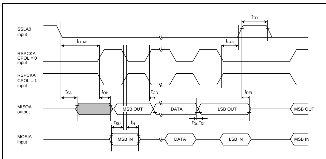
Figure 2.74 RSPI Timing (Slave, CPHA = 1)
