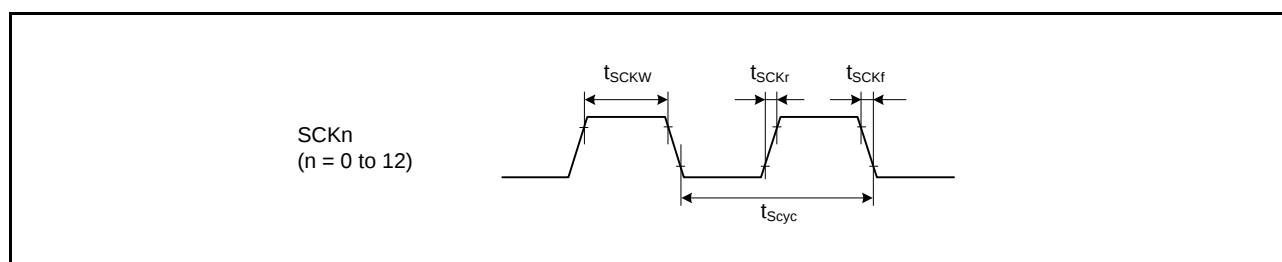
Figure 2.47 SCK Clock Input Timing
