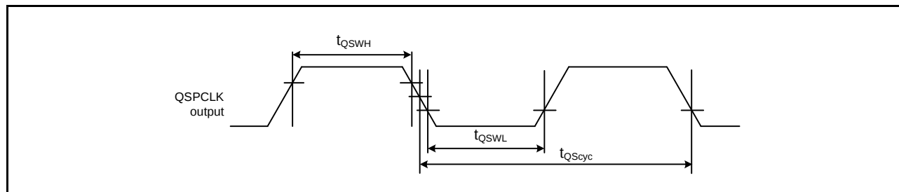
Figure 2.83 QSPIX Clock Timing
