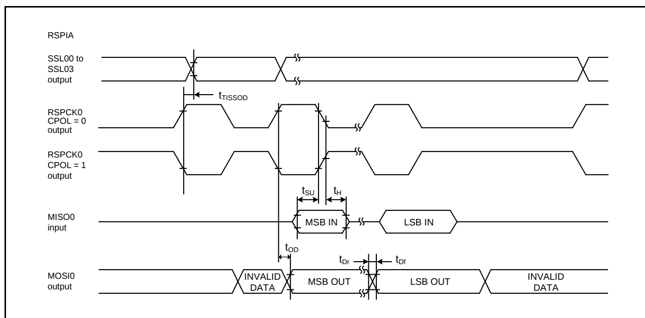
Figure 2.78 RSPIA Timing (Master, TI SSP)
