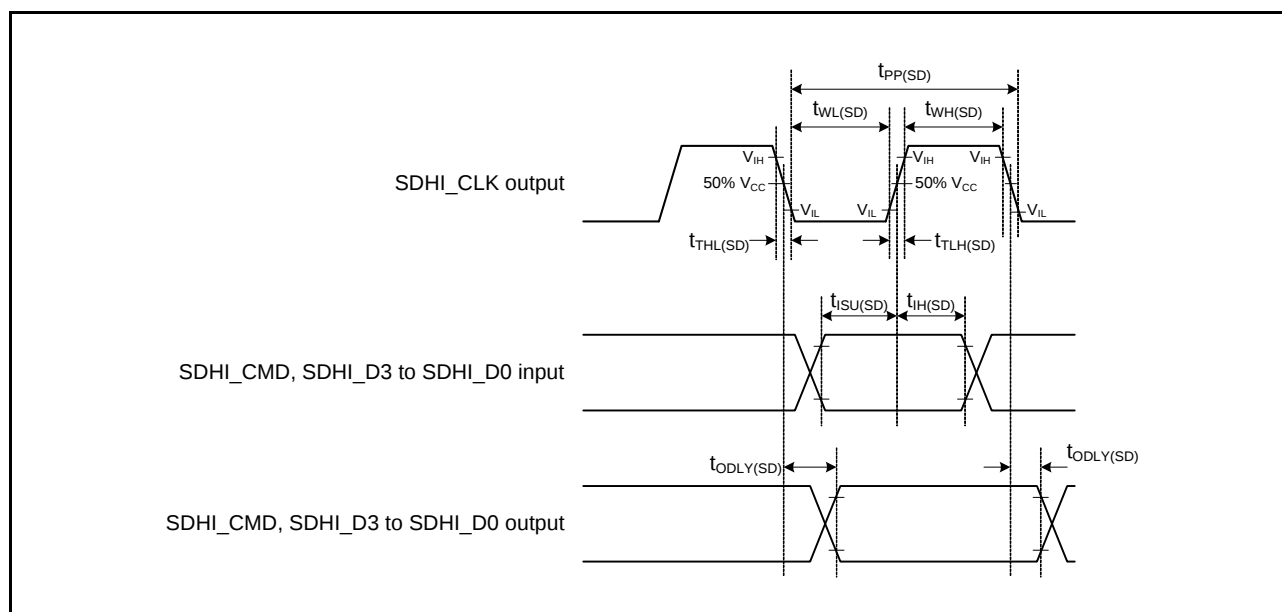
Figure 2.88 SD Host Interface Input/Output Signal Timing
