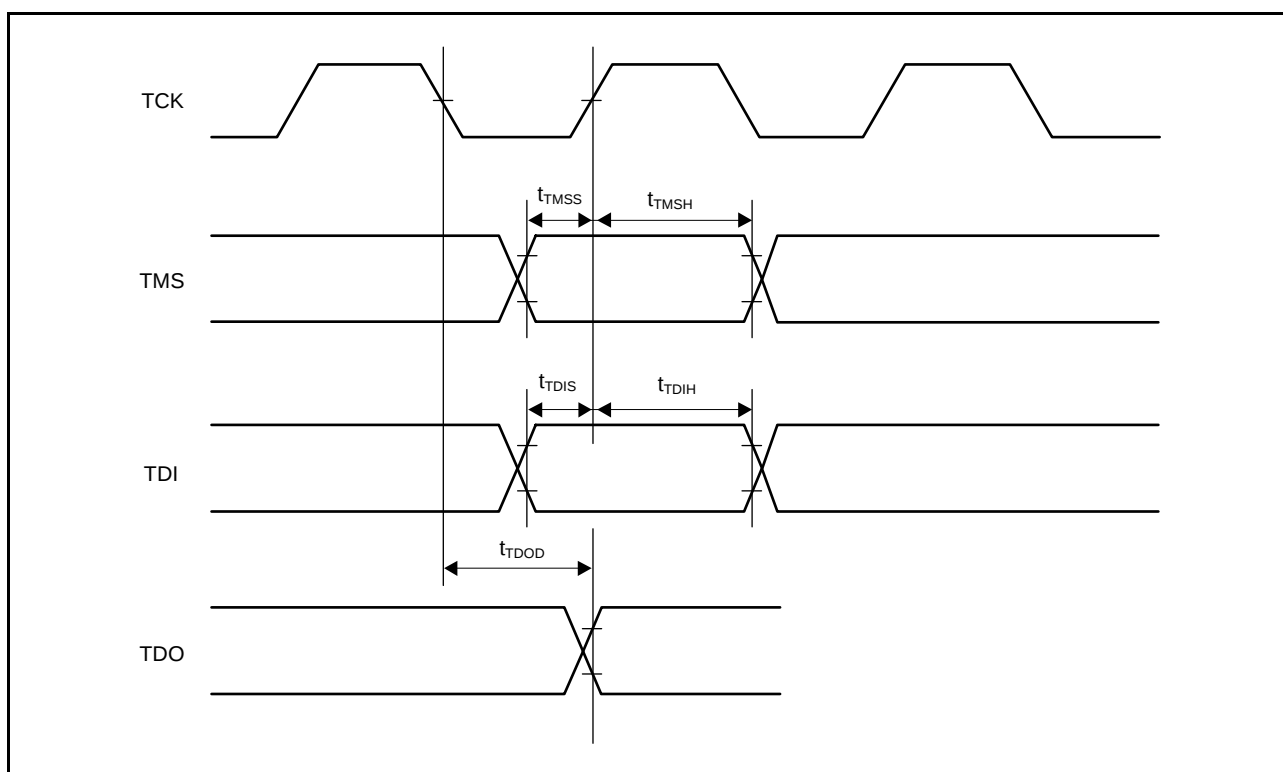
Figure 2.104 Boundary Scan Input/Output Timing
