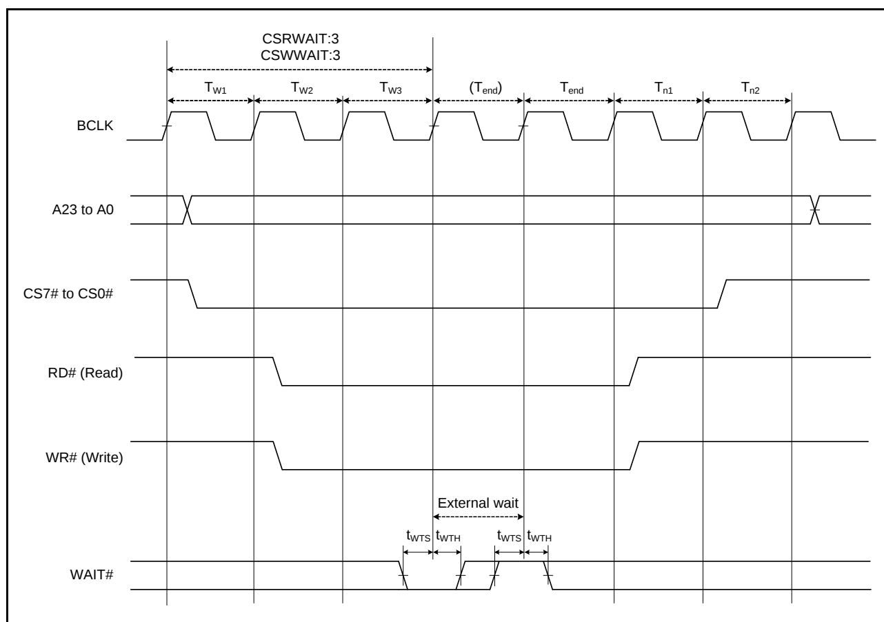
Figure 2.23 External Bus Timing/External Wait Control
