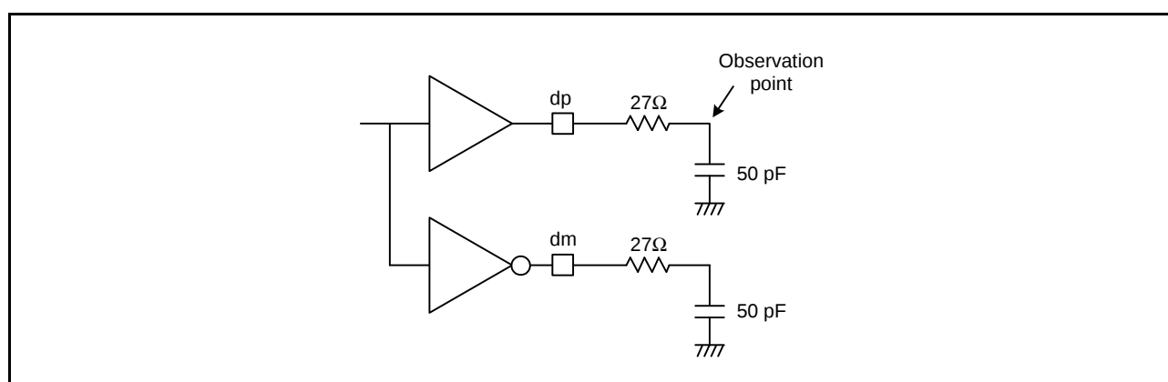
Figure 2.92 Test Circuit (Full-Speed)
