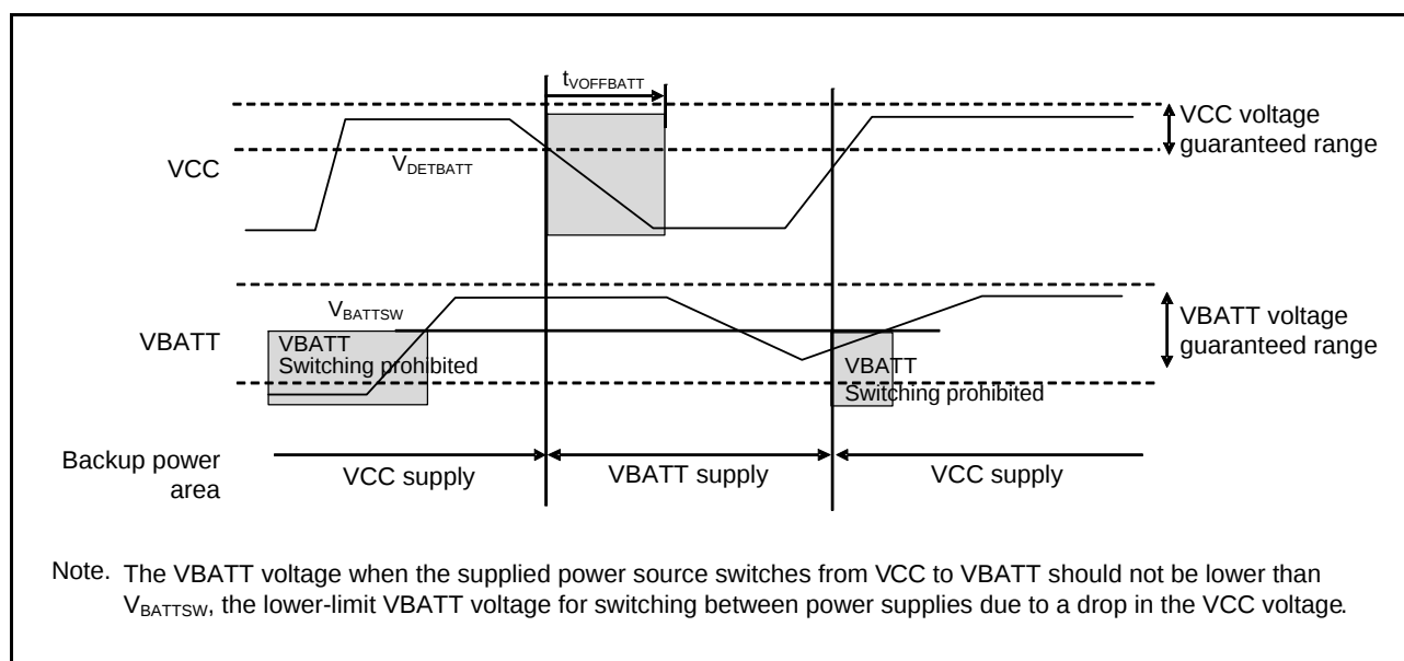
Figure 2.98 Battery Backup Function Characteristics
