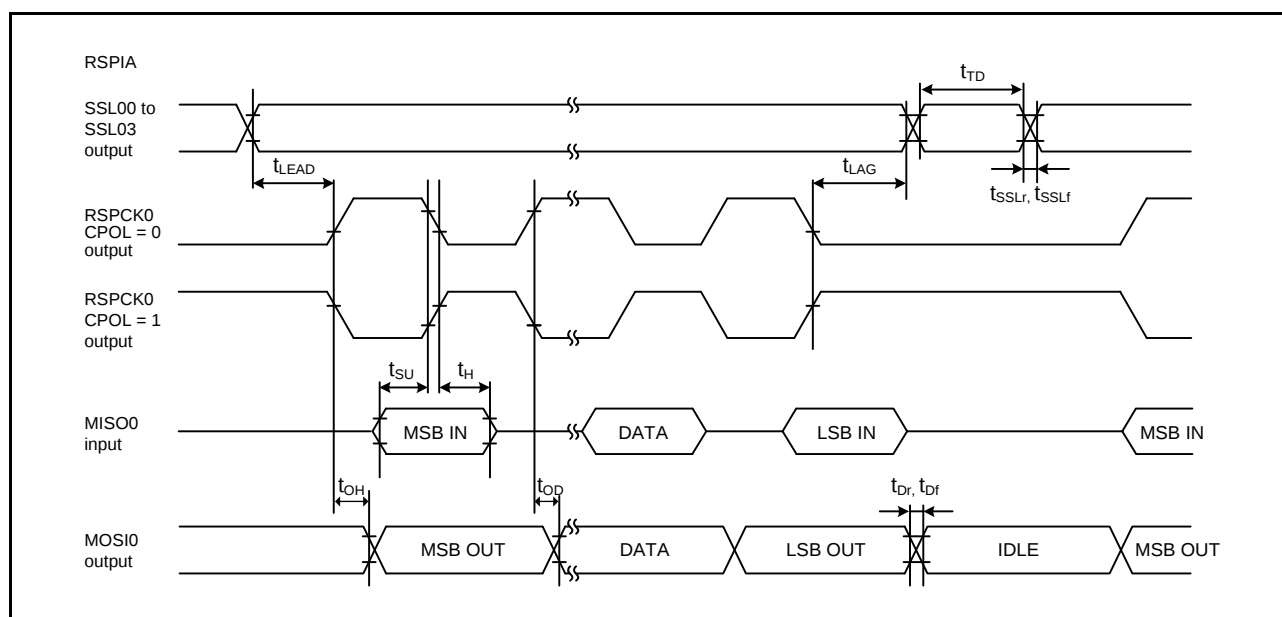
Figure 2.77 RSPIA Timing (Master, Motorola SPI, CPHA = 1)
