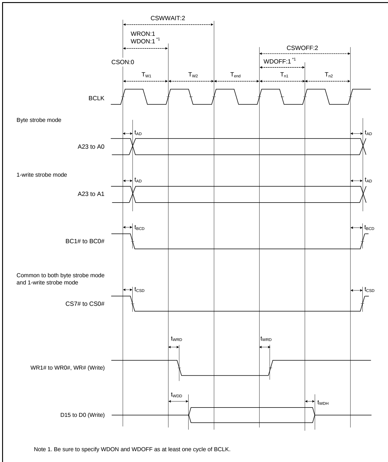
Figure 2.20 External Bus Timing/Normal Write Cycle (Bus Clock Synchronized)
