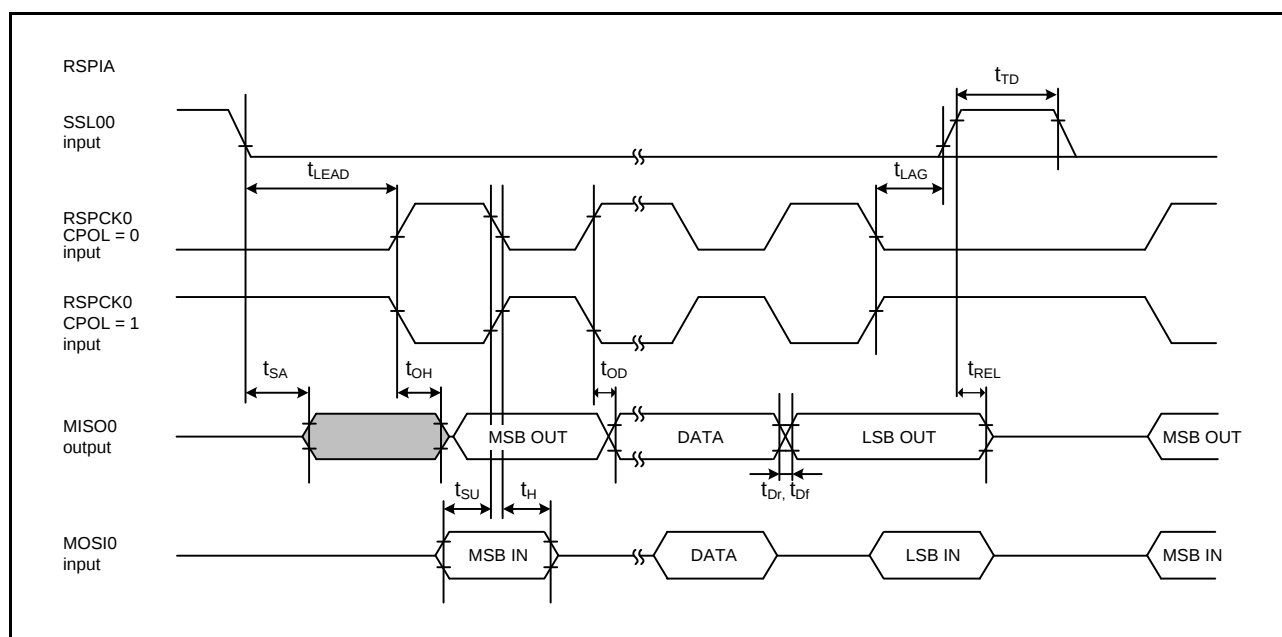
Figure 2.80 RSPIA Timing (Slave, Motorola SPI, CPHA = 1)
