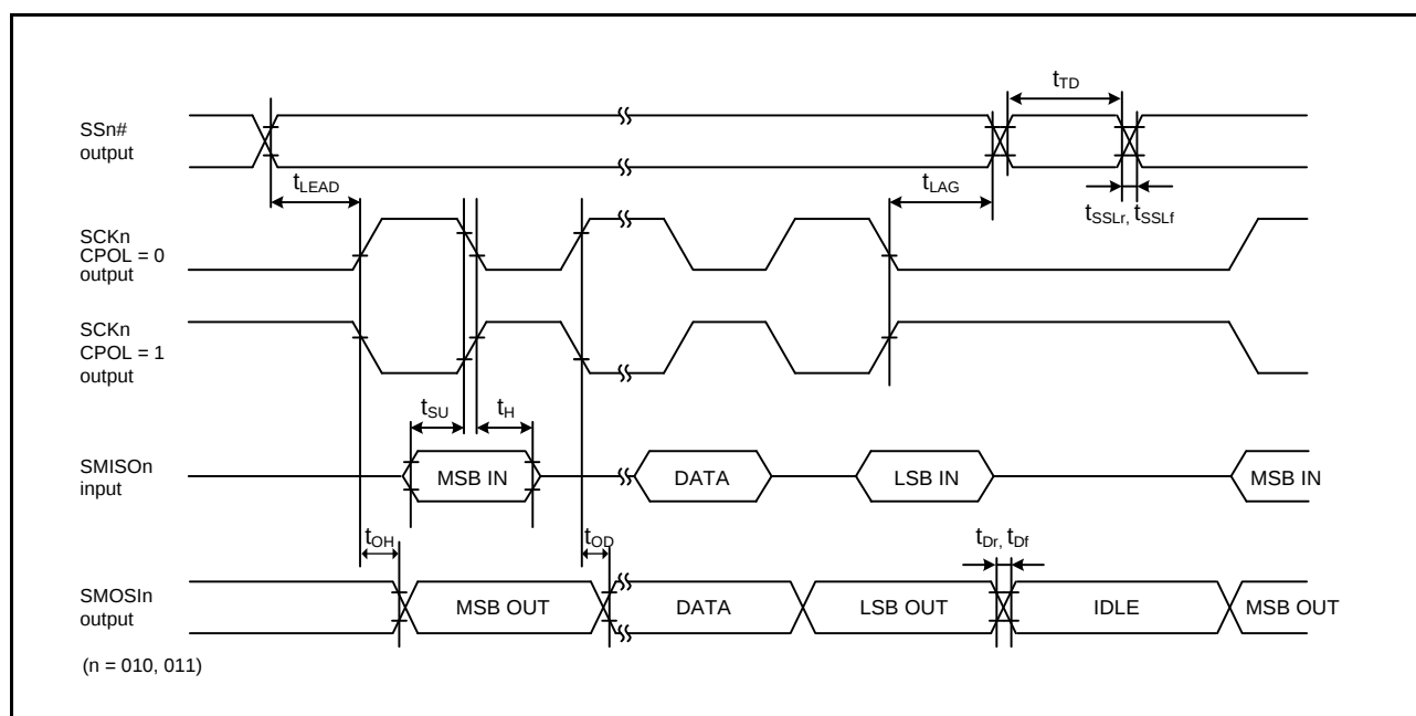
Figure 2.60 Simple SPI Timing (Master, CPHA = 1)
