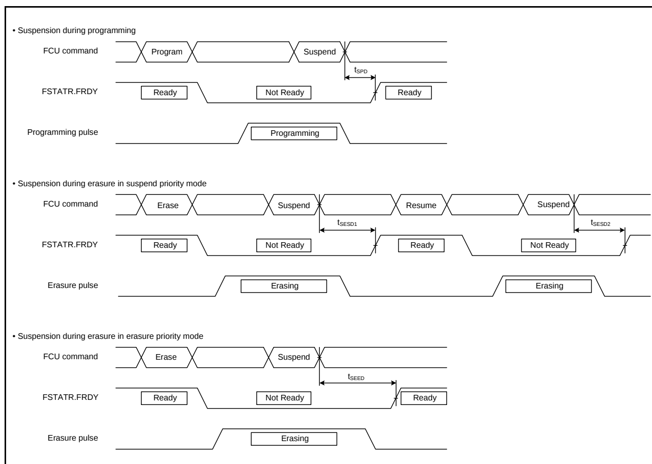
Figure 2.101 Flash Memory Programming/Erase Suspension Timing
