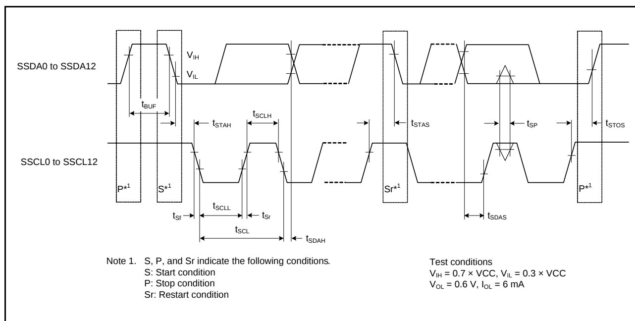
Figure 2.49 Simple IIC Bus Interface Input/Output Timing
