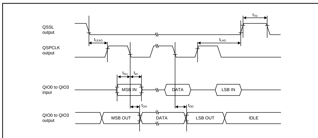
Figure 2.84 Transmit/Receive Timing
