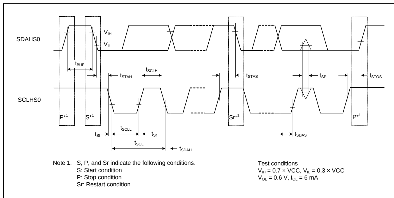
Figure 2.86 RII/CHS Bus Interface Input/Output Timing
