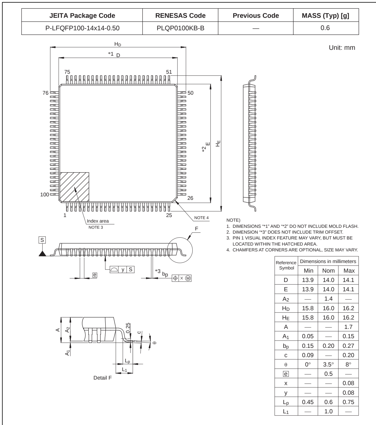
Figure E 100-Pin LFQFP (PLQP0100KB-B)
