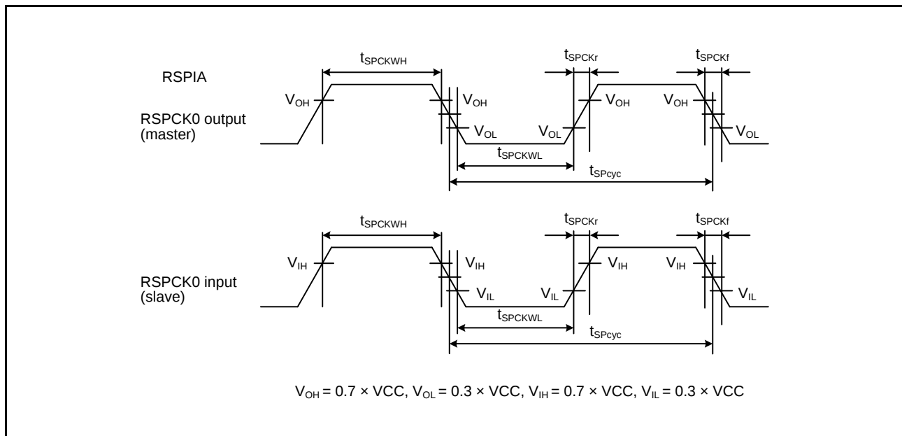
Figure 2.75 RSPIA Clock Timing
