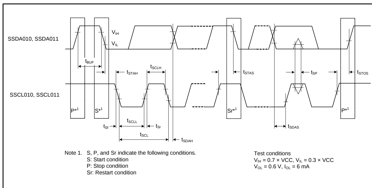
Figure 2.57 Simple IIC Bus Interface Input/Output Timing
