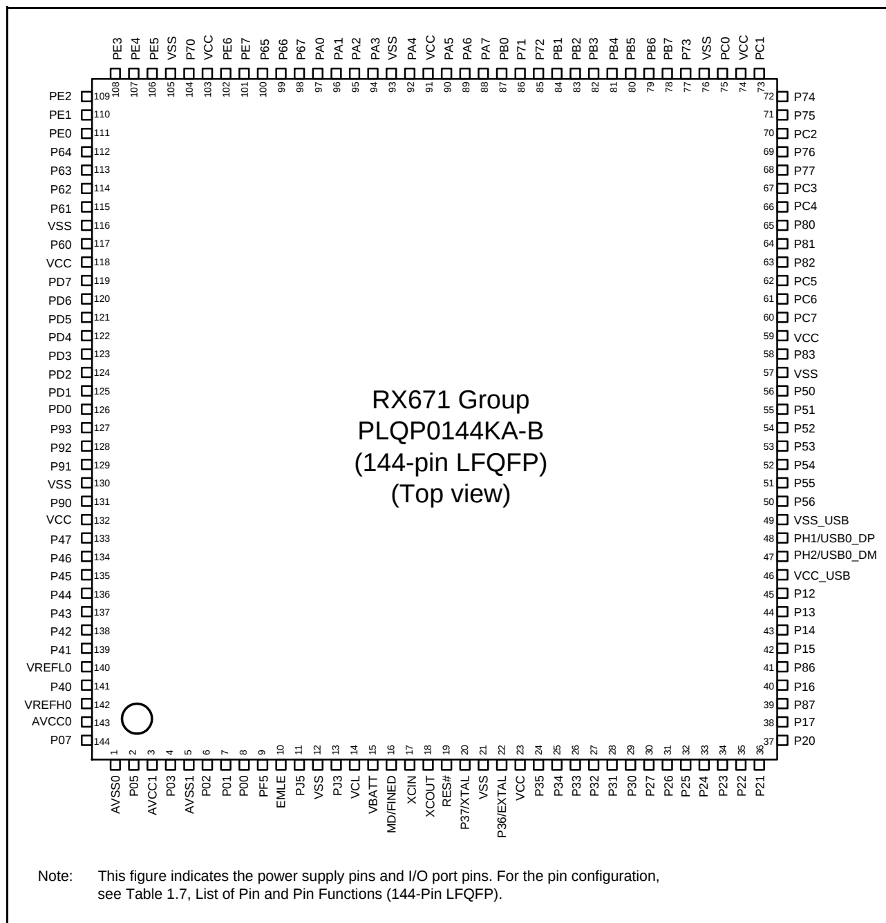
Figure 1.5 Pin Assignment (144-Pin LFQFP)
