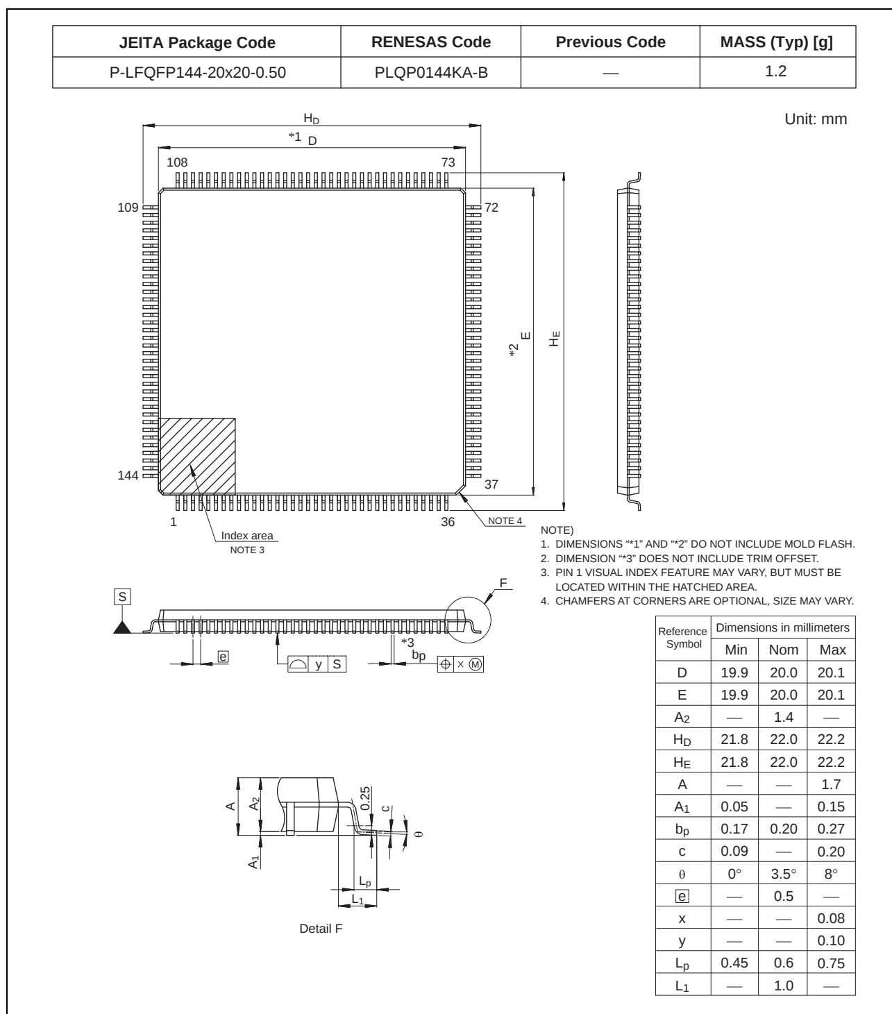
Figure C 144-Pin LFQFP (PLQP0144KA-B)
