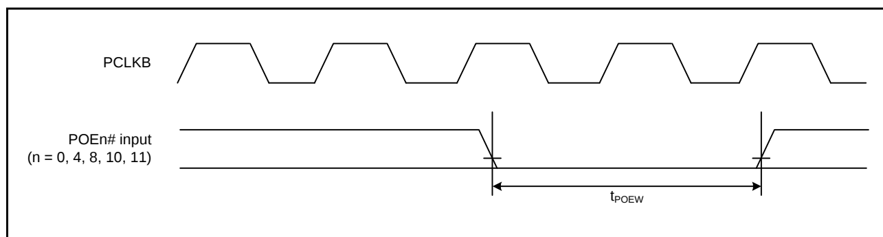
Figure 2.41 POE# Pin Input Timing
