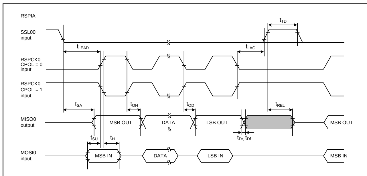
Figure 2.79 RSPIA Timing (Slave, Motorola SPI, CPHA = 0)
