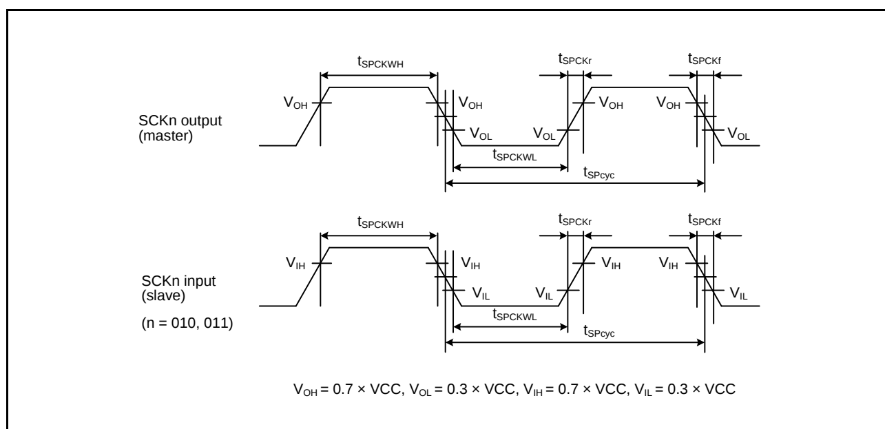
Figure 2.58 Simple SPI Clock Timing
