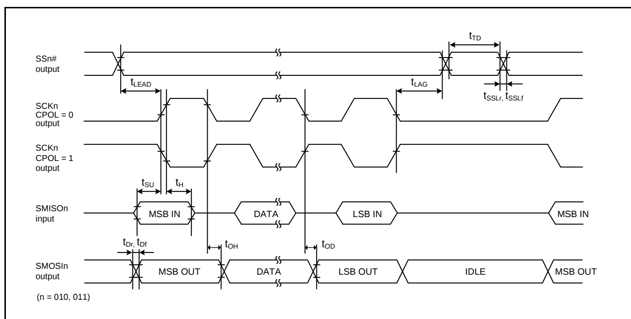
Figure 2.59 Simple SPI Timing (Master, CPHA = 0)
