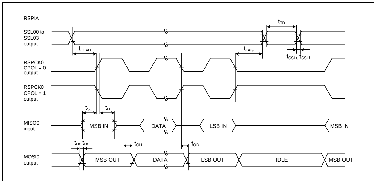
Figure 2.76 RSPIA Timing (Master, Motorola SPI, CPHA = 0)
