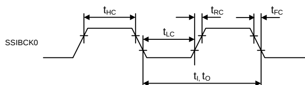
Figure 2.64 SSIE Clock Input/Output Timing
