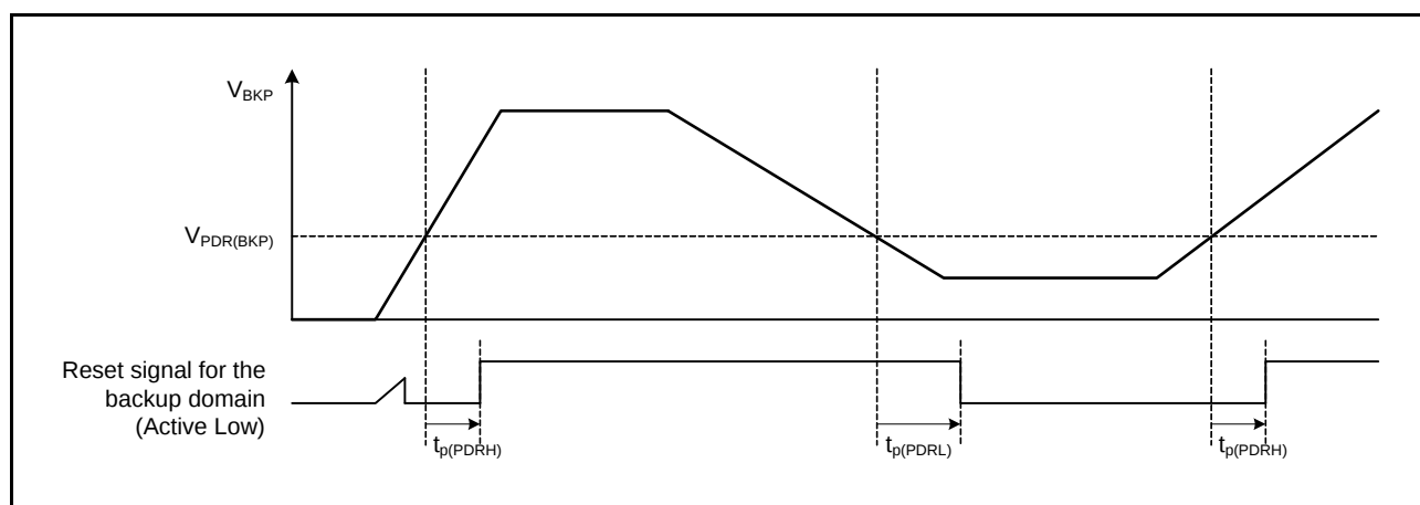
Figure 2.99 Backup Domain Reset Characteristics
