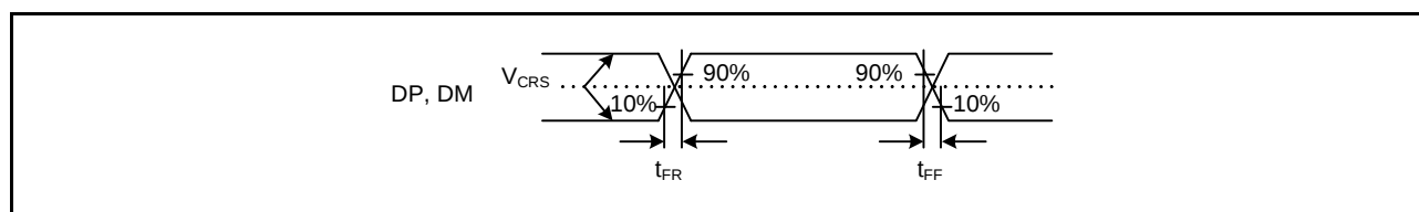
Figure 2.91 DP and DM Output Timing (Full-Speed)
