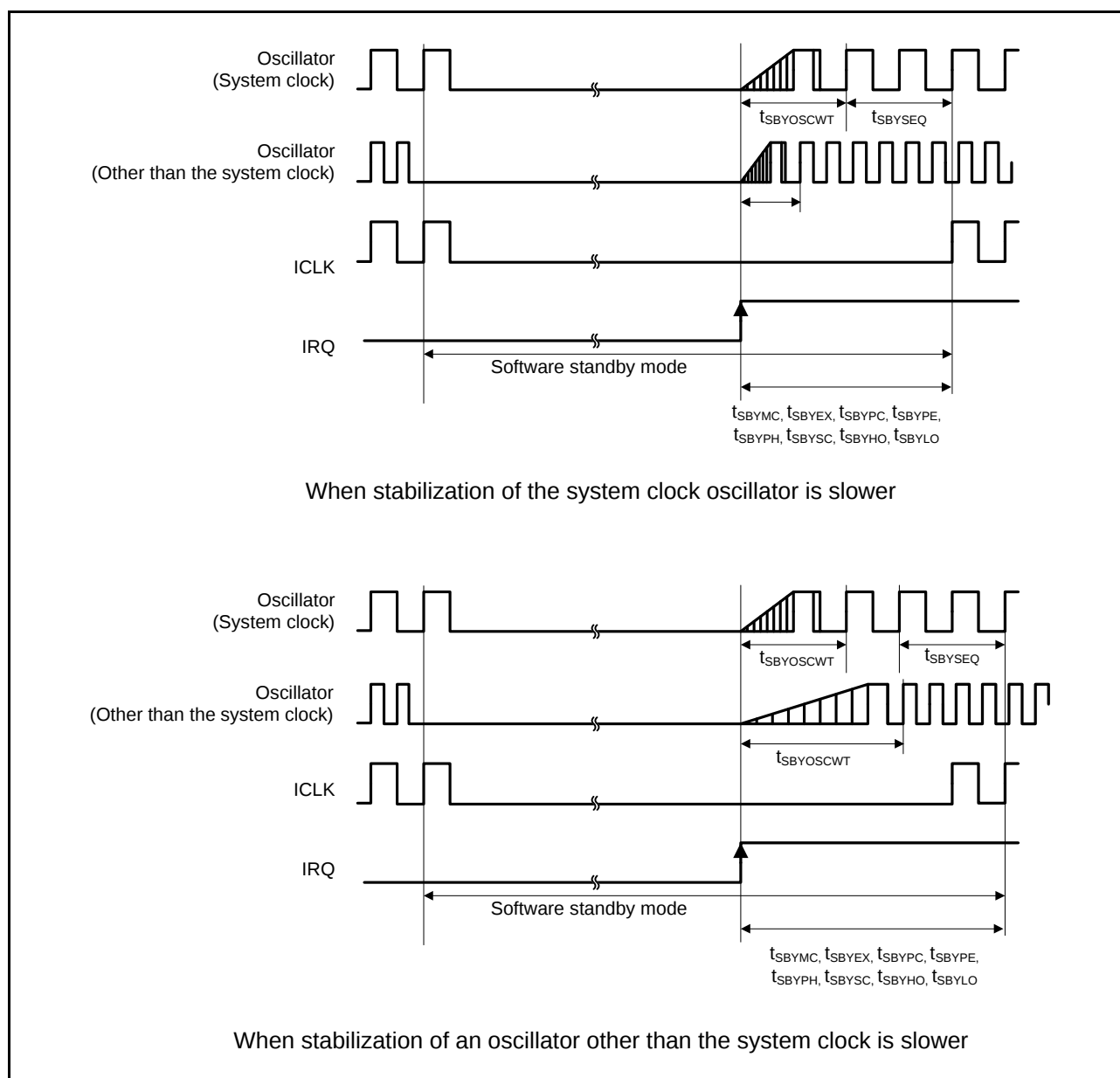
Figure 2.13 Software Standby Mode Recovery Timing
