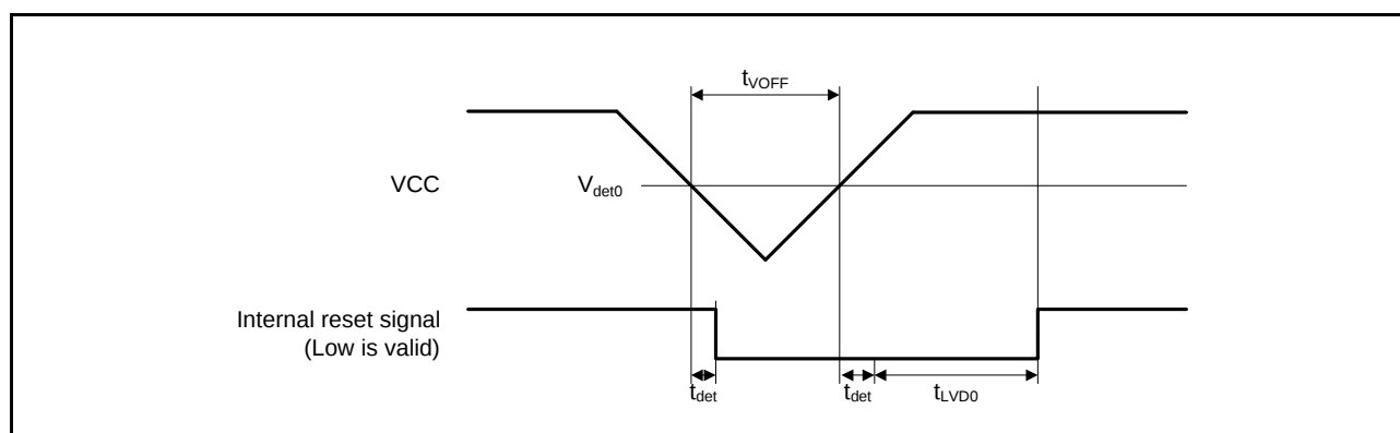
Figure 2.94 Voltage Detection Circuit Timing (V det0 )
