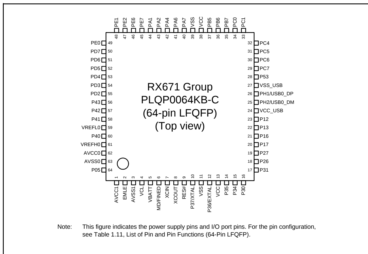
Figure 1.9 Pin Assignment (64-Pin LFQFP)
