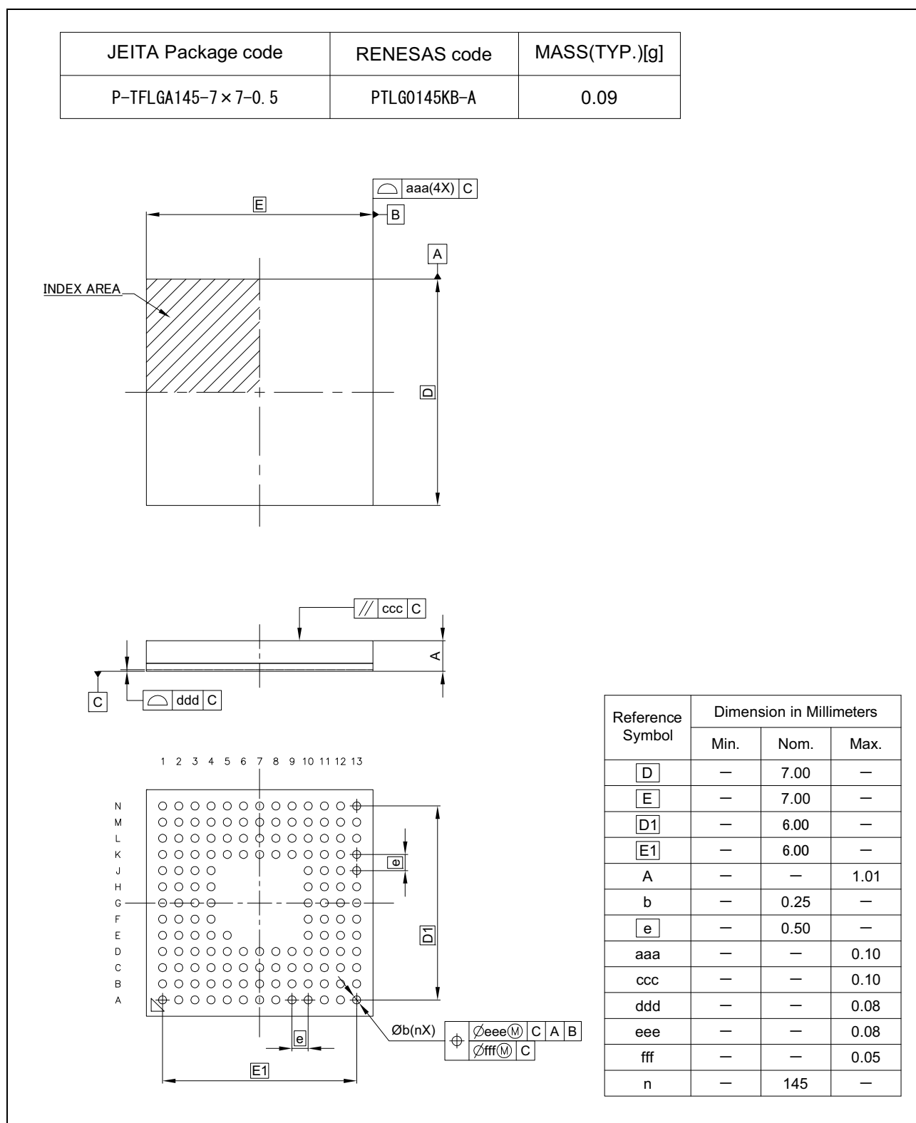
Figure B 145-Pin TFLGA (PTLG0145KB-A)
