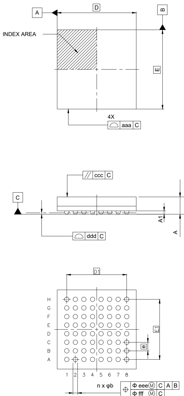
Figure 2.4 BGA 64-pin
