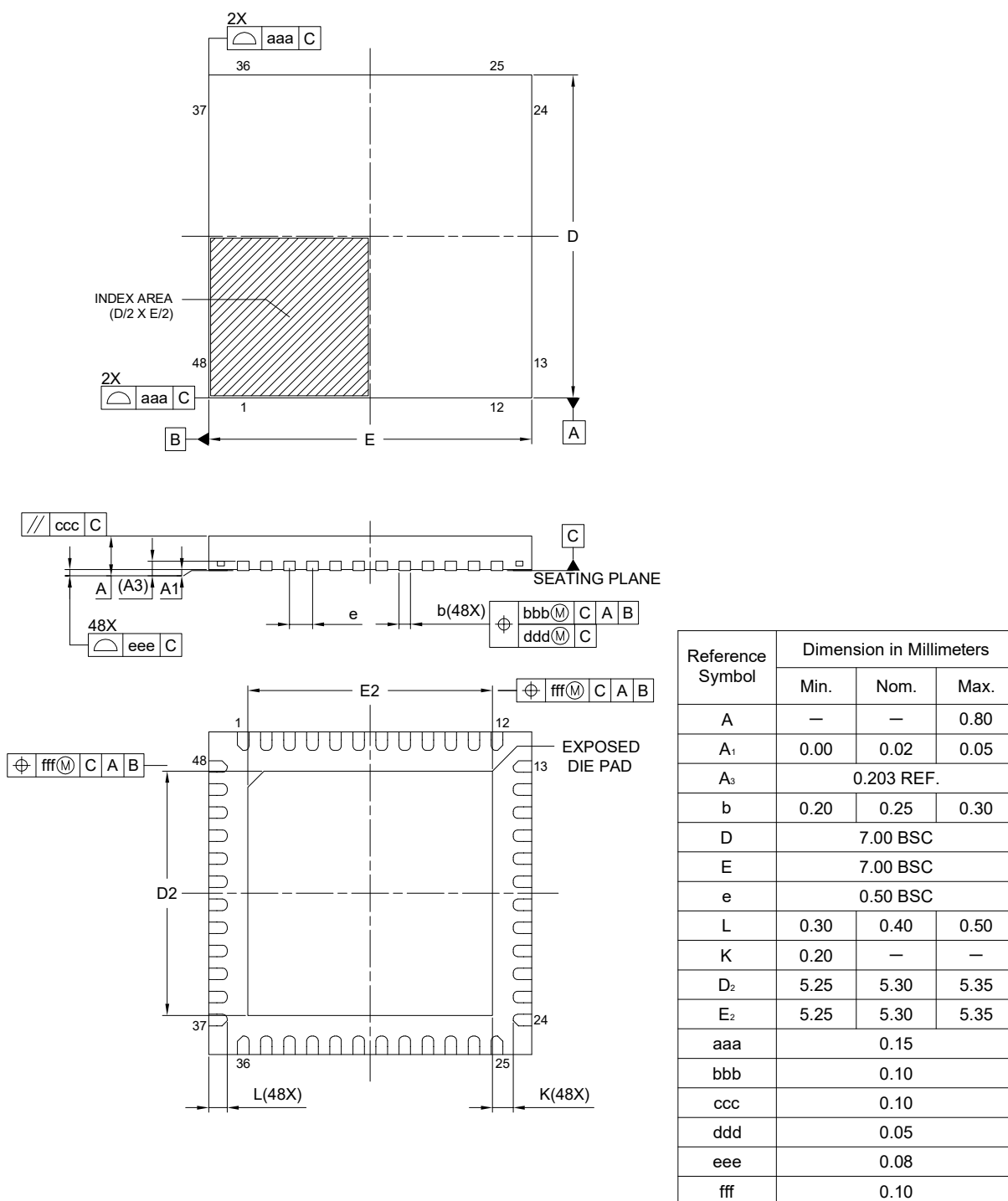
Figure 2.4 QFN 48-pin
