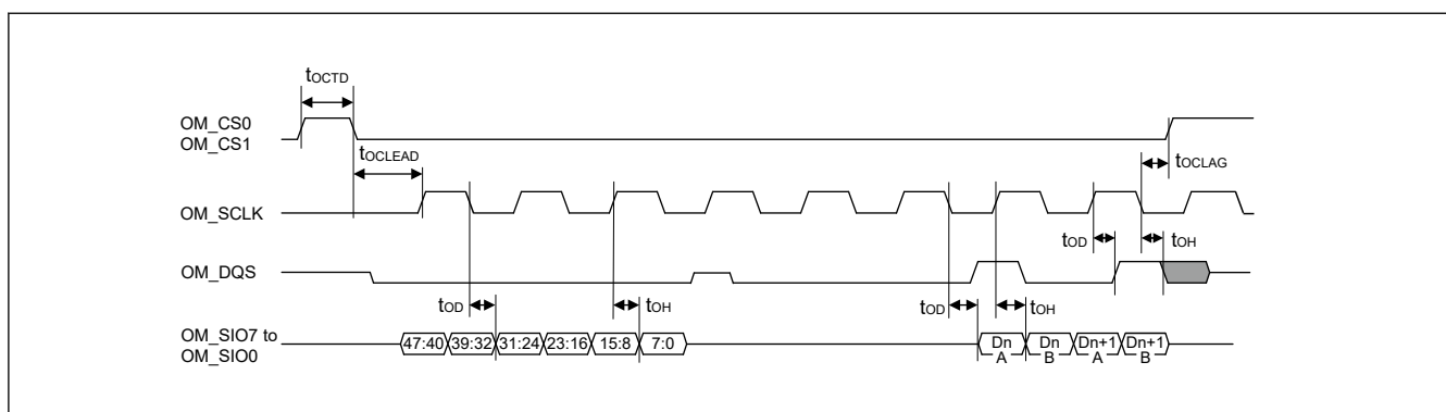
Figure 2.55 DOPI Transfer Format Transmission Timing
