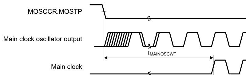
Figure 2.9 Main clock oscillation start timing
