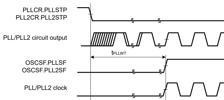
Figure 2.11 PLL/PLL2 clock oscillation start timing
