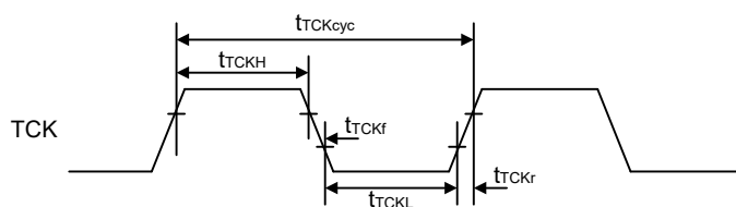
Figure 2.87 Boundary scan TCK timing
