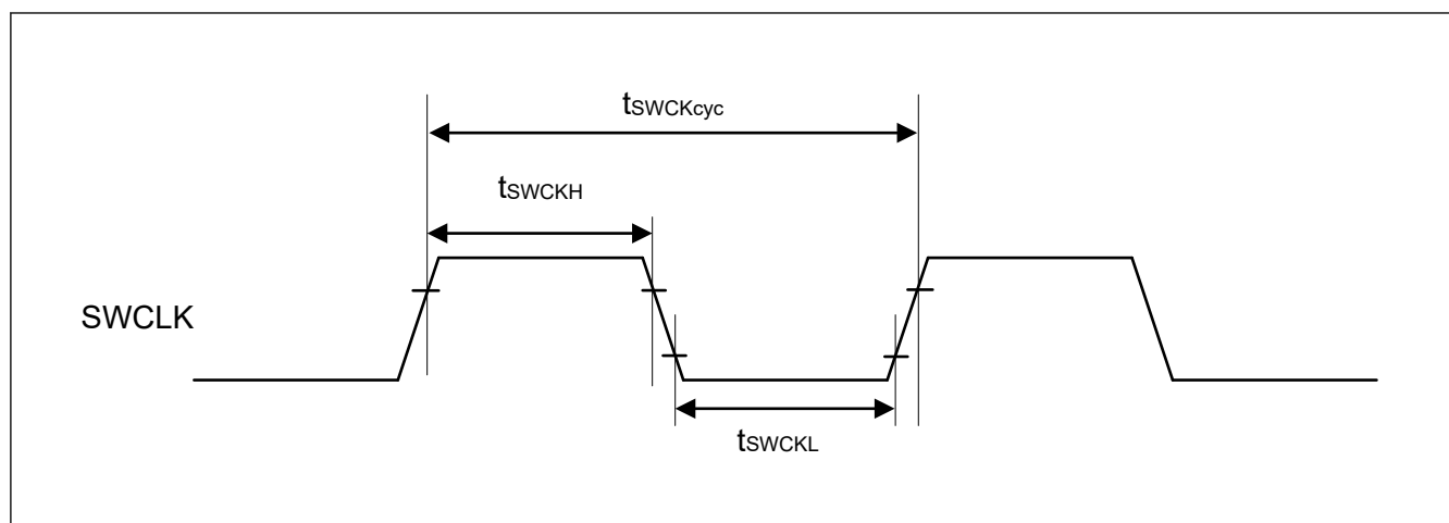
Figure 2.92 SWCLK timing
