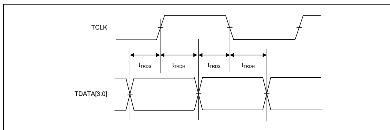
Figure 2.97 ETM output timing
