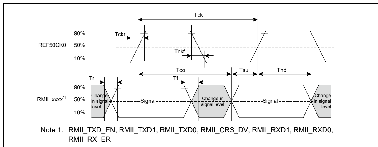
Figure 2.64 REF50CK0 and RMII signal timing
