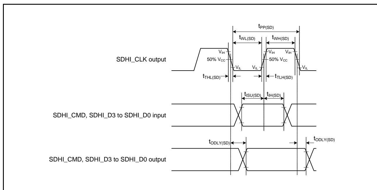
Figure 2.57 SD Host Interface Input/Output Signal Timing
