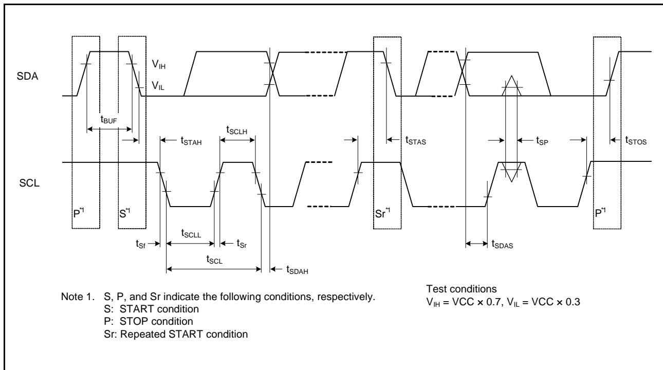
Figure 2.41 I2C Bus Interface Input/Output Timing and Simple I2C Bus Interface Input/Output Timing
