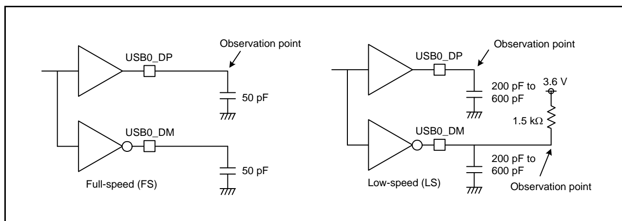
Figure 2.62 Test Circuit
