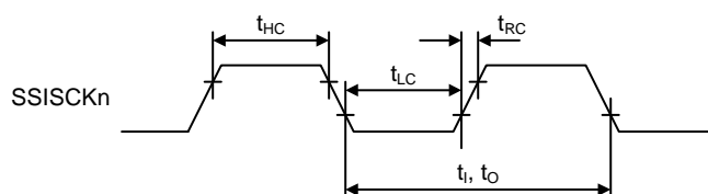
Figure 2.53 SSI Clock Input/Output Timing
