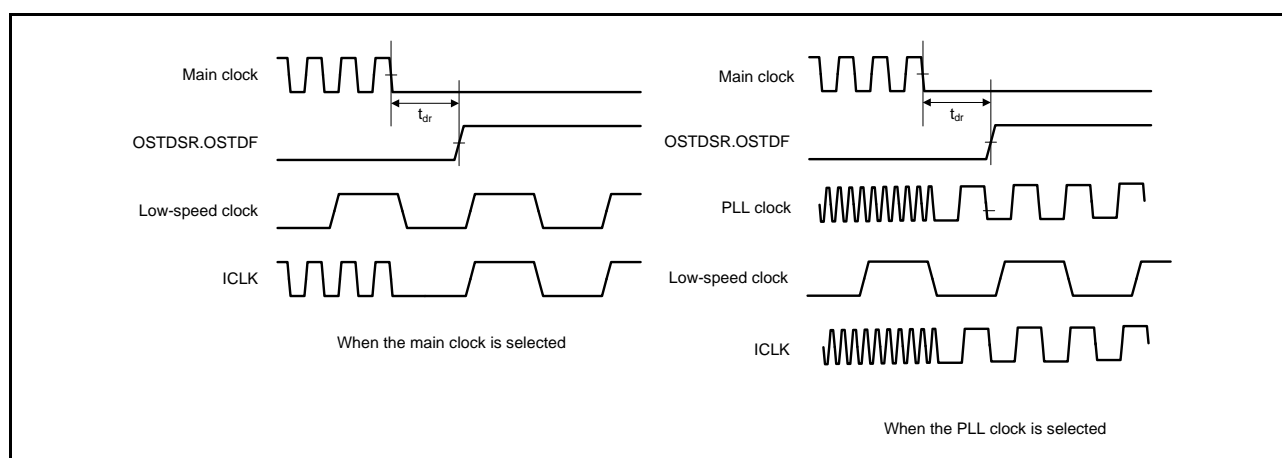
Figure 2.73 Oscillation Stop Detection Timing
