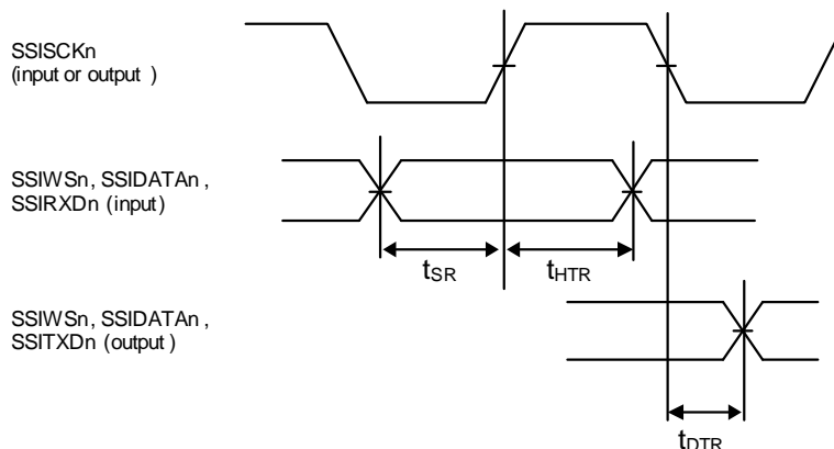
Figure 2.54 SSI Transmission/Reception Timing (SSICR.SCKP = 0)
