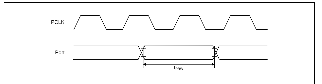
Figure 2.34 I/O Port Input Timing
