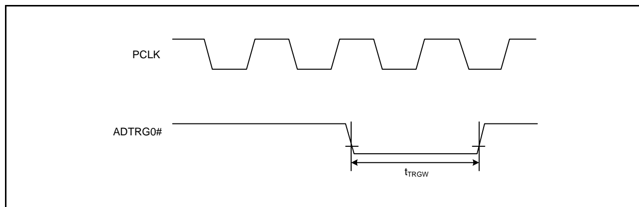
Figure 2.58 A/D Converter External Trigger Input Timing
