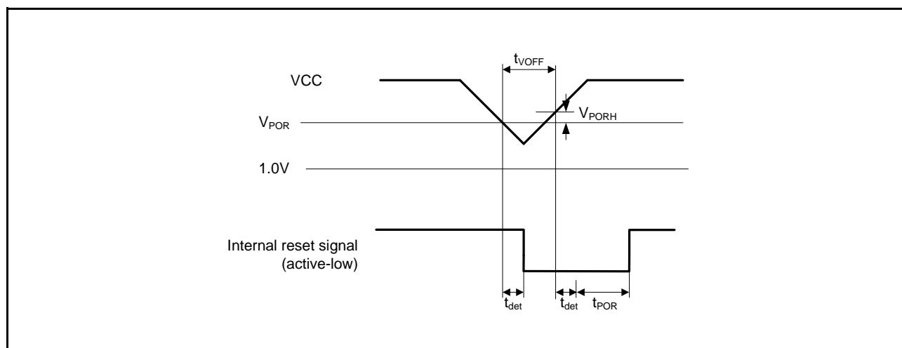
Figure 2.69 Voltage Detection Reset Timing
