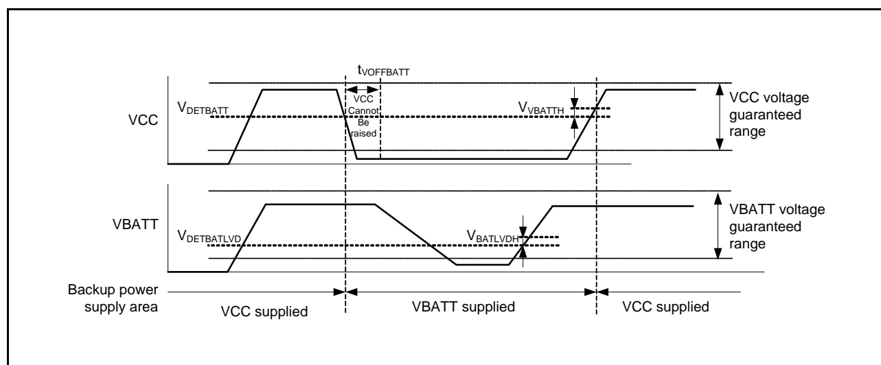
Figure 2.74 Battery Backup Function Characteristics
