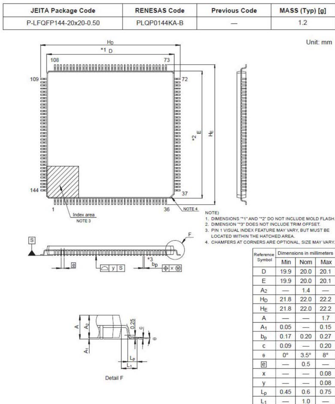
Figure D 144-Pin LFQFP (PLQP0144KA-B)
