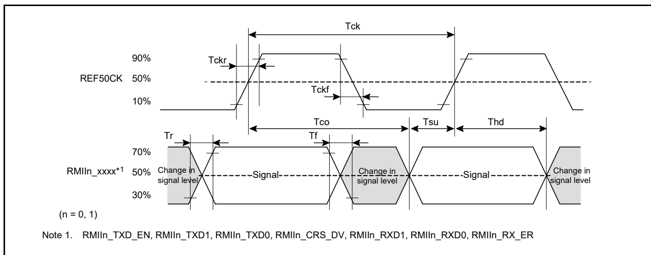
Figure 2.85 Timing with the REF50CK and RMI Signals
