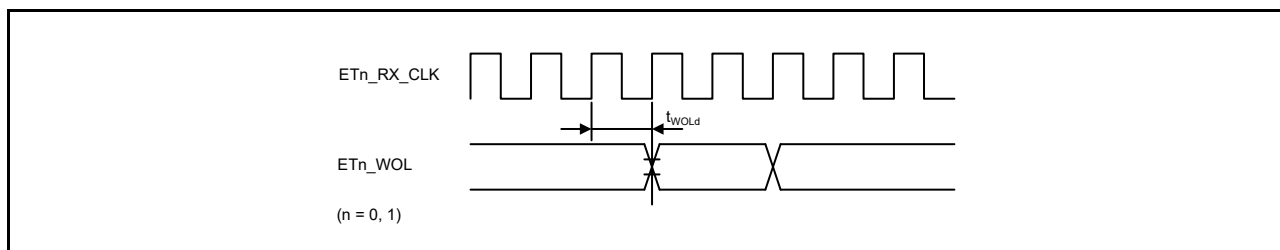
Figure 2.94 WOL Output Timing (MII)
