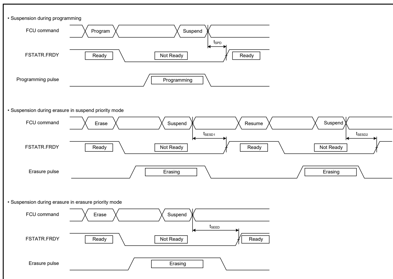
Figure 2.115 Flash Memory Programming/Erasure Suspension Timing
