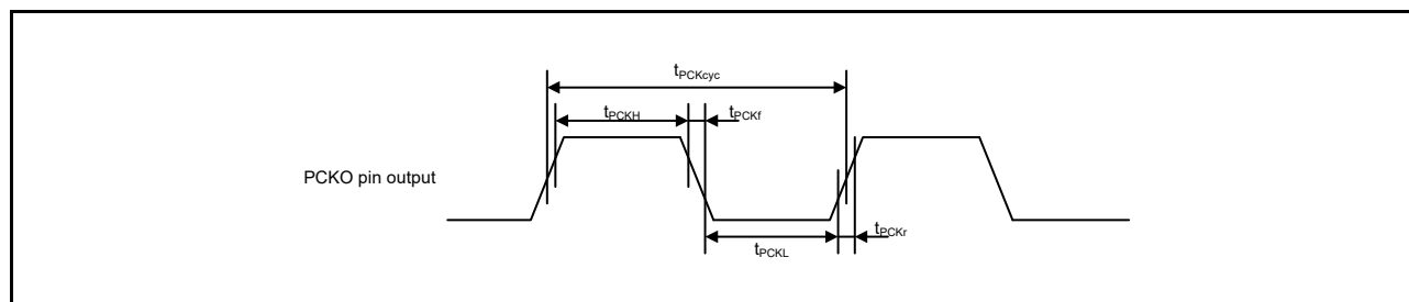
Figure 2.96 PDC Output Clock Timing
