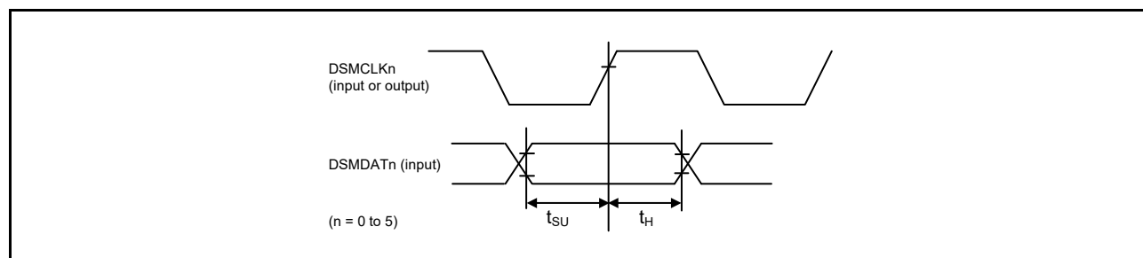
Figure 2.103 Reception Timing (DSMCLKn Rising Synchronous)
