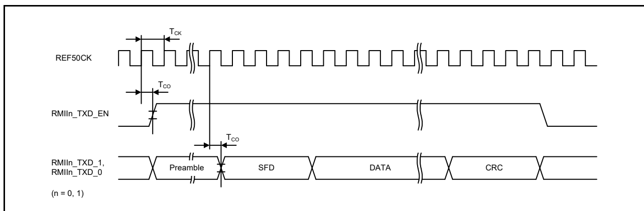
Figure 2.86 RMI Transmission Timing
