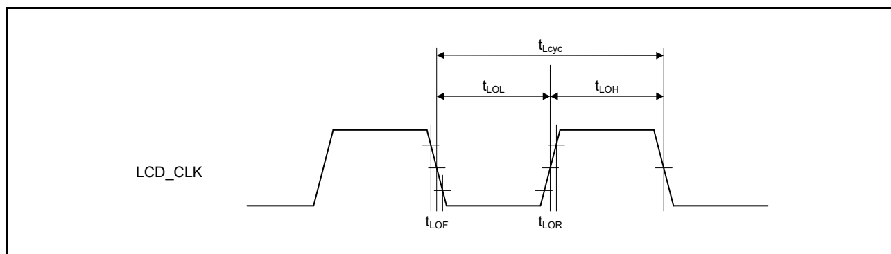
Figure 2.99 LCD_CLK Clock Output Timing
