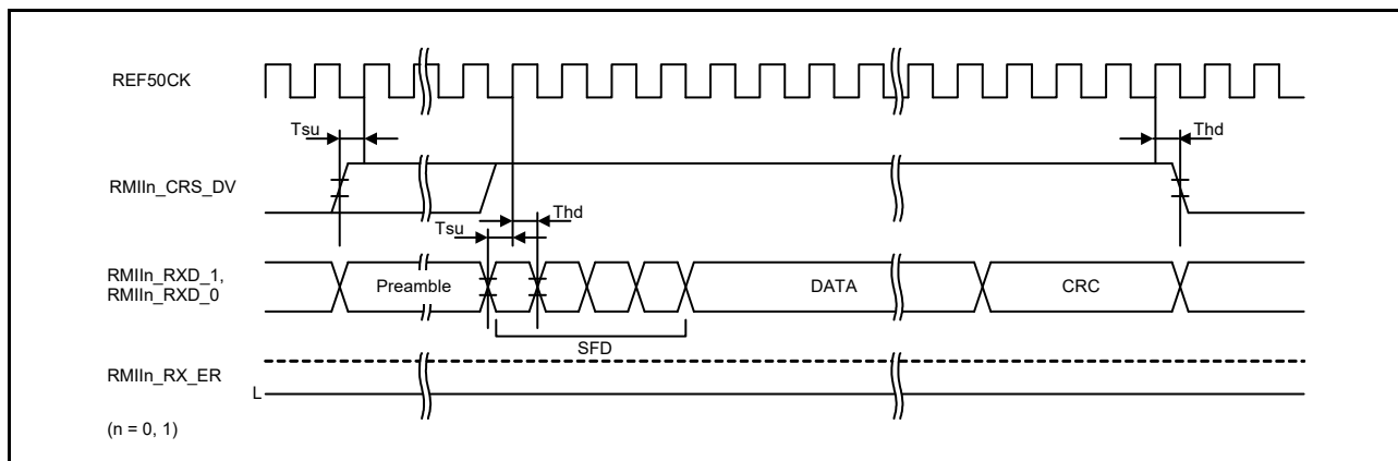
Figure 2.87 RMI Reception Timing (Normal Operation)
