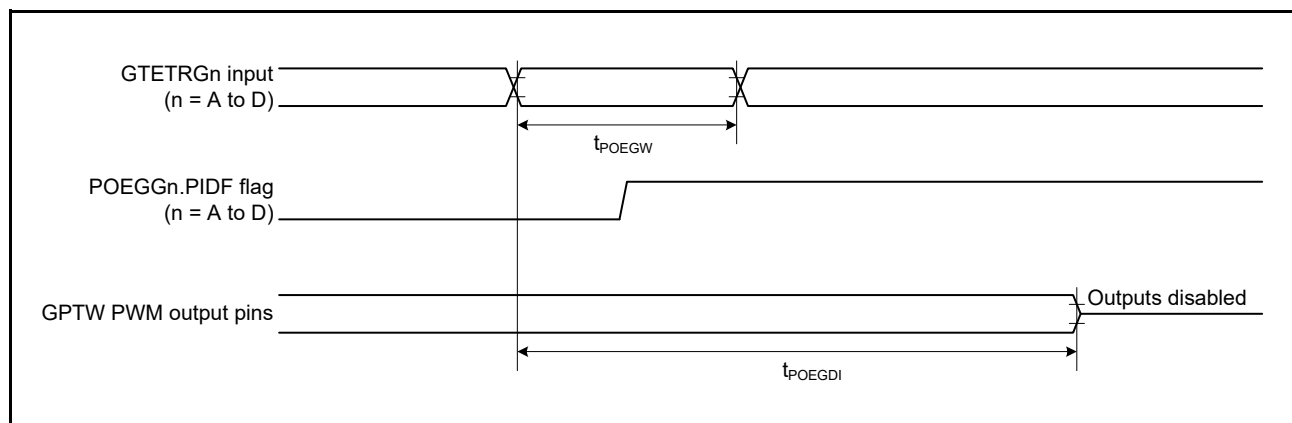
Figure 2.48 Output Disable Time for POEG via Detection Flag in Response to the Input Level Detection of the GTETR Gn pin
