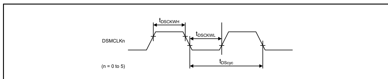
Figure 2.102 Clock Input/Output Timing
