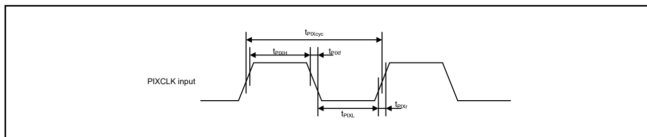
Figure 2.95 PDC Input Clock Timing
