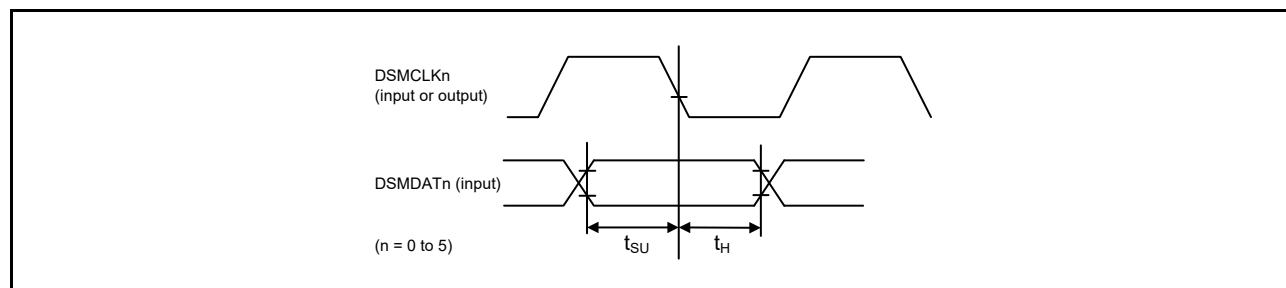
Figure 2.104 Reception Timing (DSMCLKn Falling Synchronous)
