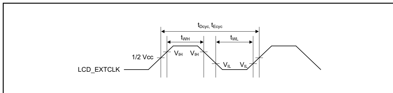
Figure 2.98 LCD_EXTCLK Clock Input Timing
