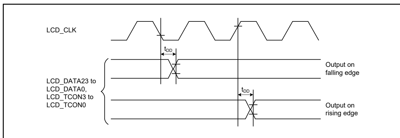
Figure 2.100 LCD Output Data Timing
