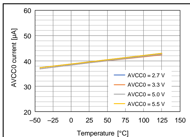
Figure 2.18 Temperature Dependence of Operating Current of Voltage Reference
