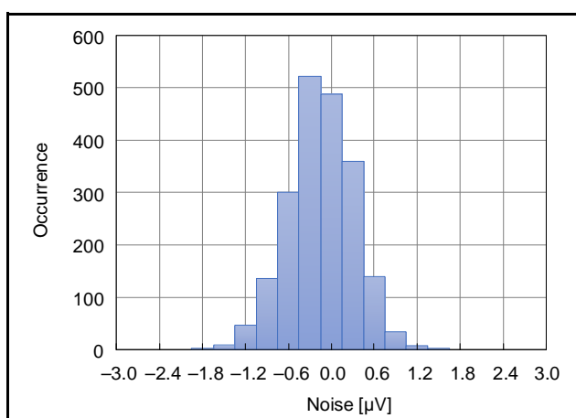
Figure 2.85 Noise Histogram (AVCC0 = 5.0 V, T_a = 25°C, Low Power Mode, Gain = 1 (PGA disabled, BUF disabled), f_{DR} = 1.9 SPS, V_{ID} = 0V, V_{REF} = 2.5V)
