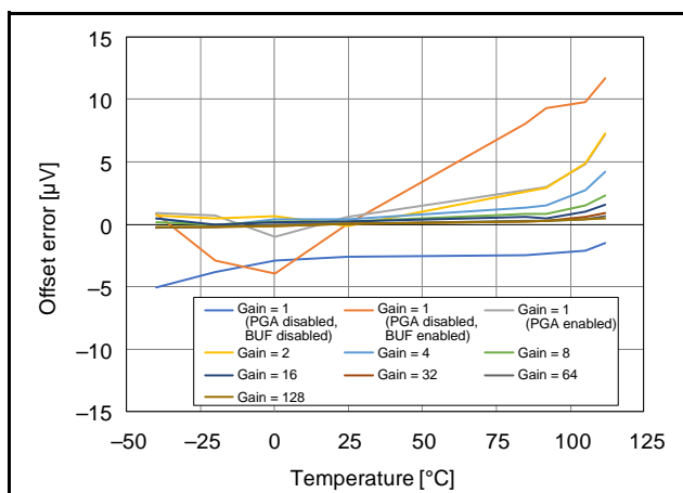
Figure 2.94 Temperature Dependence of Offset Error ( AVCC0 = 5.0\text{ V} , V_{ID} = 0\text{ V} , V_{REF} = 2.5\text{ V} )
