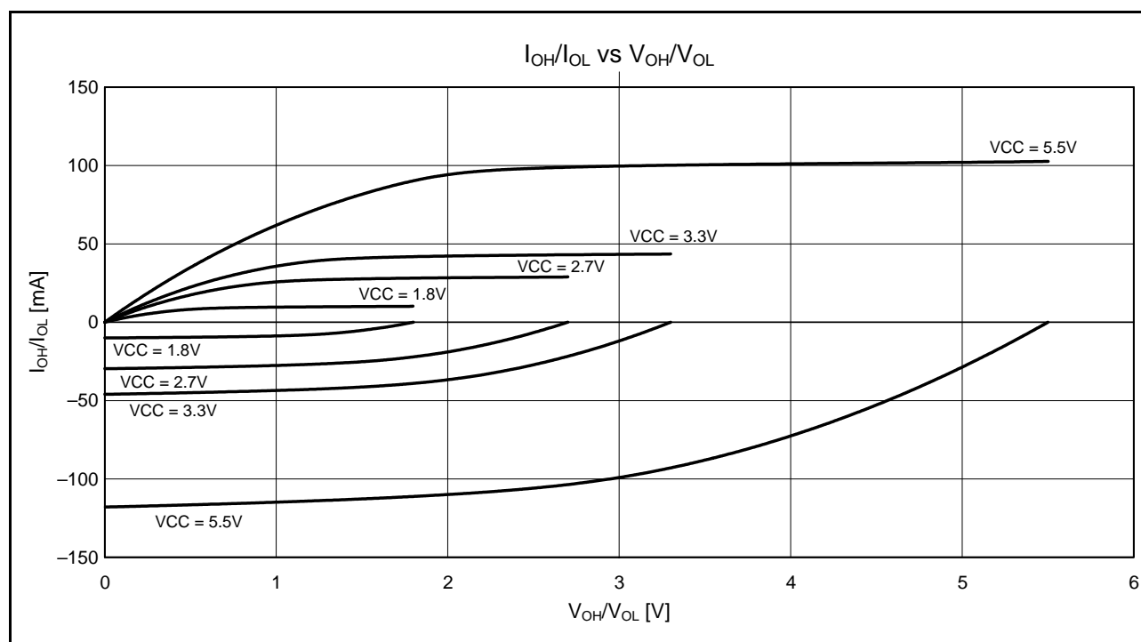
Figure 2.27 V_{OH}/V_{OL} and I_{OH}/I_{OL} Voltage Characteristics at T_a = 25^\circ\text{C} When High-Drive Output is Selected (Reference Data)
