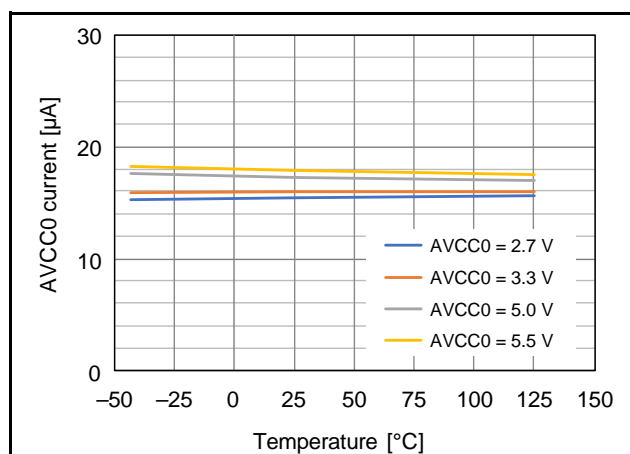
Figure 2.20 Temperature Dependence of Operating Current of Bias Voltage Generator
