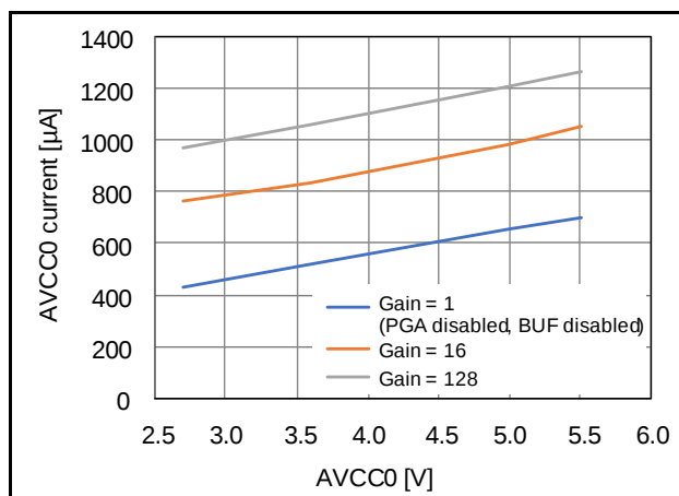
Figure 2.9 Power-Supply Voltage Dependence of Operating Current of 24-Bit Delta-Sigma A/D Converter ( T_a = 25^{\circ}\text{C} , Normal Mode, OPCR.DSADLVM bit = 1)
