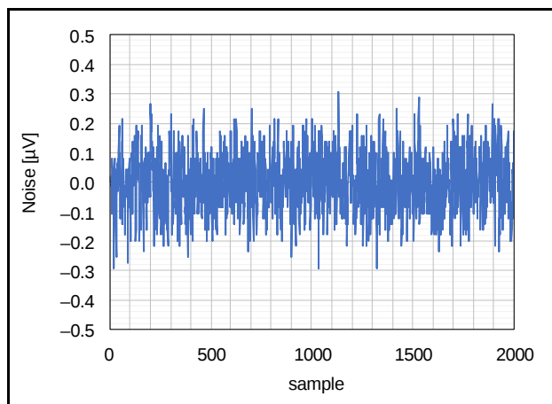
Figure 2.78 Plot of Noise (AVCC0 = 5.0 V, T_a = 25°C, Normal Mode, Gain = 16, f_{DR} = 7.6 SPS, V_{ID} = 0V, V_{REF} = 2.5V)
