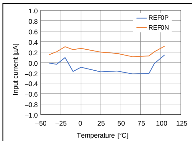
Figure 2.108 Temperature Dependence of External Reference Input Current (AVCC0 = 5.0 V, Reference Buffer Enabled)
