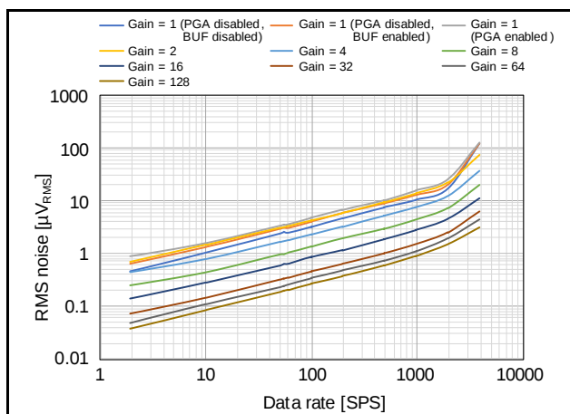
Figure 2.89 Data Rate Dependence of RMS Noise (AVCC0 = 5.0 V, T_a = 25^\circ\text{C} , Low Power Mode, V_{ID} = 0\text{V} , V_{REF} = 2.5\text{V} )
