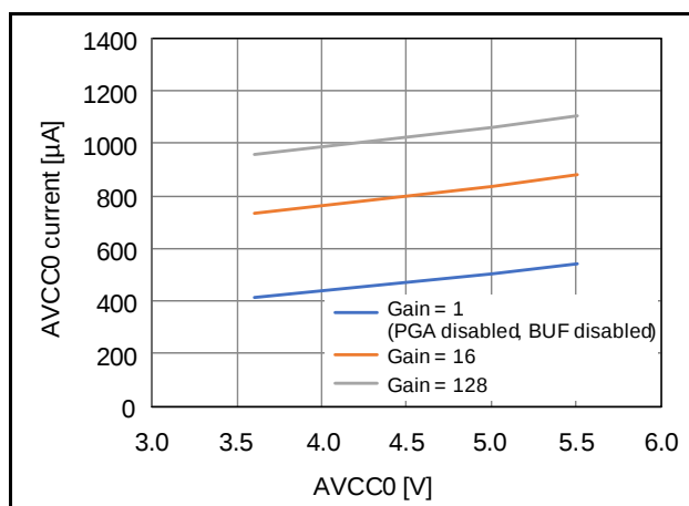
Figure 2.7 Power-Supply Voltage Dependence of Operating Current of 24-Bit Delta-Sigma A/D Converter ( T_a = 25^{\circ}\text{C} , Normal Mode, OPCR.DSADLVM bit = 0)
