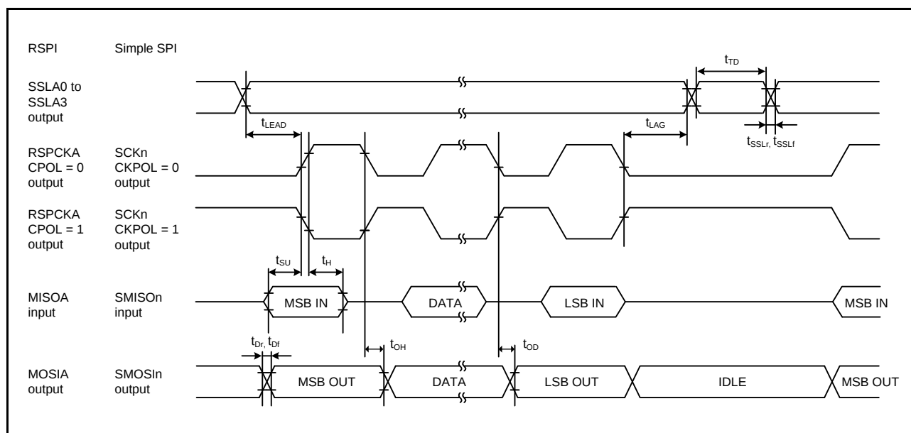
Figure 2.63 RSPI Timing (Master, CPHA = 0) and Simple SPI Clock Timing (Master, CKPH = 1) (n = 1, 5, 6, 12)
