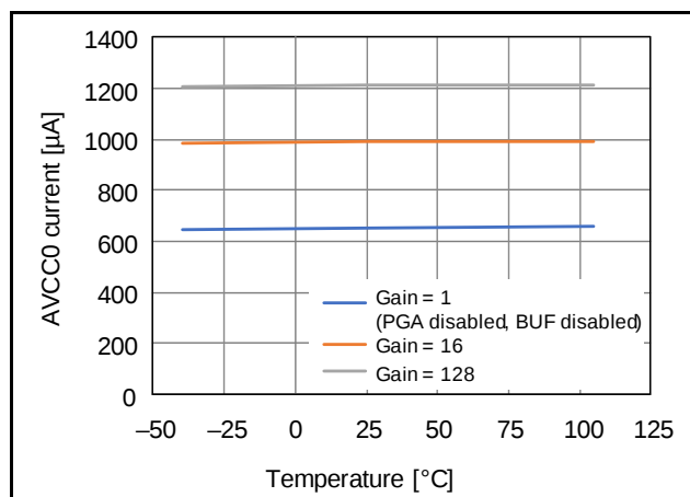
Figure 2.8 Temperature Dependence of Operating Current of 24-Bit Delta-Sigma A/D Converter (AVCC0 = 5.0 V, Normal Mode, OPCR.DSADLVM bit = 1)
