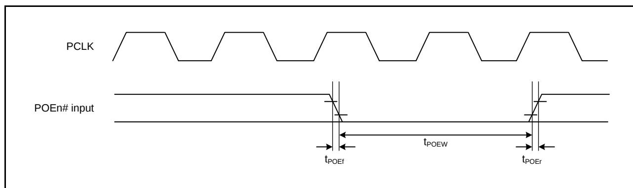
Figure 2.53 POE Input Timing (n = 0 to 3, 8)
