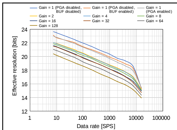
Figure 2.88 Data Rate Dependence of Effective Resolution (AVCC0 = 5.0 V, T_a = 25^\circ\text{C} , Normal Mode, V_{ID} = 0\text{V} , V_{REF} = 2.5\text{V} )
