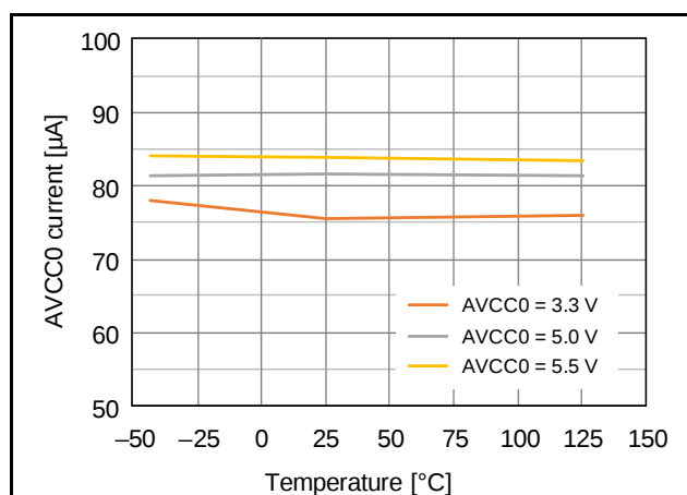
Figure 2.16 Temperature Dependence of Operating Current of Reference Buffer (Normal Mode)
