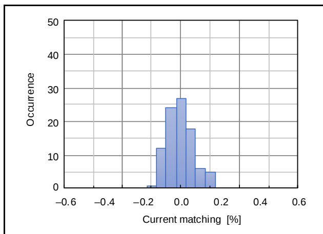
Figure 2.104 Matching of Output Current of Excitation Current Source (AVCC0 = 5.0 V, T_a = 25°C, I EXC = 250 \mu A, 93 samples)
