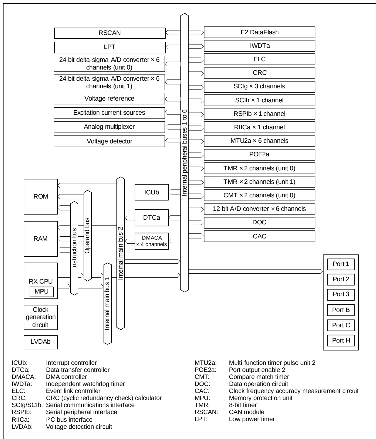
Figure 1.2 Block Diagram
