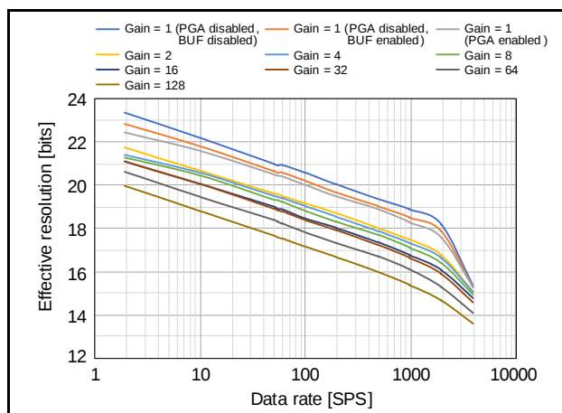
Figure 2.90 Data Rate Dependence of Effective Resolution (AVCC0 = 5.0 V, T_a = 25^\circ\text{C} , Low Power Mode, V_{ID} = 0\text{V} , V_{REF} = 2.5\text{V} )
