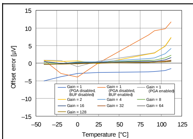
Figure 2.94 Temperature Dependence of Offset Error (AVCC0 = 5.0 V, V_{\text{ID}} = 0\text{V} , V_{\text{REF}} = 2.5\text{V} )
