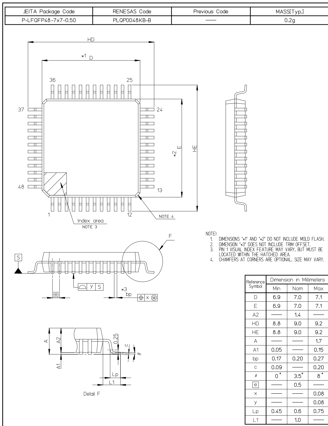
Figure A 48-Pin LFQFP (PLQP0048KB-B)
