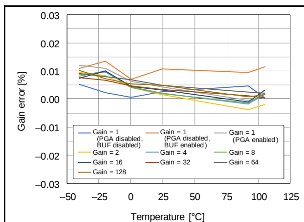
Figure 2.95 Temperature Dependence of Gain Error (AVCC0 = 5.0 V, OPCR.DSADLVM bit = 0, V_{\text{REF}} = 2.5\text{V} )
