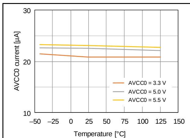
Figure 2.15 Temperature Dependence of Operating Current of Analog Input Buffer (Low Power Mode)
