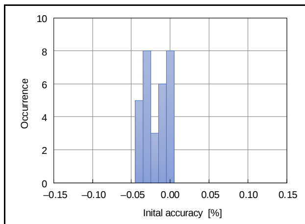
Figure 2.99 Initial Accuracy of Voltage Reference (AVCC0 = 5.0 V, 30 samples)
