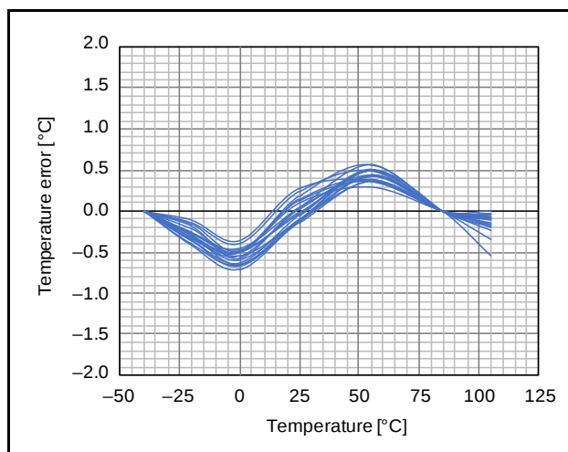
Figure 2.101 Accuracy of Temperature Sensor (AVCC0 = 5.0 V)
