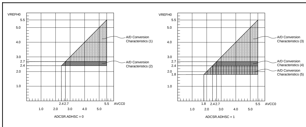
Figure 2.109 AVCC0 to VREFH0 Voltage Range
