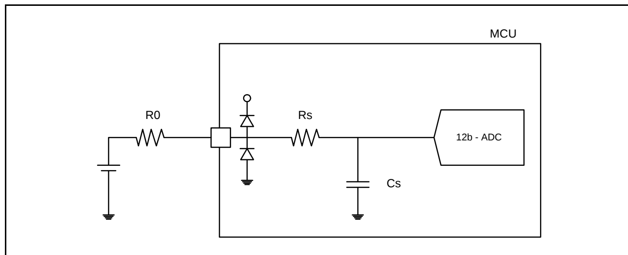
Figure 2.110 Equivalent Circuit
