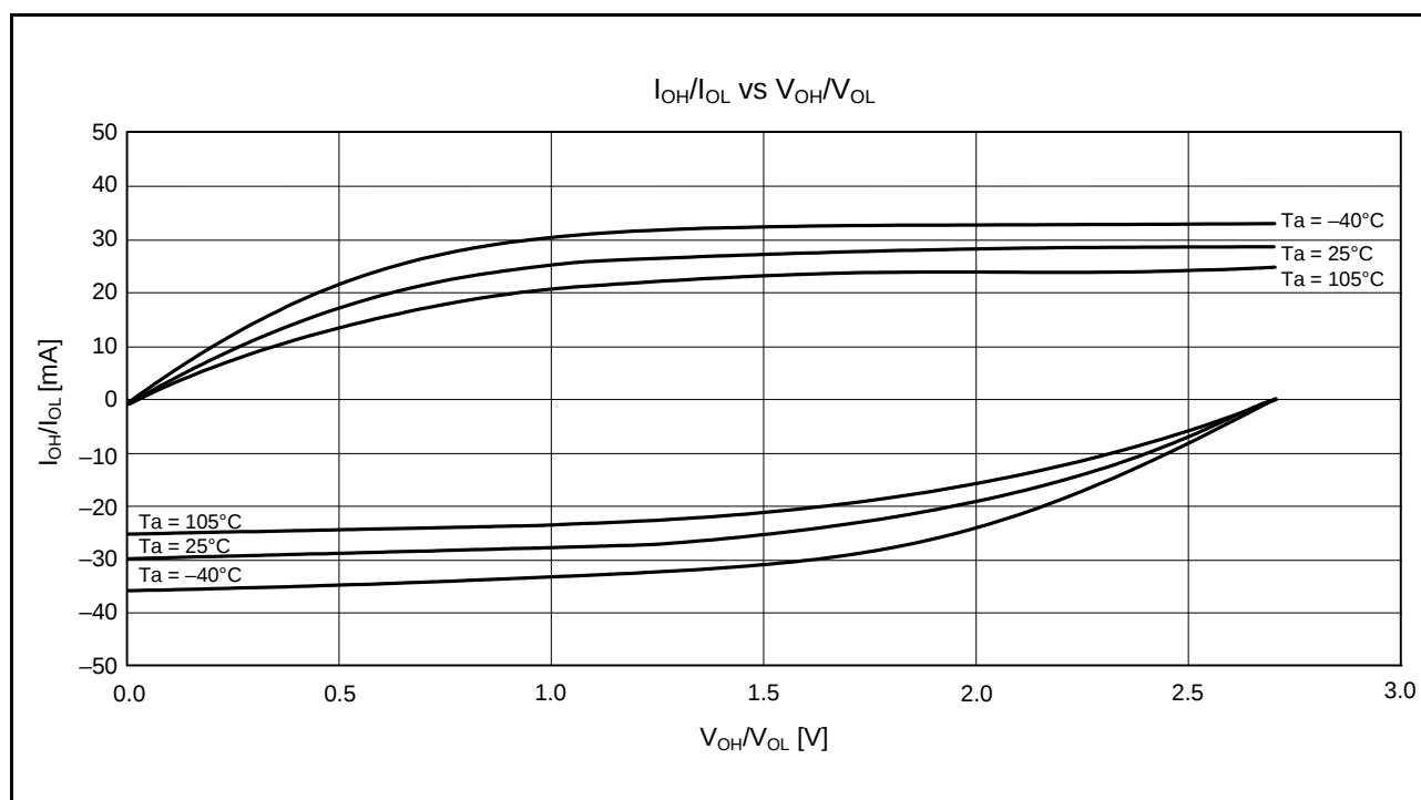
Figure 2.29 V_{OH}/V_{OL} and I_{OH}/I_{OL} Temperature Characteristics at V_{CC} = 2.7 V When High-Drive Output is Selected (Reference Data)
