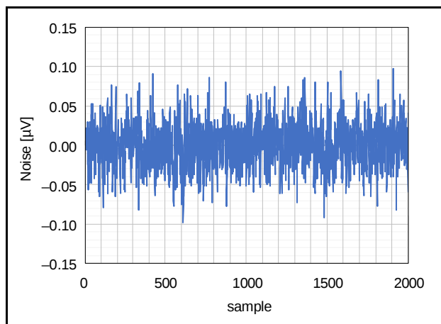
Figure 2.76 Plot of Noise (AVCC0 = 5.0 V, T_a = 25°C, Normal Mode, Gain = 128, f_{DR} = 7.6 SPS, V_{ID} = 0V, V_{REF} = 2.5V)
