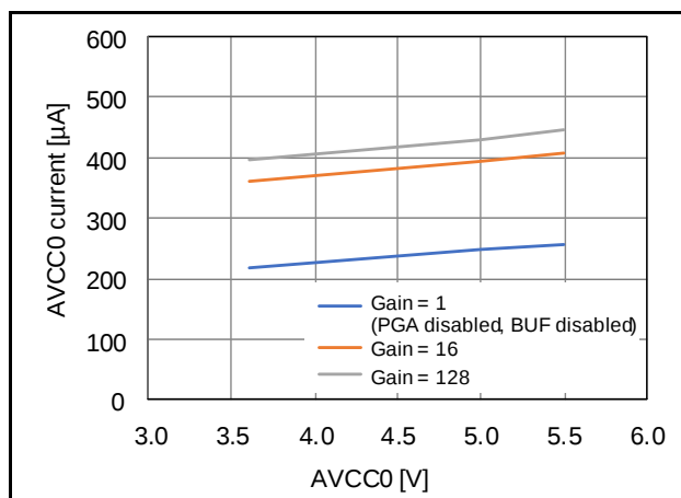
Figure 2.11 Power-Supply Voltage Dependence of Operating Current of 24-Bit Delta-Sigma A/D Converter ( T_a = 25^{\circ}\text{C} , Low Power Mode, OPCR.DSADLVM bit = 0)
