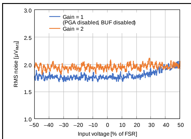
Figure 2.91 Input Voltage Dependence of RMS Noise (AVCC0 = 5.0 V, T_a = 25^\circ\text{C} , Normal Mode, f_{DR} = 122\text{ SPS} , V_{REF} = 2.5\text{V} )
