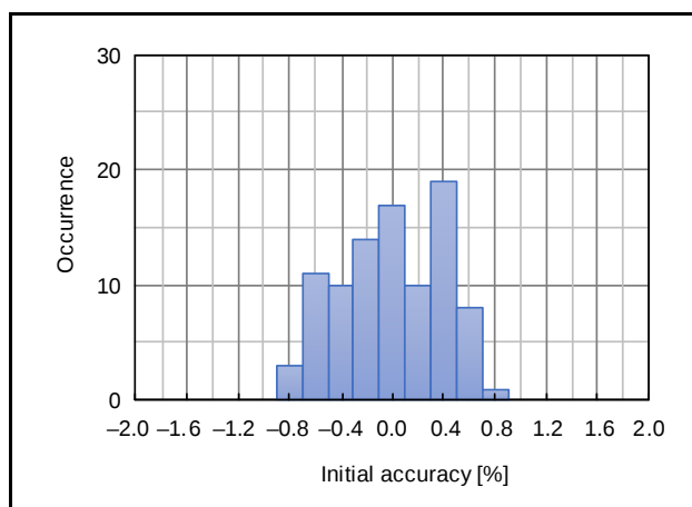
Figure 2.103 Initial Accuracy of Output Current of Excitation Current Source (AVCC0 = 5.0 V, T_a = 25^\circ\text{C} , I_{EXC} = 250\ \mu\text{A} , 93 samples)
