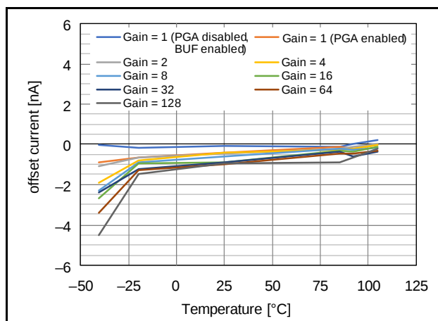
Figure 2.97 Temperature Dependence of Analog Input Offset Current (AVCC0 = 5.0 V)
