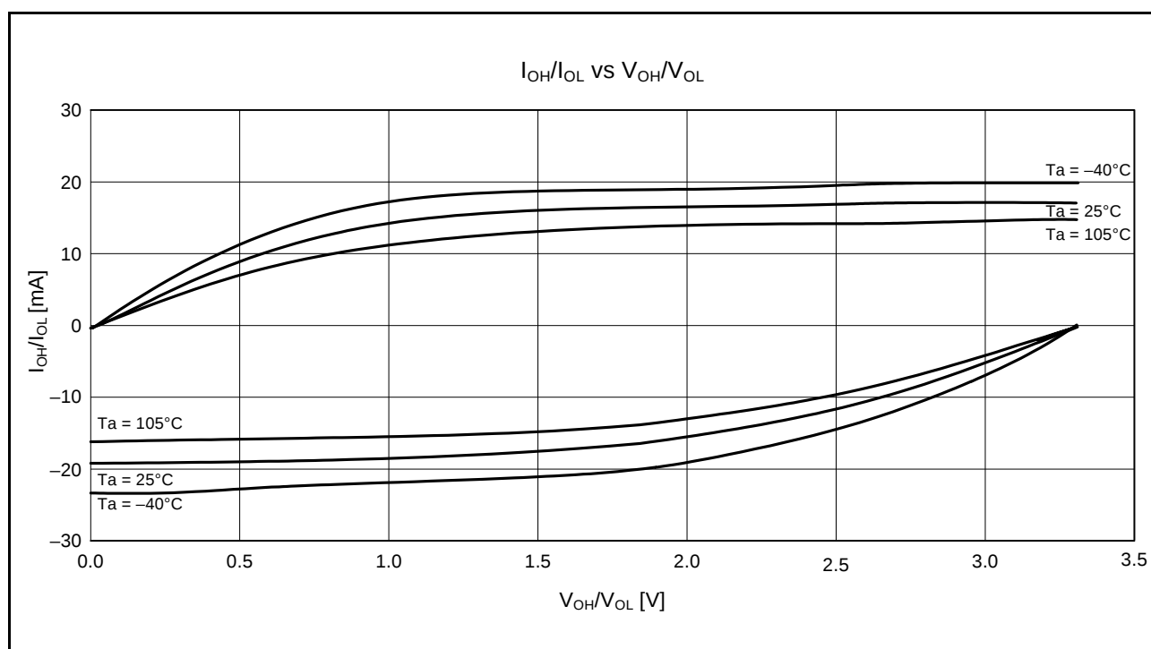
Figure 2.25 V_{OH}/V_{OL} and I_{OH}/I_{OL} Temperature Characteristics at V_{CC} = 3.3 V When Normal Drive Output is Selected (Reference Data)
