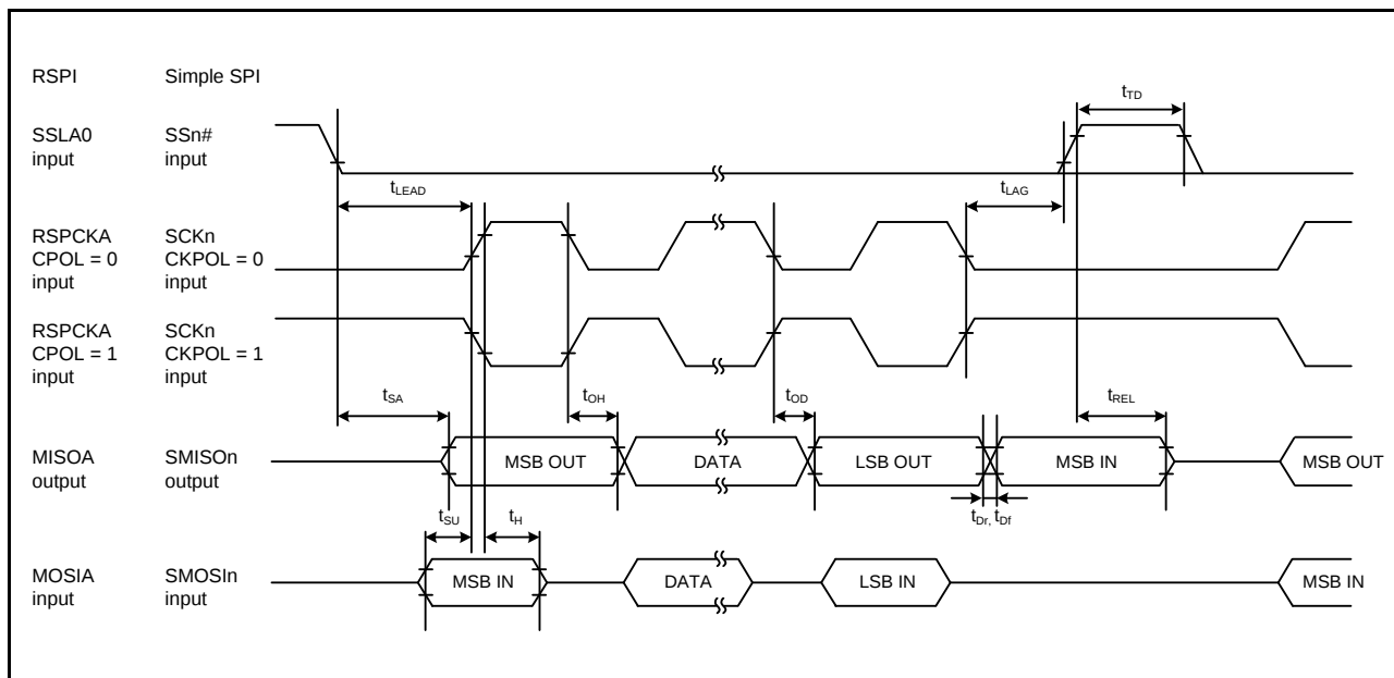
Figure 2.65 RSPI Timing (Slave, CPHA = 0) and Simple SPI Clock Timing (Slave, CKPH = 1) (n = 1, 5, 6, 12)
