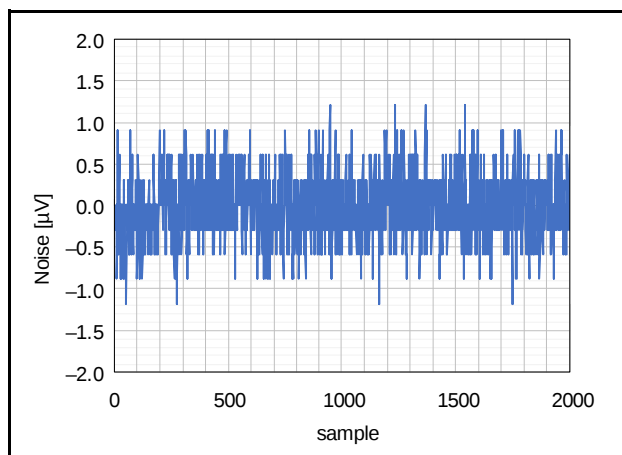
Figure 2.80 Plot of Noise (AVCC0 = 5.0 V, T_a = 25°C, Normal Mode, Gain = 1 (PGA disabled, BUF disabled), f_{DR} = 7.6 SPS, V_{ID} = 0V, V_{REF} = 2.5V)
