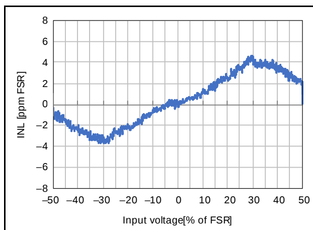
Figure 2.93 Input Voltage Dependence of Integral Non-Linearity (AVCC0 = 5.0 V, T_a = 25^\circ\text{C} , Normal Mode, Gain = 1 (PGA disabled, BUF disabled), OPCR.DSADLVM bit = 0, V_{\text{REF}} = 2.5\text{V} )
