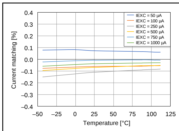
Figure 2.105 Temperature Dependence of Matching of Output Current of Excitation Current Source (AVCC0 = 5.0 V)
