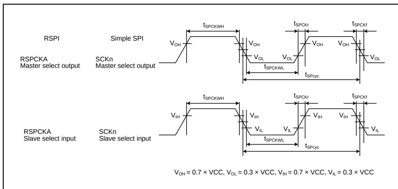
Figure 2.62 RSPI Clock Timing and Simple SPI Clock Timing (n = 1, 5, 6, 12)
