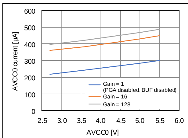
Figure 2.13 Power-Supply Voltage Dependence of Operating Current of 24-Bit Delta-Sigma A/D Converter ( T_a = 25^\circ\text{C} , Low Power Mode, OPCR.DSADLVM bit = 1)
