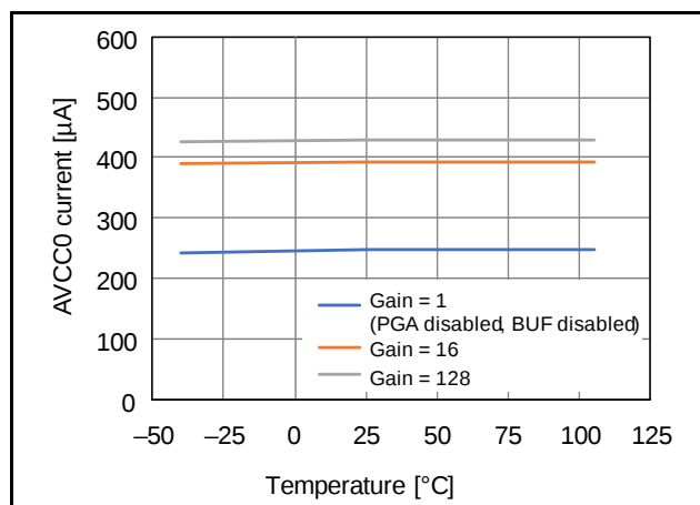
Figure 2.10 Temperature Dependence of Operating Current of 24-Bit Delta-Sigma A/D Converter (AVCC0 = 5.0 V, Low Power Mode, OPCR.DSADLVM bit = 0)
