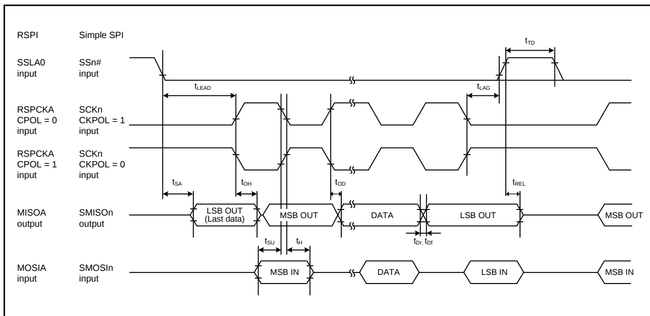
Figure 2.66 RSPI Timing (Slave, CPHA = 1) and Simple SPI Clock Timing (Slave, CKPH = 0) (n = 1, 5, 6, 12)
