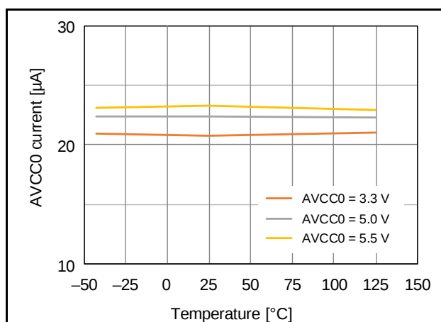
Figure 2.17 Temperature Dependence of Operating Current of Reference Buffer (Low Power Mode)
