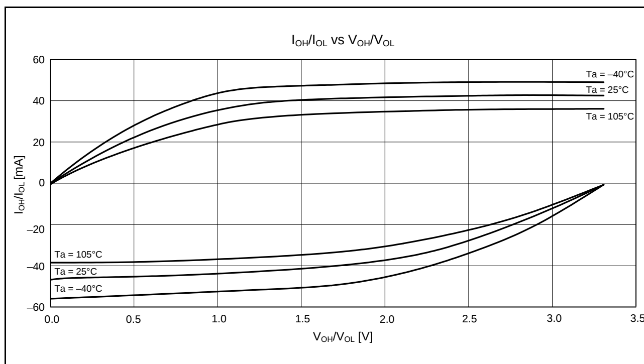
Figure 2.30 V_{OH}/V_{OL} and I_{OH}/I_{OL} Temperature Characteristics at V_{CC} = 3.3 V When High-Drive Output is Selected (Reference Data)
