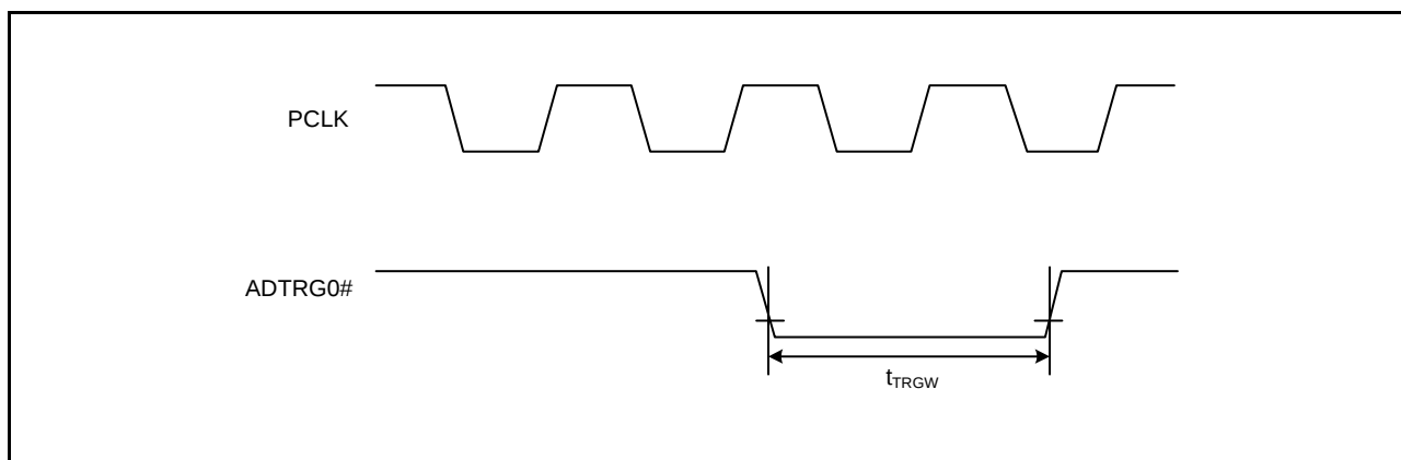
Figure 2.67 A/D Converter External Trigger Input Timing
