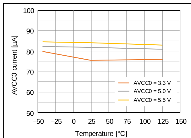
Figure 2.14 Temperature Dependence of Operating Current of Analog Input Buffer (Normal Mode)
