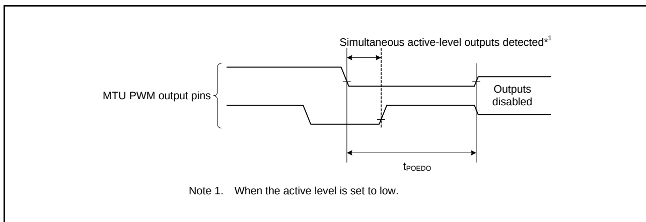
Figure 2.55 Output Disable Time for POE in Response to the Simultaneous Conduction of Output Pins
