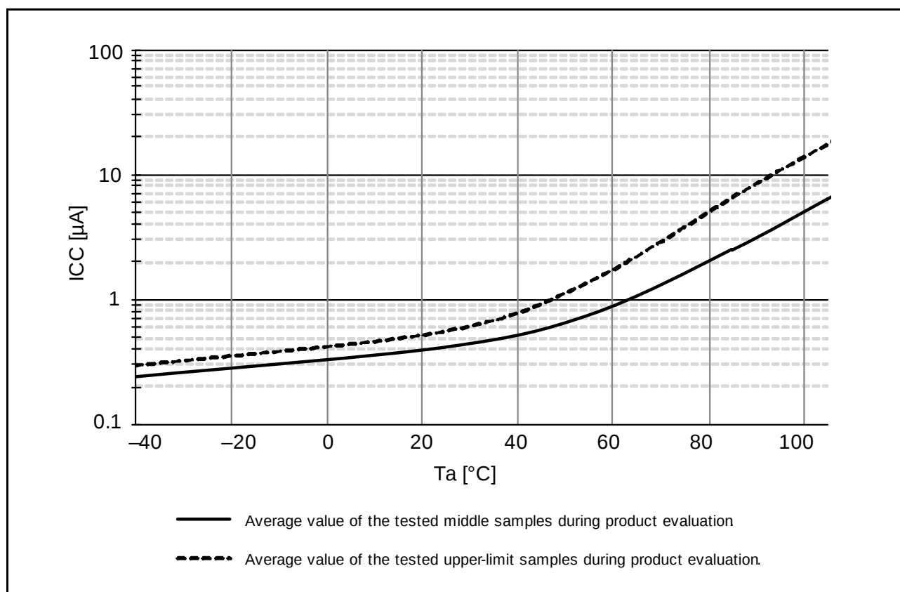
Figure 2.4 Temperature Dependence in Software Standby Mode (Reference Data)
