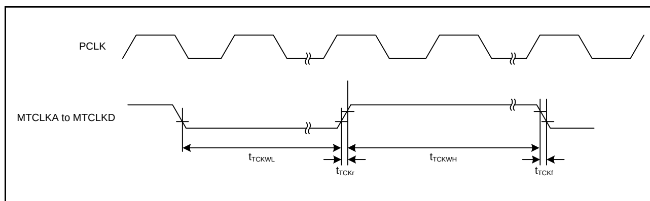
Figure 2.52 MTU Clock Input Timing
