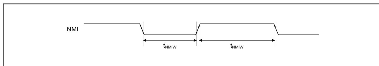
Figure 2.48 NMI Interrupt Input Timing
