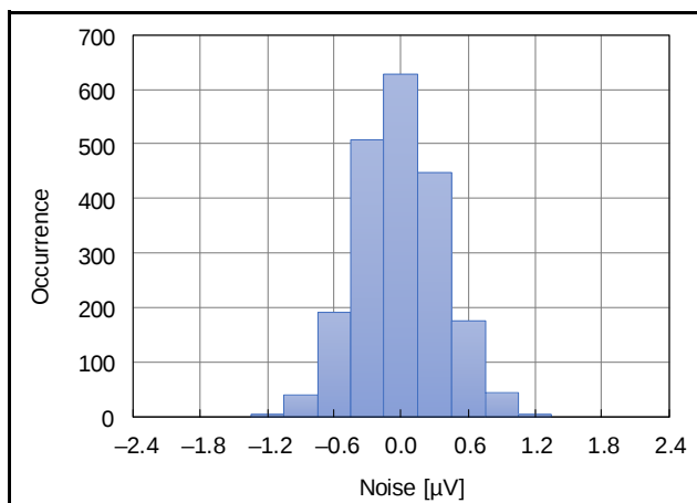
Figure 2.79 Noise Histogram (AVCC0 = 5.0 V, T_a = 25°C, Normal Mode, Gain = 1 (PGA disabled, BUF disabled), f_{DR} = 7.6 SPS, V_{ID} = 0V, V_{REF} = 2.5V)
