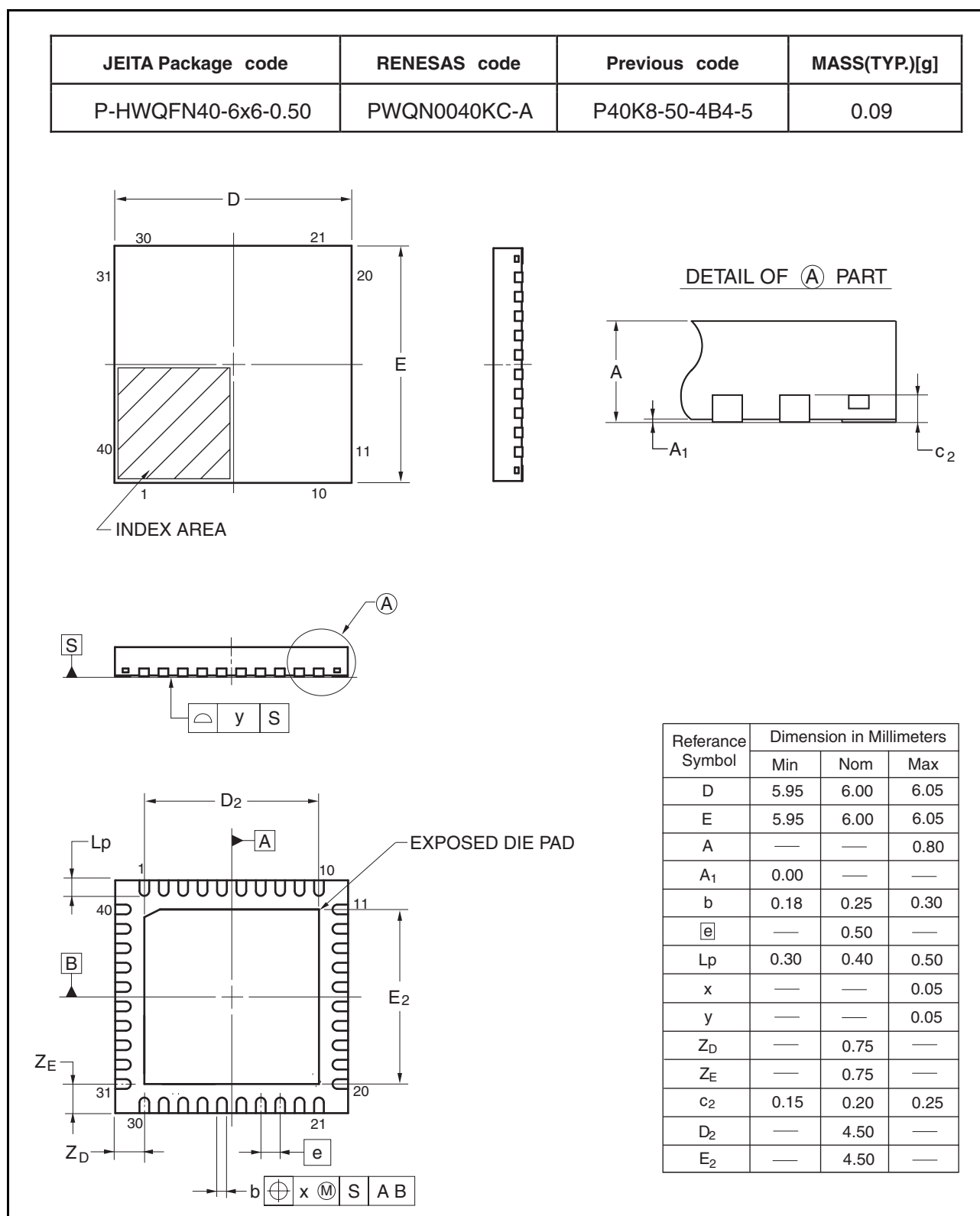
Figure B 40-Pin HWQFN (PWQN0040KC-A)
