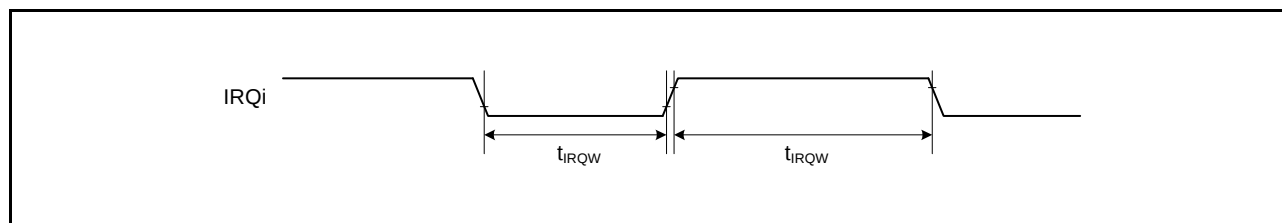
Figure 2.49 IRQ Interrupt Input Timing
