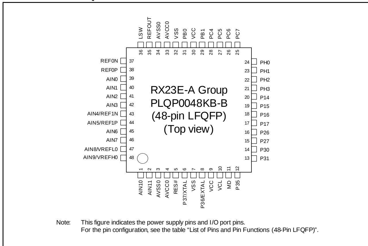
Figure 1.3 Pin Assignments of the 48-Pin LFQFP
