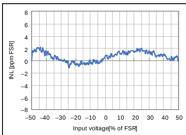
Figure 2.92 Input Voltage Dependence of Integral Non-Linearity (AVCC0 = 5.0 V, T_a = 25^\circ\text{C} , Normal Mode, Gain = 2, OPCR.DSADLVM bit = 0, V_{\text{REF}} = 2.5\text{V} )
