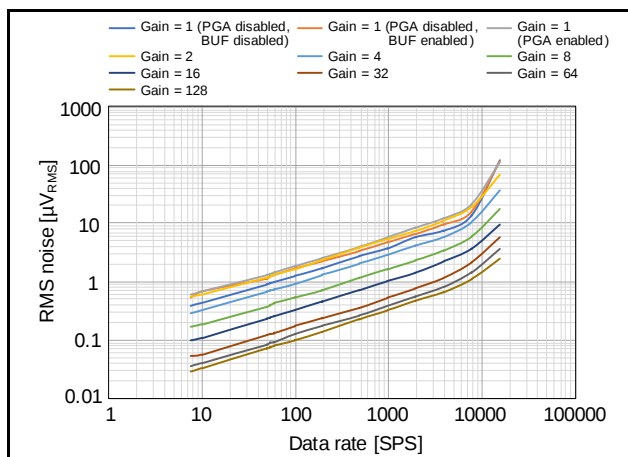
Figure 2.87 Data Rate Dependence of RMS Noise (AVCC0 = 5.0 V, T_a = 25^\circ\text{C} , Normal Mode, V_{ID} = 0\text{V} , V_{REF} = 2.5\text{V} )
