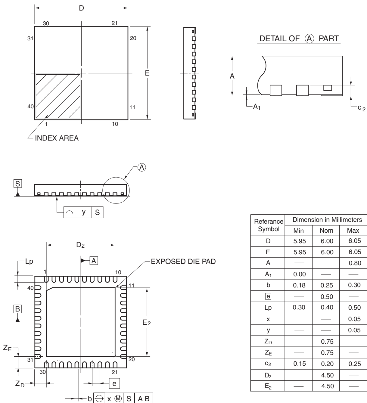
Figure B 40-Pin HWQFN (PWQN0040KC-A)
