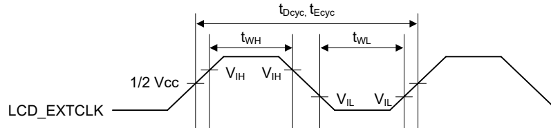
Figure 2.79 LCD_EXTCLK Clock Input Timing
