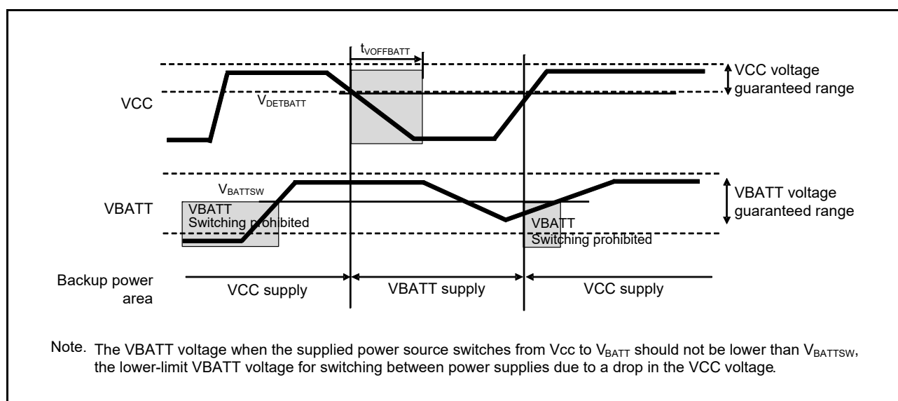
Figure 2.95 Battery Backup Function Characteristics
