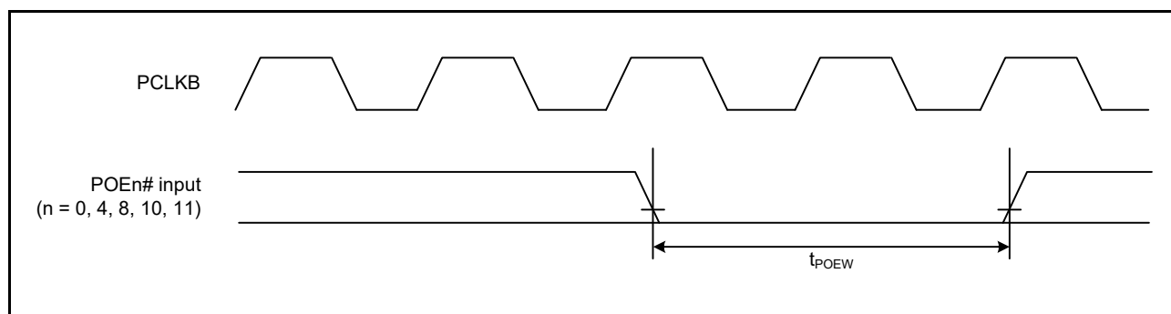
Figure 2.40 POE# Pin Input Timing
