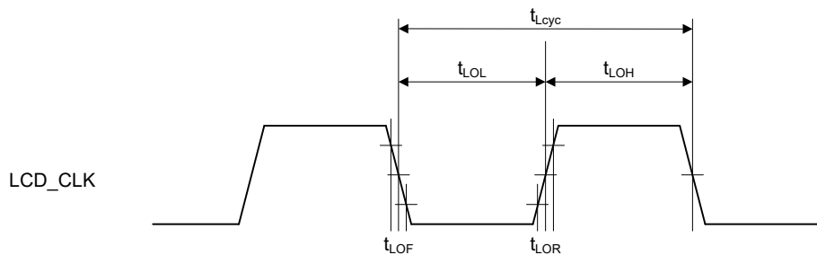
Figure 2.80 LCD_CLK Clock Output Timing
