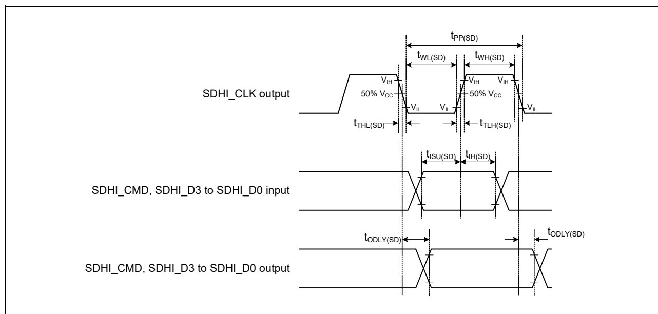
Figure 2.82 SD Host Interface Input/Output Signal Timing
