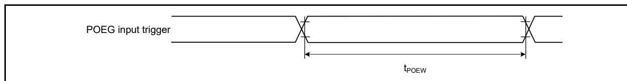
Figure 2.45 POEG input trigger timing
