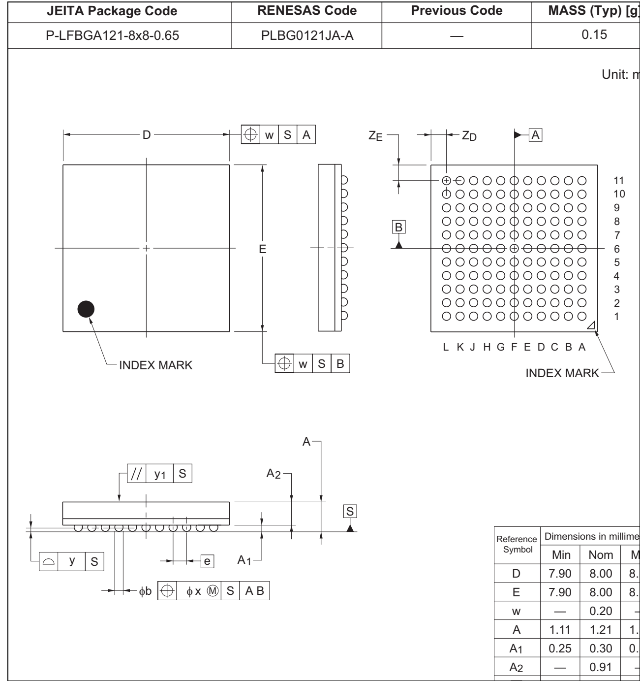
Figure 1.3 BGA 121-pin
