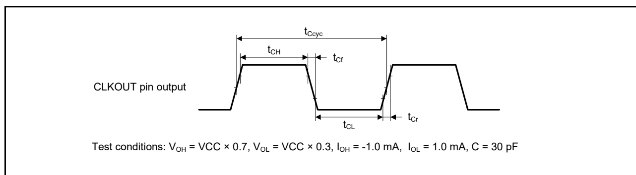
Figure 2.73 CLKOUT output timing
