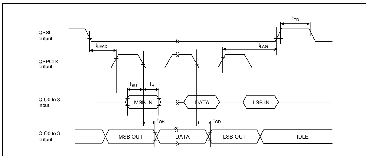
Figure 2.66 Transfer/receive timing
