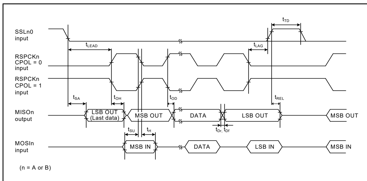
Figure 2.64 SPI timing (slave, CPHA = 1)
