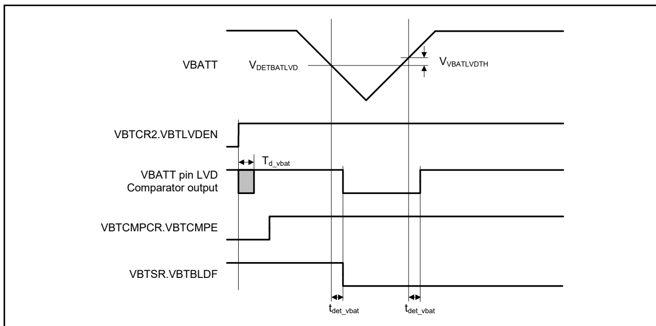
Figure 2.89 VBATT pin voltage detection circuit timing
