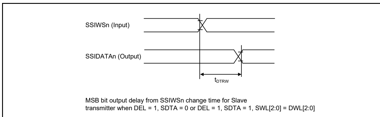
Figure 2.71 SSI data output delay from SSIWSn change time
