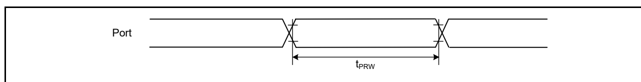
Figure 2.44 I/O ports input timing
