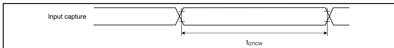
Figure 2.46 GPT input capture timing
