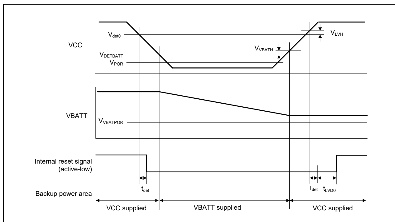
Figure 2.87 Power supply switching and LVD0 reset Timing
