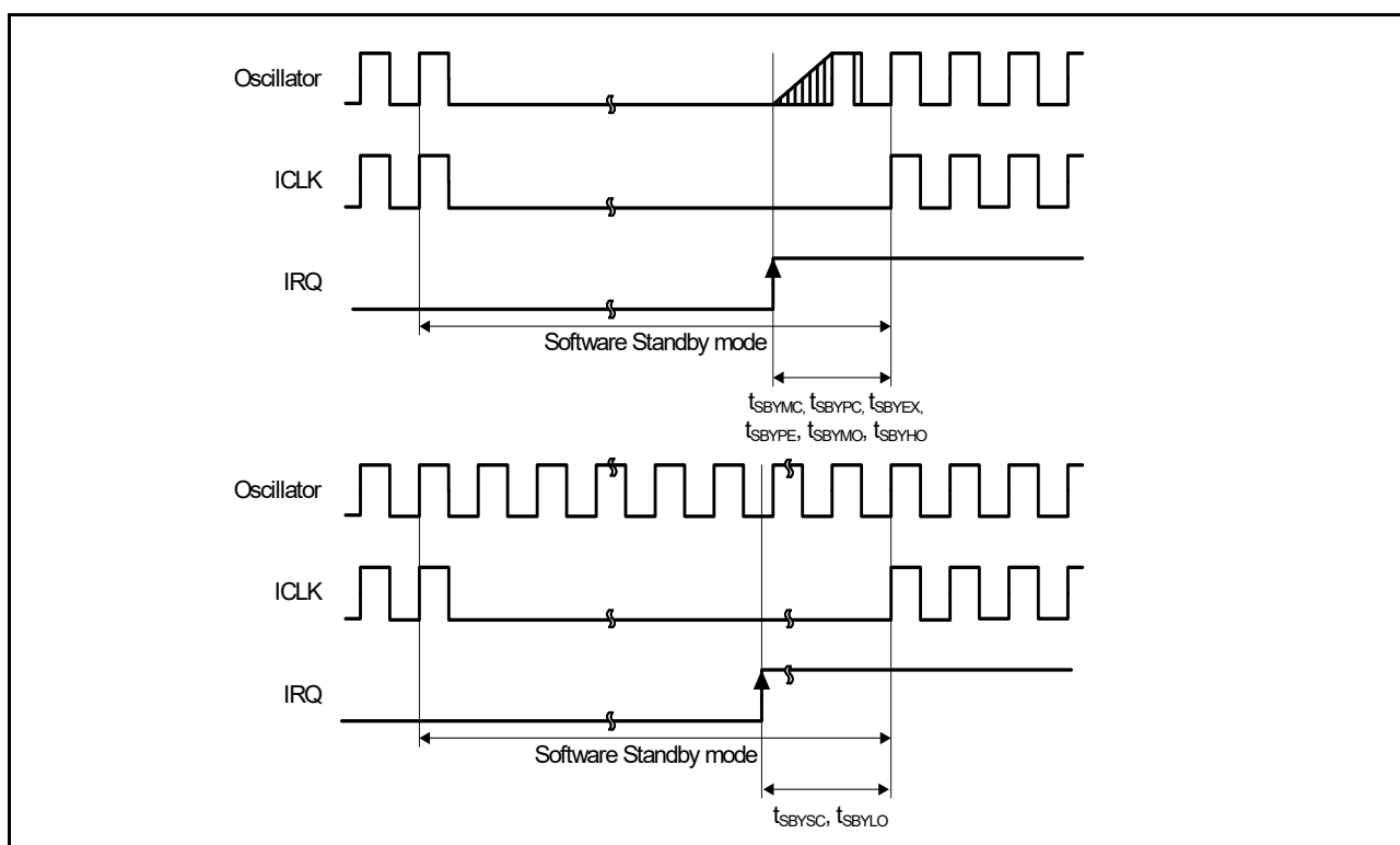
Figure 2.35 Software Standby mode cancellation timing
