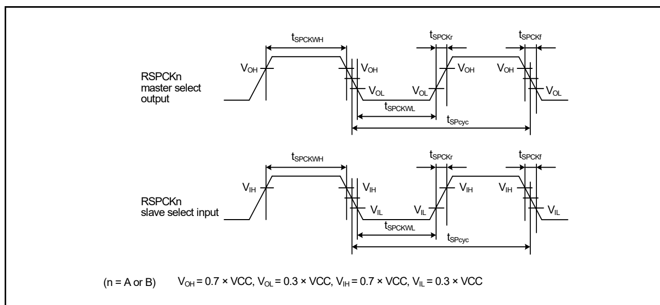
Figure 2.58 SPI clock timing
