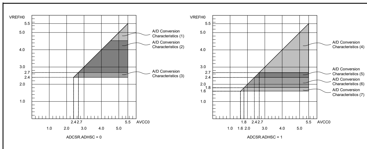
Figure 2.77 AVCC0 to VREFH0 voltage range
