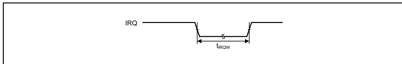
Figure 2.38 IRQ interrupt input timing
