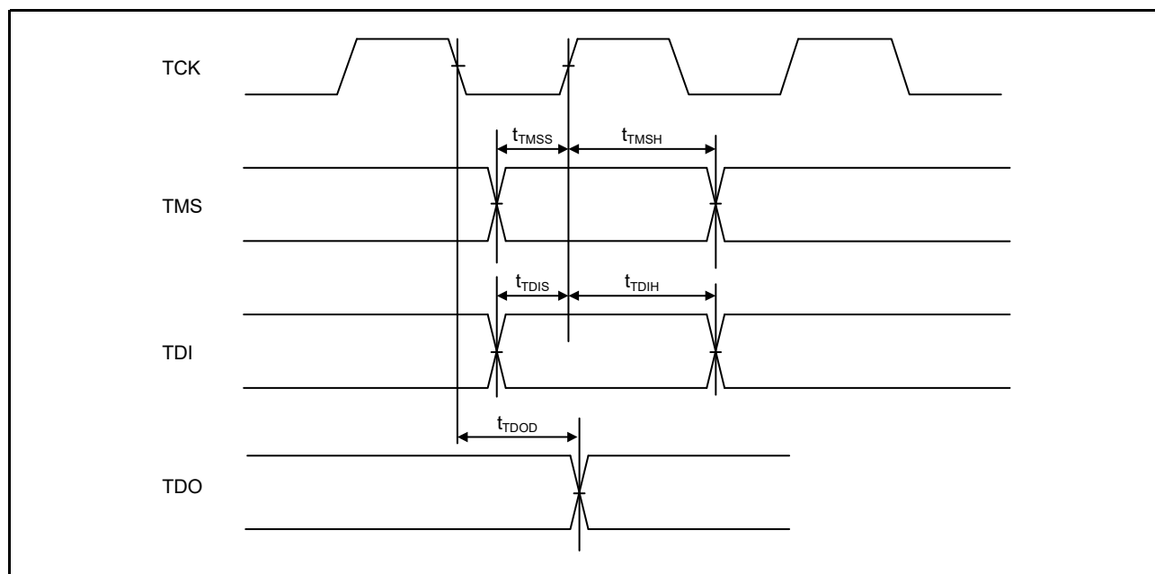
Figure 2.95 JTAG input/output timing
