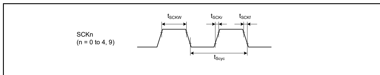
Figure 2.50 SCK clock input timing
