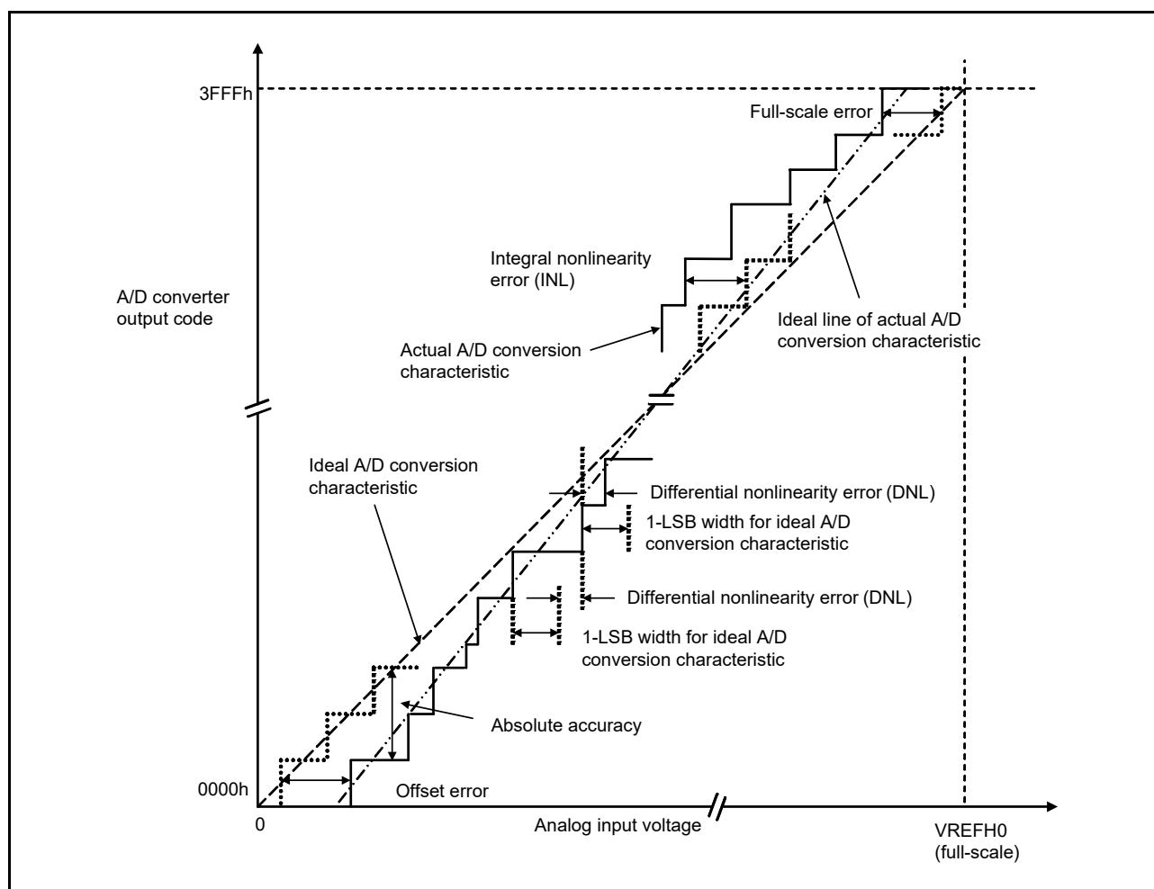
Figure 2.79 Illustration of 14-bit A/D converter characteristic terms
