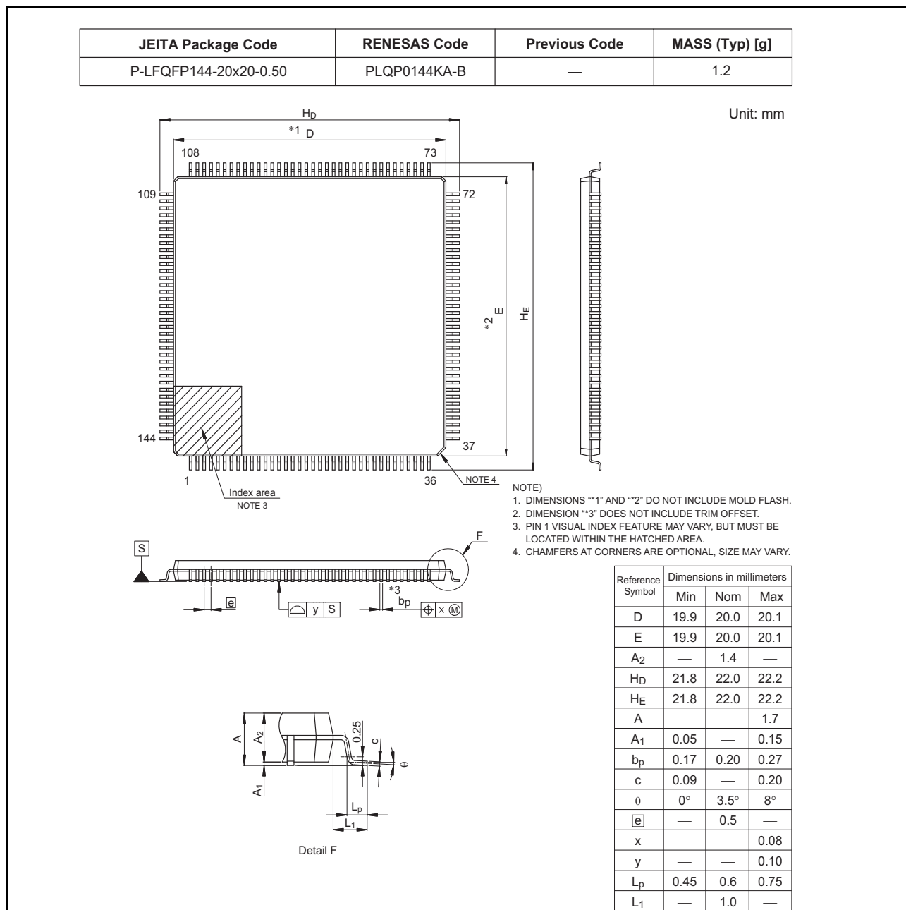
Figure 1.2 LQFP 144-pin
