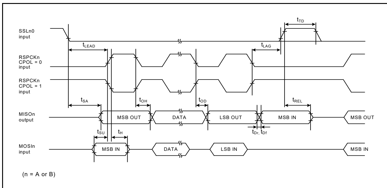
Figure 2.63 SPI timing (slave, CPHA = 0)
