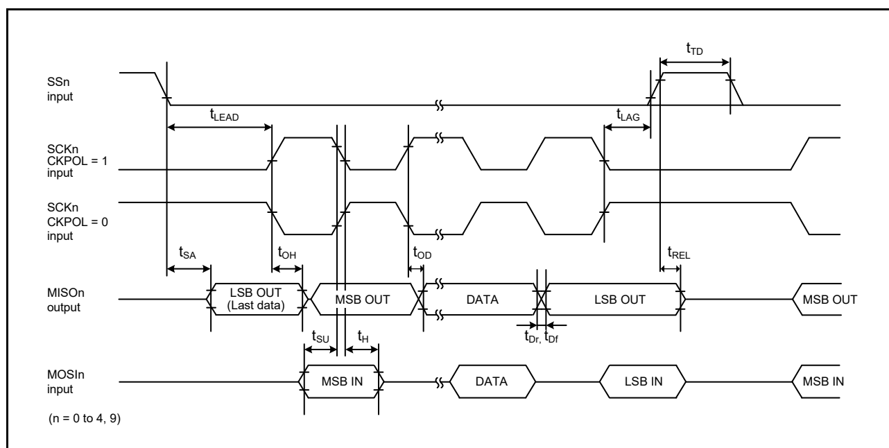
Figure 2.56 SCI simple SPI mode timing (slave, CKPH = 0)
