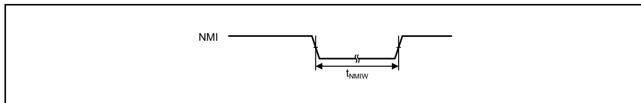
Figure 2.37 NMI interrupt input timing
