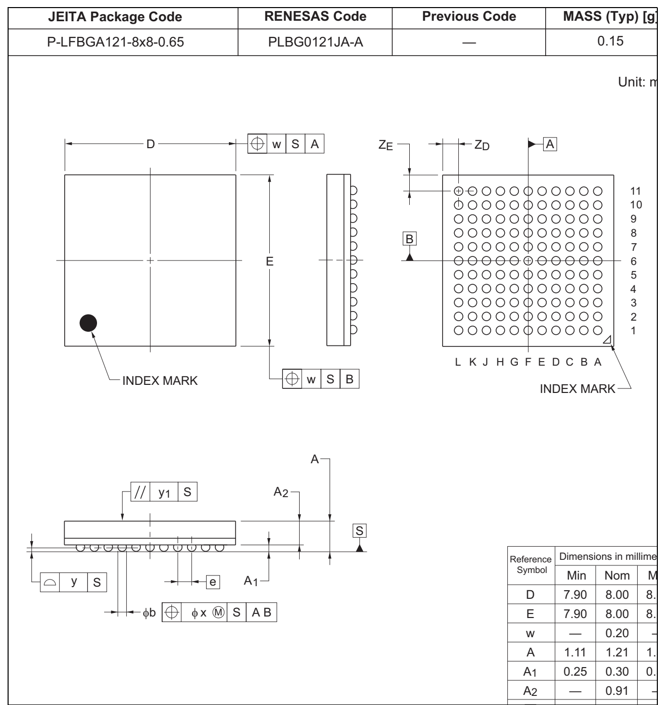
Figure 1.3 BGA 121-pin
