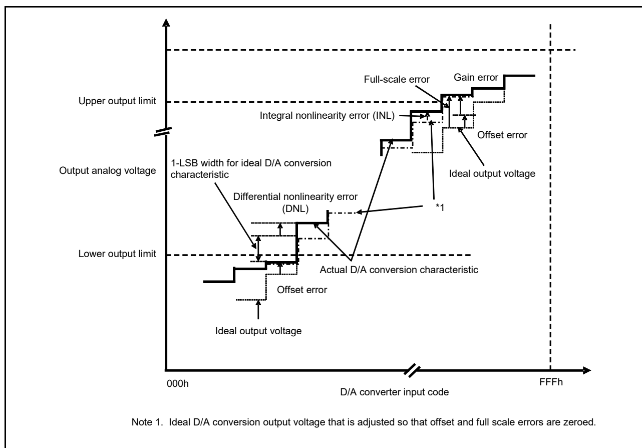
Figure 2.80 Illustration of D/A converter characteristic terms
