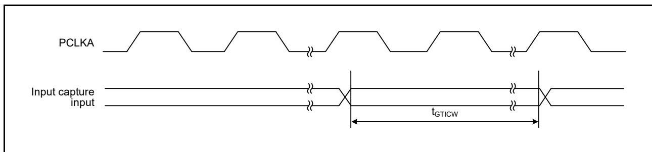
Figure 5.40 Input Timing of GPT Input Capture
