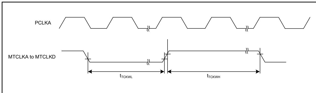
Figure 5.38 MTU3 Clock Input Timing
