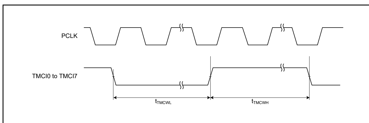
Figure 5.43 TMR Clock Input Timing
