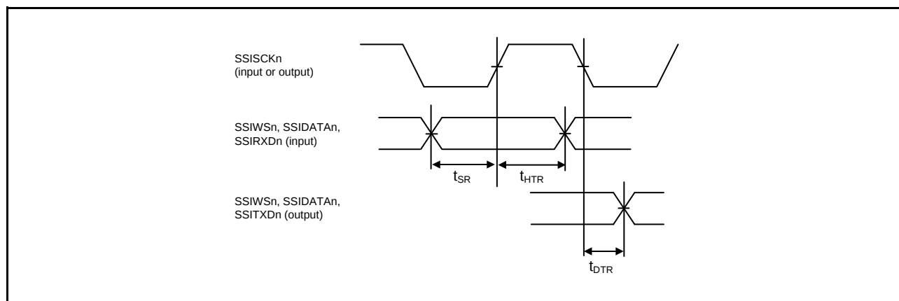
Figure 2.67 Transmit/Receive Timing (SSISCKn Rising Synchronous)
