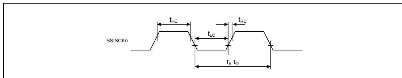
Figure 2.66 Clock Input/Output Timing
