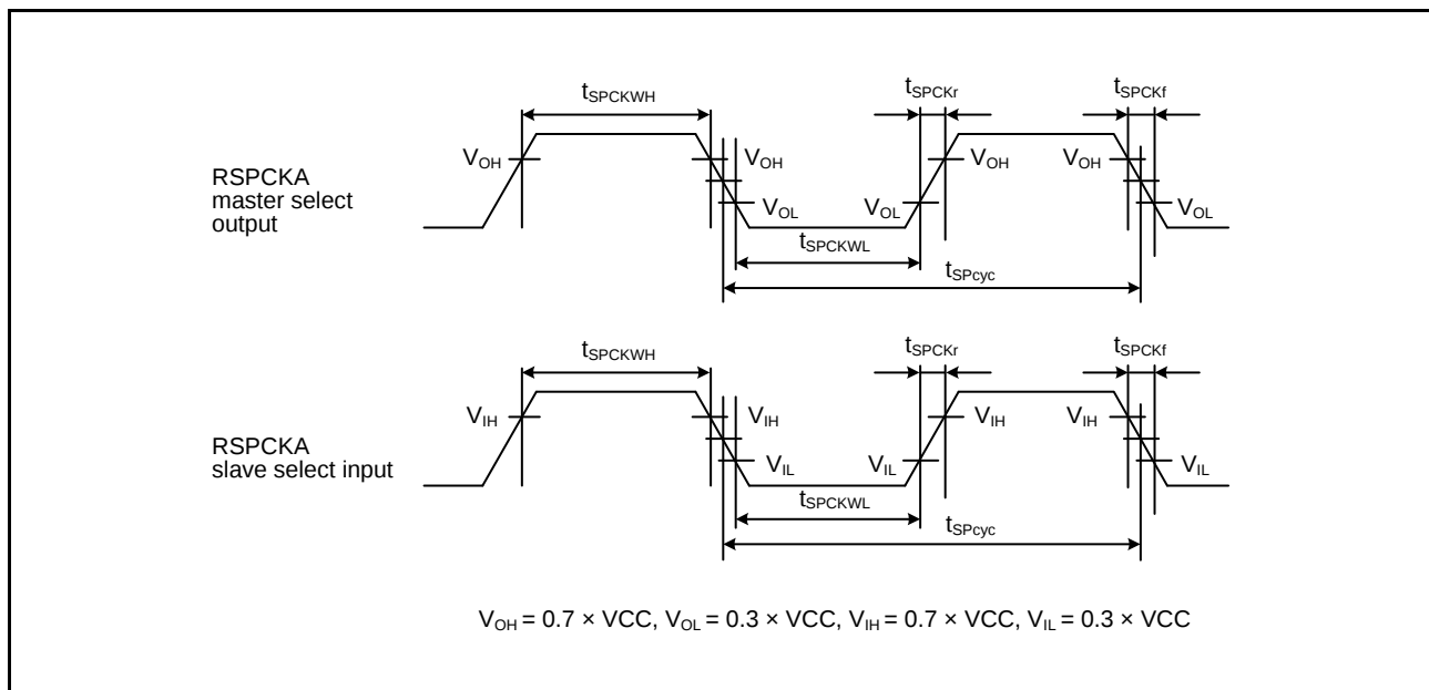
Figure 2.56 RSPI Clock Timing
