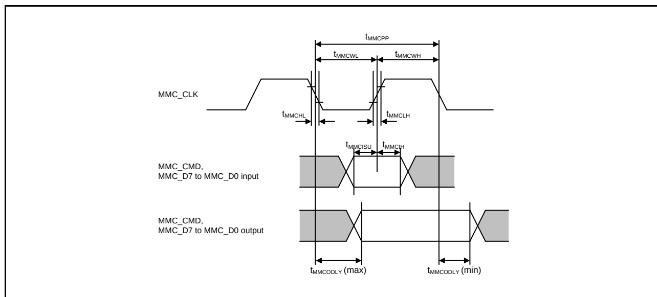
Figure 2.70 MMC Interface
