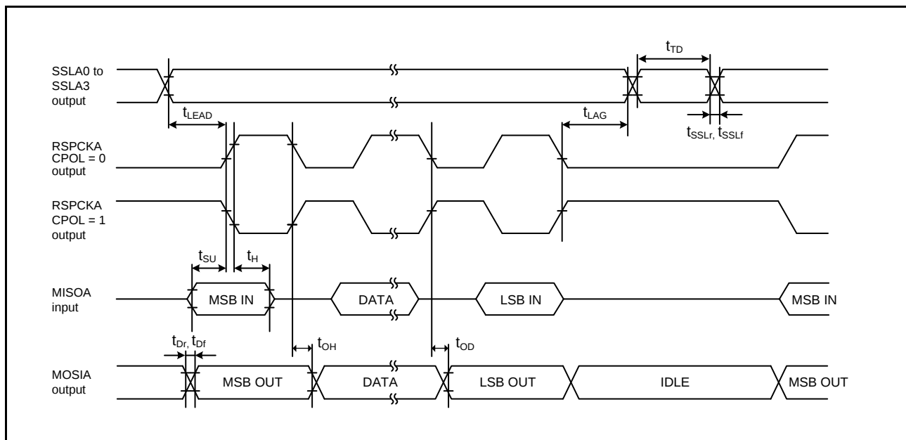
Figure 2.57 RSPI Timing (Master, CPHA = 0) (Bit Rate: PCLKA Division Ratio Set to a Value Other Than 1/2)
