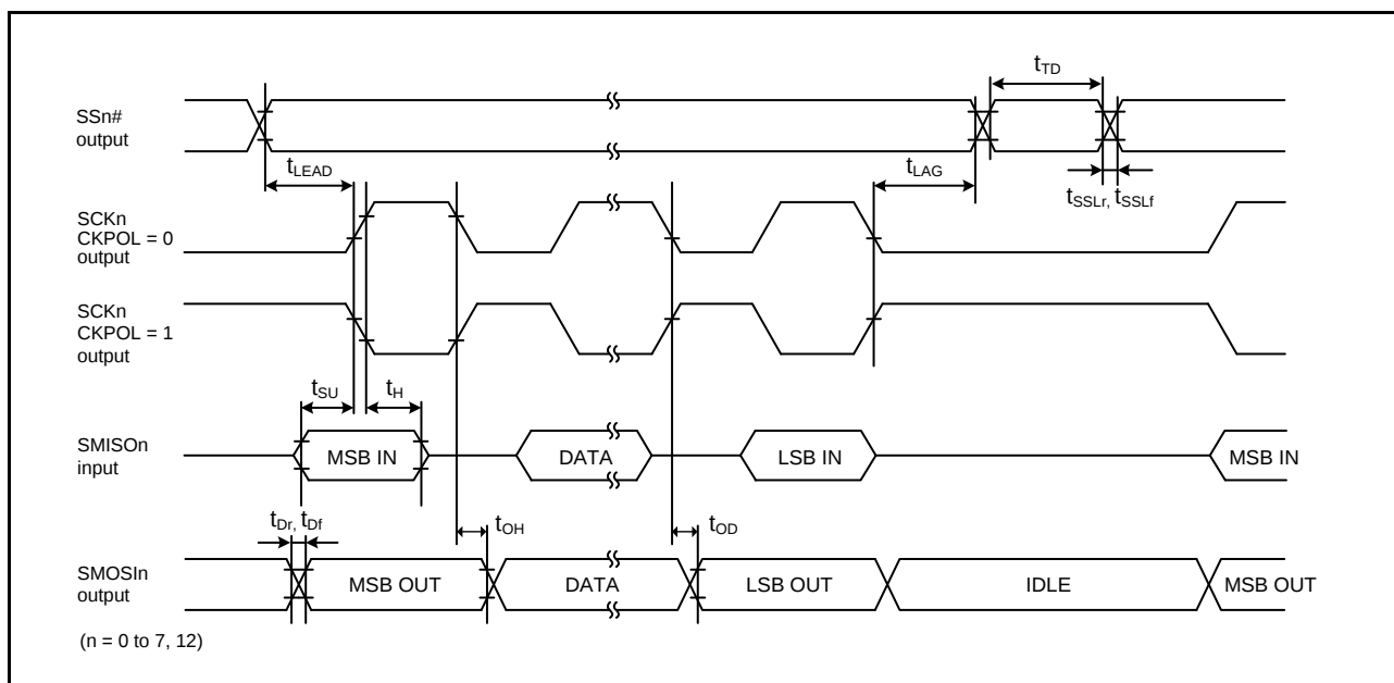
Figure 2.51 Simple SPI Timing (Master, CKPH = 1)
