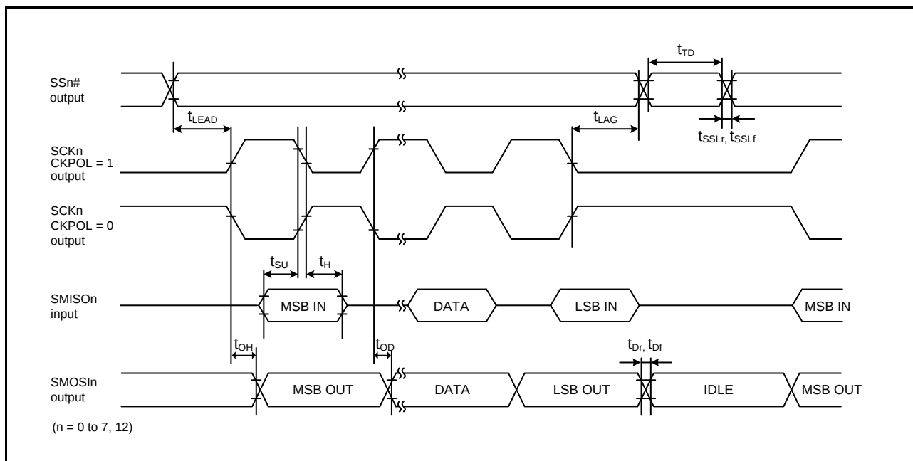
Figure 2.52 Simple SPI Timing (Master, CKPH = 0)
