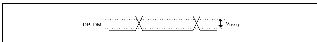
Figure 2.90 DP and DM Squelch detect sensitivity (High-Speed)
